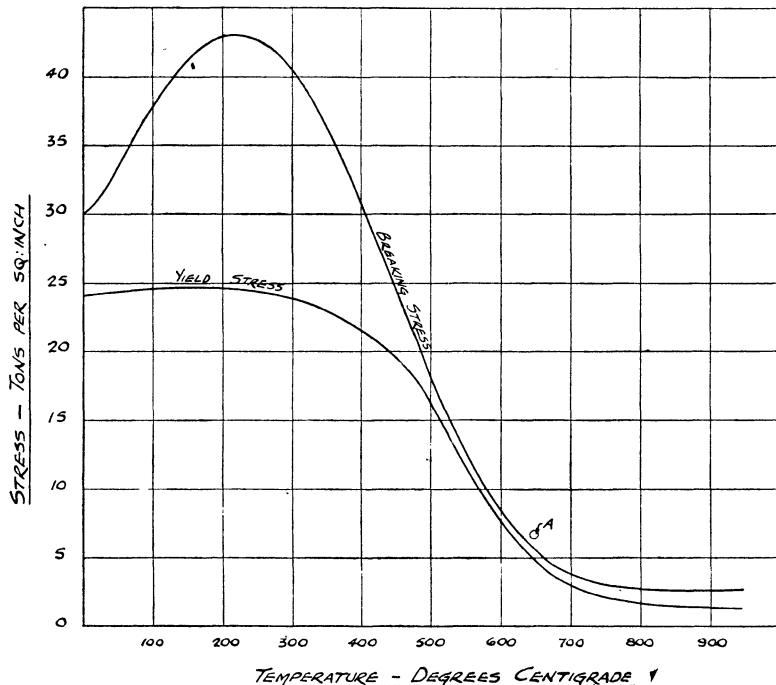
Fig. 6.—Effect of Temperature on Strength of Mild Steel.
