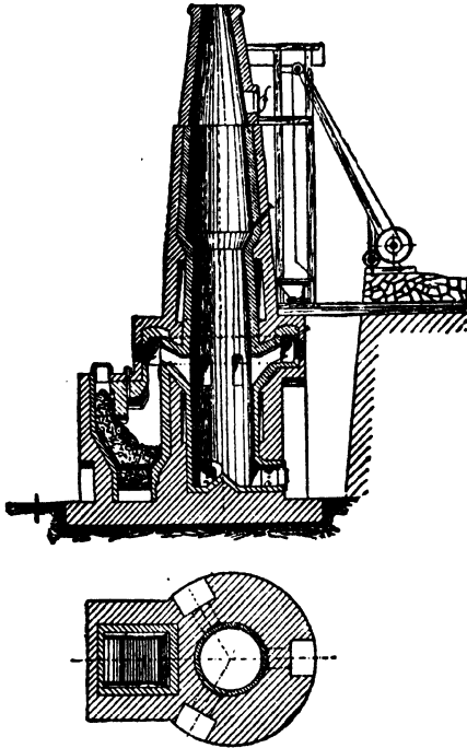
FIG. 4.—Schmatolla's Kiln.
