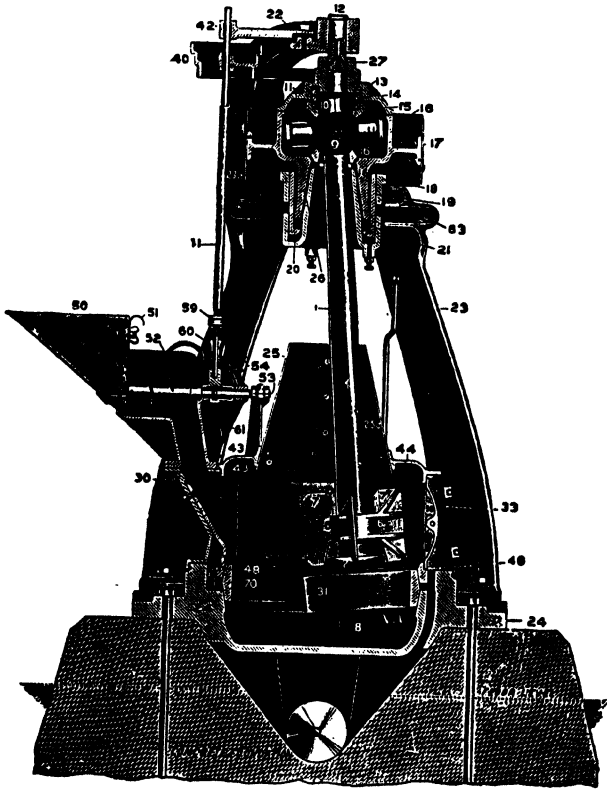
FIG. 10.—Section of Griffin Mill.
