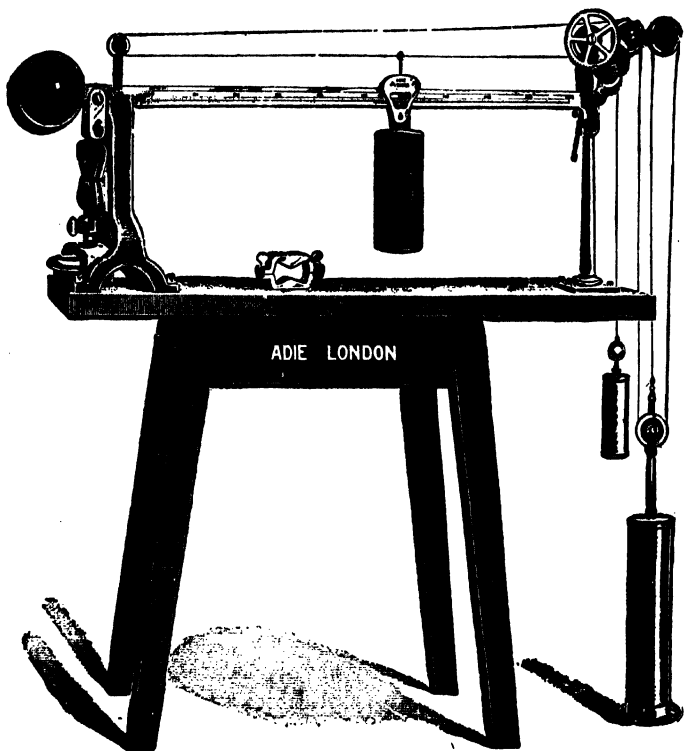
FIG. 20.—The Adie testing machine.
