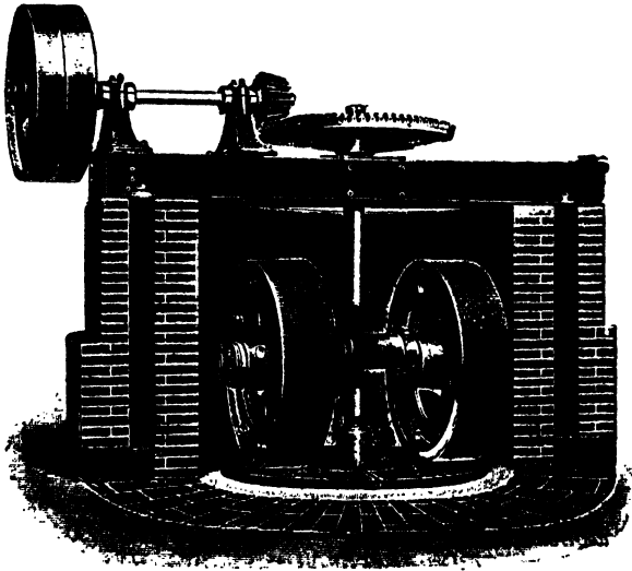
FIG. 5.—Wet Edge-Runner.
