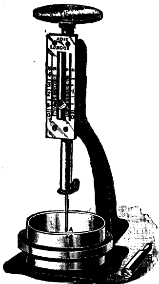
FIG. 17.—The Vicat Needle.
