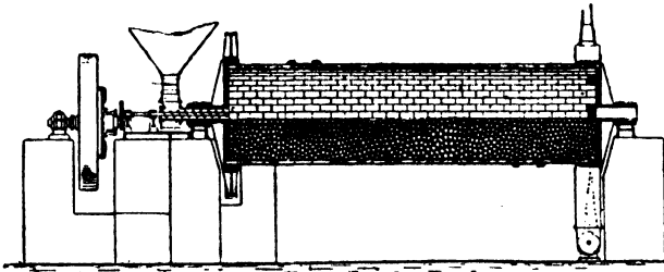
FIG. 9.—Section of Davidsen Tube-Mill.
