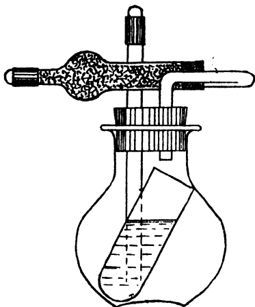
FIG. 15.—Apparatus for Estimation of \text{CO}_2 .
