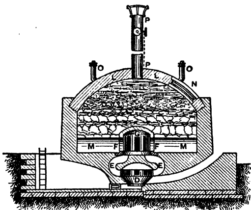
FIG. 14.—Transverse Section of the Dumesnil Kiln.
