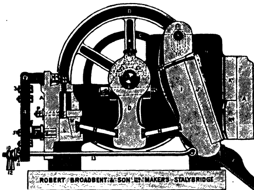
FIG. 7.—Section of Broadbent's Improved Blake Stonebreaker.
