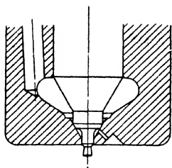
C.A.V. "Pintaux" nozzle showing auxiliary spraying hole beneath valve seat; the curves indicate its performance characteristics
