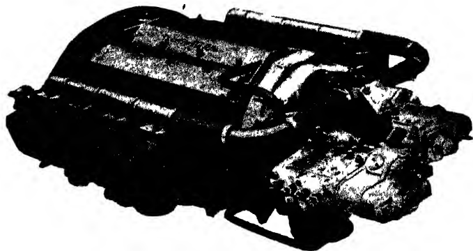
Tilling-Stevens horizontally opposed eight-cylinder flat diesel
