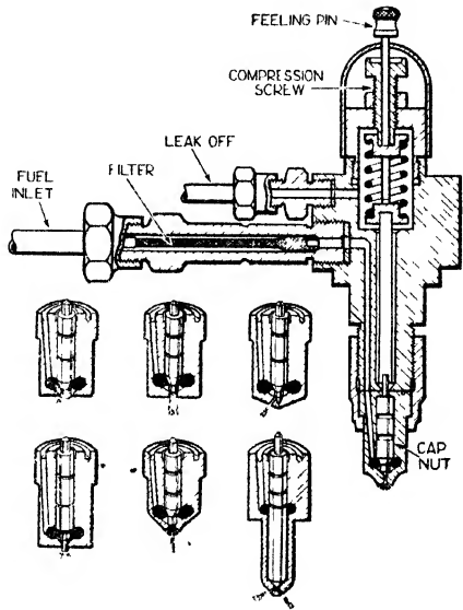
C.A.V. fuel injector and different types of nozzle
