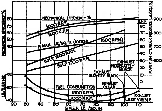
Curves indicating in full the technical qualities of the four-cylinder 44-60 h.p. Paxman-Ricardo
