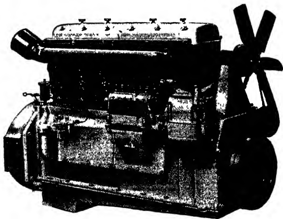
Pre-war six-cylinder 130 × 170 mm M.W.M. engine, which developed 150 b.h.p. at 1,600 r.p.m.
