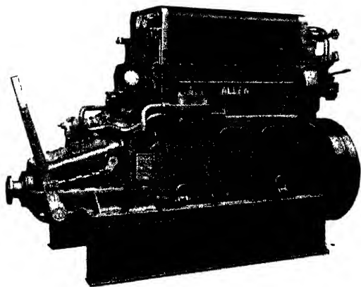
Three-cylinder 94/116 h.p. Allen marine diesel with mechanical reverse gear
