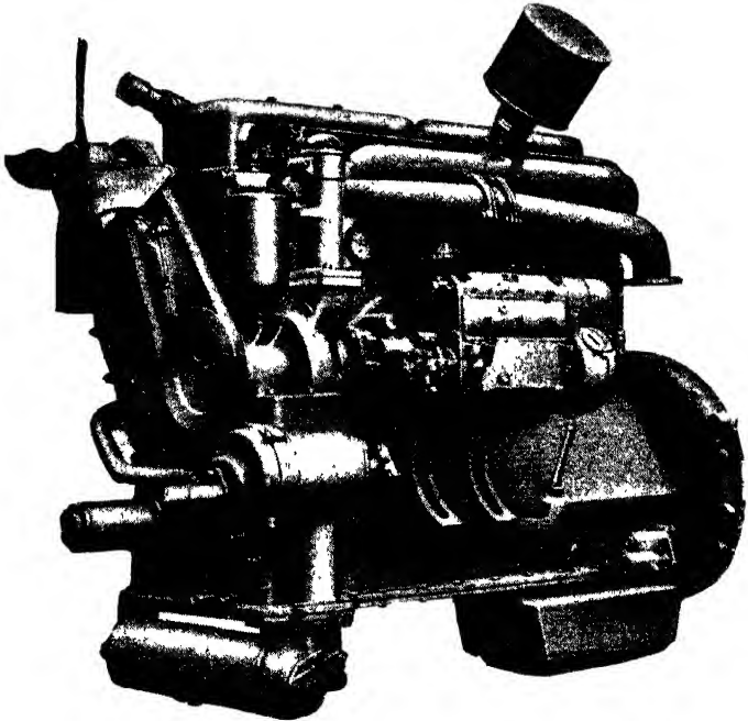
Crossley direct-injection six-cylinder 102·7 b.h.p. 8·6-litre bus engine
