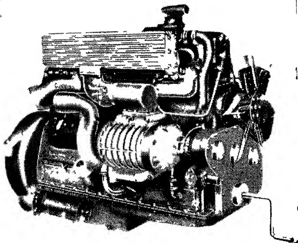
One of the earliest and still one of the most original American transport diesels, the Cummins 11,000 c c six-cylinder four-stroke engine, which develops 150 b h p at 1,800 r p m or 200 b h p when supercharged (as shown)
