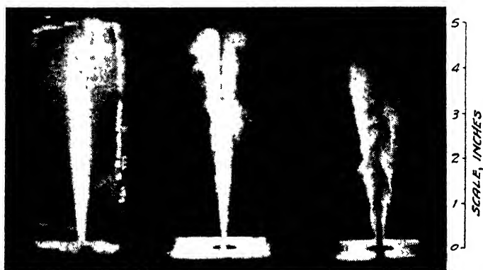
Fiedler's ciné film of a four-hole spray in the combustion chamber. White specks in (3) indicate early combust. of dissociated hydrogen
