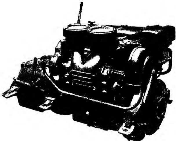
The four-cylinder 110 h.p. G.M.C. two-stroke
