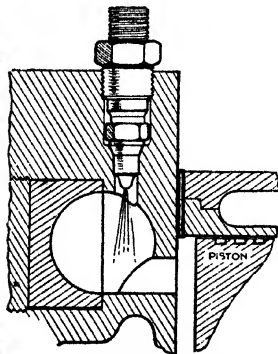
Cub combustion chamber
