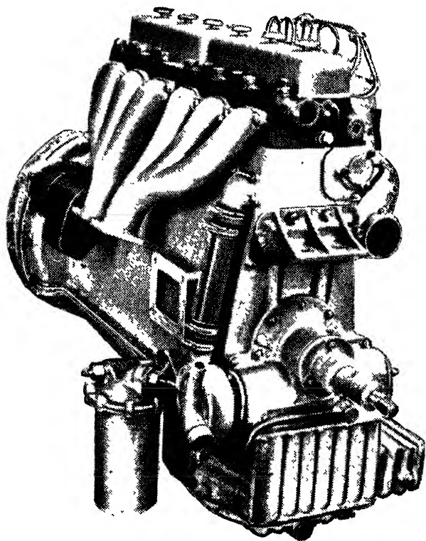
Off side of Foden engine, showing the exhaust manifold
