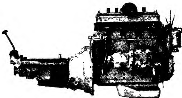
Godiva 2¼-litre engine with clutch and gear box for a private car
