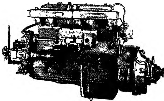
Thornycroft 60/90 b.h.p. six-cylinder marine engine with oil operated reversing gear
