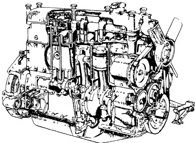
Leyland 5-litre 75 b.h.p. six-cylinder engine
