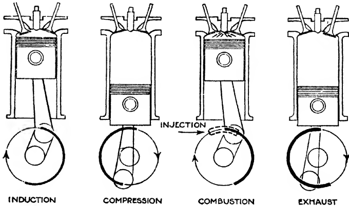
Four-stroke cycle of operations in a heavy-oil engine during two revolutions of the crankshaft
