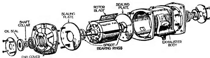
Constructional details of the Clayton Dewandre six-vane exhaustor, with special blade control and end sealing features
