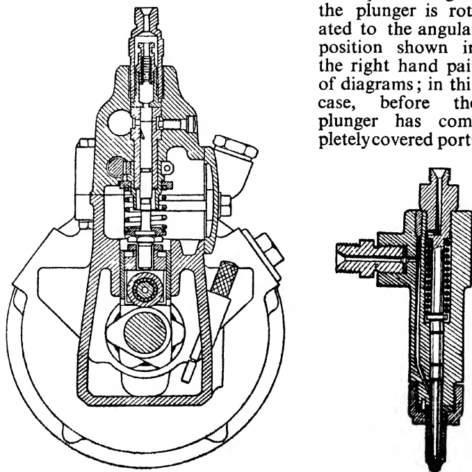
Cross-section of the Simms PA pump and (right) of the injector
