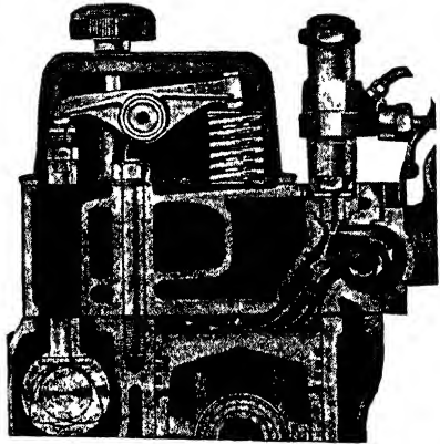
Perkins Aeroflow combustion head
