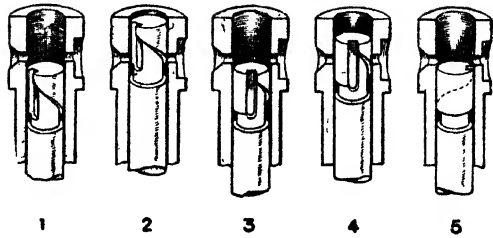
Illustrating the injection cycle of the C.A.V. fuel pump
