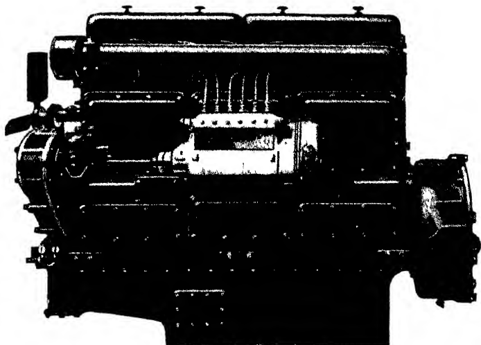
A pre-war French design, the 130 h.p. six-cylinder Renault
