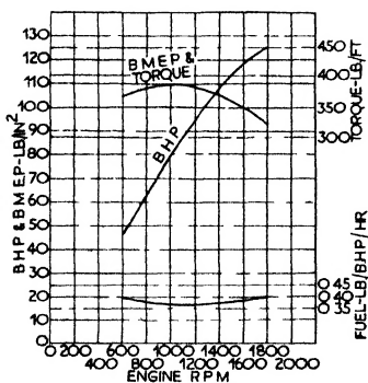
TYPICAL BRITISH HIGH-SPEED DIESEL Sectioned view of a 9.6 litre 125 b.h.p. road transport engine with performance curves
