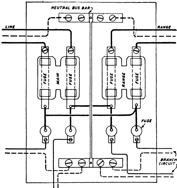
Fig. 14. Wiring Diagram for Enclosed Pull-Out Switch
