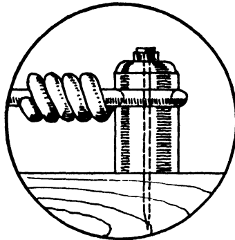
Fig. 40. Dead-Ending a Wire at a Knob Courtesy of James Steel Mahan
