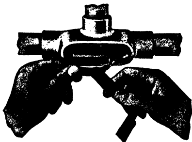
Fig. 30. Taping Splice in Conduit Fitting Courtesy of Crouse-Hinds Company
