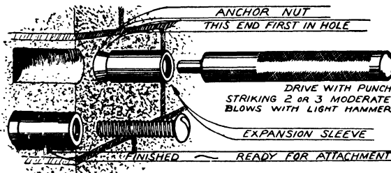
Fig. 50. Method of Setting A-J Anchors
