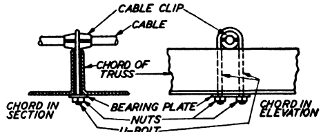
Fig. 47. Method of Holding Messenger Cable to Truss
