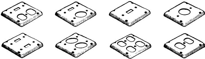
Fig. 30. Covers for Exposed Outlet Boxes Courtesy of the M. B. Austin Company, Chicago, Illinois
