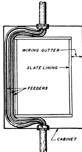
Fig. 29. The Wrong Way of Running a Feeder Through a Cabinet. Note the Four Sharp Bends in the Wire
