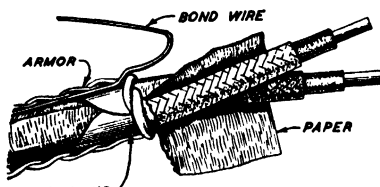
Fig. 16. Armored Cable Bond Wire
