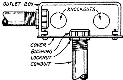
Fig. 45. Fastening Reflector to Outlet Box
