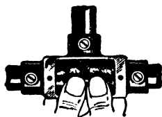
Fig. 31. Pushing Splice in Conduit Fitting
