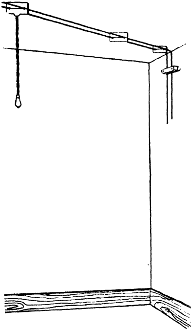
Fig. 35. Drop Cord Suspended from Cleat
