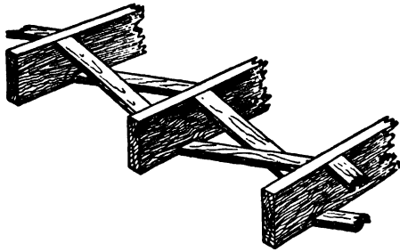
Fig. 46. Cross Bridging Between Floor Joists
