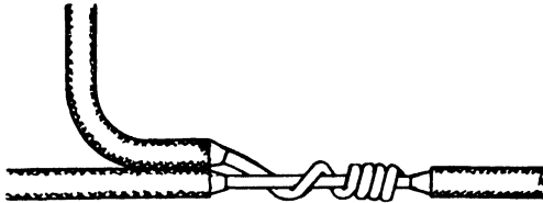
Fig. 56. Tee Tap on Solid Wire
