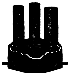
Fig. 62. Cutaway View of Installation of Conduit to Concrete Box, Using Bushlocks and Clamping Plates
