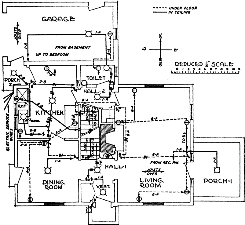
Fig. 3. Wiring Plan of First Floor of 1 1/2-Story Building
