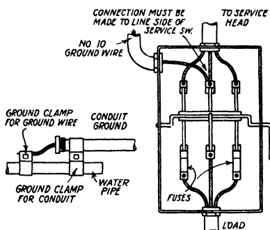
Fig. 28. Method of Grounding Conduit and Neutral Wire
