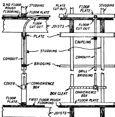
Fig. 14. Method of Installing Conduit to Convenience Outlets or Switch Boxes
