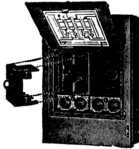
Fig. 13. Combined Main and Range Switches, Fuse Puller, and Branch Circuit Fuses Courtesy of The Arrow-Hart and Hegeman Electric Company
