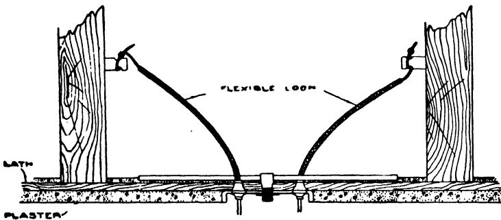
Fig. 51. Shallow Outlet Box Supported by Metal Box Hanger Laid Across Lath
