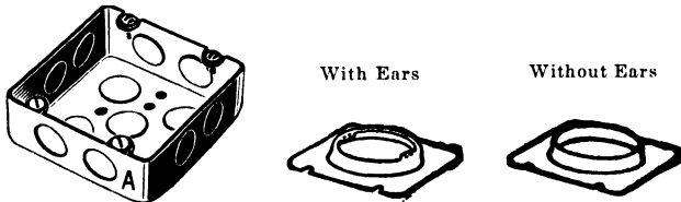
Fig. 11. Square Outlet Box and Plaster Ring Covers, with and without Ears Courtesy of the M. B. Austin Company, Chicago, Illinois
