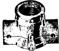
Fig. 38. Standard Key Socket Cleat Courtesy of Pass and Seymour
