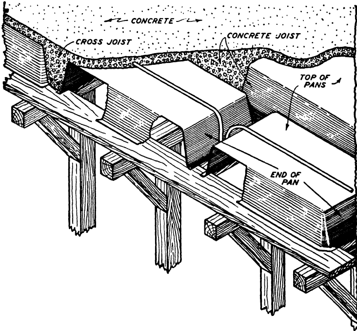
Fig. 60. Method of Installing Outlet in a Cross-Joist by the Use of Pans
