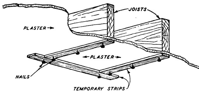
Fig. 42. Temporary Strips for Supporting Plaster When Cutting a Scuttle Hole
