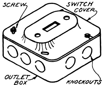
Fig. 11. Standard Outlet Box with Tumbler Switch Cover
