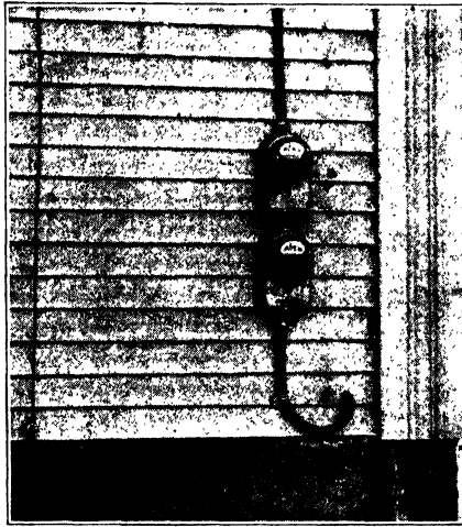
Fig. 8. Service Entrance Cable Installed on a Two-Family Meter Service Courtesy of Anaconda Wire and Cable Company
