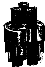
Fig. 38. Methods of Supporting Cables in Vertical Conduit Courtesy of Russell and Stoll Company
