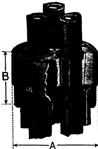
Fig. 14. Cross-Sectional View of a Cable Support for a Vertical Cable Run Courtesy of the Russell & Stoll Company, New York City
