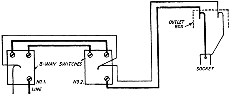
Fig. 59. Wiring Three-Way Switches with Current Fed to First Switch
