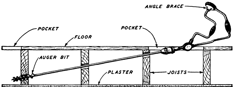
Fig. 50. Boring Floor Joists with an Extension Bit
