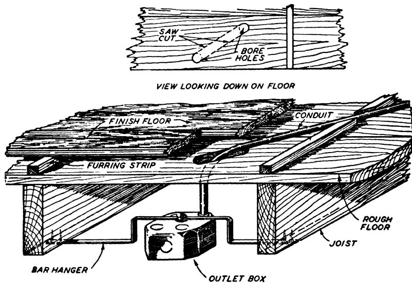
Fig. 72. View Showing Installation of Conduit in Wooden Floor Construction
