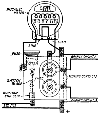
Fig. 29. Wiring Diagram of Meter and Service Switch
