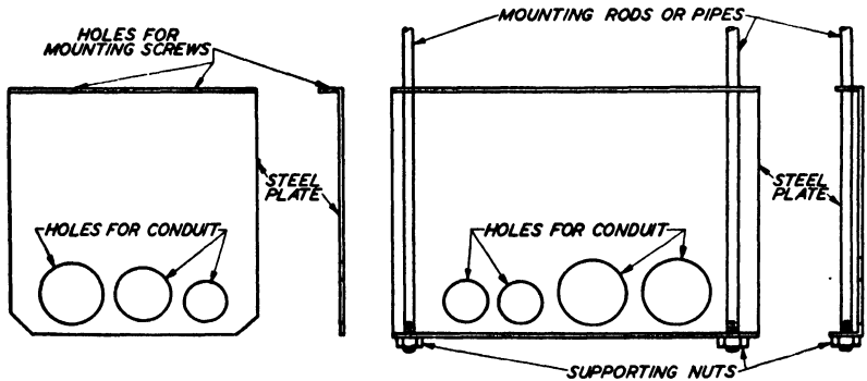
Fig. 41. A Plate Hanger for Supporting Several Conduits
