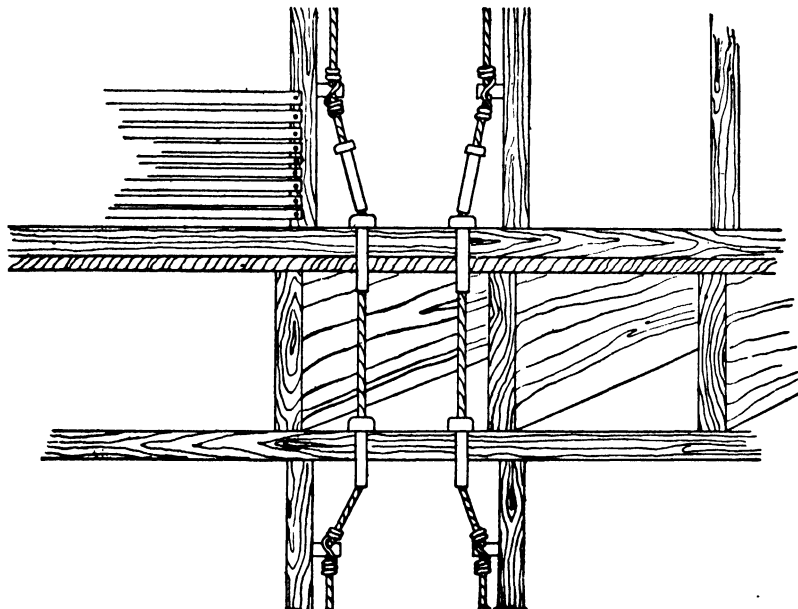
Fig. 47. Conductors Passing through Cross Timbers
