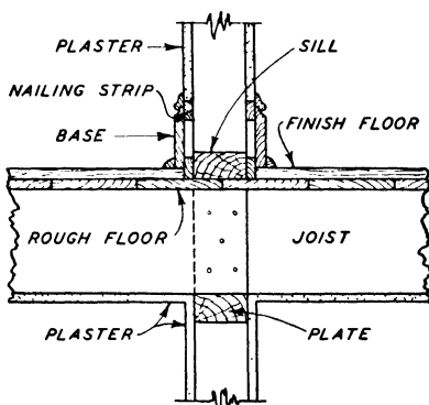
Fig. 47. Construction of Partition Wall
