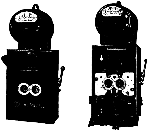
Fig. 10. Two Views of a Meter Service Switch Having Two Branch Circuits Courtesy of Trumbull Electric Manufacturing Company
