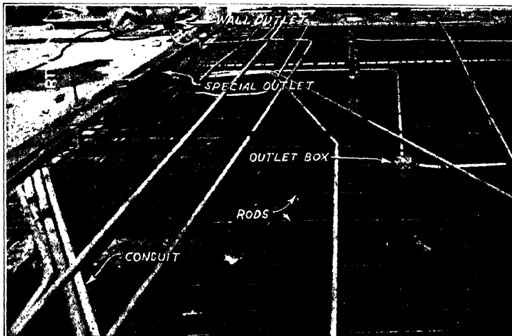
Fig. 52. Installation of Thin-Wall Tubing and Outlet Boxes before a Concrete Floor Slab Is Poured Courtesy of Steel and Tubes, Inc., Cleveland, Ohio
