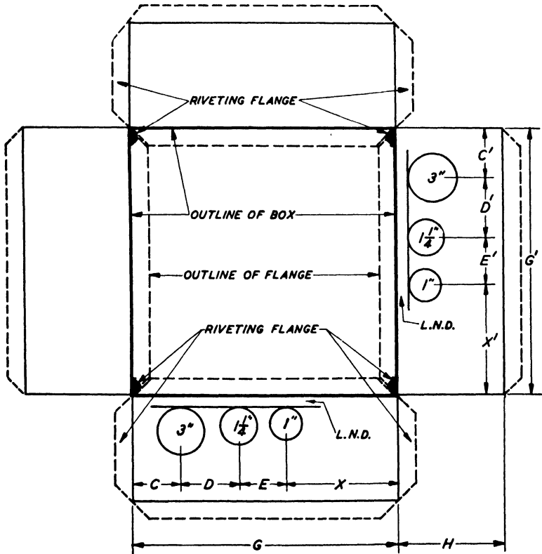
Fig. 35. Sheet Steel Box Layout for a Surface Mounted Pull Box with Screw Cover
