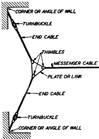
Fig. 46. Detail of Securing Messenger Cable to End of Building
