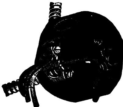
Fig. 8. Octagon Box with Armored Cable Clamps
