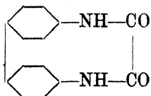
III. Oxalyl-benzidine 3
