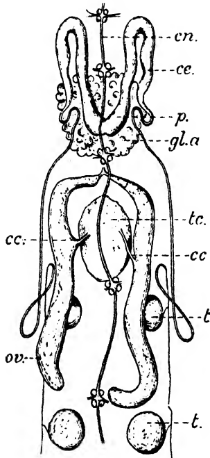
Fig. 8.—Reproductive organs of Piscicola geometra , showing conductive tissue (after Brumpt). t. , testis; cc. , ejaculatory canal; p. , its terminal portion; gl.a. , glands communicating with the terminal portion of the ejaculatory canal and secreting the walls of the spermatophore (these glands in most species lie in the walls of the terminal portion); tc. , mass of conductive tissue underlying the copulatory area; cc. , its paired connections with the ovaries ov. cn. , ventral nerve cord with ganglia.
