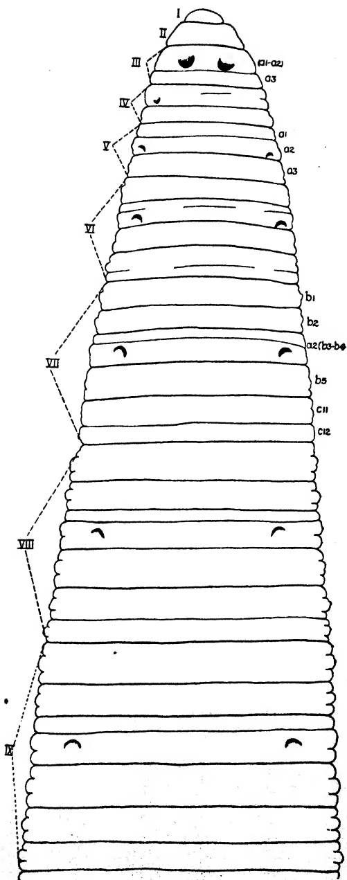
Fig. 43.— Herpobdelloidea indica . Dorsal aspect of somites I-X of a cleared specimen, showing annulation and pigment-cups of eyes. \times 36 . L
