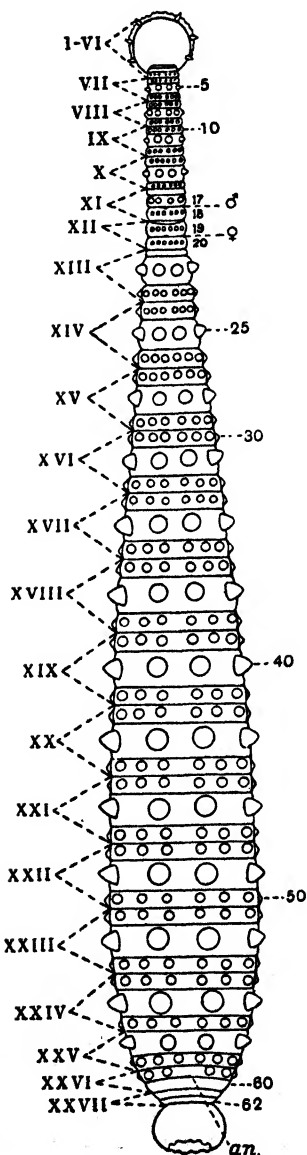
Fig. 11.— Pontobdella loricata , Harding, 1924. (After Harding.) Diagram showing external features of the dorsal surface. Somites numbered in Roman, and rings in ordinary figures. an. Anus.
