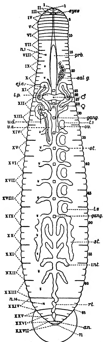
Fig. 29.— Placobdella smydeae , Harding, 1920. (After Harding.) Diagram showing external and internal features. Somites numbered in Roman and rings in ordinary figures. prb. Proboscis. sal.g. Salivary glands. ejc. Ejaculatory canal. t.p. Terminal portion of ejaculatory canal. v.s. Vesicula seminalis or seminal reservoir. v.d. Vas deferens. gang. Ventral ganglion. st. Stomach. rt. Rectum. an. Anus. n. 1, n. 14. First and fourteenth pair of nephridiopores (on ventral surface).
