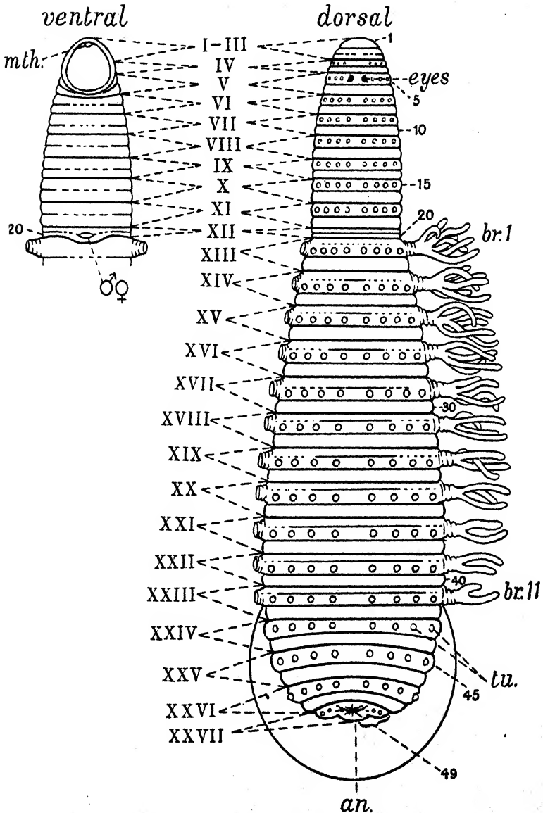
Fig. 10.— Osobranchus shipleyi , Harding, 1909. Diagram showing dorsal and part of the ventral surface. Somites numbered in Roman, and rings in ordinary figures. mth. Mouth. an. Anus. br. 1 , br. 11 . First and eleventh pairs of branchiae. (The branchiae are shown fully on one side only, for the sake of clearness.) tu. Tubercles.
