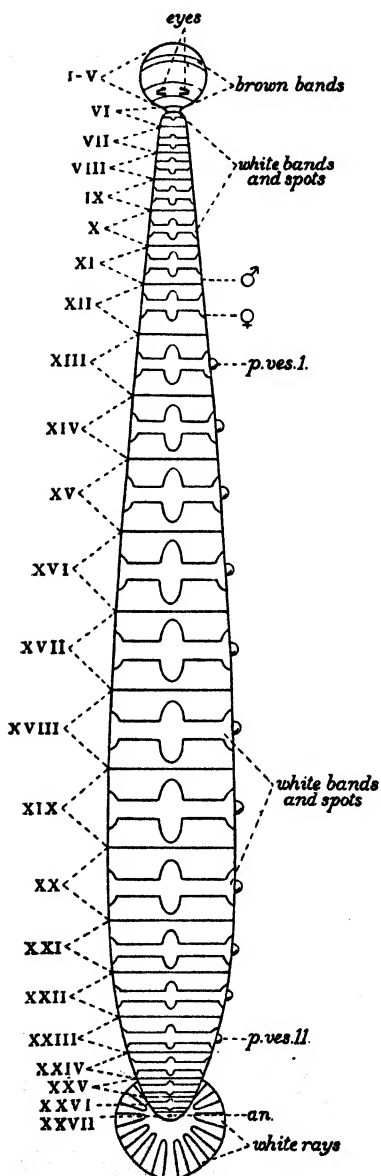
Fig. 16.— Piscicola olivacea , Harding, 1920. Diagram showing dorsal pattern and other external features. Somites numbered in Roman figures. p. ves. I. , p. ves. II. Pulsating vesicles (shown on one side only). an. Anus. (After Harding.)
