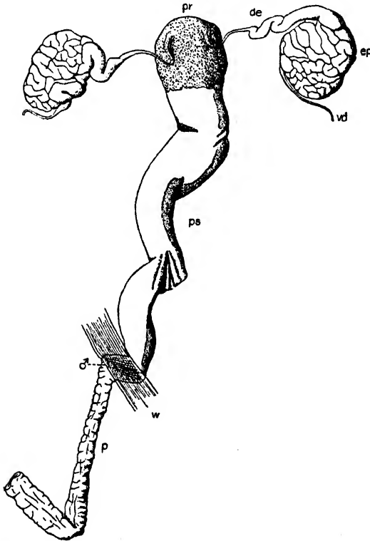
Fig. 57.— Hirudinaria viridis . Terminal male organs removed, and straightened out, as seen from in front, with penis protruded. \times 3\frac{1}{2} . p. , penis. Other lettering as before.
