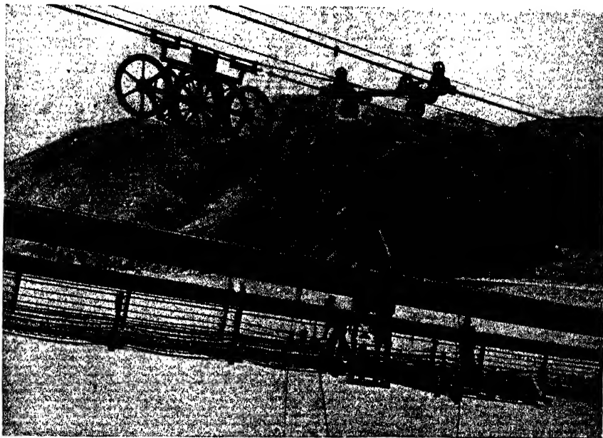
FIG. 39.—Spinning carriage, Golden Gate Bridge. (Courtesy of the Bethlehem Steel Co.)
