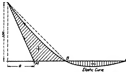
FIG. 15.—Influence diagram for bending moments at M . (Bridge continuous over three supports).
