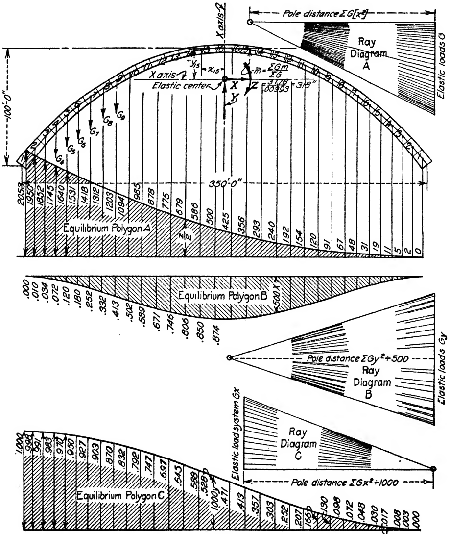
Influence Lines for Moment and Thrust
