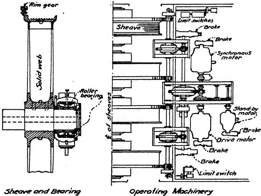
Fig. 16.—Driving machinery, Buzzard's Bay Bridge. (Courtesy of Engineering-News-Record.)
