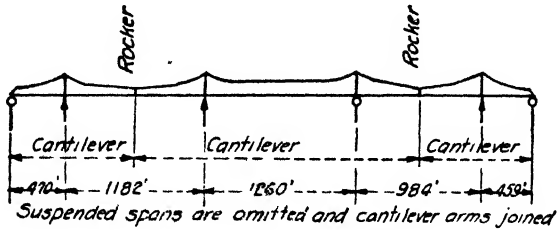
FIG. 10.—Queensboro Bridge.
