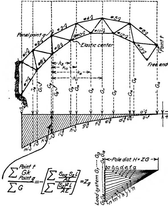
"Reversed" Cantilever
