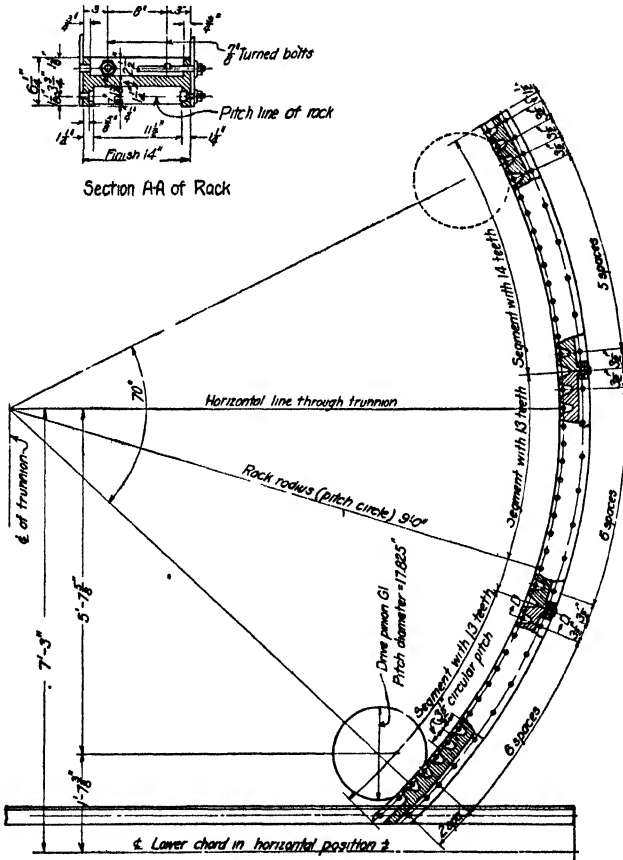
FIG. 101.—Details of operating rack.
