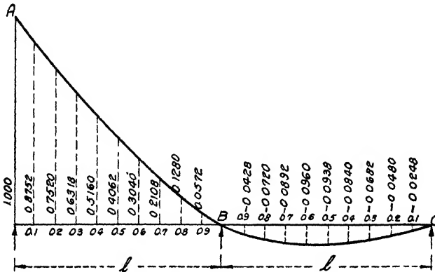
FIG. 14.—Elastic curve for end reaction. (Continuous girder of two equal spans—uniform l ).
