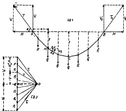
FIG. 1.—The cable as a funicular polygon.
