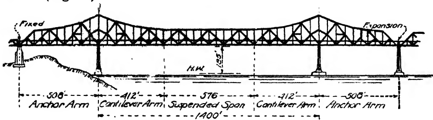
Fig. 37.—Cantilever span, San Francisco-Oakland Bay Bridge. (Courtesy of the American Bridge Co.)
