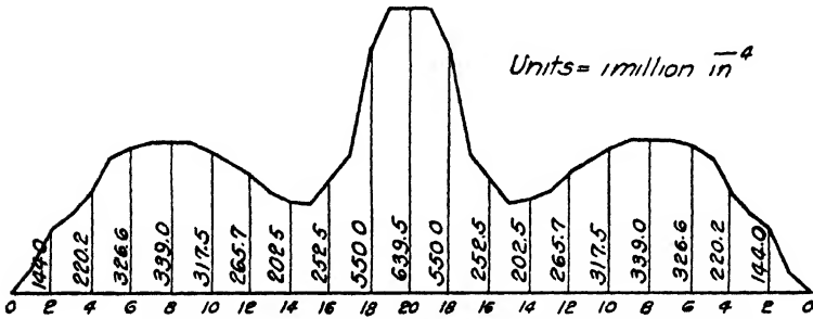
(b) Variation of Moment of Inertia (per truss)
