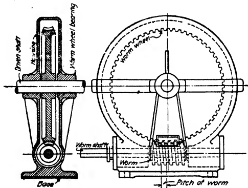
FIG. 110.—Diagram of worm gear speed transformer.
