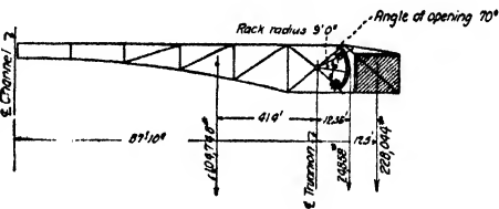
FIG. 99.—General dimensions and weights.
