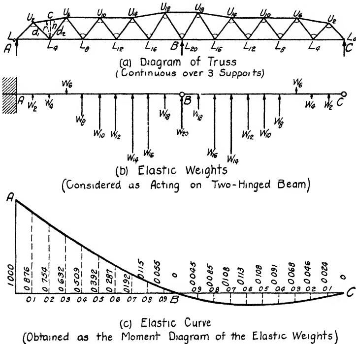
FIG. 20.—Construction of elastic curve for Sciotoville Bridge.
