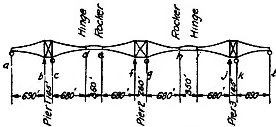
FIG. 9.—Forth Bridge, Scotland.
