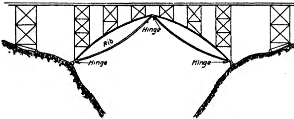
FIG. 9.—Lenticular rib arch (three-hinged).
