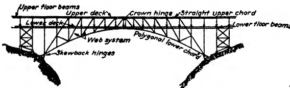
FIG. 11.—Double deck spandrel braced arch.
