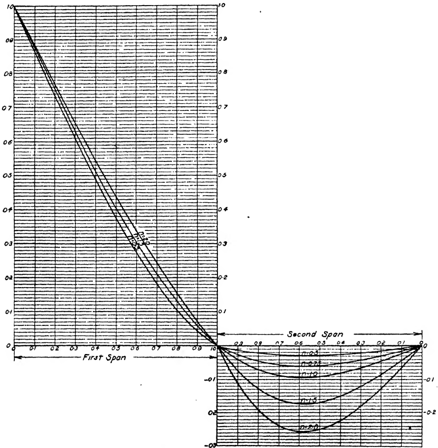
PLATE I.—Two-span continuous beam (Constant I ). Elastic curve for end-reaction ( n = ratio of second span to first span).
