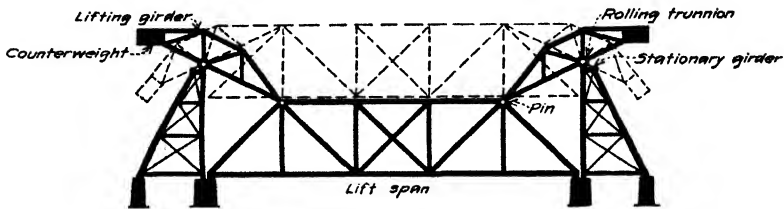
FIG. 25.—Rall direct lift span (Type A).
