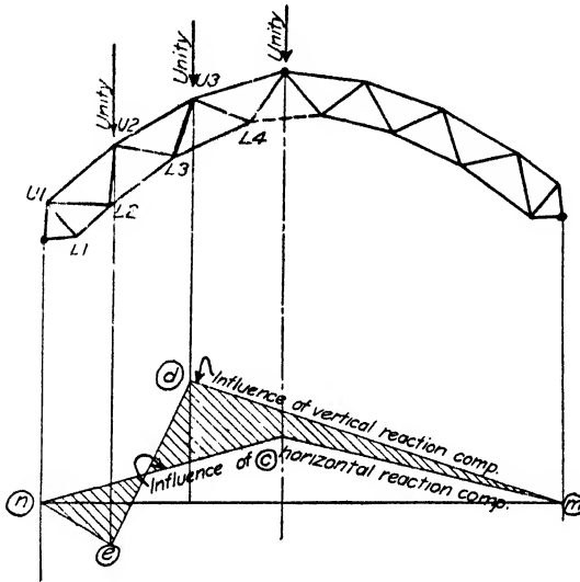
FIG. 11.—Influence line for stress in L3-U3 .
