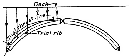
FIG. 22.—Method of selecting arch curve to coincide with the dead load thrust line.
