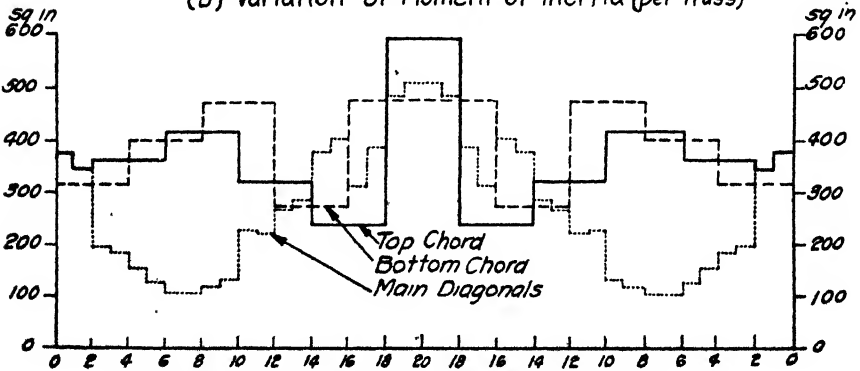
(c) Variation of Sections of Truss Members
