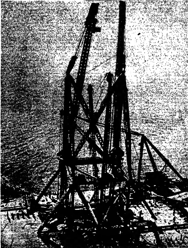
FIG. 35.—Erection traveler Golden Gate Bridge. (Courtesy of the Bethlehem Steel Co.)
