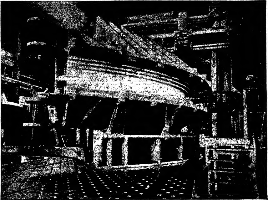
FIG. 41.—Tower saddle, San Francisco Bay Bridge. (Courtesy of the American Bridge Co.)
