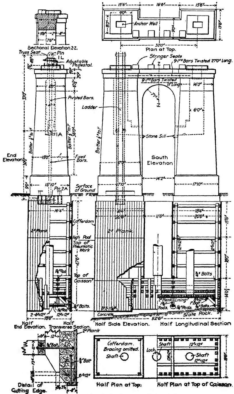
FIG. 22.—Anchor pier, Monongahela Bridge.
