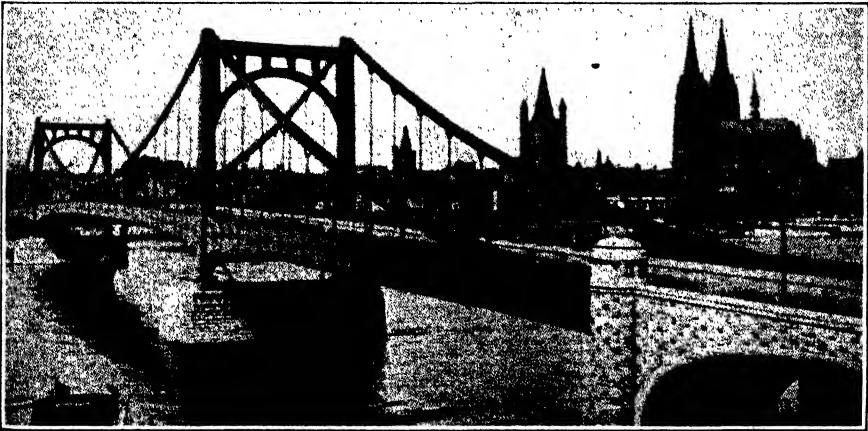
Fig. 26.—Cologne Chain Bridge—1915—Span 605 ft.—Type OS.
