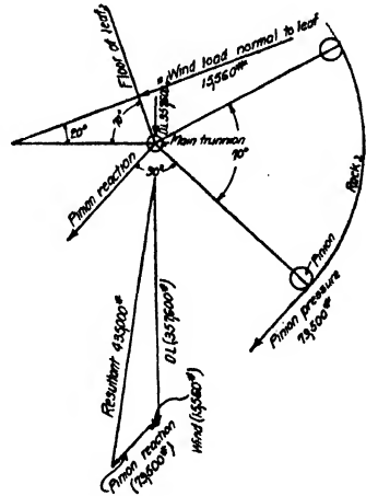
FIG. 112.—Trunnion stresses.
