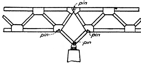
FIG. 27.—Typical arrangement of members at pier, Wichert truss.
