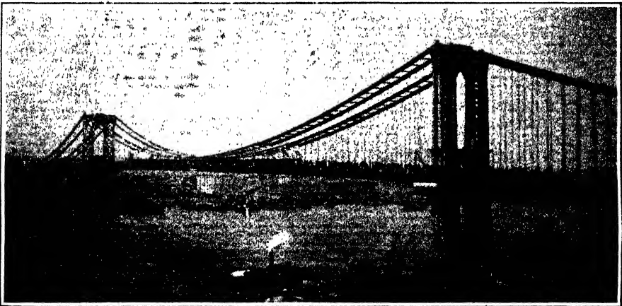
FIG. 33.—Manhattan Bridge—Erection of upper chords of stiffening truss. (1909—Span 1,476 ft.)
