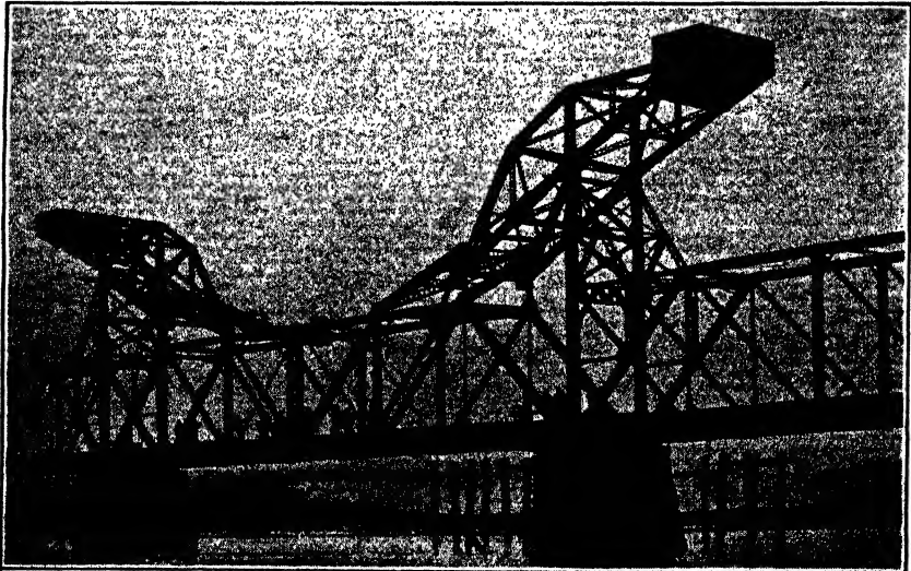
FIG. 27.—Rall type, semi-lift span, C. B. & Q. Railroad near La Salle, Ill. (Span closed.)
