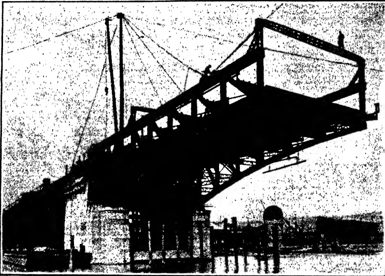
FIG. 21.—Construction view of north leaf of bascule span at 15th Avenue N.W., Seattle Washington—simple trunnion, half through design.
