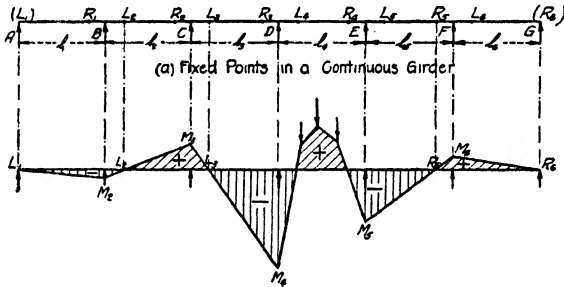
(b) Moment Diagram Constructed with Aid of Fixed Points
