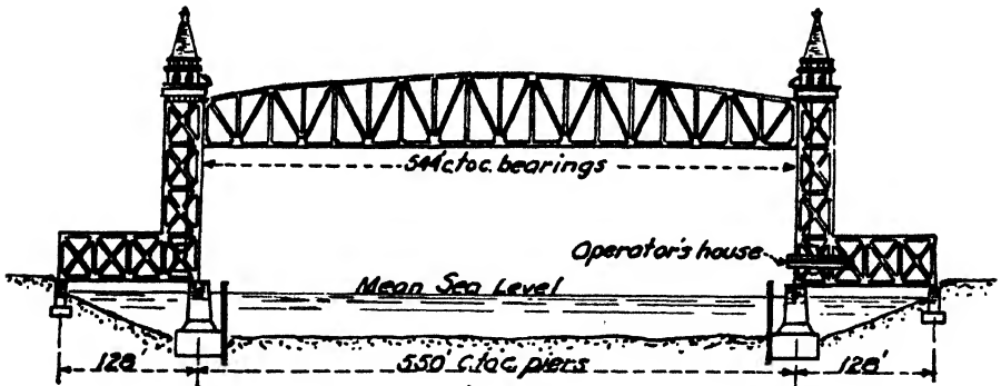
FIG. 15.—Buzzard's Bay Bridge over Cape Cod Canal, Massachusetts. (Courtesy of Engineering-News-Record. )
