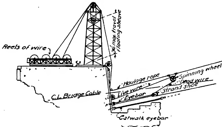
FIG. 38.—Compensation tower and spinning equipment, San Francisco Bay Bridge. (Courtesy of Engineering News-Record.)
