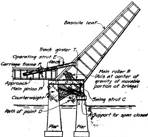
FIG. 13.—Rail type bascule bridge (deck girder span).
