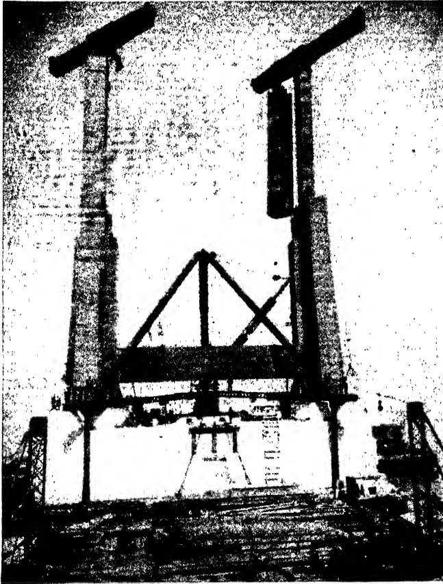
FIG. 36.—Hammerhead cranes, San Francisco Bay Bridge. (Courtesy of the American Bridge Co.)
