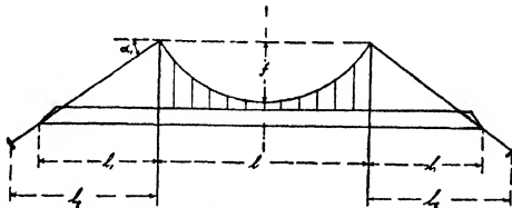
FIG. 13.—Two-hinged stiffening truss with straight backstays (Type 2F).
