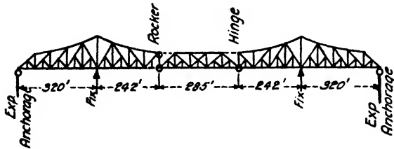
FIG. 12B.—Beaver, Pa., Bridge over Ohio River.
