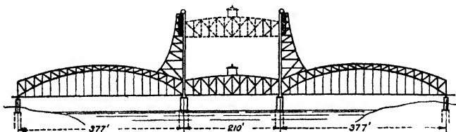
FIG. 14.—Vladicaucase Railroad Company's bridge over the Don River near Rostoff, Russia.
