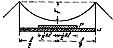
Fig. 5.—Loading for maximum vertical deflection.
