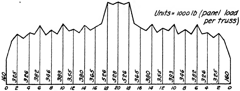
(a) Distribution of Dead Load
