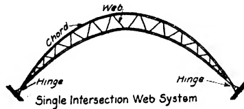
Single Intersection Web System
