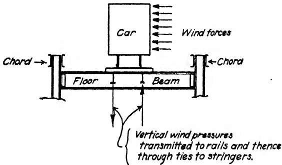
FIG. 16.—Vertical wind forces due to overturning action of wind against train.
