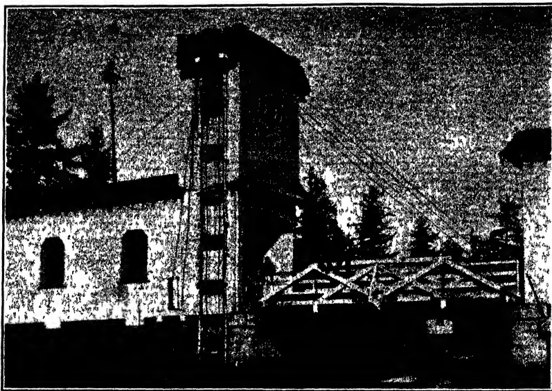
FIG. 7—John Day River Bridge, Clatsop County, Oregon. Cable bascule span with sectional counterweights (Span closed, see also Fig. 3.)
