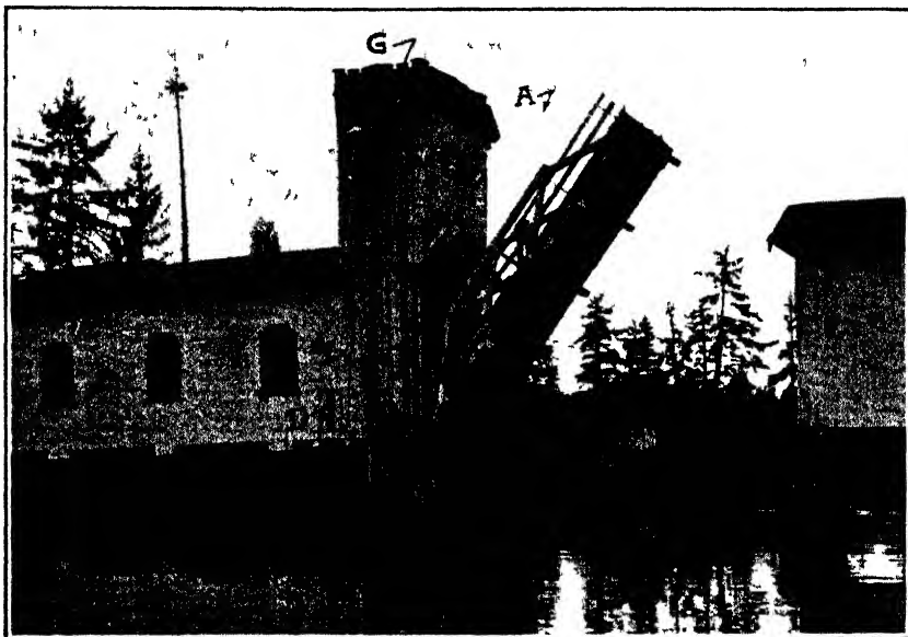
FIG. 3.—John Day River Bridge, Clatsop County, Oregon. Cable bascule span with sectional counterweight. (Span partly open.)
