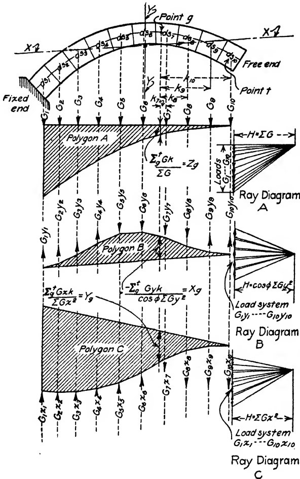
FIG. 31.—Reversed cantilever.
