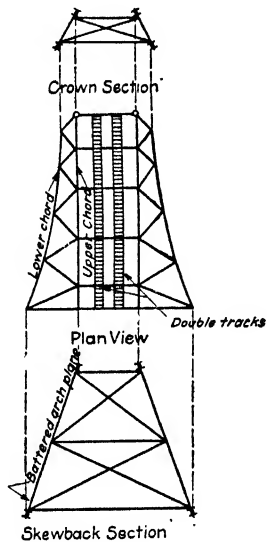
FIG. 12.—Showing method of inclining the planes of the arch frames to provide greater lateral stability at skewbacks.
