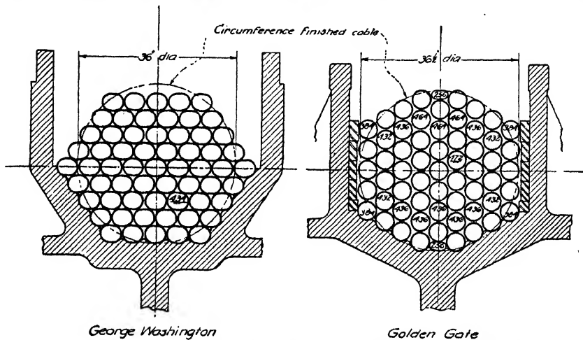
FIG. 42.—Cross sections of cables at tower saddles. (Courtesy of Engineering News-Record .)
