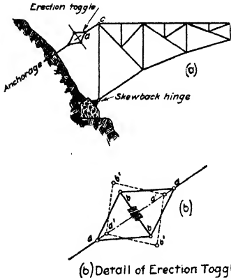
FIG. 18.—Cantilever method for erecting an arch frame.
