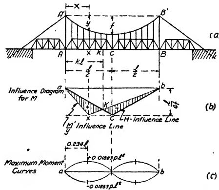
FIG. 8.—Three-hinged stiffening truss (Type 3 F )—Moment diagrams.
