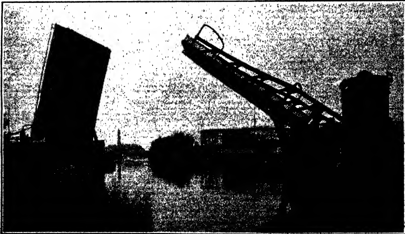
FIG. 22.—Chicago type bascule bridge, Belmont Avenue, Chicago.
