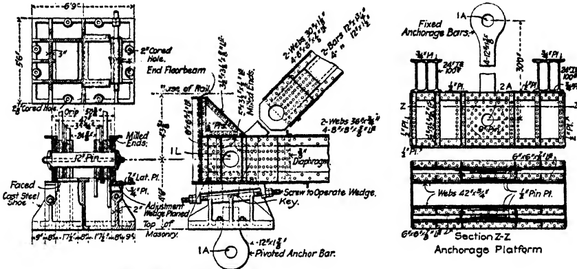
Connections on Anchor Pier
