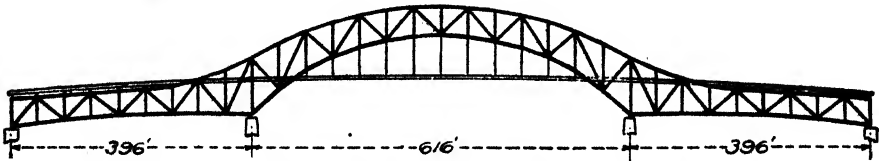
FIG. 30.—Continuous truss bridge over Cape Cod Canal, Sagamore, Mass.
