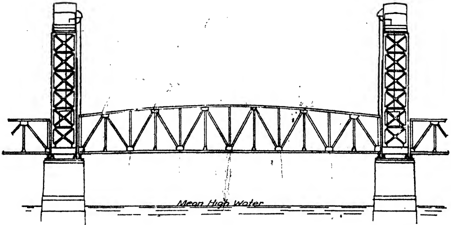
FIG. 17.—Triborough Bridge over Harlem River, New York. (Courtesy of Engineering-News-Record .)
