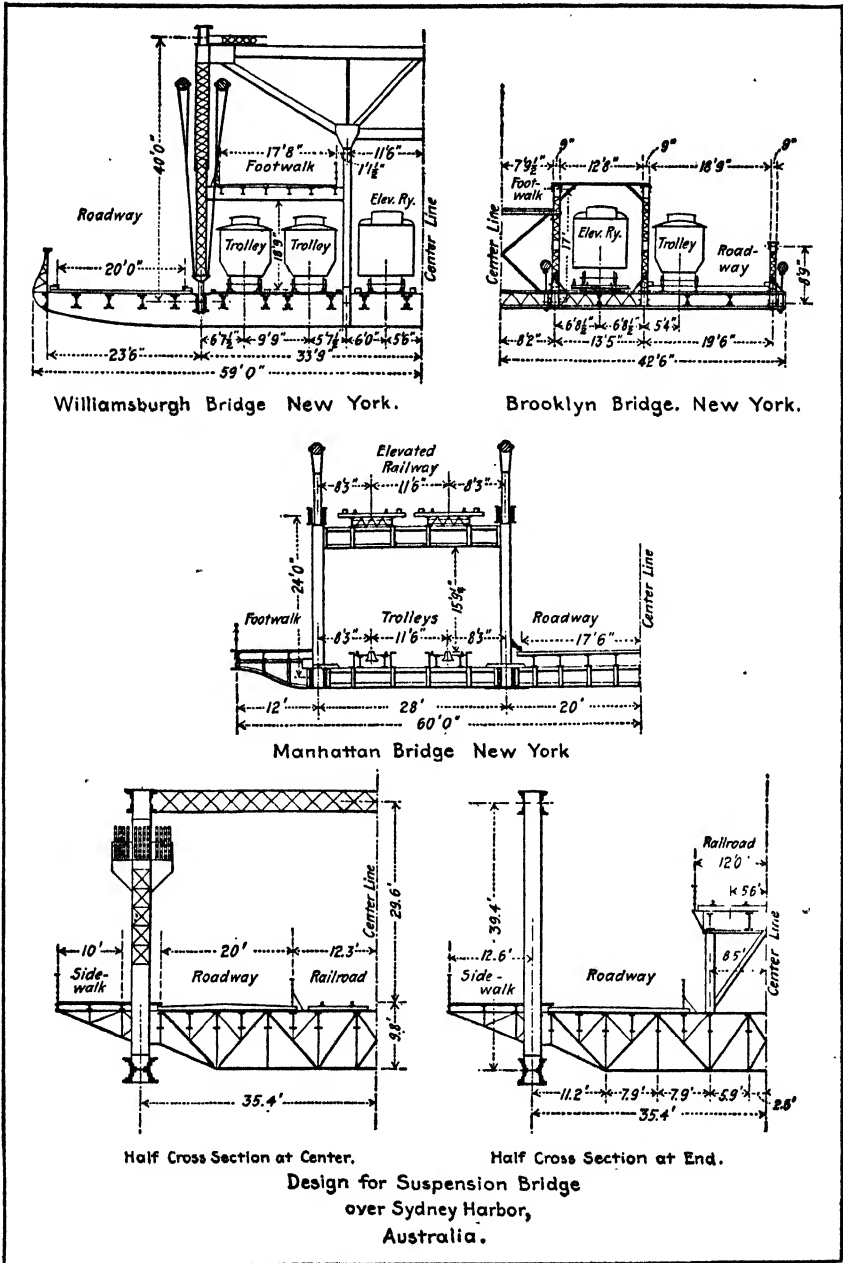
FIG. 24.—Cross-sections of suspension bridges.
