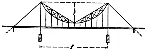
FIG. 17.—Three-hinged braced chain with straight backstays (Type 3BF).
