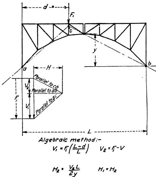
FIG. 4.—Reaction components for single unit load.
