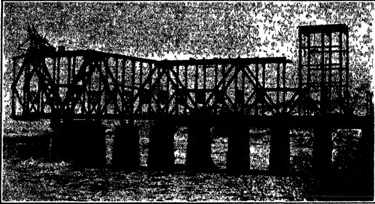
FIG. 5.—Sciotoville Bridge—Erection of Ohio span on falsework
