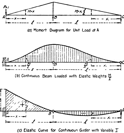
FIG. 17.—Construction of elastic curve for variable I .
