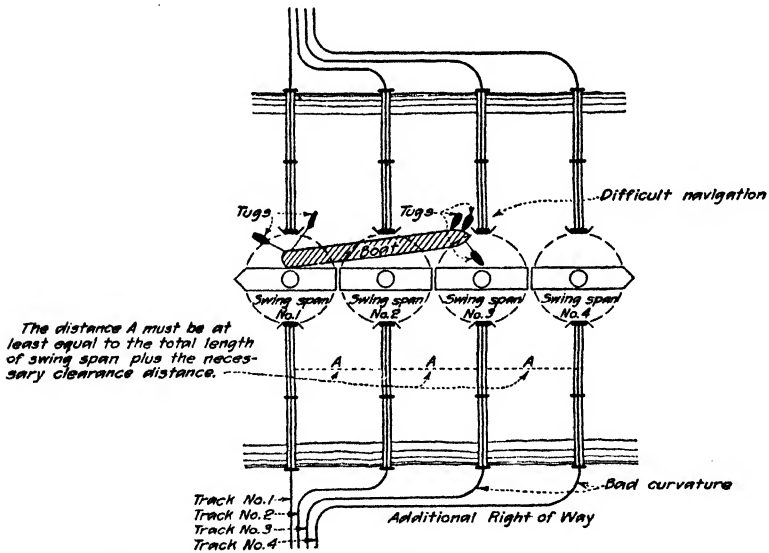
FIG. 1.—Four single track swing spans constructed from time to time to carry additional rail-road trackage.
