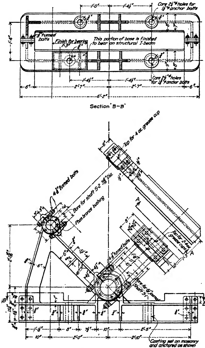
Fig. 115.—Cast machinery frame. For {shafts S1 and S2} see Fig. 104. {gears G2 and G3}
