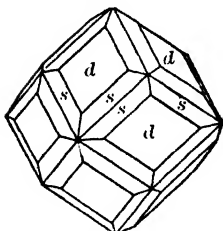
Fig. 48. Dodecahedron and Hexoctahedron.
