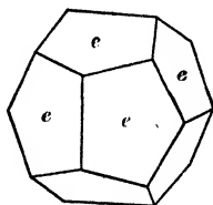
Fig. 227. Pyritohedron
