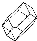
Fig. 20. Distorted Dodecahedron.
