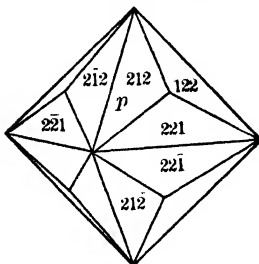
Fig. 44. Trisoctahedron.
