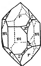
Fig. 141. Right-handed Quartz.
