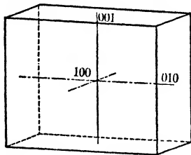
Fig. 150. Macropinacoid, Brachypinacoid, and Basal Pinacoid.
