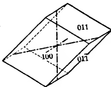
Fig. 184. Brachydomes and Macropinacoid.
