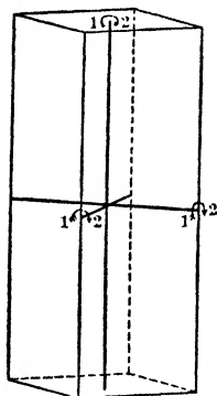
Fig. 144. Axes of Symmetry. Orthorhombic System.
