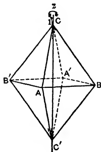
Fig. 4. Symmetry Axis.
