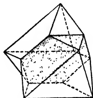
Fig. 22. Twinned Octahedron.
