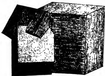
Fig. 226. Striated Cubes.
