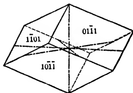
Fig. 121. Negative Rhombohedron.
