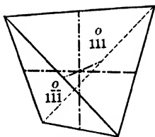
Fig. 65. Positive Tetrahedron.
