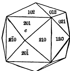
Fig. 38. Tetrahexahedron.
