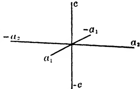
Fig. 76. Tetragonal Axes.
