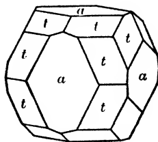
Fig. 61. Diploid and Cube.
