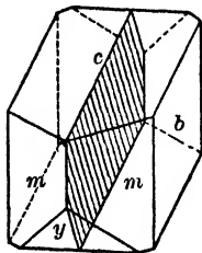
Fig. 3. Symmetry Plane.
