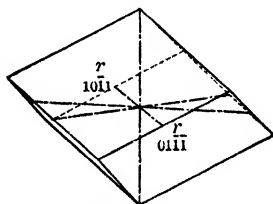
Fig. 120. Positive Rhombohedron.
