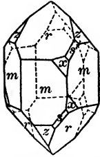
Fig. 248. Right-handed Crystal.
