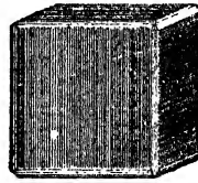
Fig. 55. Striated Cube.
