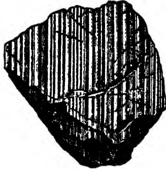
Fig. 298. Albite Twinning.
