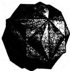
Fig. 231. Twinned Pyritohedrons.
