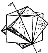
Fig. 21. Twinned Cubes.
