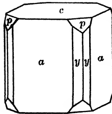
Fig. 94. Apophyllite.
