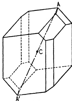
Fig. 5. Symmetry Center.
