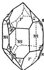
Fig. 142. Left-handed Quartz.
