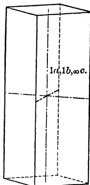
Fig. 8. Orthorhombic Prism.
