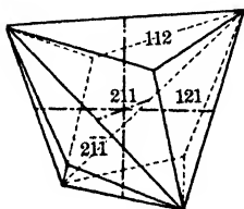
Fig. 68. Tristetrahedron.
