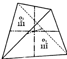
Fig. 66. Negative Tetrahedron.
