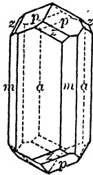
Fig. 100. Scapolite.
