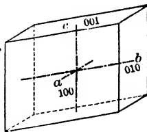
Fig. 185. Macropinacoid, Brachypinacoid, and Basal Pinacoid.
