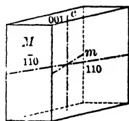
Fig. 182. Prisms and Basal Pinacoid.
