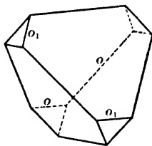
Fig. 67. Positive and Negative Tetrahedrons.
