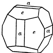
Fig. 228. Cube and Pyritohedron.
