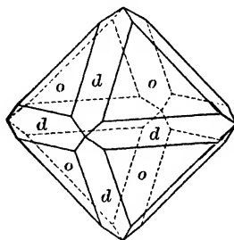
Fig. 35. Octahedron and Dodecahedron.
