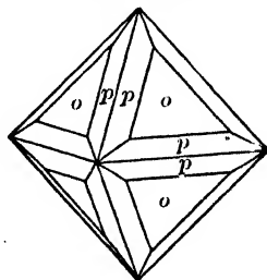
Fig. 45. Octahedron and Trisoctahedron.
