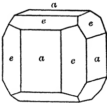
Fig. 56. Cube and Pyritohedron.
