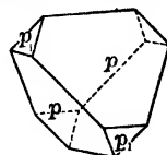
Fig. 99. Positive and Negative Sphenoids.
