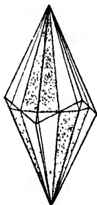
Fig. 131. Showing Relation between Dihexagonal Pyramid and Scalenohedron.
