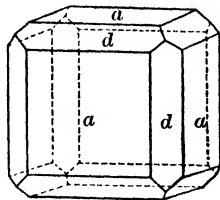
Fig. 34. Cube and Dodecahedron.
