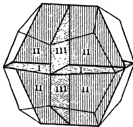
Fig. 50. Symmetry of Pyritohedral Class, Isometric System.
