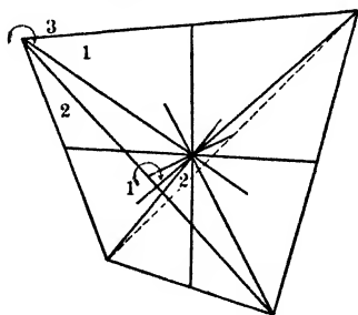
Fig. 62. Symmetry of Tetrahedral Class, Isometric System.
