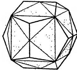
Fig. 53. Showing Relation between Pyritohedron and Tetrahexahedron.
