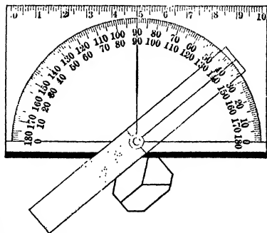
Fig. 2. Contact Goniometer.
