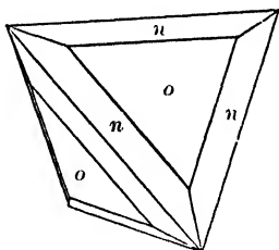
Fig. 75. Tetrahedron and Tristetrahedron.
