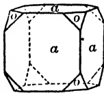
Fig. 218. Cube and Octahedron.
