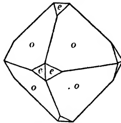
Fig. 57. Octahedron and Pyritohedron.
