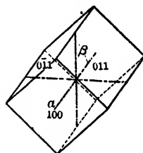
Fig. 171. Clinodome and Orthopinacoid.
