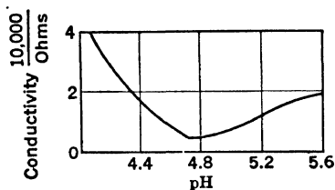
FIG. 12. The Electrical Conductivity of Gelatin Solutions.*
