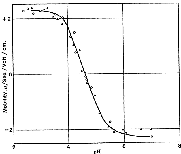
FIG. 2. Cataphoresis of Protected MnO_2 and Fe_2O_3 Sols.* O— Fe_2O_3 Sol, \Delta — MnO_2 Sol
