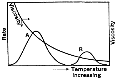
FIG. 9. Rates of Crystallization and Nucleus Formation.
