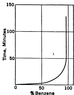
FIG. 3. Emulsification of Benzene in 1% Sodium Oleate Solution.†
