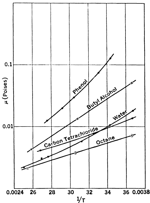
FIG. 12. Temperature-Viscosity Curves for Various Liquids.
