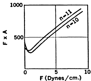
FIG. 5. FA - F Curve for Dibasic Esters.*
