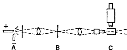
FIG. 8. The Ultramicroscope.
