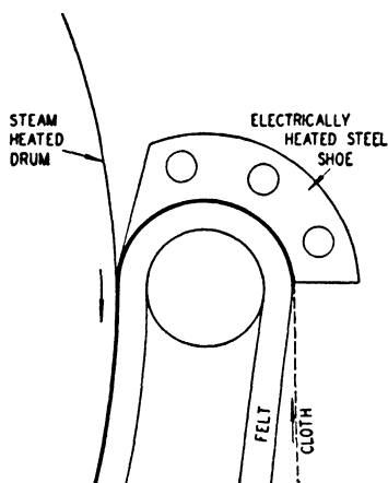
FIG. 5. Technique of Sanforizing.†
