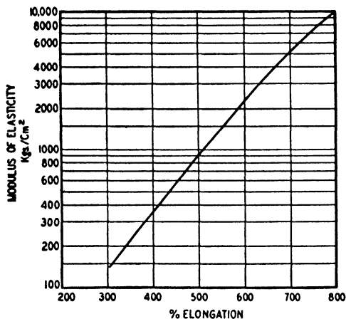
FIG. 21. Effect of Distortion on Young's Modulus for Loaded Rubber.
