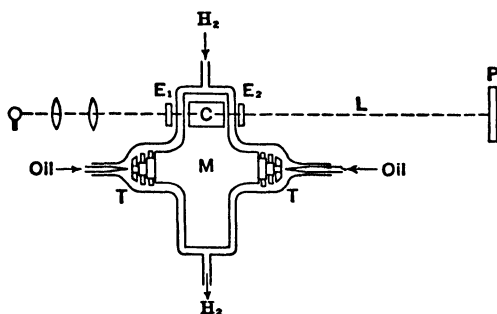
FIG. 2. The Ultracentrifuge.
