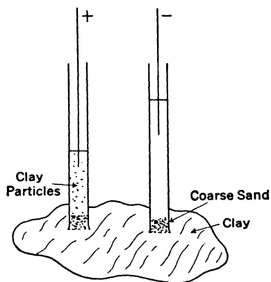
FIG. 1. Reuss' Experiment.
