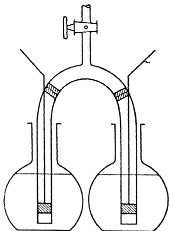
FIG. 4. Transference Apparatus.*
