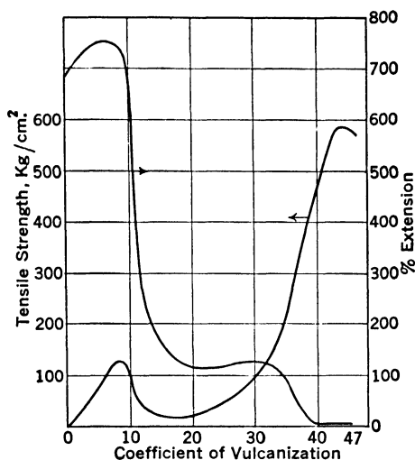
FIG. 10. Variation in Properties with Coefficient of Vulcanization.*
