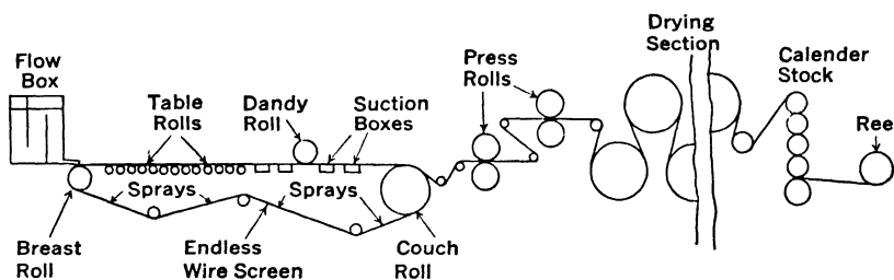
FIG. 12. Paper-making Machine.
