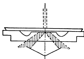
FIG. 10. Cell for Use with Cardioid Condenser.
