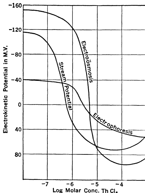
FIG. 7. Effect of ThCl 4 on \zeta -Potentials as Determined by Various Methods of Measurement.*
