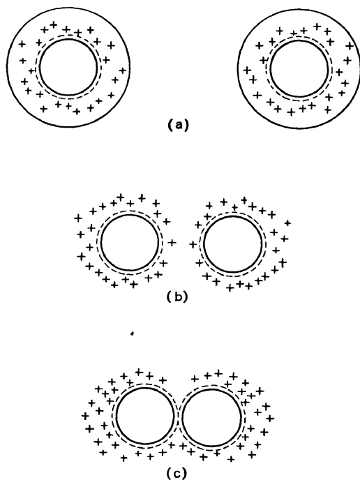
FIG. 5. Gold Particles.
