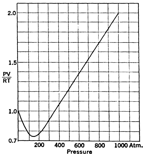
FIG. 5. Compressibility Factors for Methane at 0^{\circ} C.*
