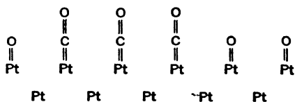
FIG. 10. Oxygen and Carbon Monoxide at a Platinum Surface.
