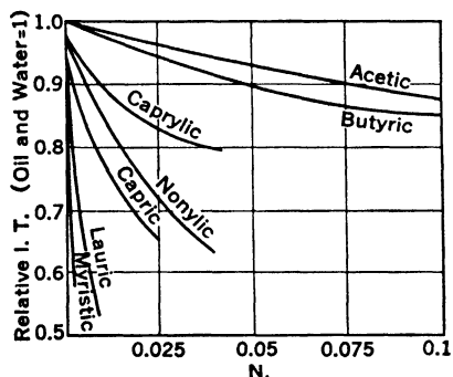
FIG. 6. Relative Interfacial Tensions of Oil and Aqueous Soap Solutions.*
