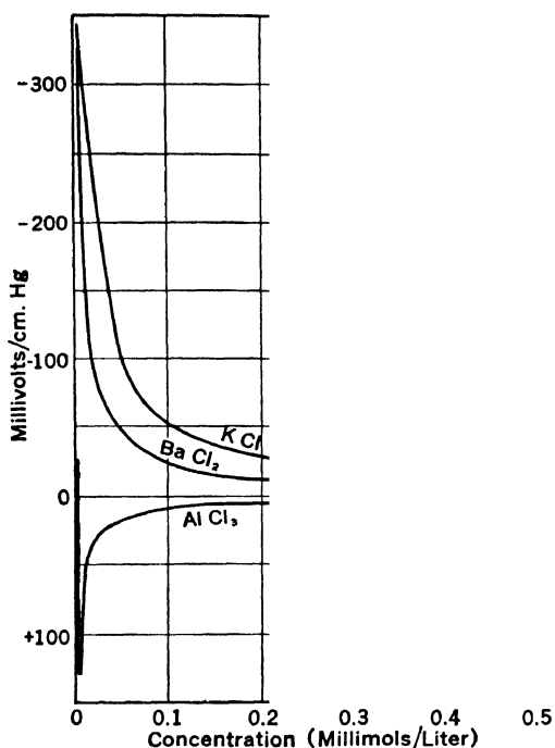
FIG. 6. Streaming Potentials through a Glass Capillary.*
