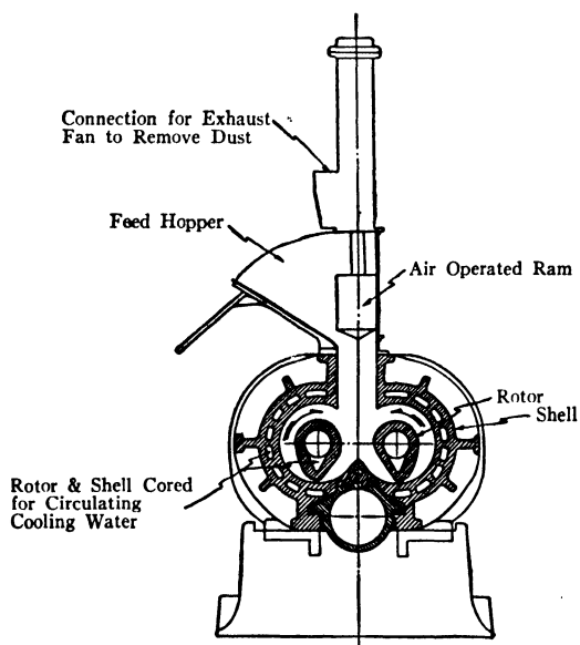
FIG. 6. Banbury Mixer.*
