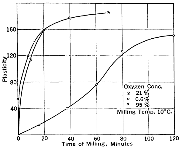
FIG. 9. Effect of Oxygen Concentration on Milling.*
