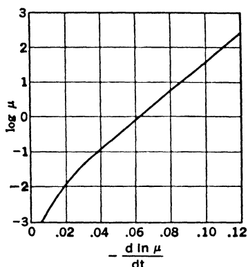
FIG. 13. Change in Viscosity (Poises) with Rising Temperature.
