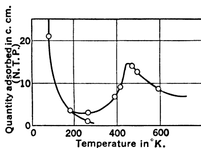
FIG. 5. Adsorption of Hydrogen on 20.0 gms. Zinc Oxide at 400 mm. pressure.*
