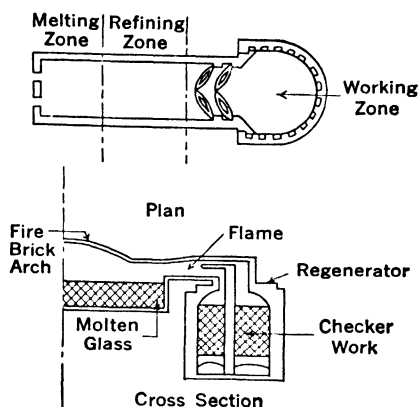
FIG. 8. Glass Furnace.
