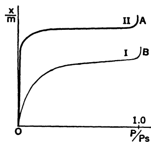
FIG. 6. Adsorption of a Vapor on a Porous Adsorbent.
