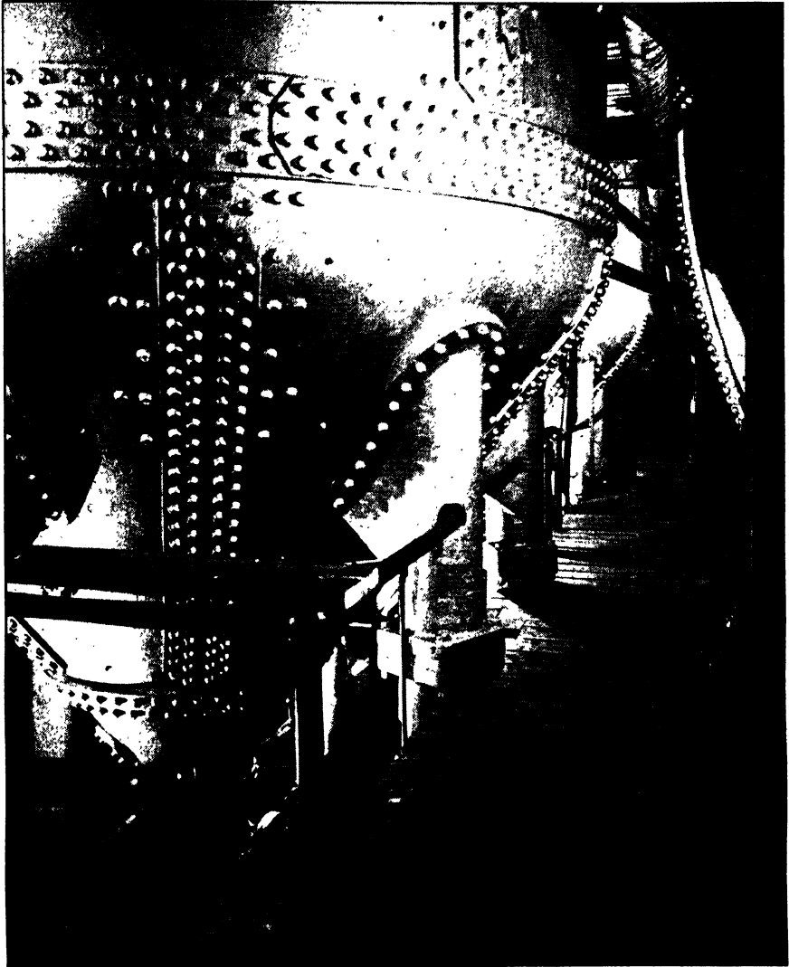
FIG. 1. Bottom Cone of Digester Showing Blow Valve.*
