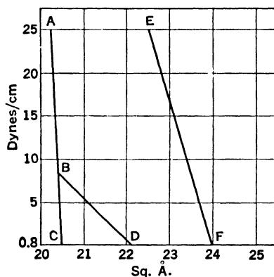
FIG. 8. Force-Area Curves for Condensed Films.†
