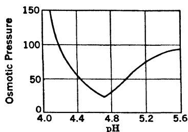
FIG. 11. The Osmotic Pressure of Gelatin Solutions.*
