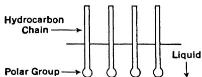
FIG. 1. Orientation in the Interface.
