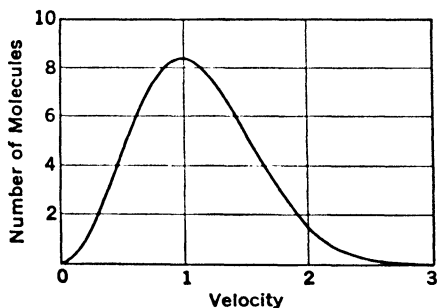
FIG. 1. Molecular Velocity Distribution of Gases.
