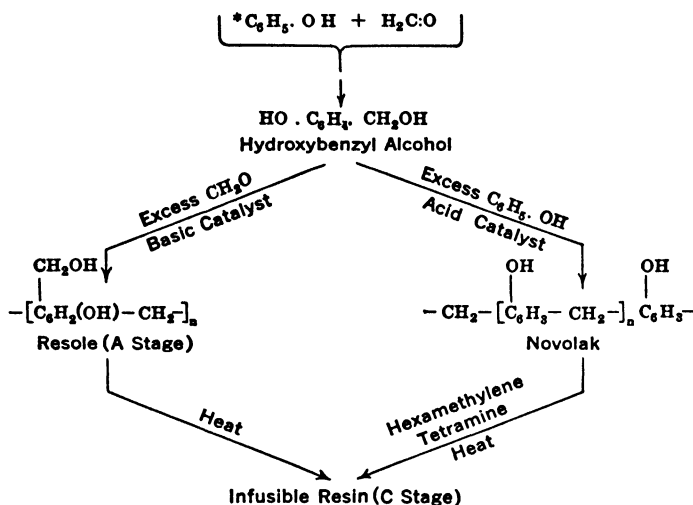
FIG. 3. Phenol-Formaldehyde Condensation.
