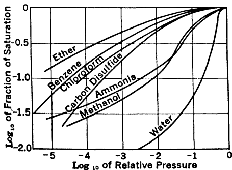
FIG. 8. The Adsorption of Vapors on Charcoal.*
