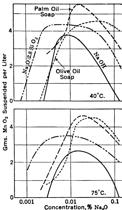
FIG. 9. Suspending Power versus Concentration of Detergent Employed.‡
