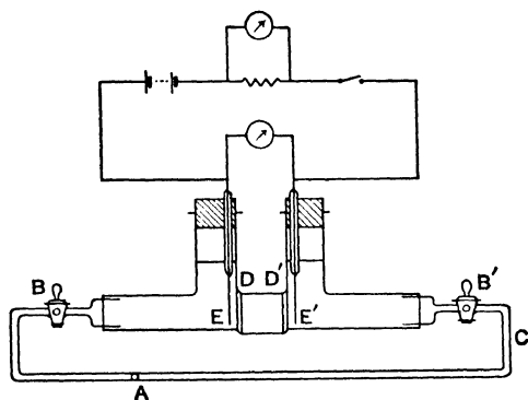
FIG. 5. Electroendosmosis Apparatus.†
