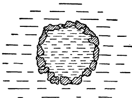
FIG. 8. Solid Emulsifier at the Interface.
