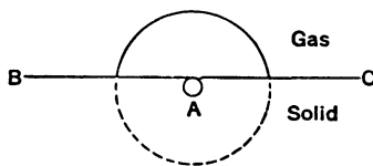
FIG. 1. The Gas-Solid Interface.
