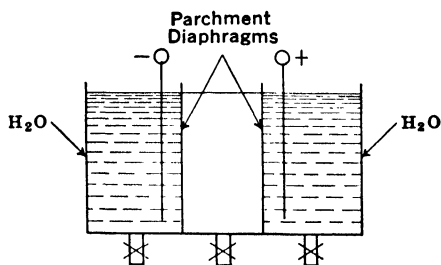
FIG. 13. Electro-dialysis Apparatus.
