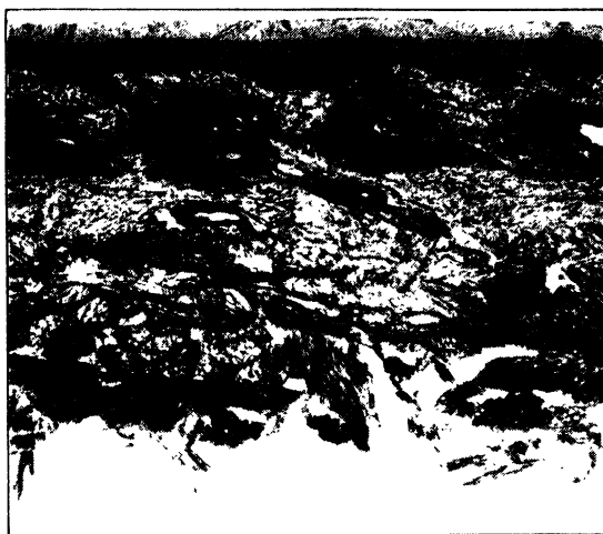
FIG. 5. Patent Leather, Three Finish Coats.* Paraffin section; 20\mu ; mounted in glycerin jelly; (45\times) .
