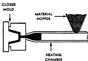
FIG. 2. Injection Molding.*
