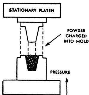
FIG. 1. Compression Molding.*
