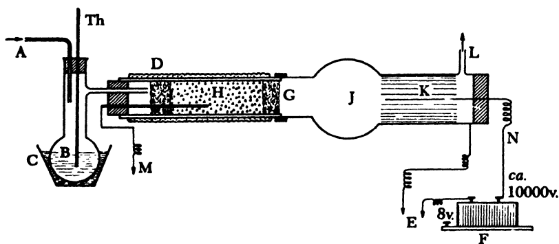
Fig. 28. Apparatus for preparation of phthalic anhydride by catalytic oxidation: A, air inlet tube; B, melted naphthalene; C, graphite bath; D, electrical heating element; E, ground; F, spark induction coil; G, glass wool; H, catalyst; J, bulb receiver; K, aluminum foil, grounded; L, gas exit tube; M, thermocouple; N, rigid wire; Th, thermometer. One side of the spark induction coil is connected to N, the other is grounded.
