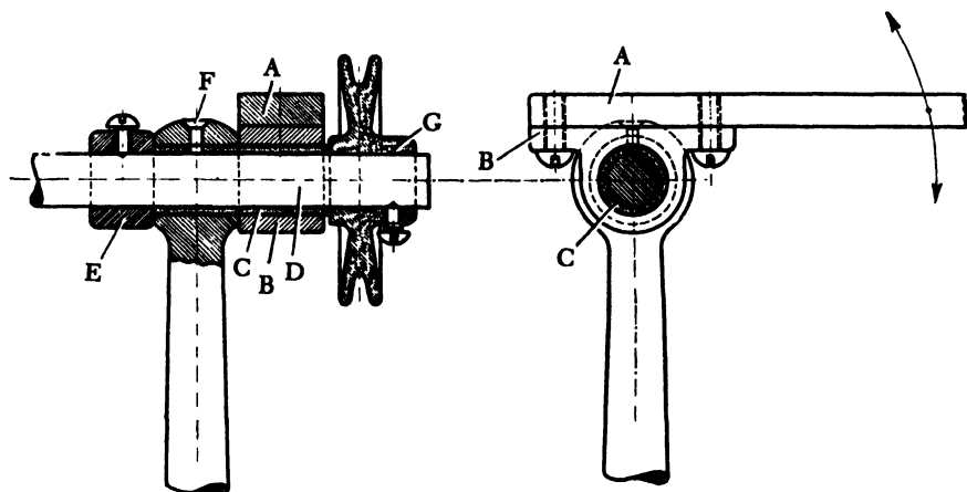
Fig. 51. Detail of the rotating autoclave: (A) support frame; (B) connecting bearing; (C) bronze bushing; (D) axle; (E) positioning ring; (F) oil hole; (G) drive pulley.
