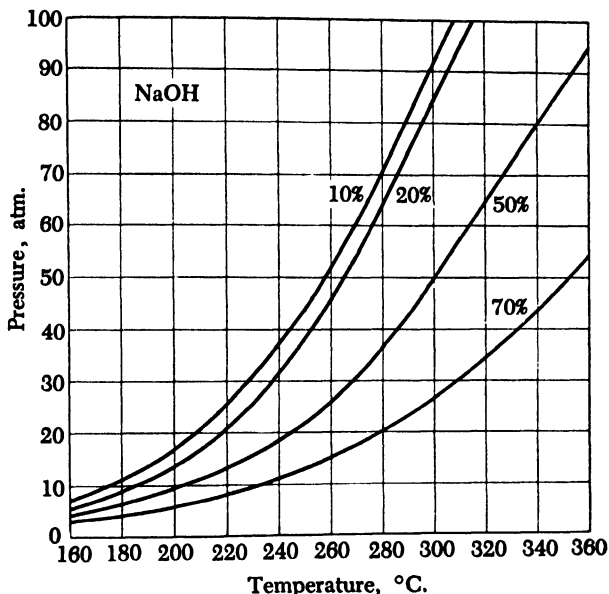
Fig. 15. Temperature-pressure curves for aqueous sodium hydroxide solutions.
