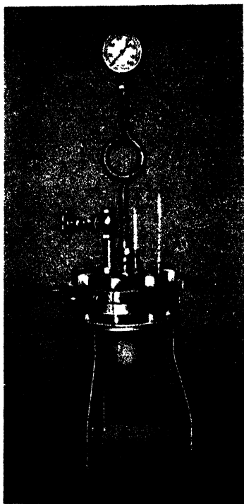
Fig. 48. Vertical cast steel autoclave: working pressure, 60 atm.; capacity, 1 liter; weight, 30 kg.
