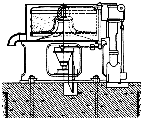
Fig. 33. Centrifuge with bottom discharge.
