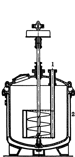
Fig. 8. Nitration kettle with auger-type stirrer, equipped for external and internal cooling: (1) water inlet tube for internal cooling; (2) heating and cooling jacket.
