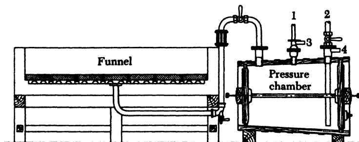
Fig. 26. Stone filter funnel for strongly acid precipitates: (1) vacuum connection; (2) discharge line for removing filtrate; (3) air outlet; (4) connection to wash water, or to the sewer for emptying.
