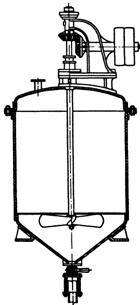
Fig. 9. Separating funnel and extraction apparatus with propeller stirrer and transparent window.
