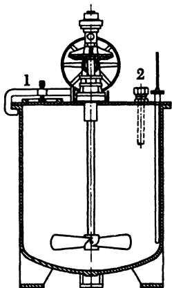
Fig. 18. Reduction kettle with auger-type stirrer: (1) filling port with clamped cover; (2) hole for blow-out tube.
