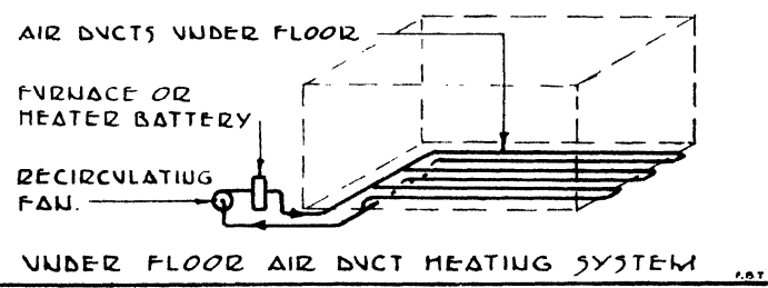
FIG. 21. Air Circulating Systems
