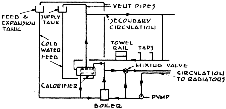
3. COMBINED HEATING AND H.W. SUPPLY SYSTEM. ...
