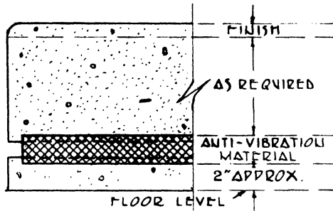
FIG. 99. INSULATED CONCRETE BASE
