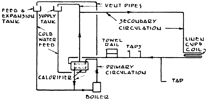
2. INDIRECT SYSTEM WITH SECONDARY CIRCULATION
