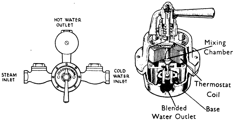
FIG. 66. STEAM AND WATER MIXER
