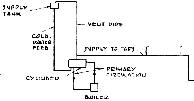
1. DIRECT SYSTEM WITHOUT SECONDARY CIRCULATION
