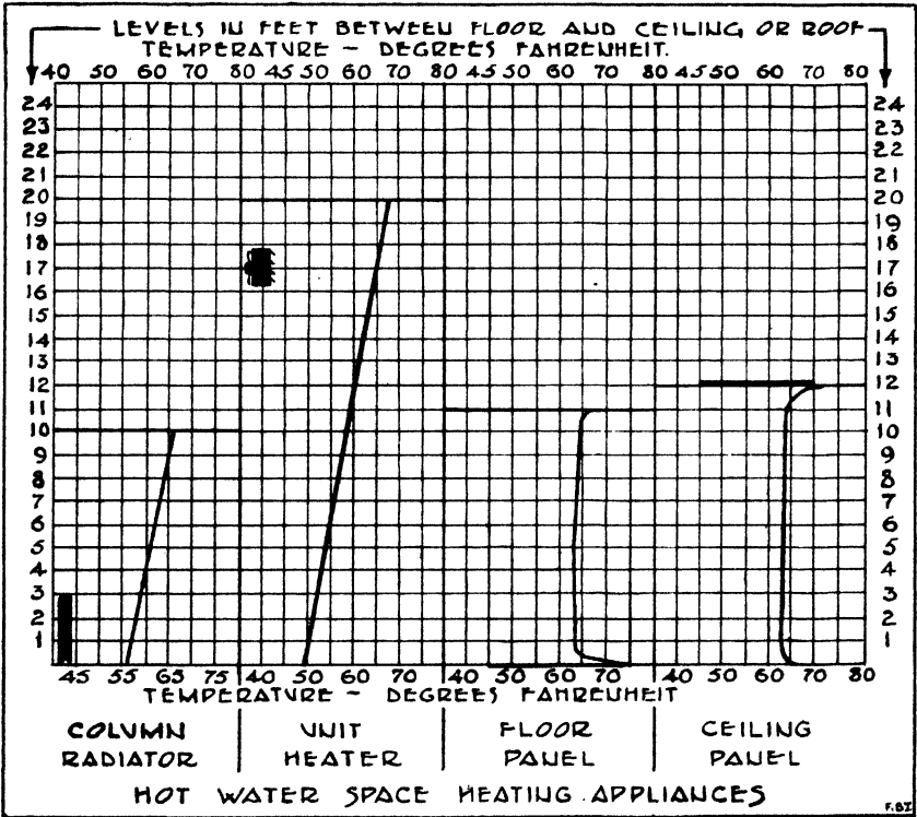
FIG. 5. VERTICAL TEMPERATURE GRADIENTS Variations in gradient produced with different types of space-warming appliances.
