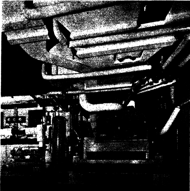
FIG. 97. AIR-CONDITIONING PLANT Installation showing humidifier, refrigerating compressor, and insulated ducting overhead. (Carrier)
