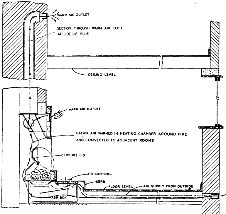
FIG. 68. CLOSEABLE FIREPLACE
