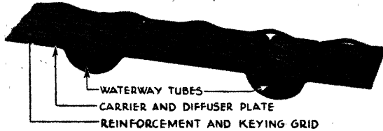
FIG. 15. RADIANT PANEL Steel panel element of the interposed type. (Solray)
