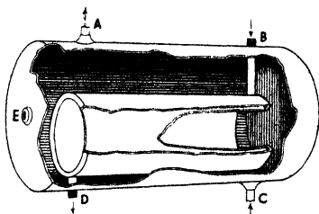
FIG. 64. INDIRECT CYLINDER OR CALORIFIER
