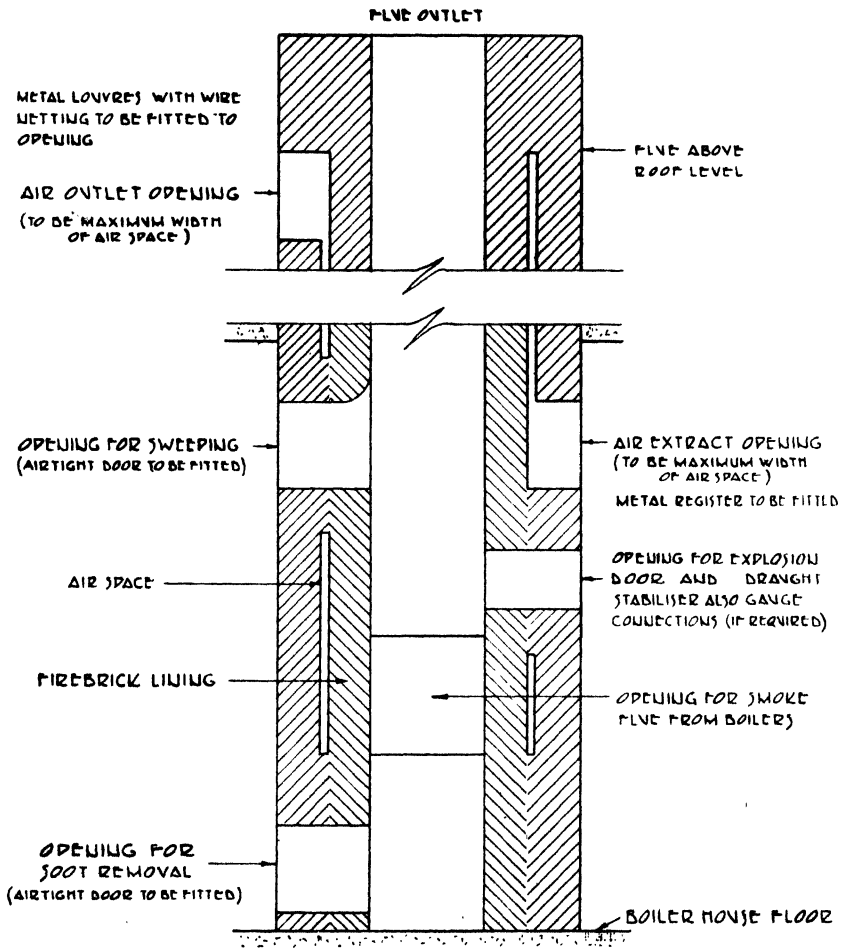
PART SECTIONAL ELEVATION OF CHIMNEY STACK
