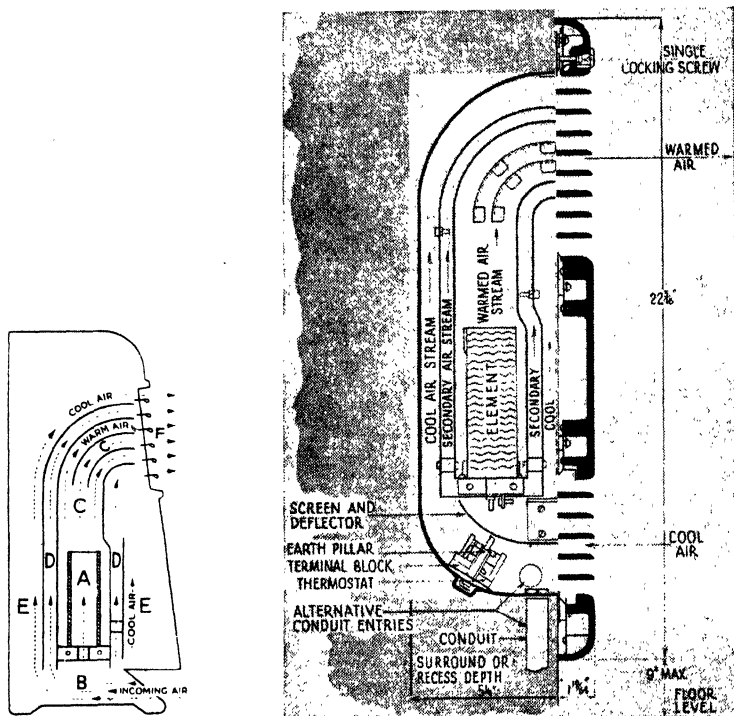
(a) Vertical cross section of floor, standing type heater.
