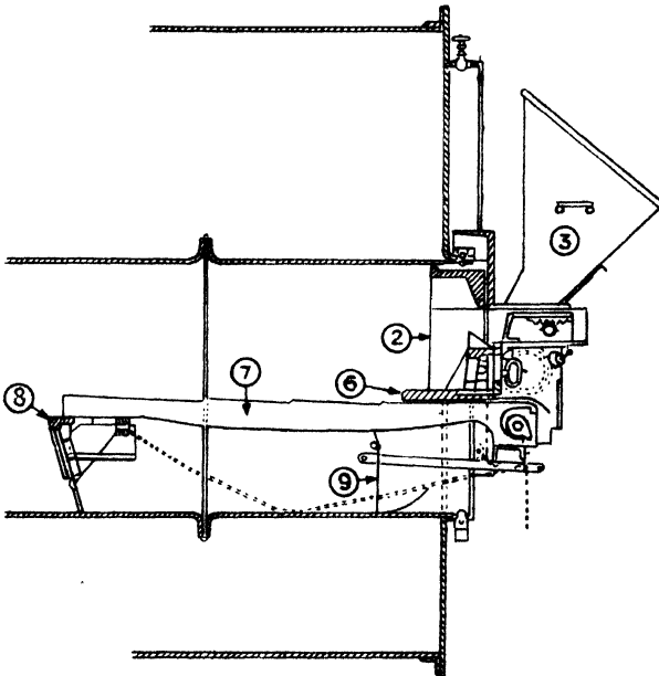
FIG. 42. NATURAL DRAUGHT COKING STOKER APPLIED TO LANCASHIRE BOILER (PART LONGITUDINAL SECTION)
