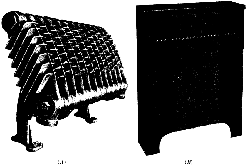
FIG. 10. CONVECTOR RADIATOR
