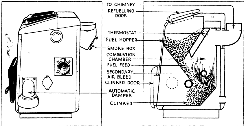
FIG. 35. MAGAZINE BOILER
