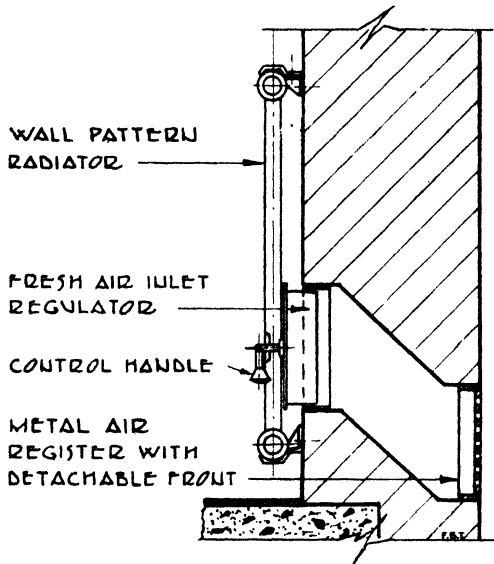
— SECTIONAL ELEVATION —
