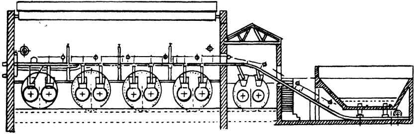
FIG. 102. COAL-HANDLING PLANT
