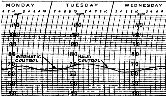
FIG. 51. THERMOGRAPH CHART Space temperatures with and without automatic control.
