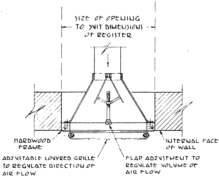
FIG. 95. FRESH AIR INLET GRILLE
