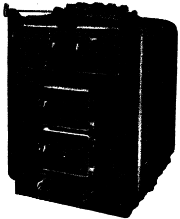
FIG. 34. CAST-IRON SECTIONAL BOILER Shown without insulating jacket. (Crane)
