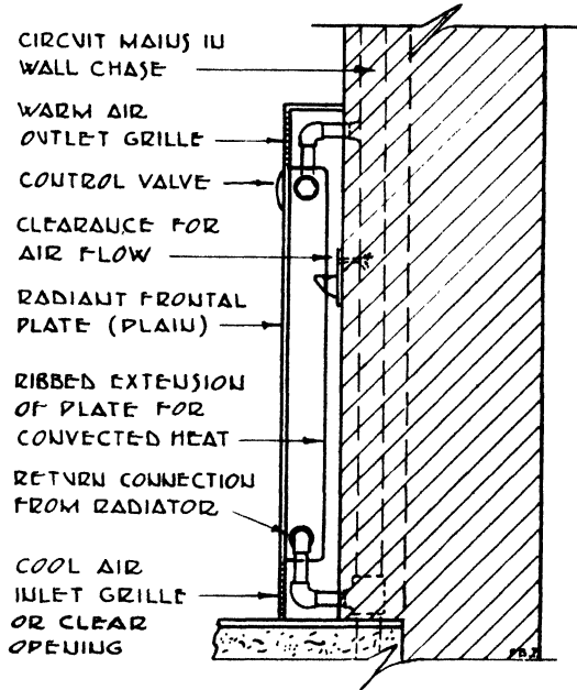
FIG. 83. CONVECTOR RADIANT RADIATOR Radiator fixed with front air outlet grille. Top outlet grille may be provided as an alternative position.
