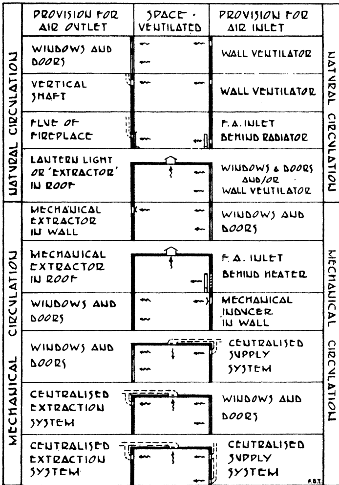
FIG. 6. VENTILATING SYSTEMS Various methods of providing ventilation.
