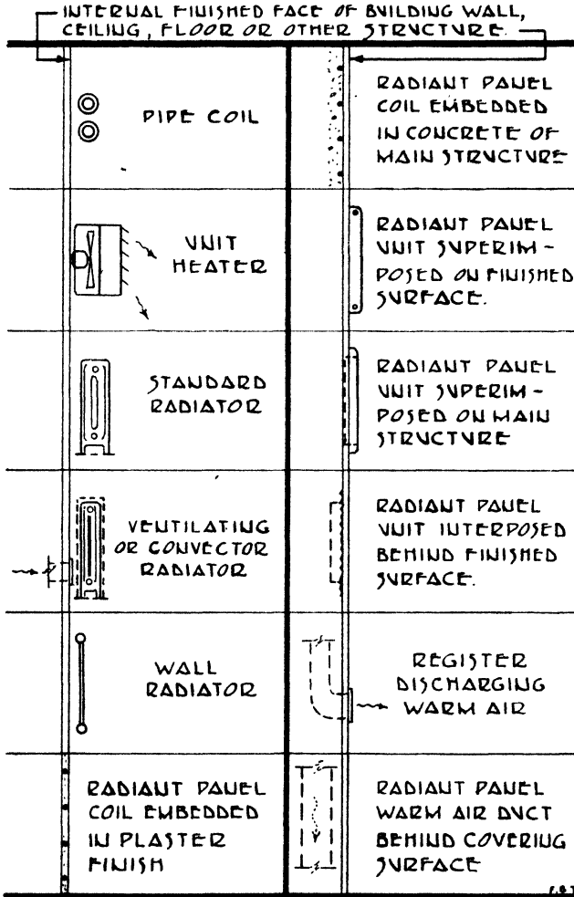
FIG. 2. WARMING METHODS
