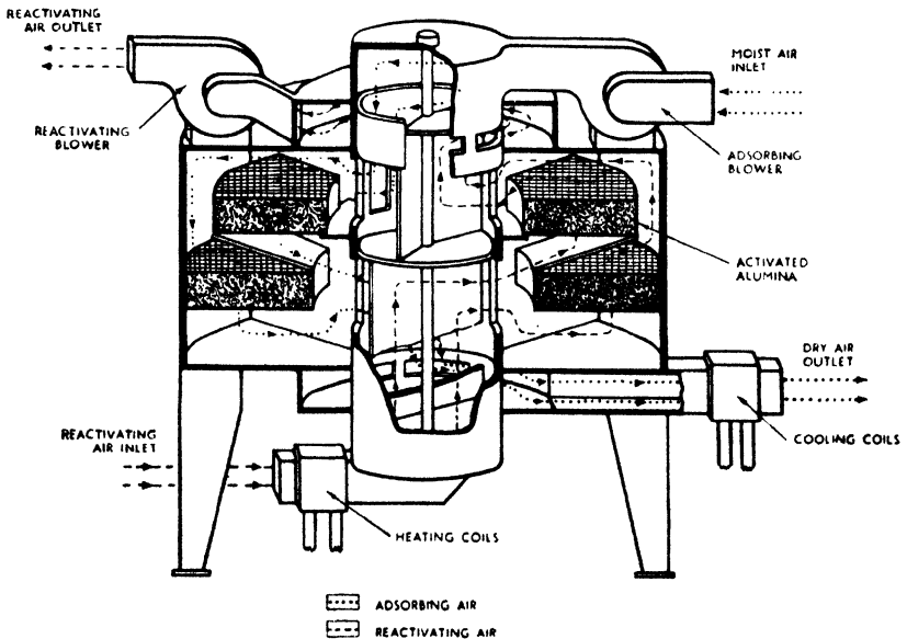
FIG. 27. ADSORPTION TYPE DE-HUMIDIFIER
