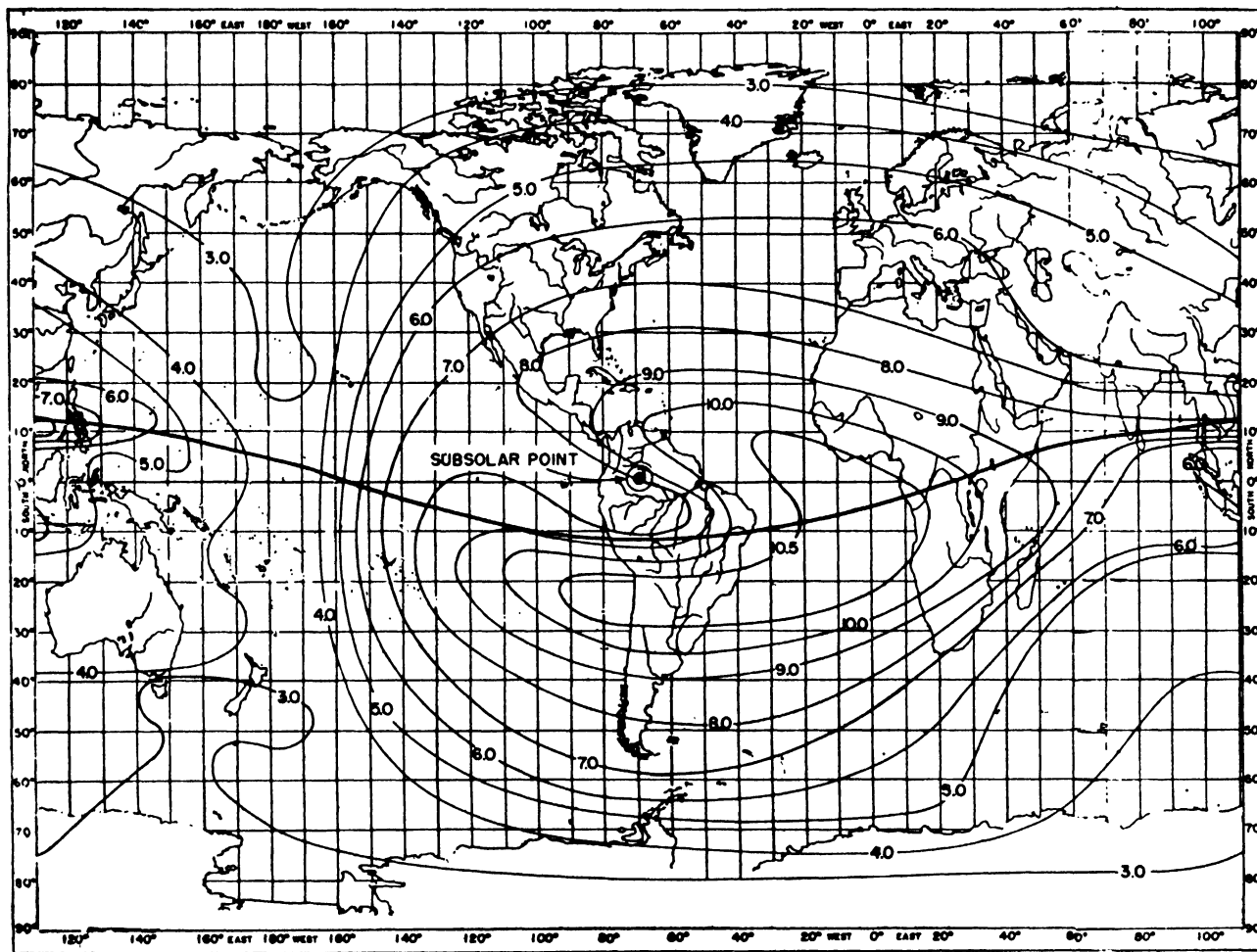
FIGURE 4.15. World-wide distribution of critical frequency of F2 layer ( f^{\circ}F_2 ) in megacycles for equinox, 1945, when it is noon at 69° W.
