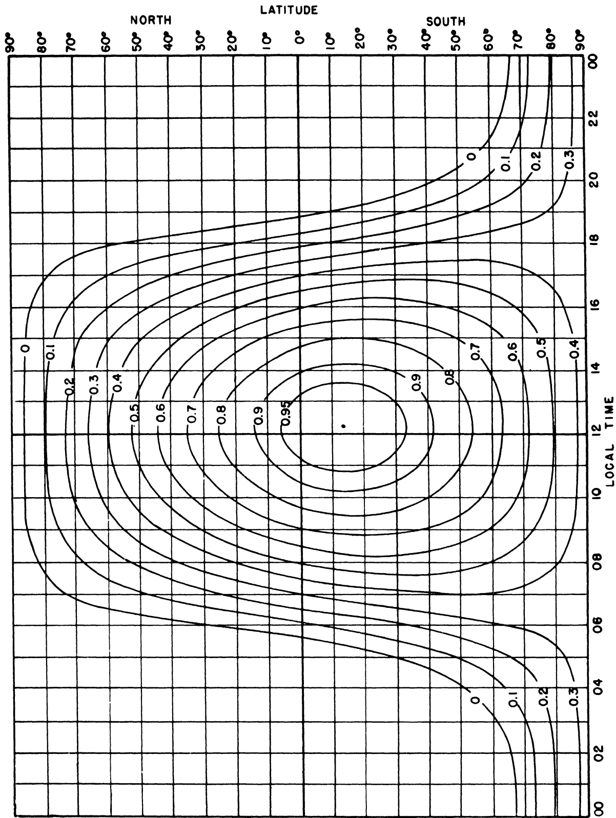
FIGURE 7.35. Absorption factor, K_p , for February.
