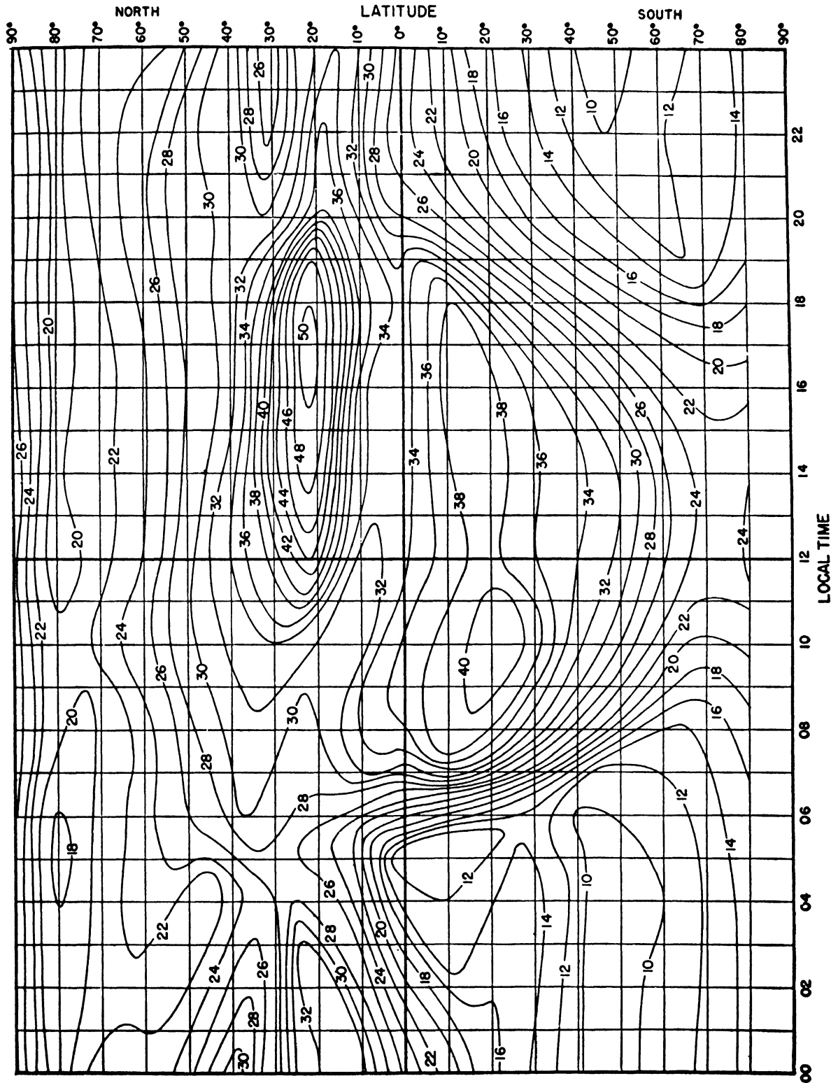
FIGURE 6.26. F_2 4000-muf, in megacycles, E zone, predicted for June 1947
