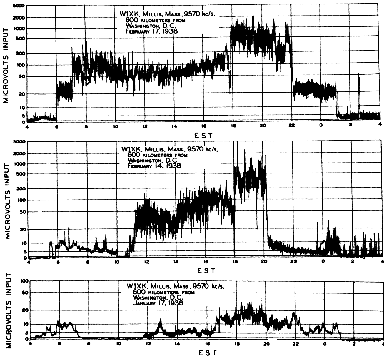
FIGURE 7.7. Field-intensity measured over the same path, on the same frequency, for a quiet day (February 17, 1938), a day of moderate storm (February 14, 1938), and a day of severe storm (January 17, 1938).
