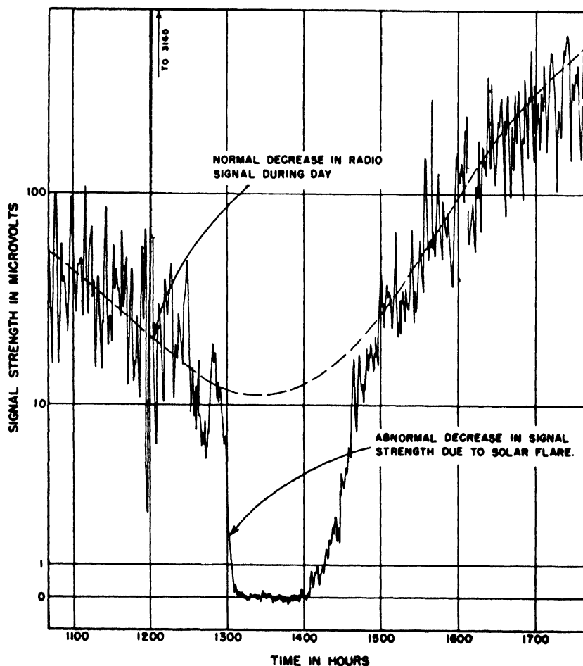
FIGURE 5.9. Effect of solar flare on radio signals received from W8XAL, Mason, Ohio, as measured at Sterling, Va.
