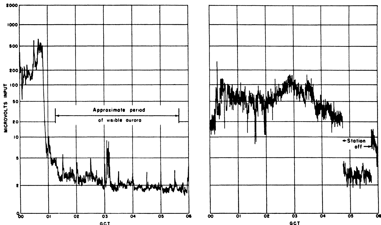
FIGURE 7.8. Field-intensity variation during and after visible aurora of October 8, 1941.
