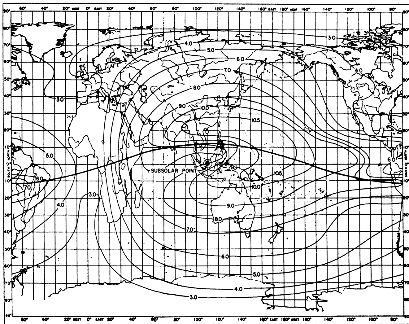
FIGURE 4.17. World-wide distribution of critical frequency of F2 layer ( f^{\circ}F_2 ) in megacycles for equinox, 1945, when it is noon at 111^{\circ} E .
