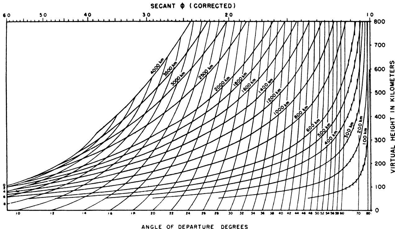
FIGURE 6.7. Transmission curves showing vertical angles.
