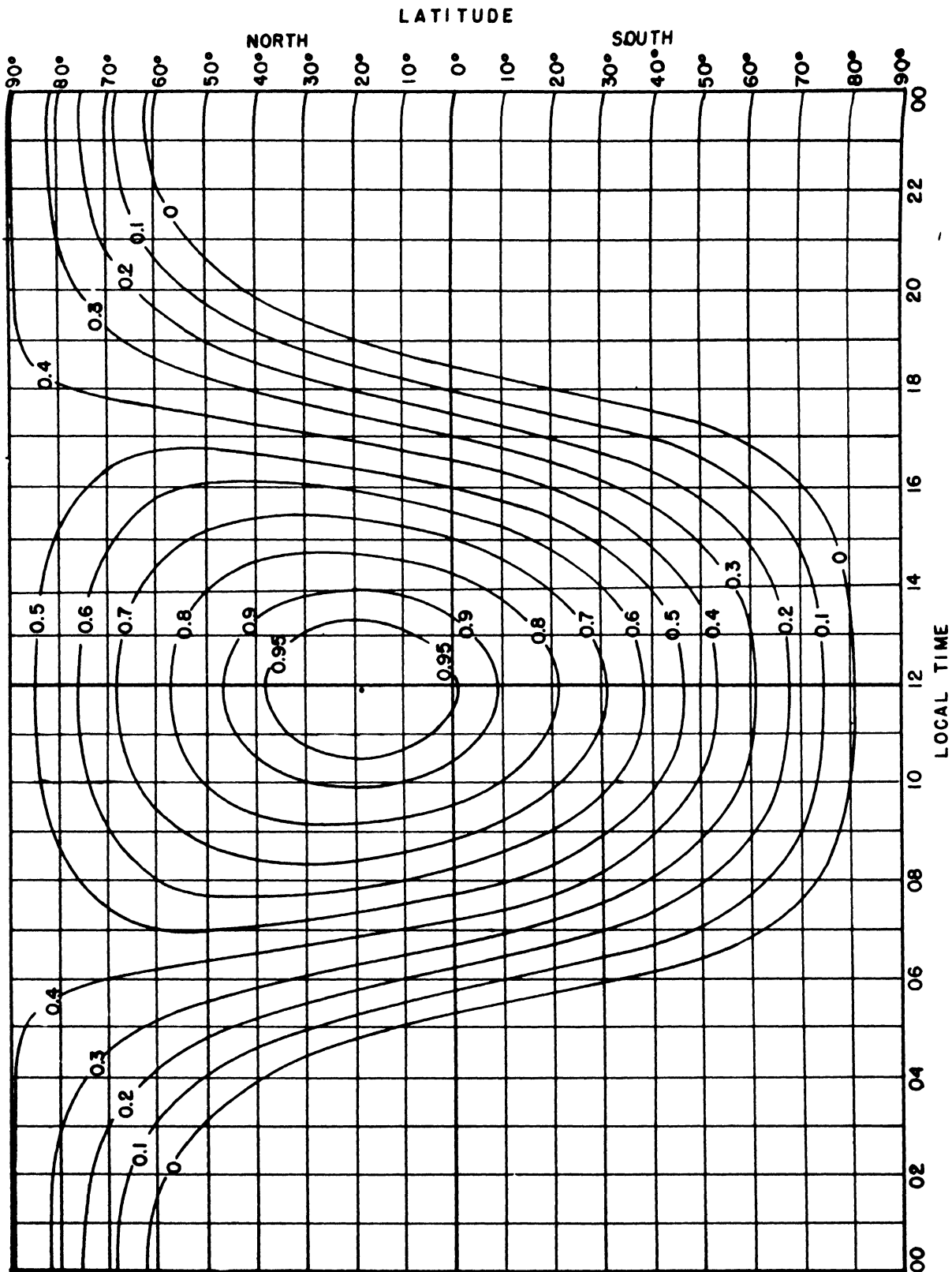
FIGURE 7.38. Absorption factor, K , for May.
