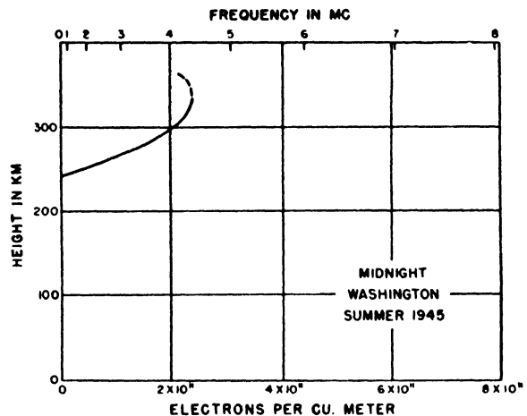
FIGURE 4.8. Distribution of ion density with height for quiet conditions.
