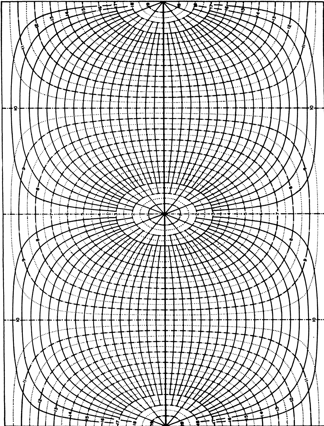
FIGURE 6.30. Great circle chart centered on equator. Solid lines represent great circles. Numbered dot-dash lines indicate distances in thousands of kilometers.
