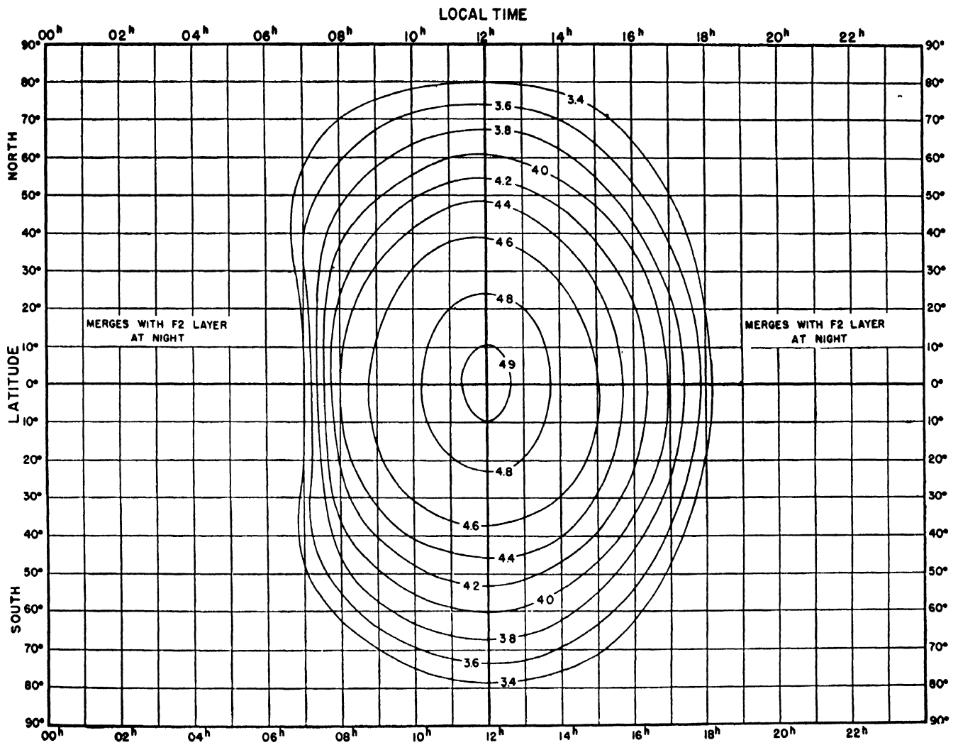
FIGURE 4.11. World-wide distribution of critical frequency of F1 layer ( f^{\circ}F1 ) in megacycles for equinox, 1945.
