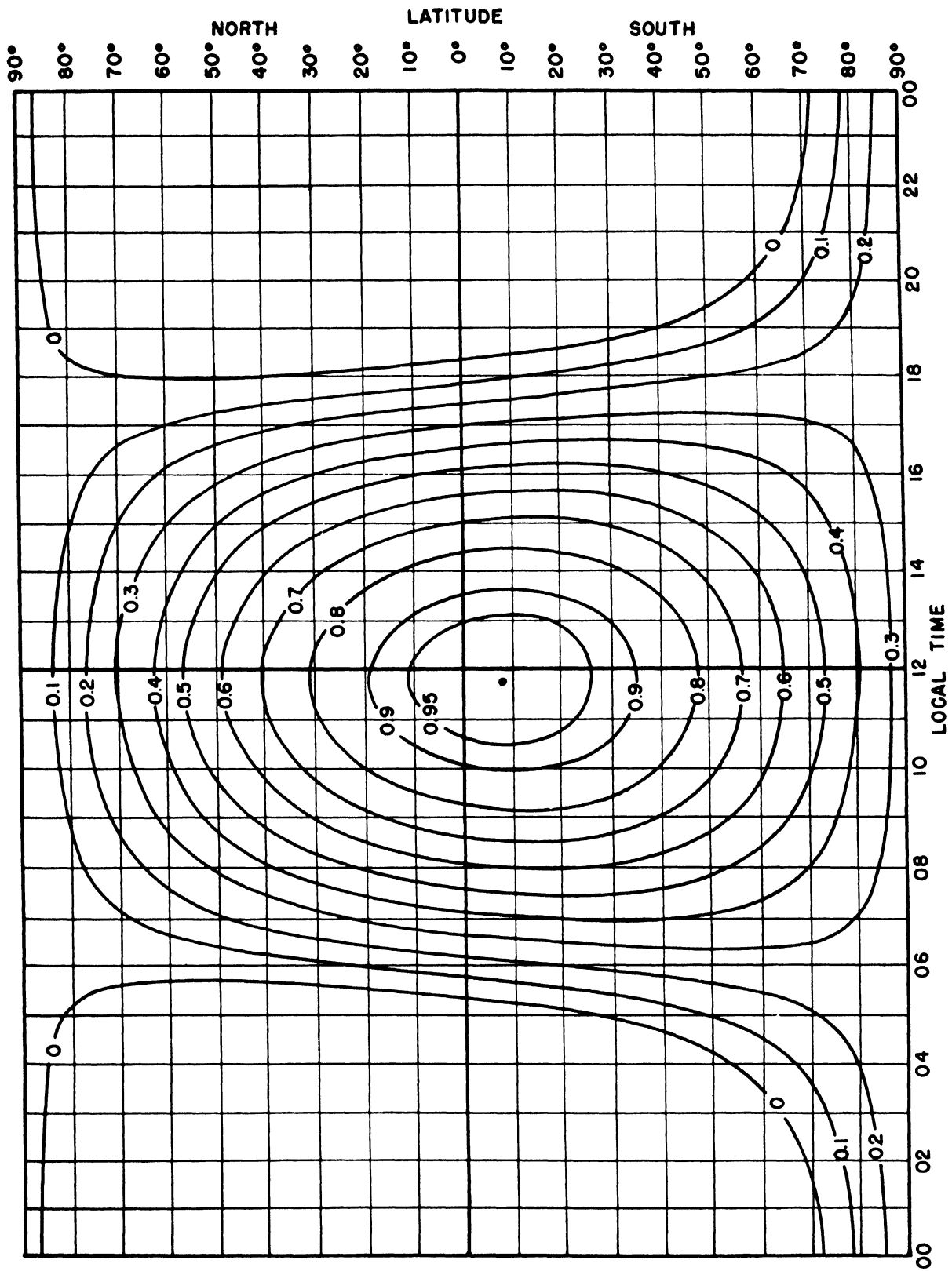
FIGURE 7.43. Absorption factor, K_1 , for October.
