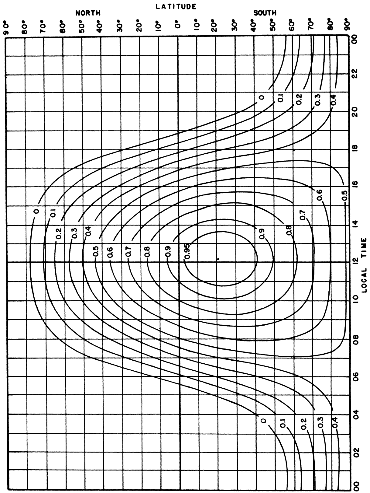
FIGURE 7.34. Absorption factor, K, for January.
