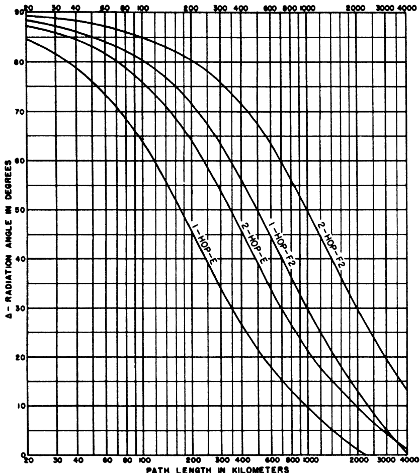
FIGURE 7.3. Radiation angle versus path length, based on virtual reflection heights, E layer—105 km, F2 layer—320 km.
