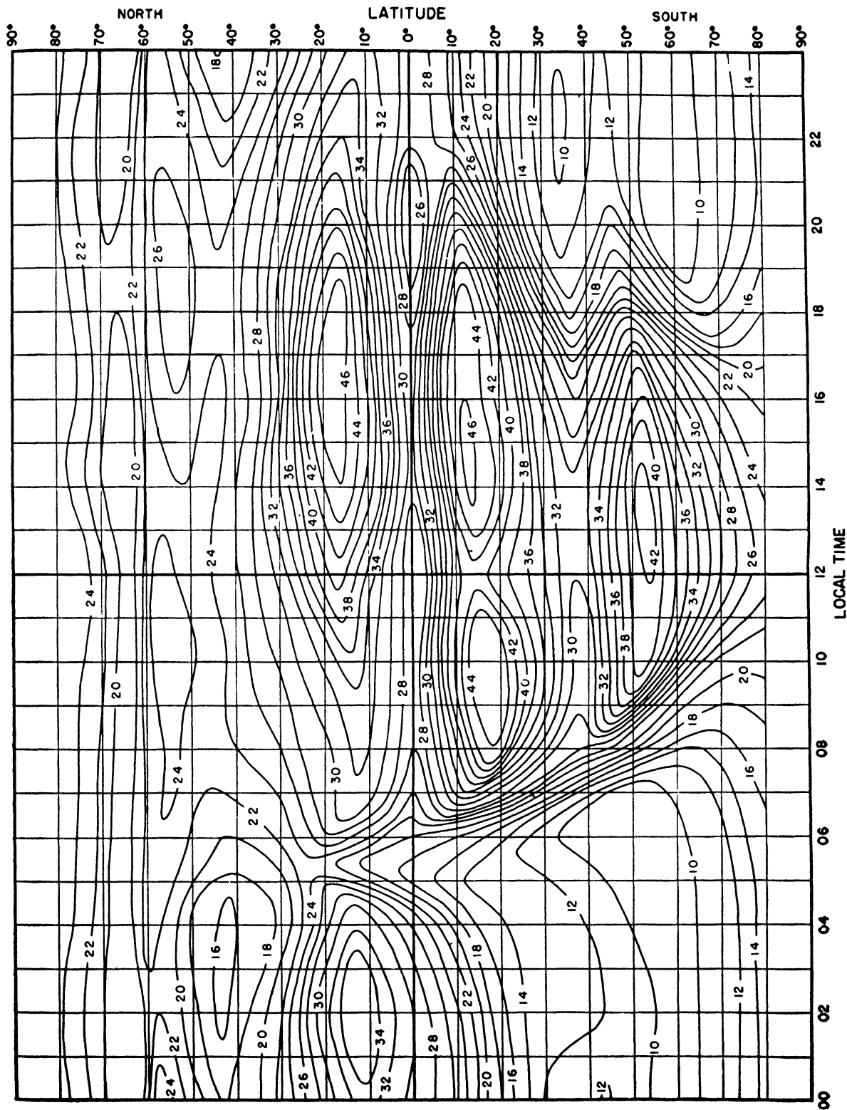
FIGURE 6.24. F 2 4000-muf, in megacycles, I zone, predicted for June 1947.
