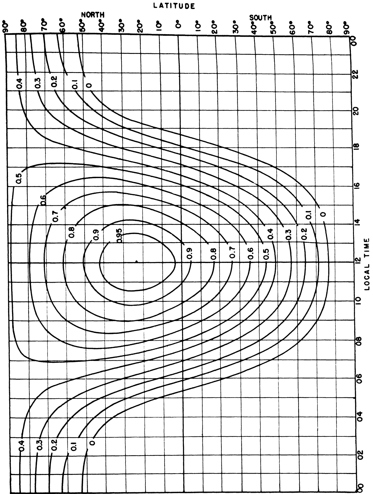
FIGURE 7.39. Absorption factor, K_1 , for June.
