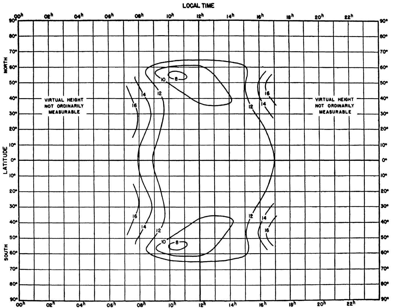
FIGURE 4.13. World-wide distribution of minimum virtual height of E layer ( h'E ) in tens of kilometers for equinox, 1946.
