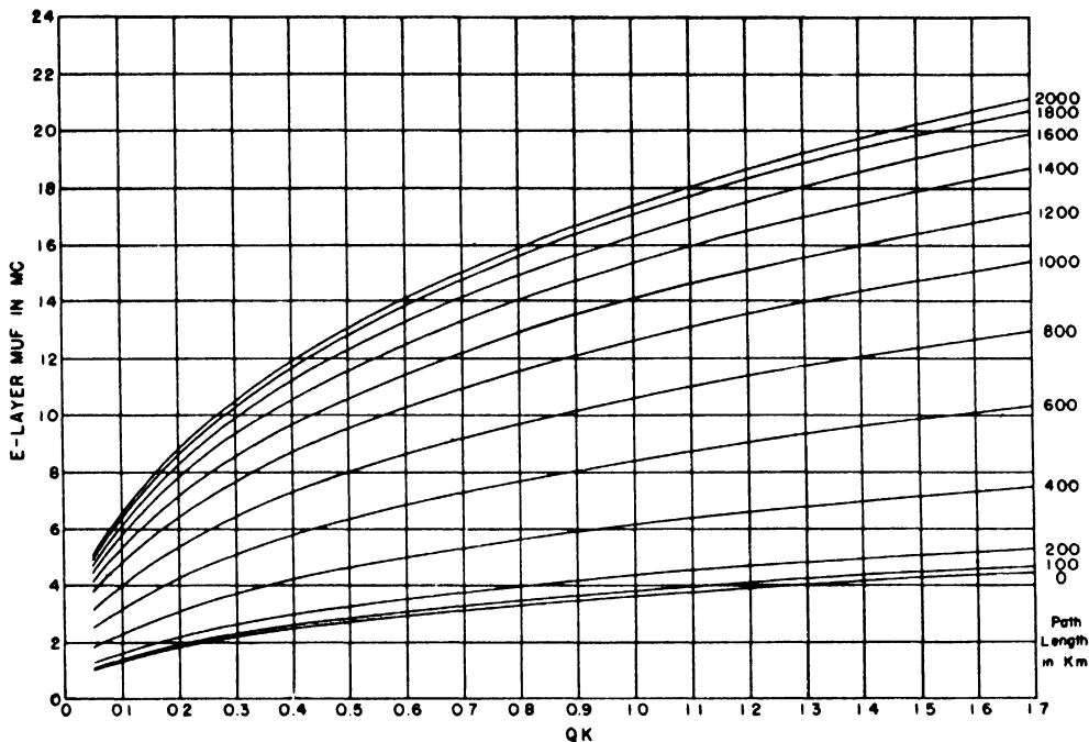
FIGURE 7.2. Approximate E -layer muf as a function of QK (product of solar-cycle variation factor Q and diurnal variation factor K ) and the path length.
