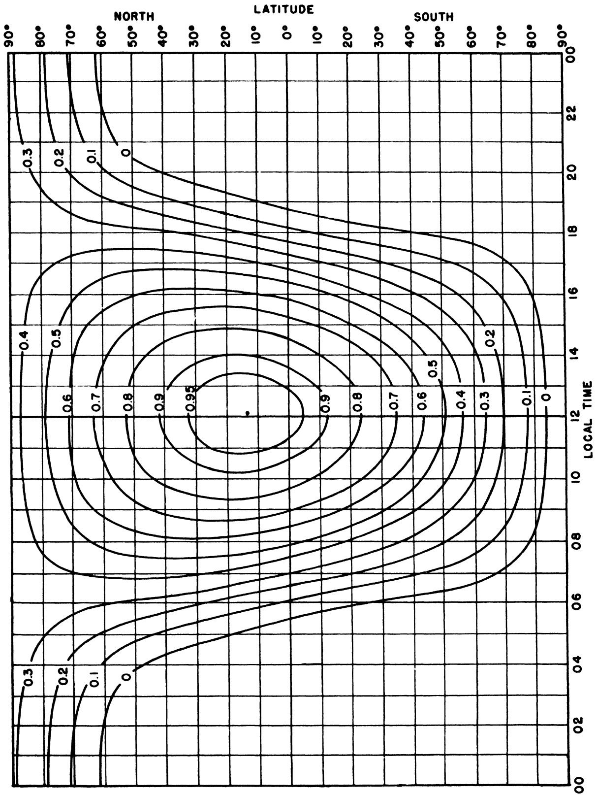
FIGURE 7.41. Absorption factor, K , for August.
