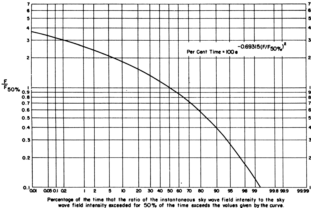
FIGURE 3.11. Rayleigh distribution of the instantaneous sky-wave field intensity.
