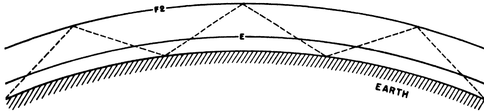
FIGURE 6.8. Propagation by a number of geometric hops.
