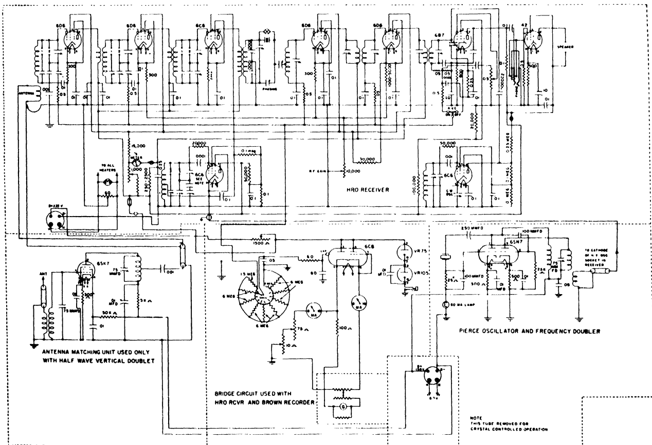
FIGURE 3.14. Automatic field-intensity recording unit.
