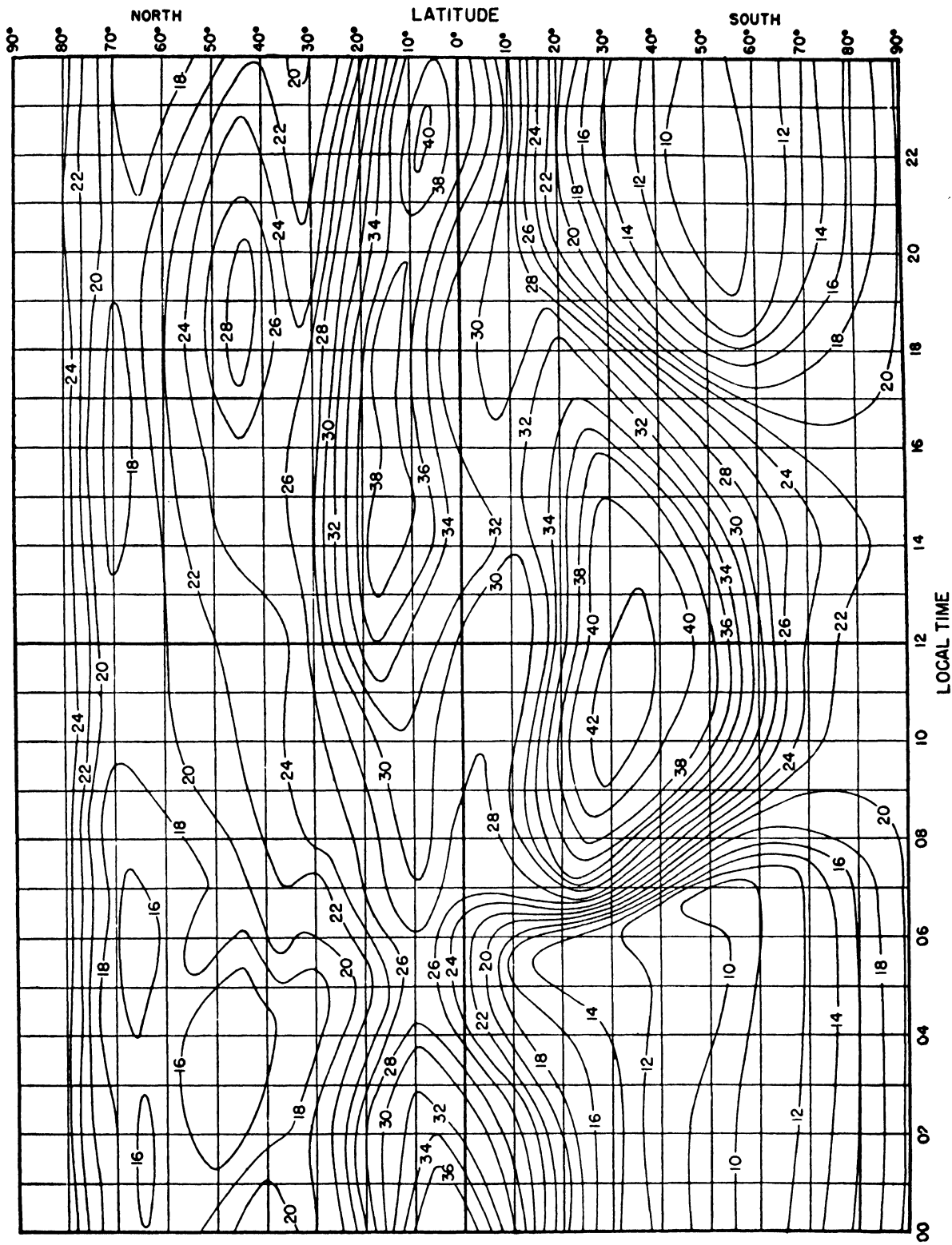
FIGURE 6.22. F_2 4000-muf, in megacycles, W zone, predicted for June 1947.
