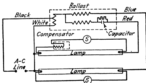
FIG. 96.—Thirty- and forty-watt tulamp circuit showing separate compensator.
