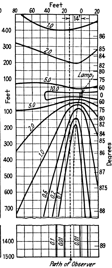
FIG. 126.—Iso-foot-candle diagram for traffic-worn asphalt to give uniform pavement brightness of 0.32 candle per square foot (lamp mounted 25 ft. high).
