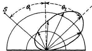
FIG. 73.—Semi-mat-surface reflection.
