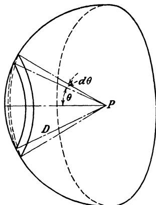
FIG. 52.—Hemispherical source.
