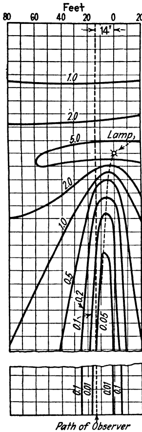
FIG. 125.—Iso-foot-candle diagram for traffic-worn concrete to give uniform pavement brightness of 0.32 candle per square foot (lamp mounted 25 ft. high).
