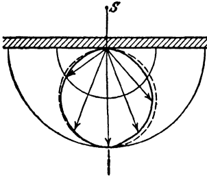
FIG. 82.—Solid opal glass transmission.
