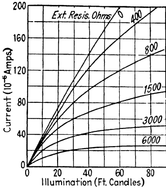
FIG. 27.—General Electric light-sensitive cell (tungsten lamp source at 2700°K.).
