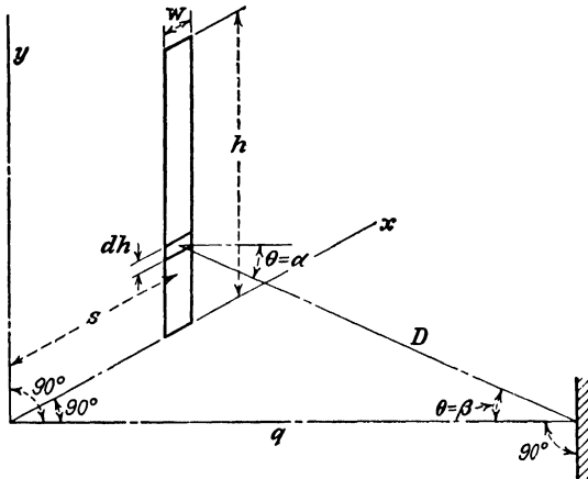
FIG. 65.—A strip source with the point P on a perpendicular erected from a point displaced a distance s from one end and on a parallel plane.
