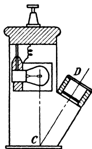
FIG. 24.—Cross section of reference standard.
