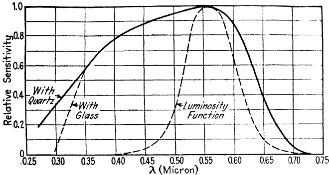
FIG. 30.—Spectral sensitivity of Weston, type 2, photonic cell.
