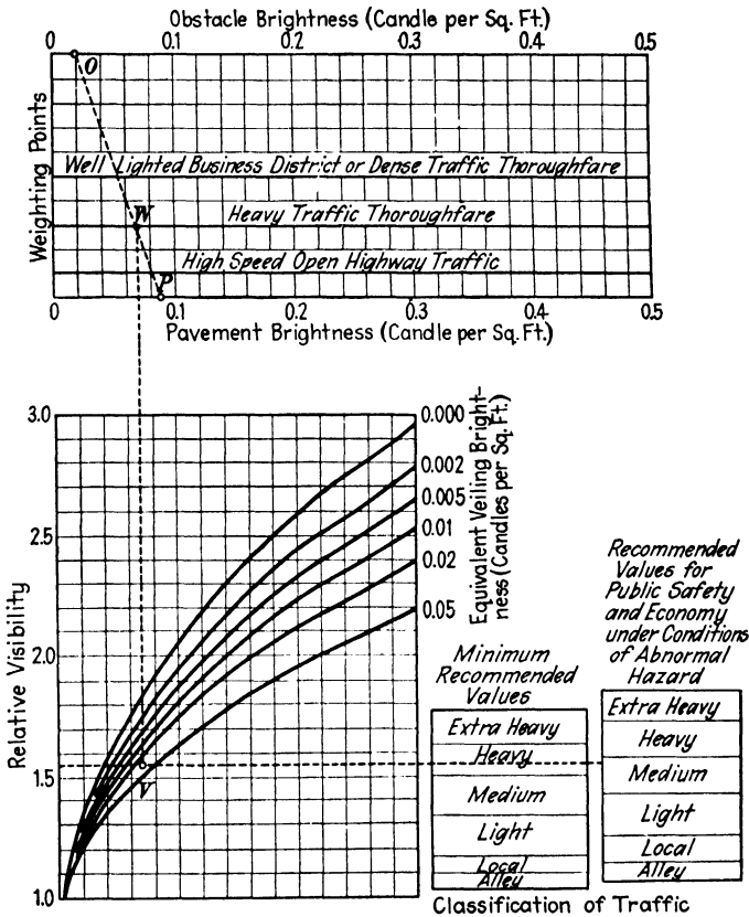
FIG. 129.—Street-lighting evaluation chart for observer in motion at 25 to 40 miles per hour.
