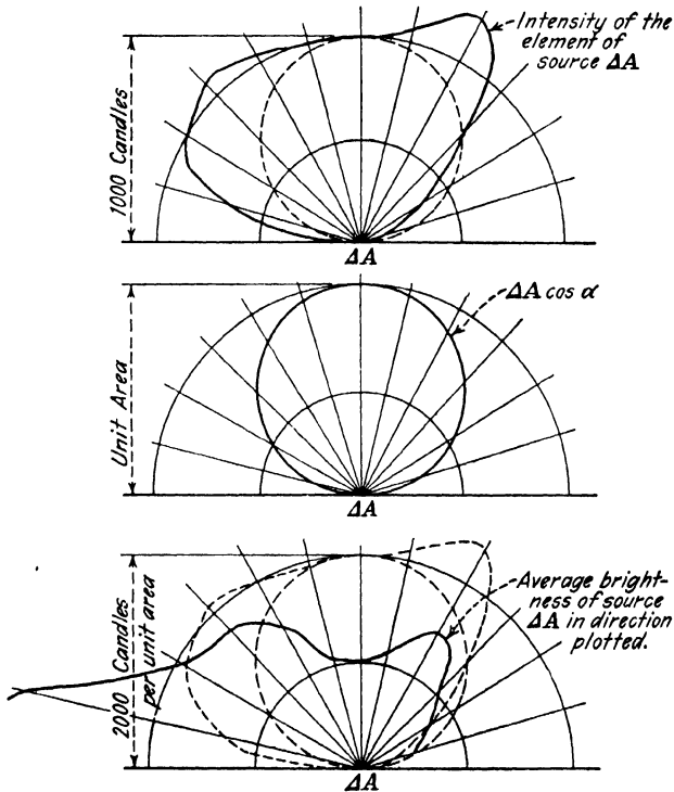
FIG. 45.—Method of determining brightness-distribution curve from an intensity-distribution curve for an elementary source.
