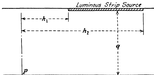
FIG. 68.—Example of continuous strip source not extending to the point P .
