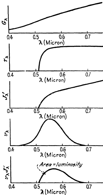
FIG. 89.—Process of evaluating luminosity through the emission due to transmission.
