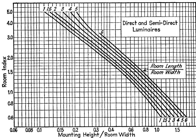
FIG. 110.—Room-index chart for directly and semi-directly illuminated rooms.
