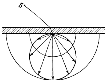
FIG. 81.—Diffuse transmission.
