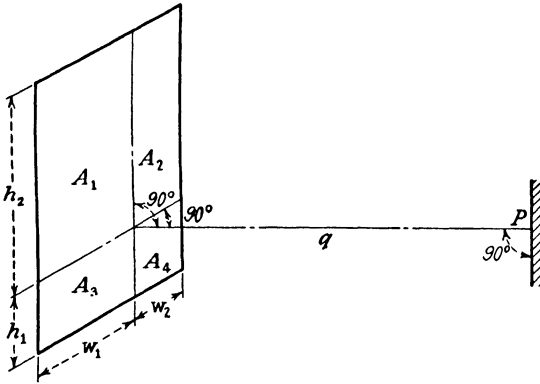
FIG. 62.—A rectangular source with the point P on a perpendicular erected within the boundary of the source and on a parallel plane.
