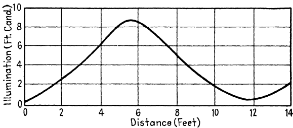
FIG. 47.—Illumination on the working plane along a line passing under a fixture.
