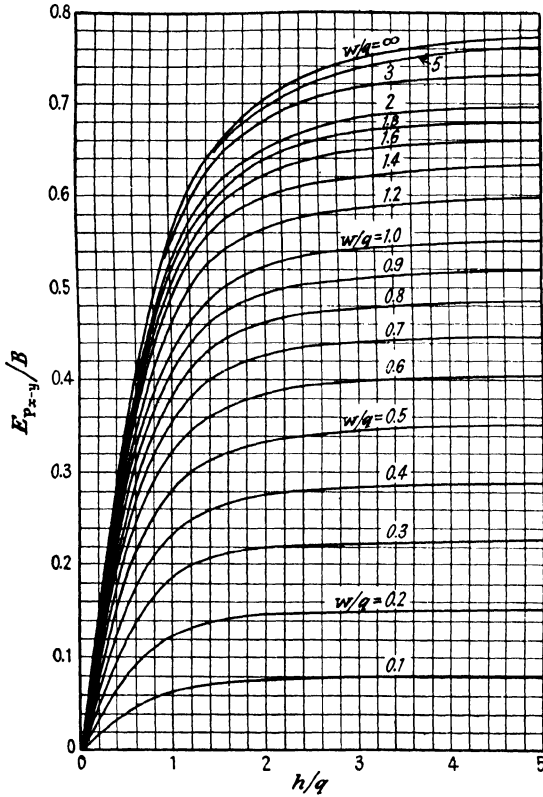
FIG. 60.—Plot of variables of equation (79). (Rectangular source on a parallel plane.)
