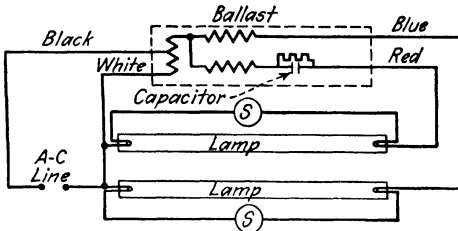
FIG. 98. One hundred-watt tulamp circuit.
