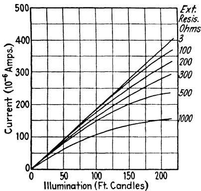
FIG. 25.—Weston, type 1, photonic cell (tungsten lamp source at 2700^{\circ}\text{K} ).
