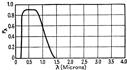
FIG. 87.—Spectral transmission of pure water, 21 mm. thick.
