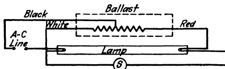
FIG. 101.—Autotransformer type, 30 and 40 watts, 110-125 volts.
