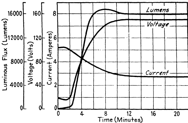
FIG. 92.—Starting characteristic of a 400-watt mercury-vapor lamp.
