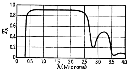
FIG. 86.—Spectral transmission factor of Pyrex glass, 2 mm. thick
