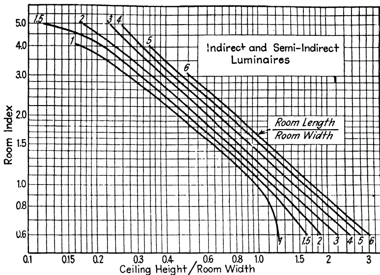
FIG. 109.—Room-index chart for indirectly and semi-indirectly illuminated rooms.
