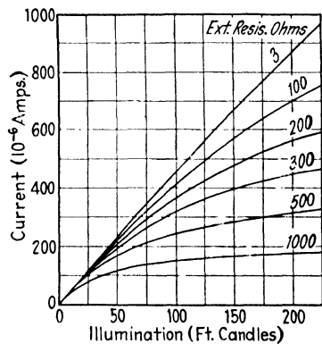
FIG. 26.—Weston, type 2, photonic cell (tungsten lamp source at 2700^{\circ}\text{K} ).
