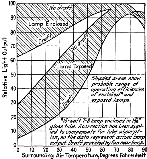
FIG. 107.—Relative light output of a 15-watt fluorescent lamp as affected by air temperature, air movement, and enclosures.
