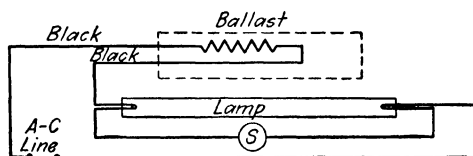
FIG. 104.—Fifteen- and twenty-watt single-lamp low-power-factor circuit; thirty- and forty-watt for 199-216 and 220-250 volts. Also 65-watt.
