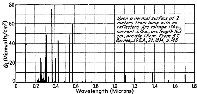
FIG. 4.—Irradiation from a high-pressure mercury vapor lamp.
