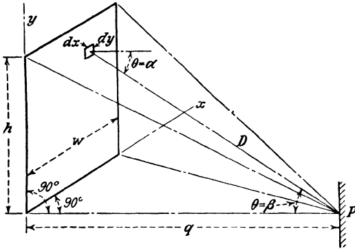
FIG. 58.—A rectangular source with the point P on a perpendicular erected at one corner of the source and on a parallel plane.
