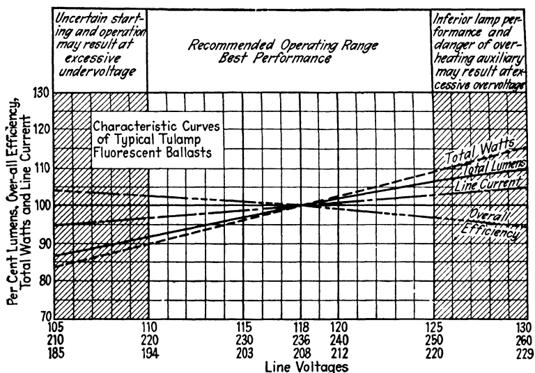
FIG. 105.—Characteristic curves of typical tulamp fluorescent ballasts.
