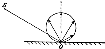
FIG. 71.—Intensity-distribution curve for diffuse reflection.
