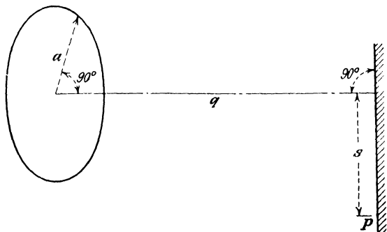
FIG. 55.—A circular disk with P not on the axis but upon a parallel plane.
