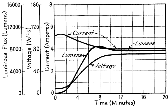
FIG. 93.—Starting characteristic of a 250-watt mercury-vapor lamp.
