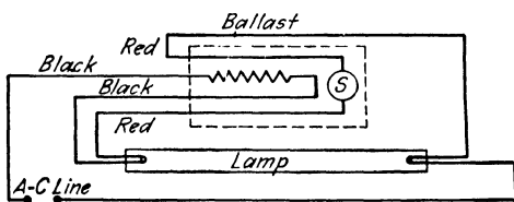
FIG. 103.—Six- and eight-watt circuit.
