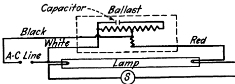
FIG. 100.—Sixty-five-watt high power-factor single-lamp circuit.
