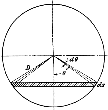
FIG. 42.—Zonal areas as determined through angular position.
