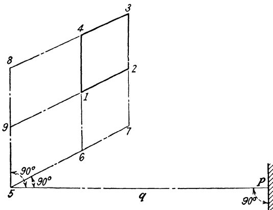
FIG. 64.—A rectangular source with the point P on a perpendicular erected outside the boundary of the source and on a parallel plane.
