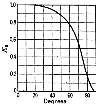
FIG. 33.—Effect of angle-of-light incidence on the current output of a Weston, type 1, cell. ( K_{\theta} = numeric by which the scale reading must be divided to yield the true value.)
