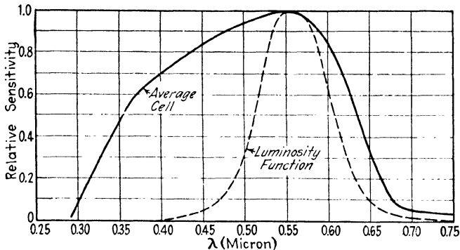
FIG. 31.—Spectral sensitivity of General Electric light-sensitive cell.
