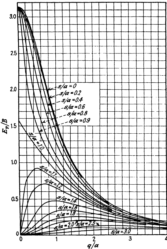
FIG. 56.—Plot of variables of equation (76). (Circular disk source on a parallel plane.)
