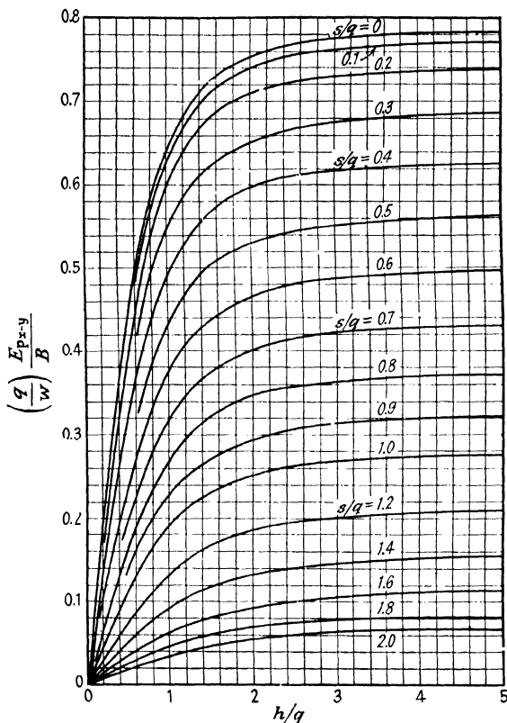
FIG. 66.—Plot of variables of equation (87). (Strip source on a parallel plane.)
