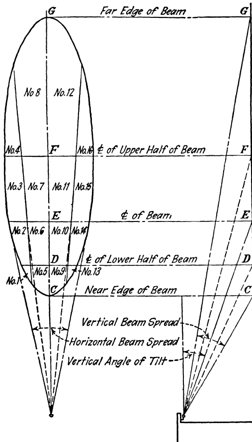
FIG. 120.—Beam outline on illuminated surface.
