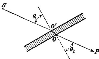
FIG. 80.—Transparent transmission.
