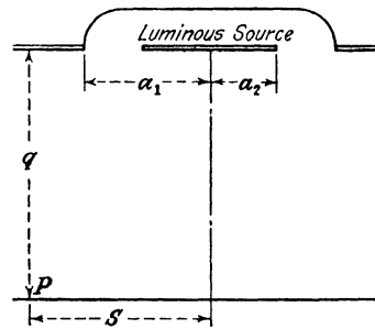
FIG. 57.—Example of subtractive method of illumination determination.
