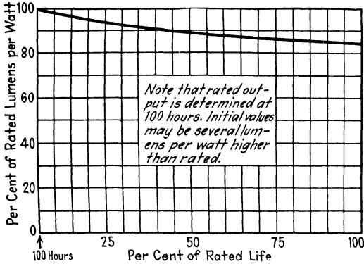
FIG. 106.—Fluorescent lamp lumen maintenance.
