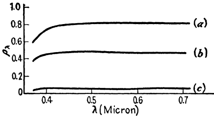
FIG. 76.—Spectral reflection factors for several fairly nonselective surfaces.
