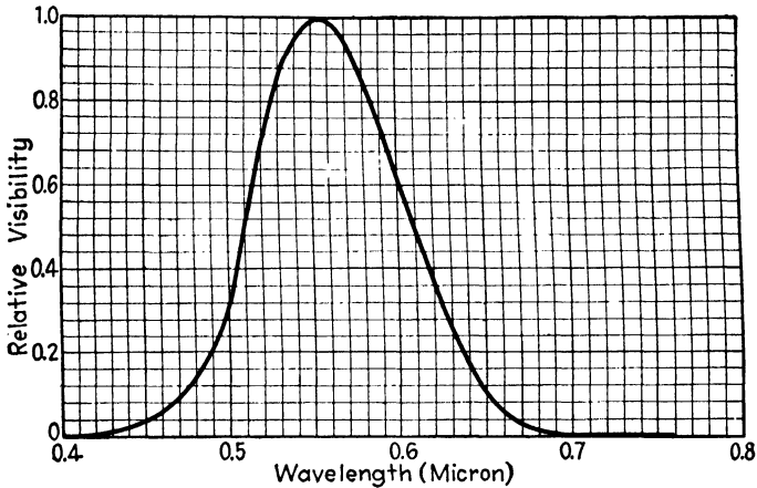
FIG. 11.—The luminosity function.
