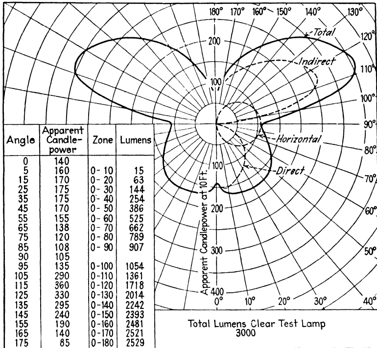
FIG. 114.—Separation of candle-power distribution curve into three component curves.
