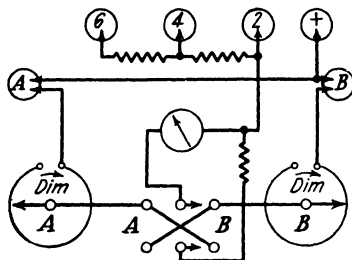
FIG. 23.—Schematic diagram of controller.
