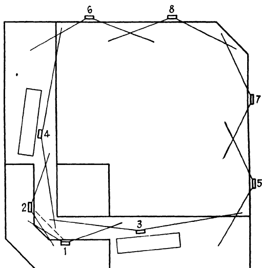
FIG. 121.—Floodlighting of baseball fields.
