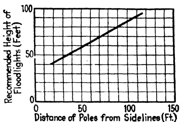
FIG. 123.—Recommended mounting heights for football floodlighting units.
