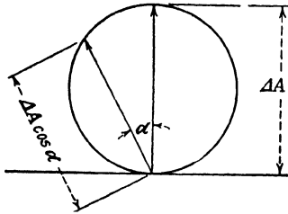
FIG. 44.—Cosine function plotted in polar coordinates.
