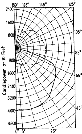
FIG. 37.—Intensity (candle-power) distribution for a standard industrial reflector.
