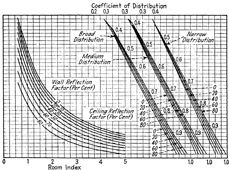
FIG. 113.—Direct component coefficients of distribution.
