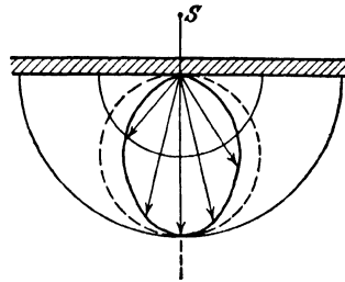
FIG. 83.—Flashed opal glass transmission.
