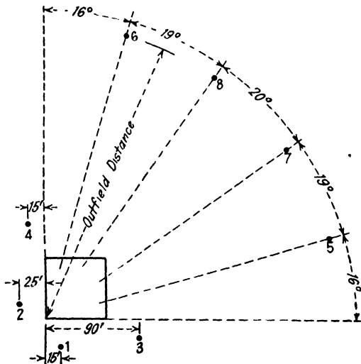
FIG. 122.—Floodlighting of Class A softball fields.
