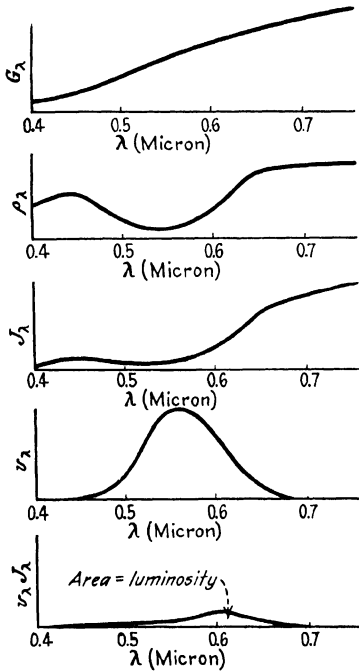
FIG. 78.—Process of evaluating luminosity through the emission due to reflection.
