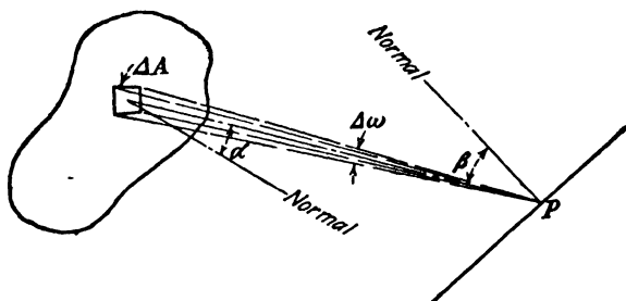
FIG. 21.—Solid angle subtended by a source.
