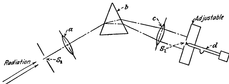
FIG. 2.—A spectroradiometer.
