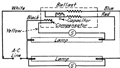
FIG. 95.—Fifteen- and twenty-watt tulamp circuit with integral starting compensator.
