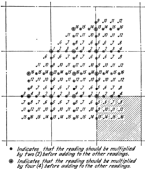
FIG. 116.—General plan of adding illuminations by the image method.
