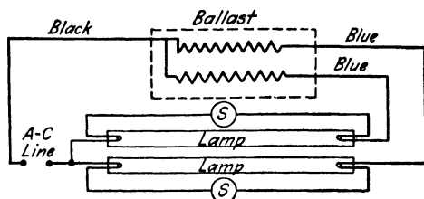
FIG. 102.—Fifteen- and twenty-watt two-multiple low power-factor circuit.
