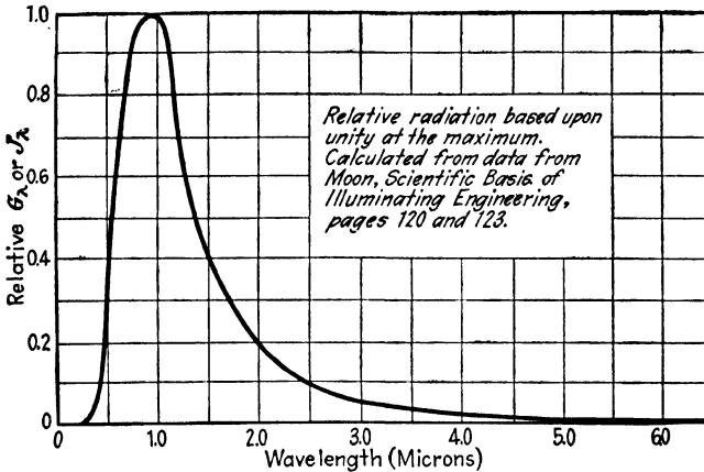
FIG. 8.—Incandescent lamp at 2950°K.
