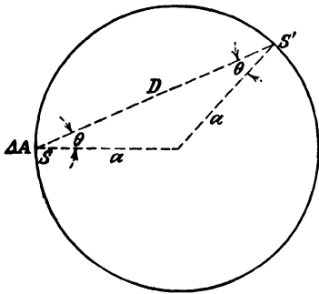
FIG. 36.—The Ulbricht sphere.
