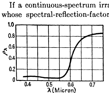
FIG. 77.—A spectral-reflection-factor graph for a red surface.
