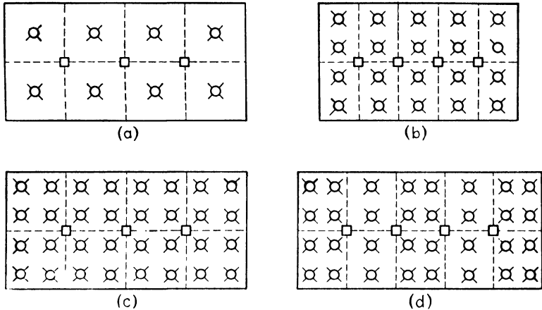
FIG. 108.—Typical layouts. (a) One unit per bay: satisfactory only where the bay size is no greater than the maximum allowable spacing an unusual condition except in high-ceilinged rooms. (b) Two units per bay: usually applicable in narrow bays where the width is less than two-thirds the length. (c) Four units per bay: this is the most common arrangement for the square bay of usual dimensions. (d) Four-two system: equivalent to three units per bay. An alternative to four per bay where spacing allows.
