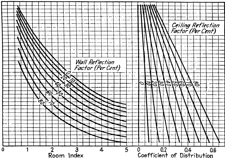
FIG. 111.—Indirect component coefficients of distribution.
