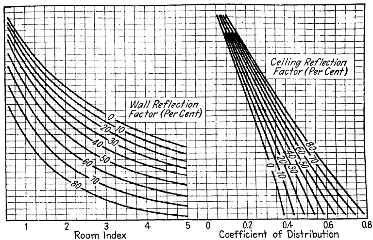
FIG. 112.—Horizontal component coefficients of distribution.
