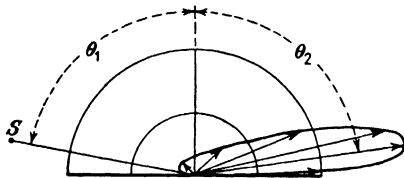
FIG. 74.—Semi-mat-surface reflection at large angle of incidence.
