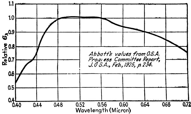
FIG. 7.—Average noon sun at Washington, D.C.
