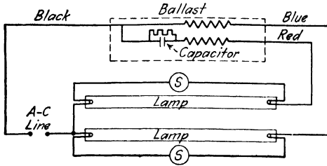
FIG. 97.—Sixty-five-watt tulamp circuit.
