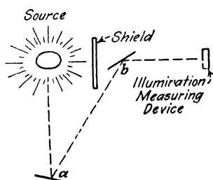
FIG. 34. Distribution photometer with two movable mirrors.
