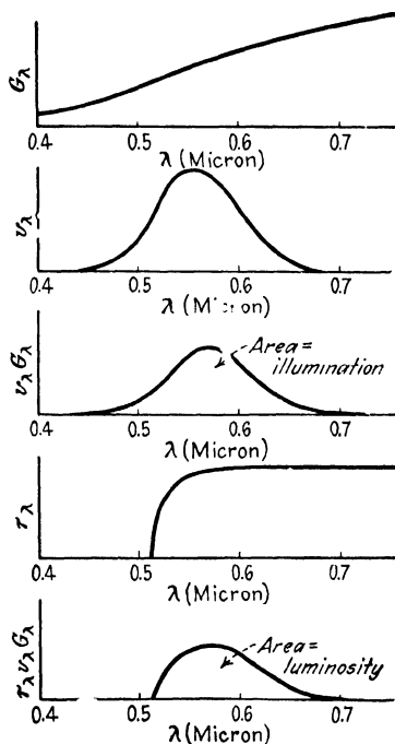
FIG. 90.—Process of evaluating luminosity of a transmitting medium through a previous evaluation of illumination from the irradiation.
