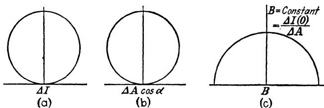
Fig. 46.—Intensity distribution and brightness distribution for a perfectly diffusing source.
