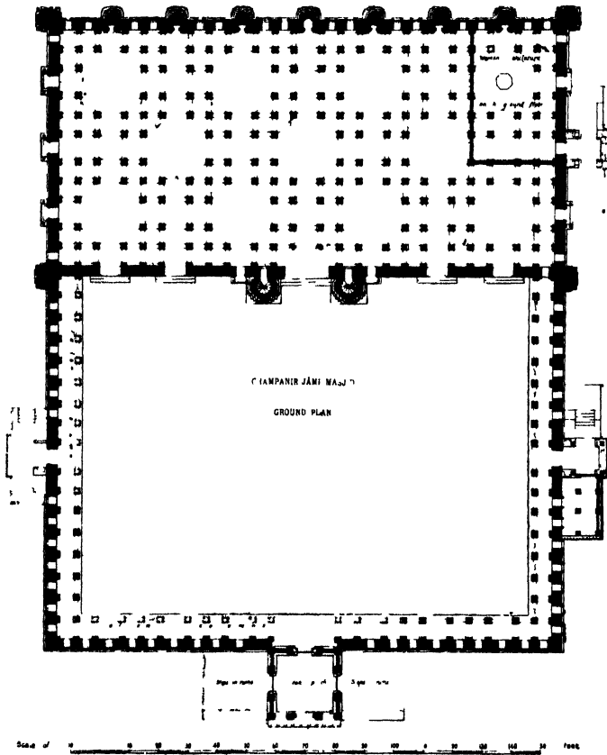
FIG. 33.—Plan of Jâmi' Masjid, Champanîr (drawn by the Archæological Survey of India)
