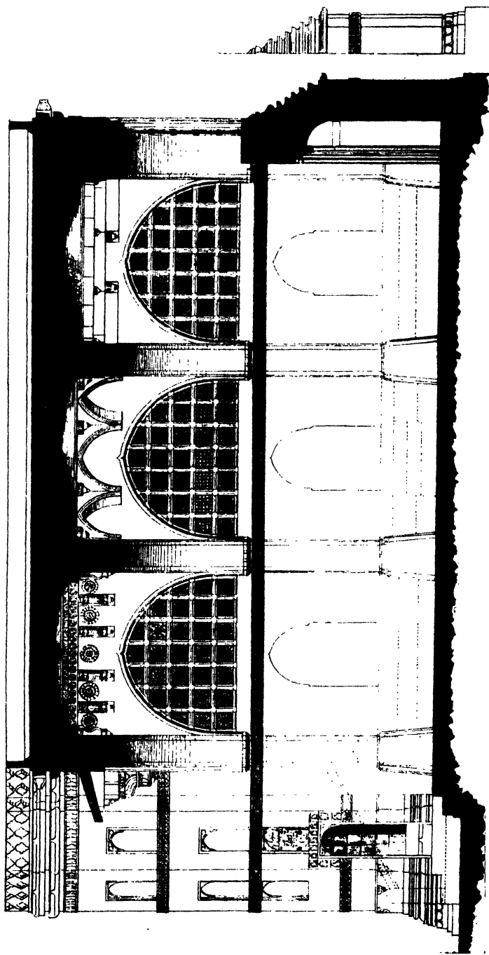
SIDI SAYYID'S MOSQUE, AHMADRABAD: CROSS SECTION OF LIWÂN (Drawn by the Archaeological Survey of India)
