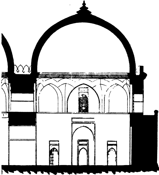
FIG. 29.—Dholkâ. The Khan's Masjid: Section of one of the Compartments of the Liwân (drawn by the Archaeological Survey of India).
