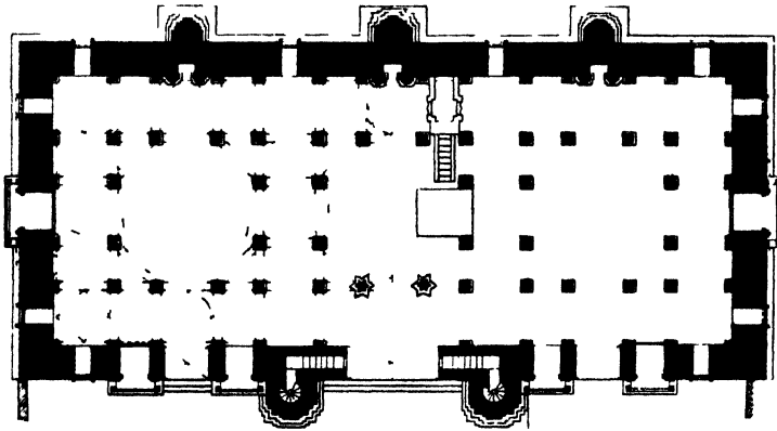
FIG. 36 — Râni Rupâvatî's Masjîd Plan of Liwân (drawn by the Archaeological Survey of India)
