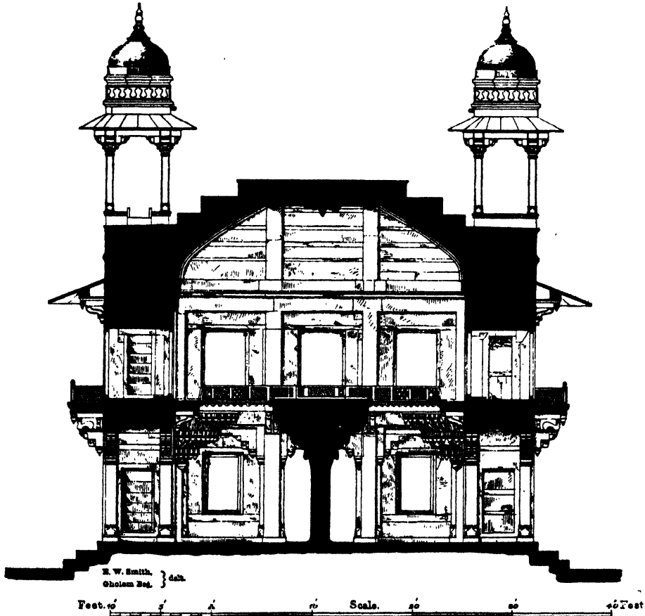
FIG. 40.—Section of the Dîwân-i-Khâs, Fatehpur-Sikri (drawn by the Archæological Survey of India).
