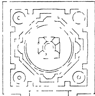
FIG 2 —Roof Plan of Chandī Sewa, Java.
