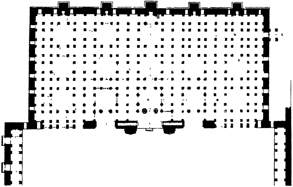
FIG. 11.—Jâmi' Masjid, Ahmadâbâd : Plan of liwân (from a drawing by the Archæological Survey of India).
