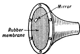
FIG. 58A—Manometric Capsule (Richardson)
