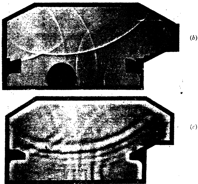
FIG. 154—Comparative Spark and Ripple Photographs (A. H. Davis)
