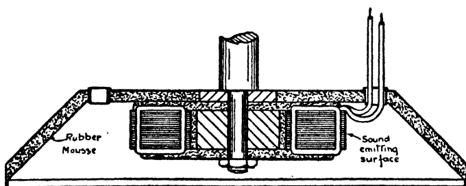
FIG. 146A—Section of Ring Type Oscillator mounted on reflector
