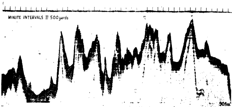
FIG. 147B—Norwegian Tanker Caledonia approaching Oslo, Norway, July 1936
