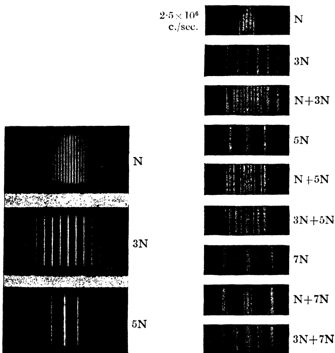
FIG. 75A—Diffraction spectra of sound waves in xylol; fundamental, and 3rd and 5th harmonic
