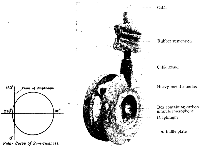
FIG. 125B—Uni-directional Hydrophone
