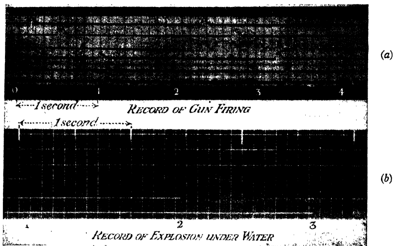
FIG. 153—Sound-ranging Records
