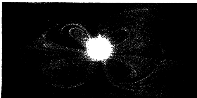
FIG. 59D—The vortex system formed round a sphere, diameter 0.317 cm.
