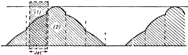
FIG. 64B—Rectangular Jet (1) and special-shaped Holes (2) to make Area of Opening vary sinusoidally
