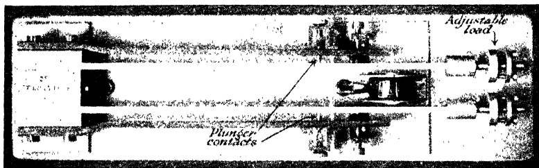
FIG. 40—Electrically-maintained Tuning-Fork (low frequency)
