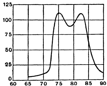
FIG. 121B—Resonance Curve with Double Resonator
