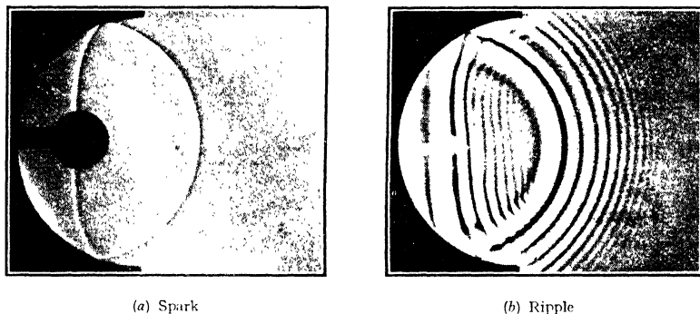
FIG. 109—Comparison of Spark and Ripple Reflections from concave Surface (Dr. A. H. Davis)
