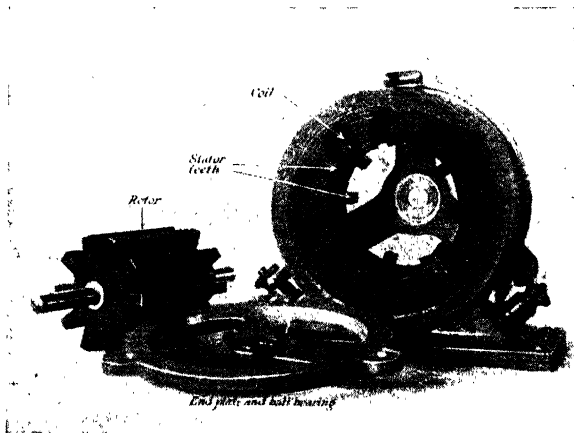
FIG. 43 (b)—Phonic Motor (parts)
