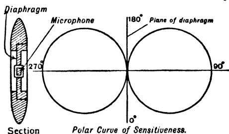
FIG. 125A—Bi-directional Hydrophone
