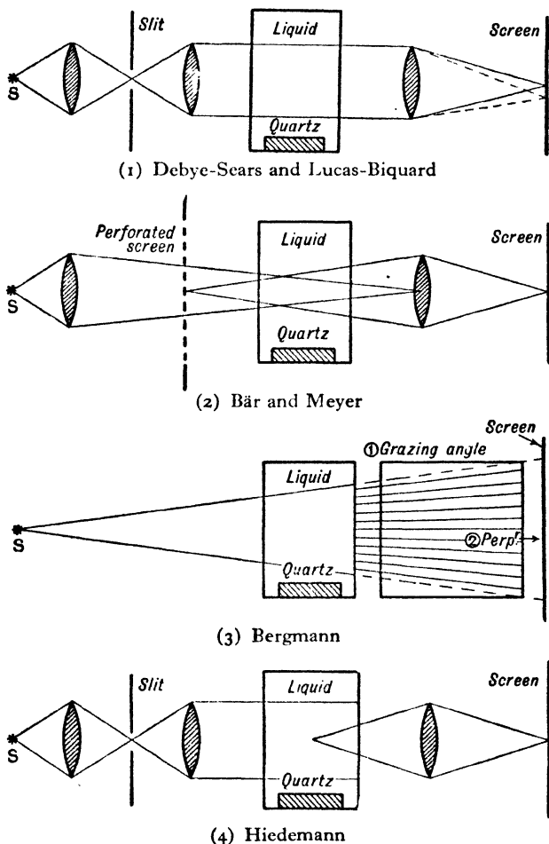
FIG. 75D—H.F. sound in liquids—optical diffraction systems
