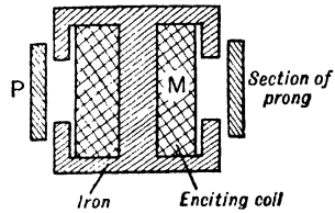
FIG. 41—Section through Magnet and Prongs of Fork
