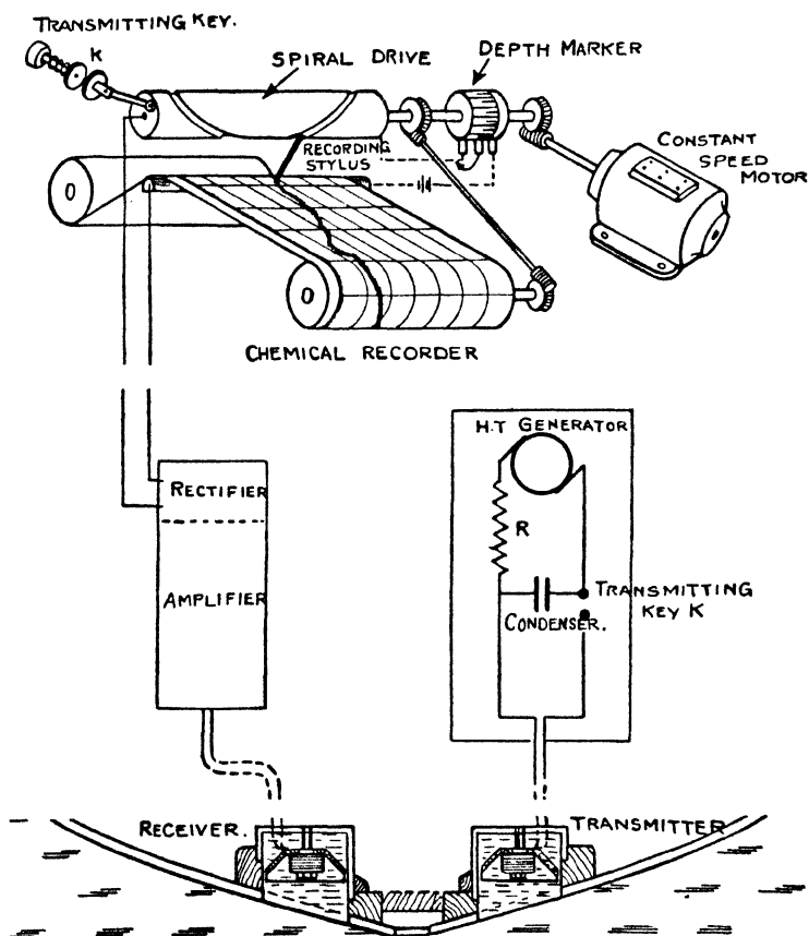
FIG. 146B—Schematic arrangement of Echo Depth-Recorder
