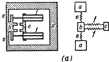
FIG. 113 (a)—Sound Transmitter (Hahnemann)
