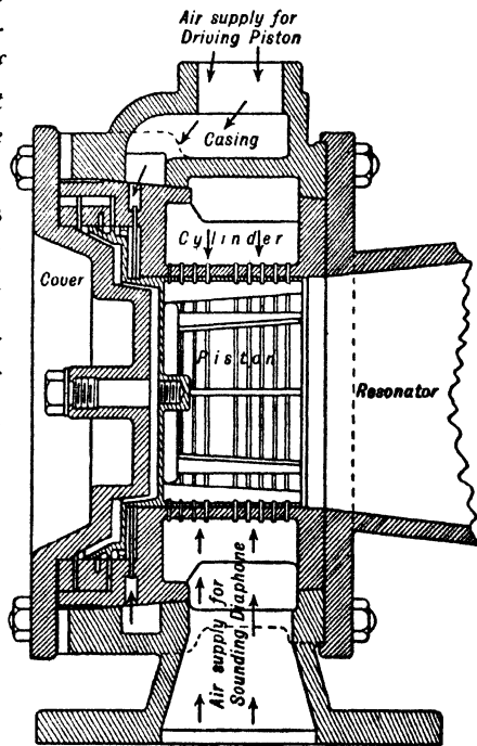
FIG. 65—Diaphone (piston 9 ports .05 inch wide at intervals of 0.29 inch. At 30 lbs. pressure—stroke 0.47 inch, 102 oscillations per second, giving a sound frequency of 204 p.p.s.)
