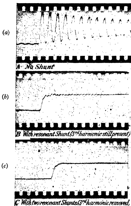
FIG. 133—Oscillograph Records illustrating damping of Einthoven fibre by 'Resonant-Shunt' Method
