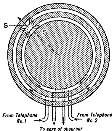
FIG. 123—Binaural Compensator (American)
