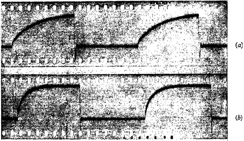
FIG. 39—Oscillograph Records of Current exciting a Tuning-Fork
