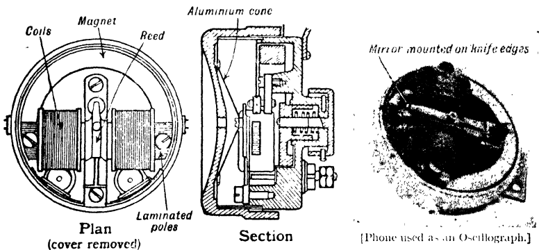
FIG. 114—Brown Reed Telephone
