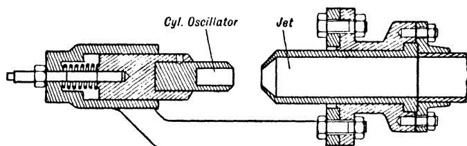
FIG. 55—Hartmann and Trolle's Air-Jet Generator
