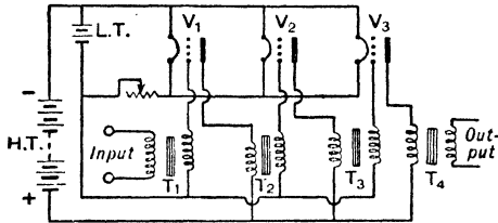
FIG. 26A—Amplifier Transformer Coupling
