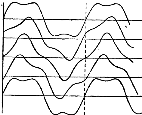
FIG. 15B—Third Harmonic and Fundamental (illustrating effect of varying relative phase)
