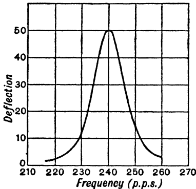
FIG. 121A—'Resonance Curve' of Hot-Wire Microphone—Single Resonator
