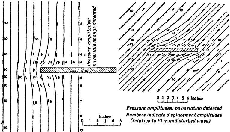
FIG. 97—Sound Distribution round a Lead Disc in Water
