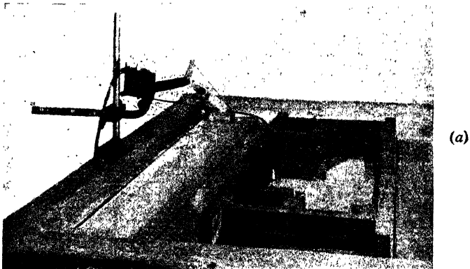
FIG. 154—Ripple Tank (with model section of auditorium)
