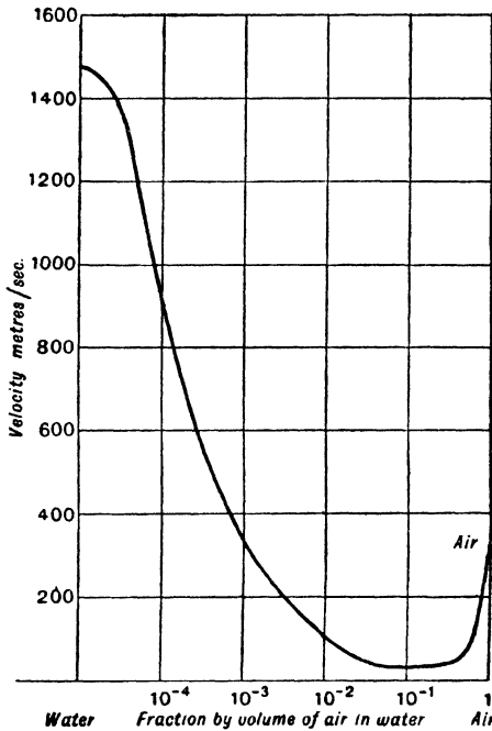
FIG. 100—Velocity of Sound in Air-Water Mixtures
