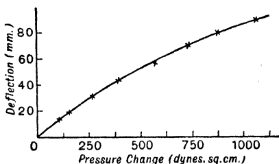
FIG. 58B—Calibration Curve of Manometric Capsule (Richardson)
