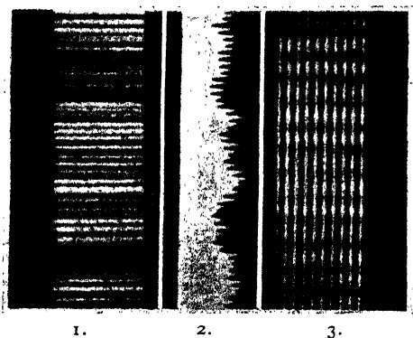
FIG. 157—Typical Sound-Film Records
