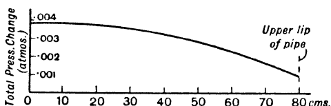
FIG. 59A—Pressure Amplitude along a Stopped Pipe (Richardson)
