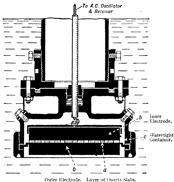
FIG. 48—Langevin Quartz Supersonic Transmitter
