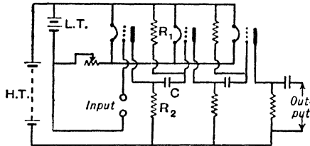
FIG. 26B—Amplifier Resistance-Capacity Coupling
