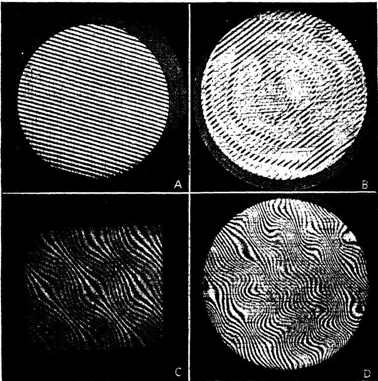
FIG. 52—Vibrations of Quartz Plates (stroboscopic interferometer method) A. Circular disc at rest. B and D. Same disc as A in vibration. C. Rectangular plate in vibration. (By courtesy of Dr. D. W. Dye, F.R.S.)
