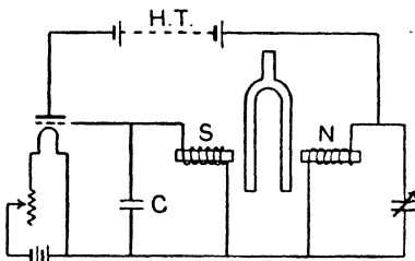
FIG. 42—Valve-maintained Tuning-Fork (Eccles)
