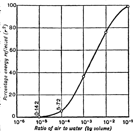
FIG. 101.—Reflection of Sound from Air-Water Mixtures
