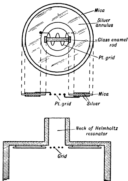
FIG. 120—Hot-Wire Microphone (Tucker)
