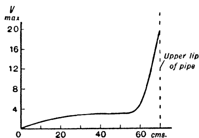
FIG. 59B—Displacement or Velocity Amplitude along a Stopped Pipe (Richardson)
