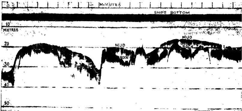
FIG. 147A—Approaching Aarhus, Denmark, record shows mud overlying rocky bottom
