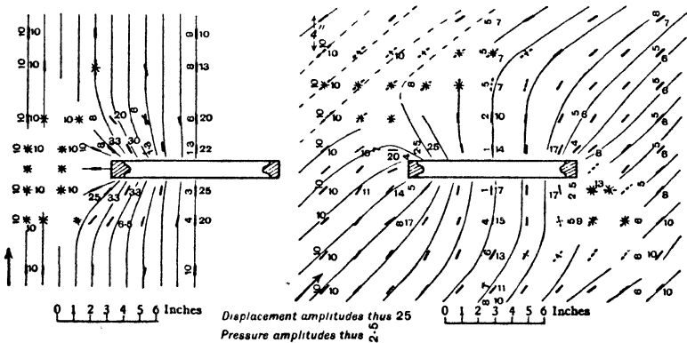
FIG. 98—Sound Distribution round an " Air-Disc " in Water
