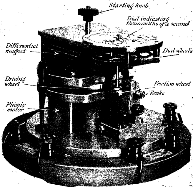
FIG. 151—Phonic Chronometer ( Journal of Scientific Instruments )
