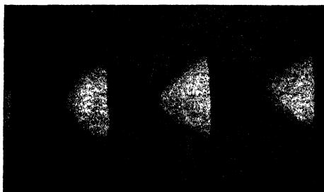
FIG. 54—Schlieren photograph showing structure of jet of Hartmann and Trolle's Air-Jet Generator
