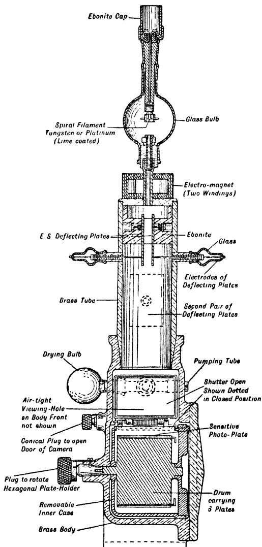
FIG. 134—Cathode Ray Oscillograph (section) (By courtesy of the Physical Society)
