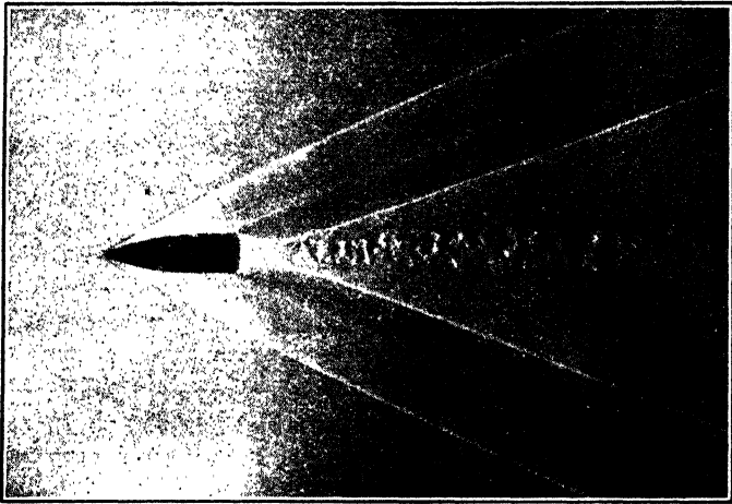
FIG. 78— Photograph of a high-speed Bullet in Flight (By courtesy of Prof. W. Cranz)
