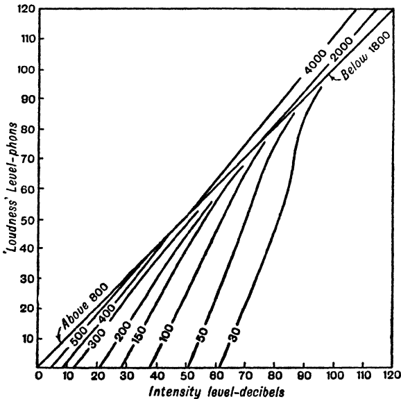
FIG. 158—Intensity-Loudness Relations (after Fletcher and Munson)
