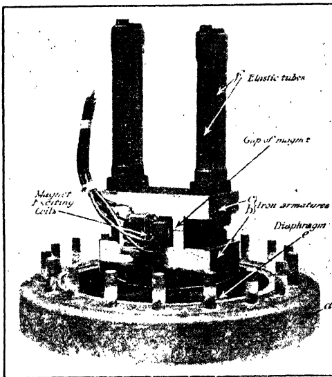
FIG. 113 (b)—Sound Transmitter (Hahnemann)
