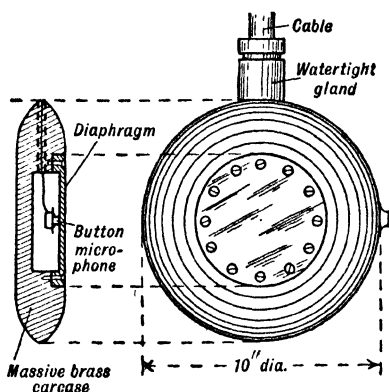
FIG. 122—Non-directional Hydrophone
