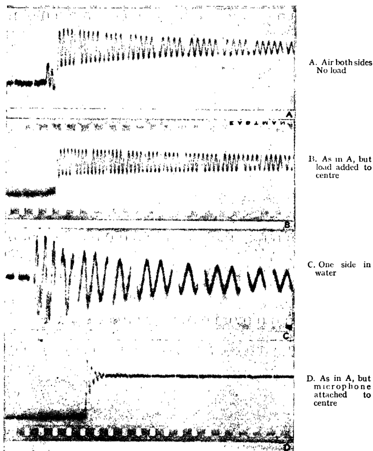
FIG. 51— Damping of a Steel Diaphragm
