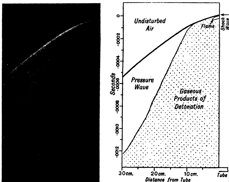
FIG. 108—Schlieren Photo of Pressure Wave (Payman, Shepherd and Robinson)
