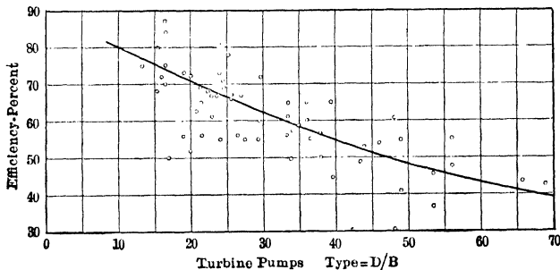
FIG. 80.—Efficiency as a function of impeller type.
