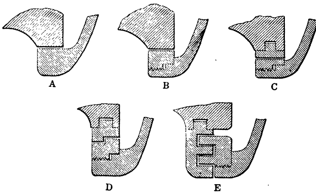
FIG. 23.—Various forms of clearance rings.
