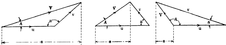
FIG. 45.—Relation between absolute and relative velocities.
