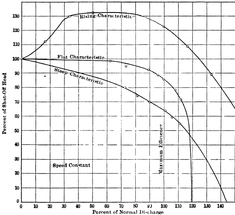
FIG. 11.—Head-discharge characteristics.
