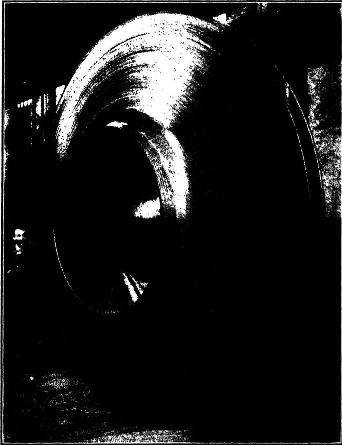
FIG. 20.—Impeller for a 42-inch centrifugal pump. Diameter of impeller = 144 inches, capacity = 44,800 G.P.M., h = 35 ft., N = 100 r.p.m. (R. D. Wood and Co.)
