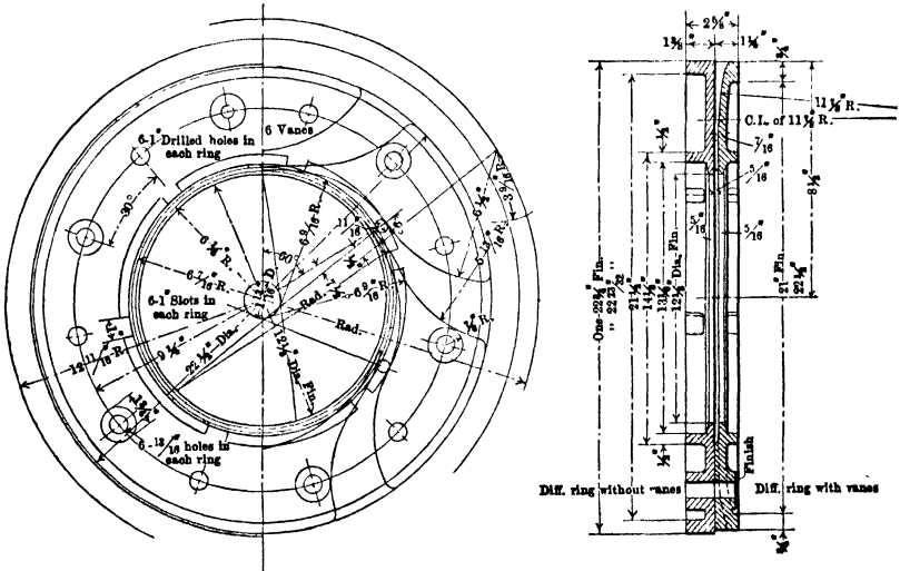
FIG. 65.—Diffuser for Worthington turbine pump.
