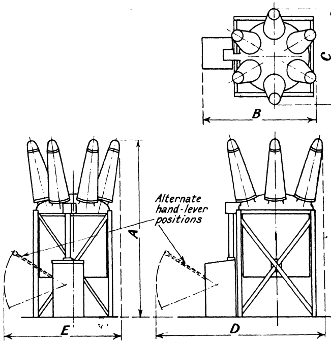
FIG. 118. OUTLINE OF FRAME MOUNTING OIL CIRCUIT-BREAKER HAVING ALL PHASES IN ONE TANK Used up to 88 kV.
