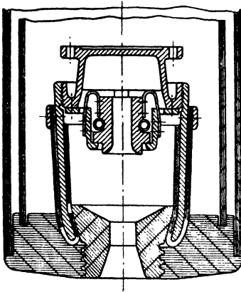
FIG. 125. SECTION THROUGH EXPLOSION POT CONTACT (A.E.G.)
