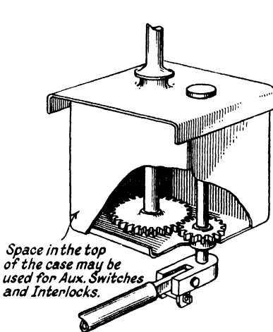
FIG. 79. ISOLATING SWITCH OPERATING HANDLE GIVING 180^\circ ROTATION OF THE HANDLE FOR 90^\circ ROTATION OF THE SWITCH
