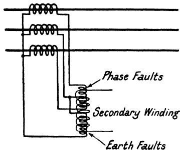
FIG. 213. DIAGRAM ILLUSTRATING SUMMATION OF THREE-PHASE CURRENTS FOR PROTECTIVE RELAYS
