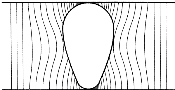
FIG. 34. DISTORTION TO THE DIELECTRIC FIELD BETWEEN PARALLEL-PLATE ELECTRODES CAUSED BY THE INTRODUCTION OF AN EGG-SHAPED PORCELAIN PLACED VERTICALLY BETWEEN THE ELECTRODES
