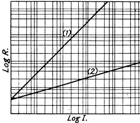
FIG. 192. VALUES OF RI = CONSTANT
