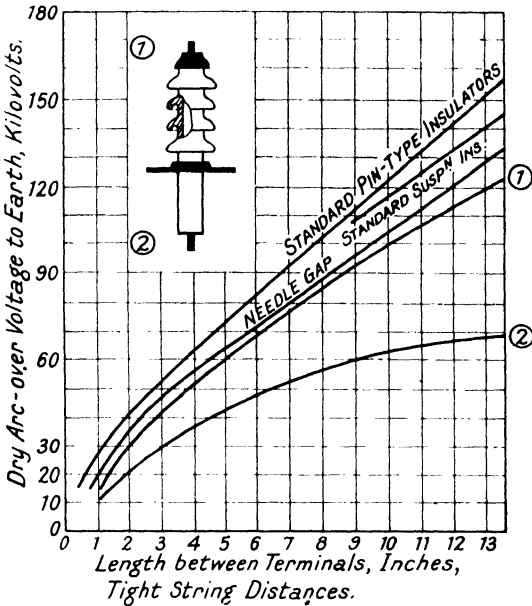
FIG. 39. DRY SPARK-OVER VOLTAGE OF VARIOUS TYPES OF INSULATORS Lapp Insulator Co., U.S.A.
