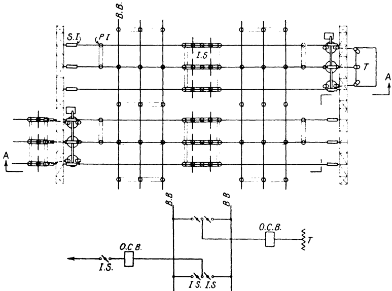
FIG. 18. AN ALTERNATIVE ARRANGEMENT TO FIG. 17 WITH PARALLEL MOUNTING FOR ISOLATORS Note double isolator for bus-bars.
