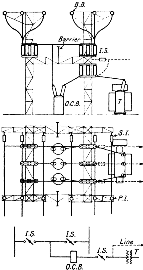
FIG. 15. DOUBLE BUS-BAR ARRANGEMENT WITH GANG-OPERATED ISOLATING SWITCHES
