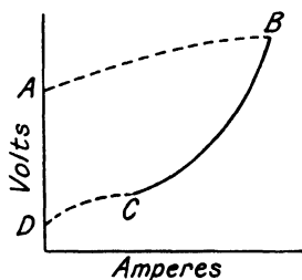
FIG. 191. SHOWING EFFECT OF DIFFERENT SIZES OF PORES ON THE VA. CHARACTERISTIC Line AB represents the different breakdown values of the different sizes of pores. Line BC represents current decreases in all pores. Line CD represents the different cut-off values for the different sizes of pores.
