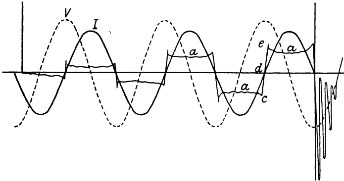
FIG. 91. CHARACTERISTICS OF ARC VOLTAGE CURVE WHICH IS IN PHASE WITH CURRENT CURVE I AND 90° DISPLACED FROM SYSTEM VOLTAGE CURVE V
