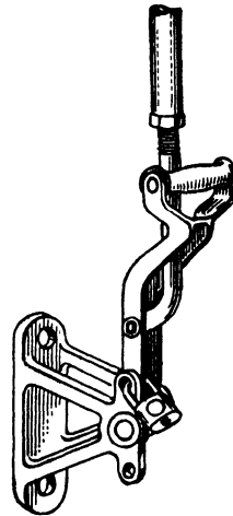
FIG. 80. ISOLATING SWITCH OPERATING HANDLE ARRANGED FOR 180^\circ TRAVEL
