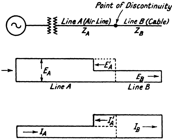
FIG. 180. EFFECT OF TRAVELLING WAVES MEETING A POINT OF DISCONTINUITY Line A is assumed to have a higher surge impedance than line B.
