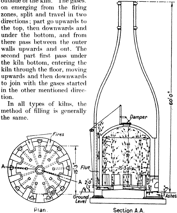
FIG. 30. A ROUND KILN USED FOR FIRING PORCELAINS (Taylor, Tunncliffe, Ltd.)
