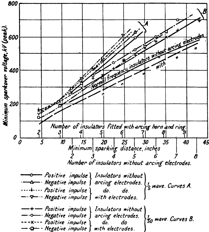
FIG. 206. MINIMUM IMPULSE SPARK-OVER (DRY) AND IMPULSE RATIO OF PORCELAIN CAP AND PIN-TYPE INSULATORS Diameter 10 in., spacing 5 in. (From a paper by Messrs. Allibone, Hawley and Perry)
