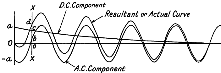
FIG. 110. ANALYSIS OF THE A.C. FUNCTION Ri + L\frac{di}{dt} = \text{SIN}(\omega t + \phi)
