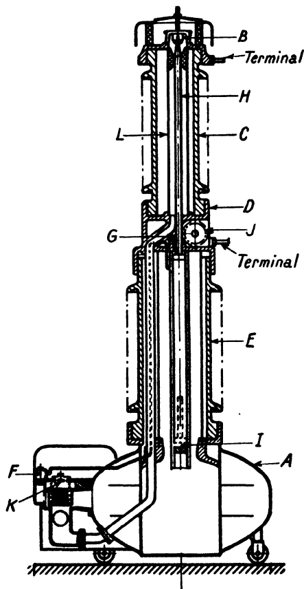
FIG. 256. SECTION OF 100 kV. AIR BLAST CIRCUIT-BREAKER (A.E.G.)
