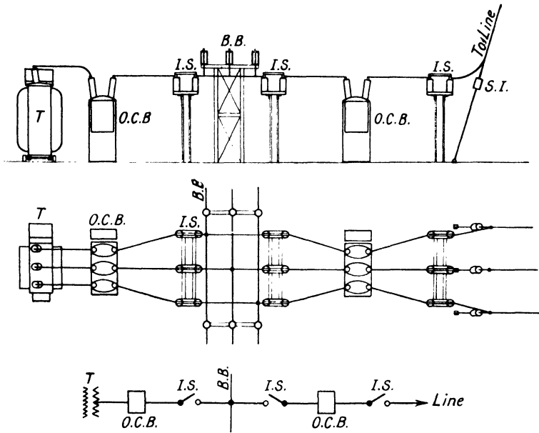
FIG. 16. SINGLE BUS-BAR ARRANGEMENT WITH GANG-OPERATED ISOLATORS
