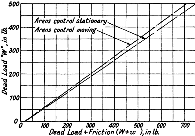
FIG. 143. FRICTION TESTS ON WIRE CONTROLS
