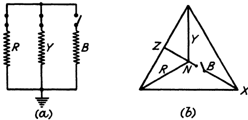
FIG. 109. THREE-PHASE SHORT CIRCUIT TO EARTH (a) Diagram showing blue phase to open first. (b) Vector diagram for above.
