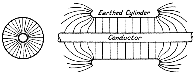
FIG. 156. SHOWING DISTRIBUTION OF FLUX BETWEEN AN ELECTRIFIED CONDUCTOR AND A CONCENTRIC EARTHED CYLINDER
