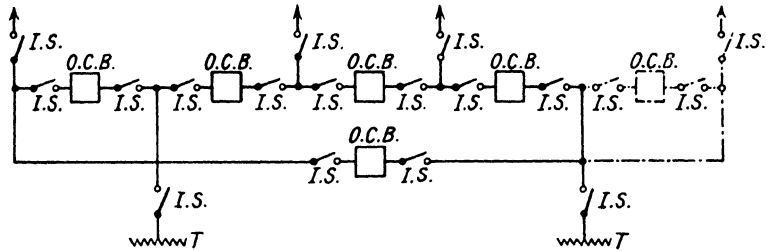
FIG. 7. AN ECONOMICAL ALTERNATIVE TO FIG. 6
