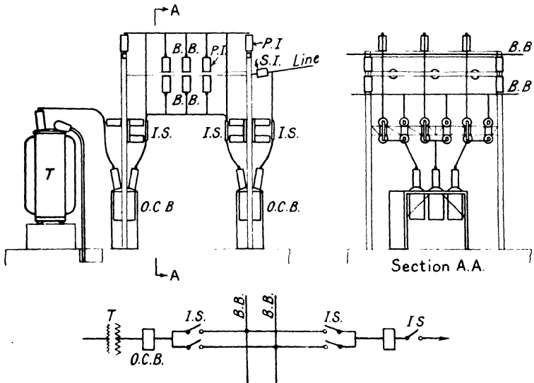
FIG. 12. A SIMILAR ARRANGEMENT TO FIG. 11, BUT ARRANGED WITH DOUBLE BUS-BARS
