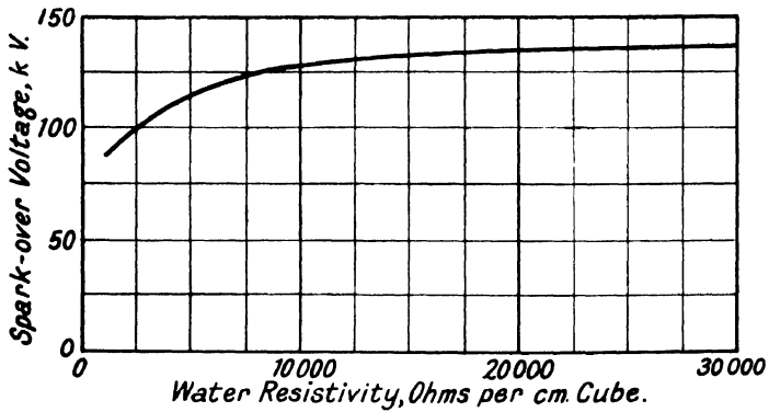
FIG. 43. VARIATION IN SPARK-OVER OF A PARTICULAR INSULATOR WITH VARYING WATER RESISTANCE ("The Testing of Porcelain Insulators," Goodlet, I.E.E. Journal , 1929.)
