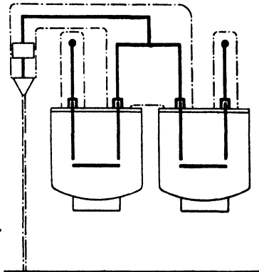
FIG. 242. VERTICAL DROP-DOWN ISOLATION USED FOR METAL-CLAD SWITCHGEAR
