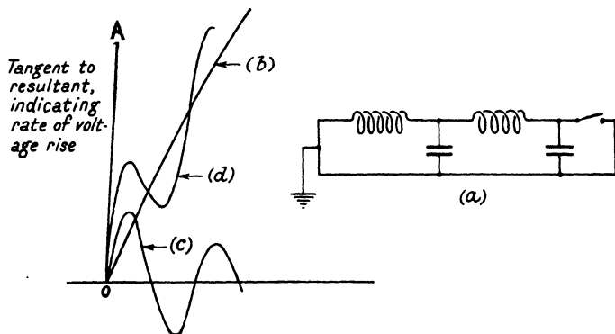
FIG. 112. EFFECT OF DOUBLE FREQUENCY CIRCUIT (a) = Equivalent circuit. (b) = First natural frequency. (c) = Second natural frequency. (d) = Resultant frequency.
