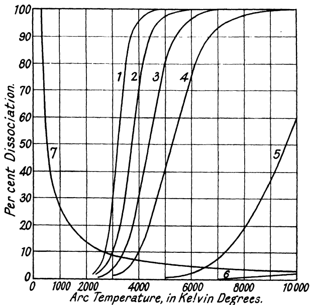
FIG. 99. DEGREE OF DISSOCIATION OF HYDROGEN AS A FUNCTION OF ABSOLUTE TEMPERATURE (From paper by Dr. Kopeliowitsch)
