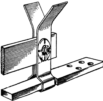
FIG. 75. CHEAP TYPE CONTACT
