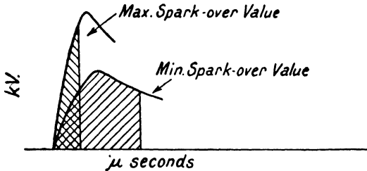
FIG. 185. WAVE SHAPES THAT GIVE MAXIMUM AND MINIMUM SPARK-OVER VALUES
