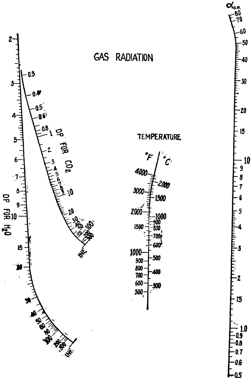
Fig. 35.—Gas Radiation.
