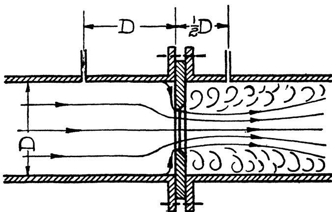
Fig. 23.—Orifice Meter.
