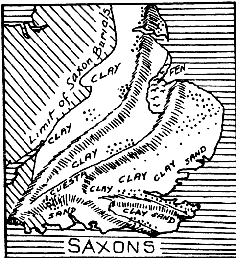
FIG. 65. The control of Saxon settlement by soils. (After S. W. Wooldridge.)
