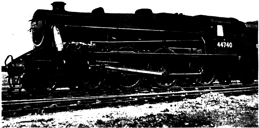
24. Walschaerts valve-motion, as seen on a Southern Region 4-cylinder 4-6-0 of the "Lord Nelson" class. ( Frank F. Moss. )
