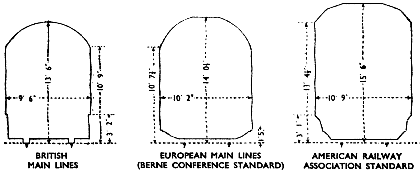
Fig. 1. TYPICAL LOADING GAUGES
