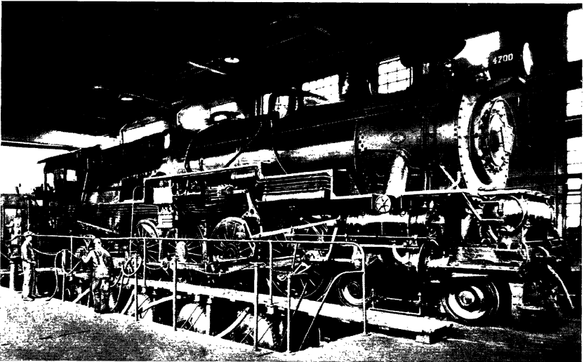
50. Prepared for indicator tests—Western Region 4-cylinder 4-6-0 Caldicot Castle fitted with indicating shelter. (Courtesy, British Railways .)
