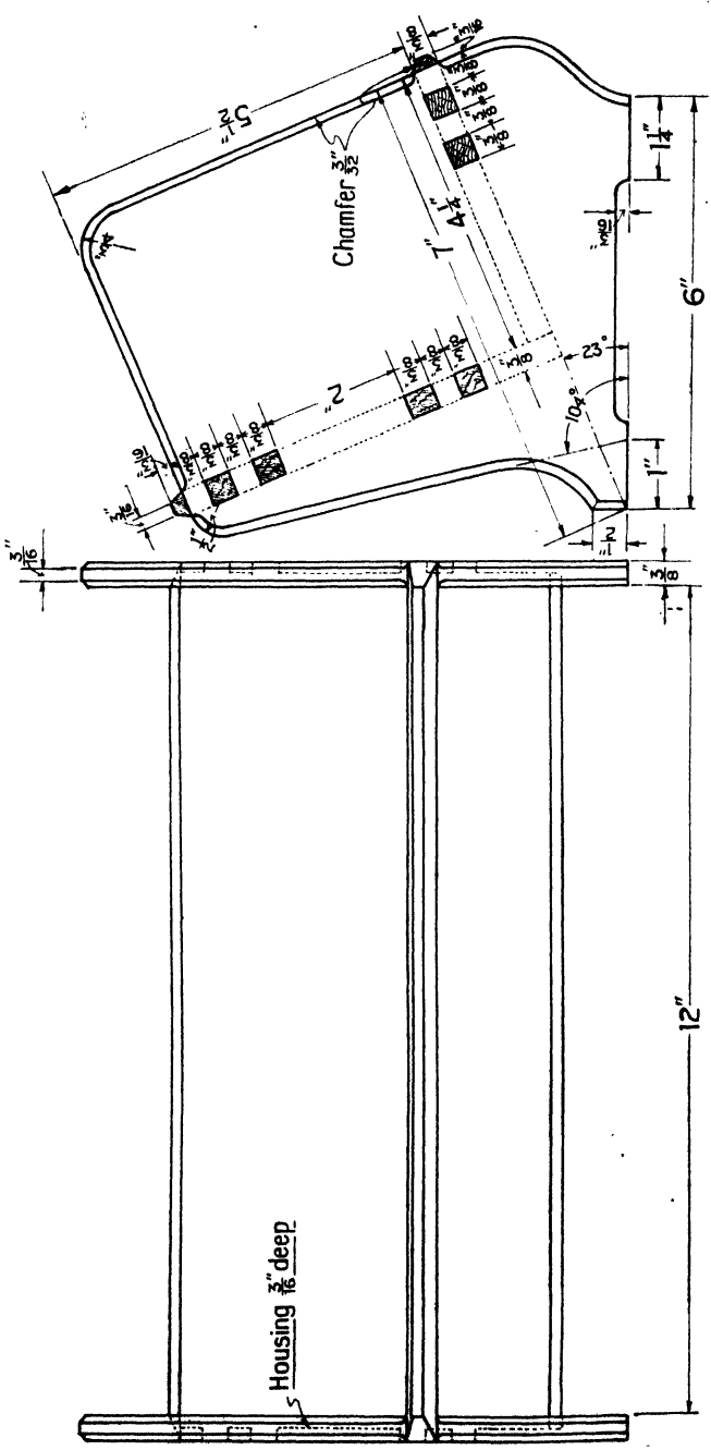
BOOK TROUGH
