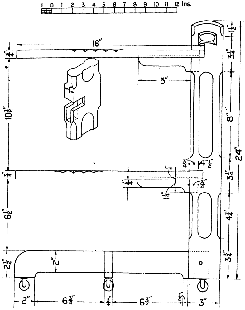
OCCASIONAL TABLE
