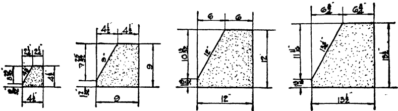
FIG. 403. Sixty-degree skewbacks. Shape 60-4½ is 9-in. thick; the others are 4½-in. thick. (Courtesy of J. S. McDowell and L. L. Gill, "Steel.")
