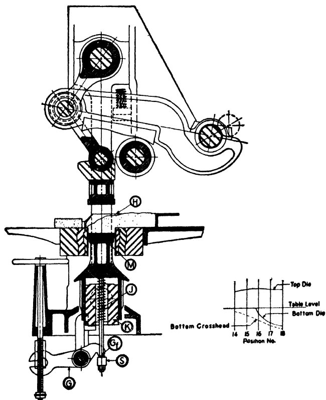
Fig. 74 i . Represents position No. 16. At position No. 16 the crosshead K has continued to move downward taking with it the pressure-adjusting mechanism G until point G 1 comes in contact with saddle bar S and starts to compress saddle springs J . The setting of the pressure-adjusting mechanism decides the length of movement of the lower die M and allows the mold box to be filled to the desired depth. The charger H has further removed the finished brick and has started to fill the mold with loose material.
