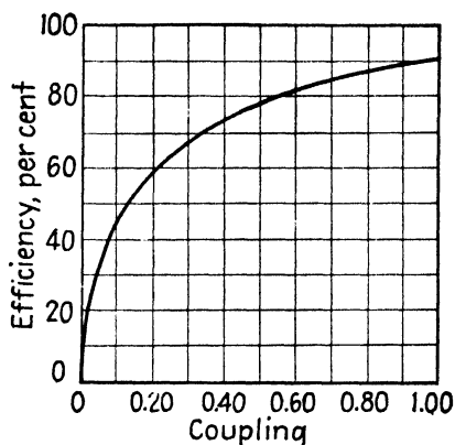
FIG. 155. Effect of coupling on heating efficiency.
