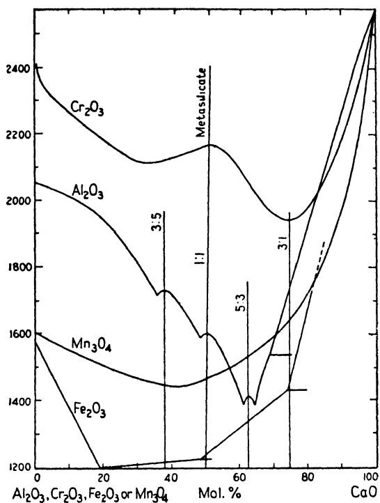
FIG. 206. Liquidus curves of systems CaO-Al 2 O 3 , CaO-Cr 2 O 3 , CaO-Fe 2 O 3 , and CaO-Mn 3 O 4 . H. v. Wartenberg, H. J. Reusch, and E. Saran, Part VII, Z. anorg. u. allgem. Chem. , 230 , 266, 1937.)
