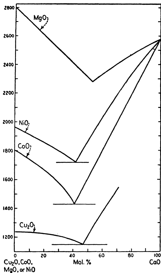
FIG. 205. Liquidus curves of systems Cu 2 O-CaO, CaO-CoO, CaO-MgO, and CaO-NiO. (H. v. Wartenberg, H. J. Reusch, and E. Saran, Part VII, Z. anorg. u. allgem. Chem. , 230 , 265, 1937.)
