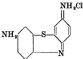
Thionin
