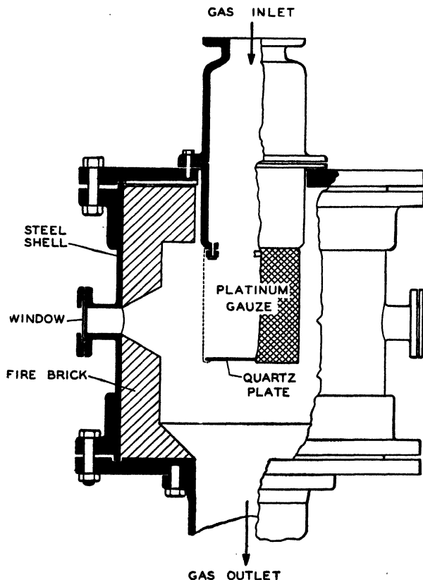
FIG. 28.—Catalyst chamber for ammonia oxidation.
