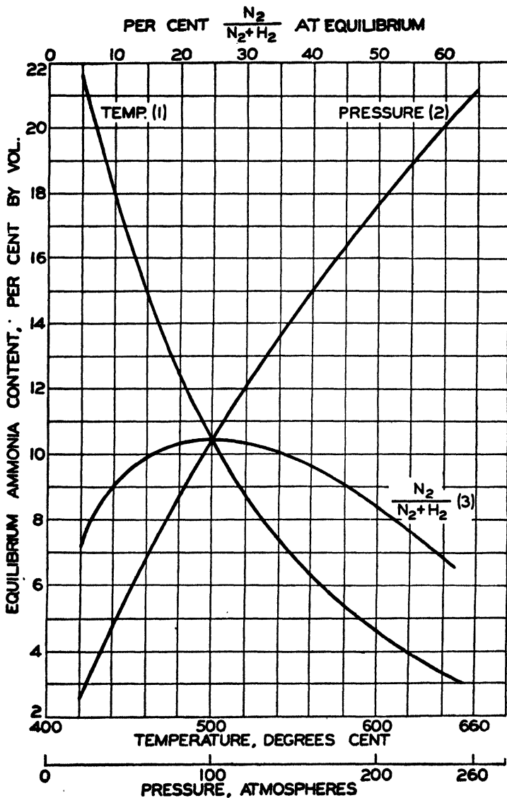
FIG. 25.—Equilibrium between nitrogen, hydrogen, and ammonia.
