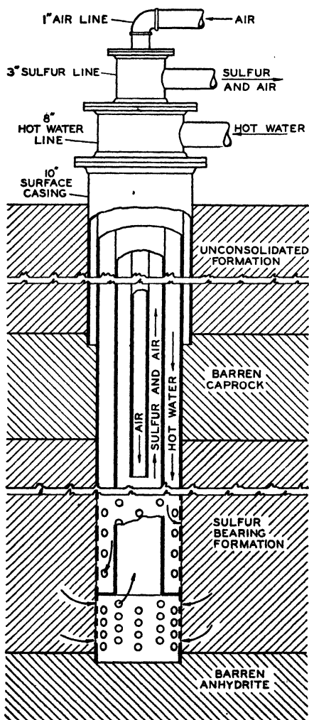
Fig. 11.—Sulfur well.
