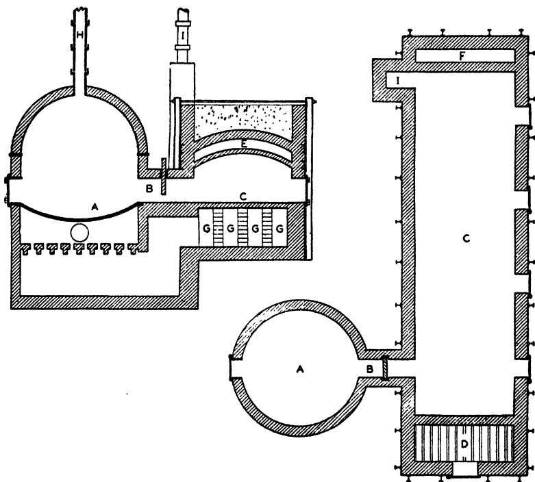
FIG. 30.—Pot-and-muffle furnace for hydrochloric acid.
