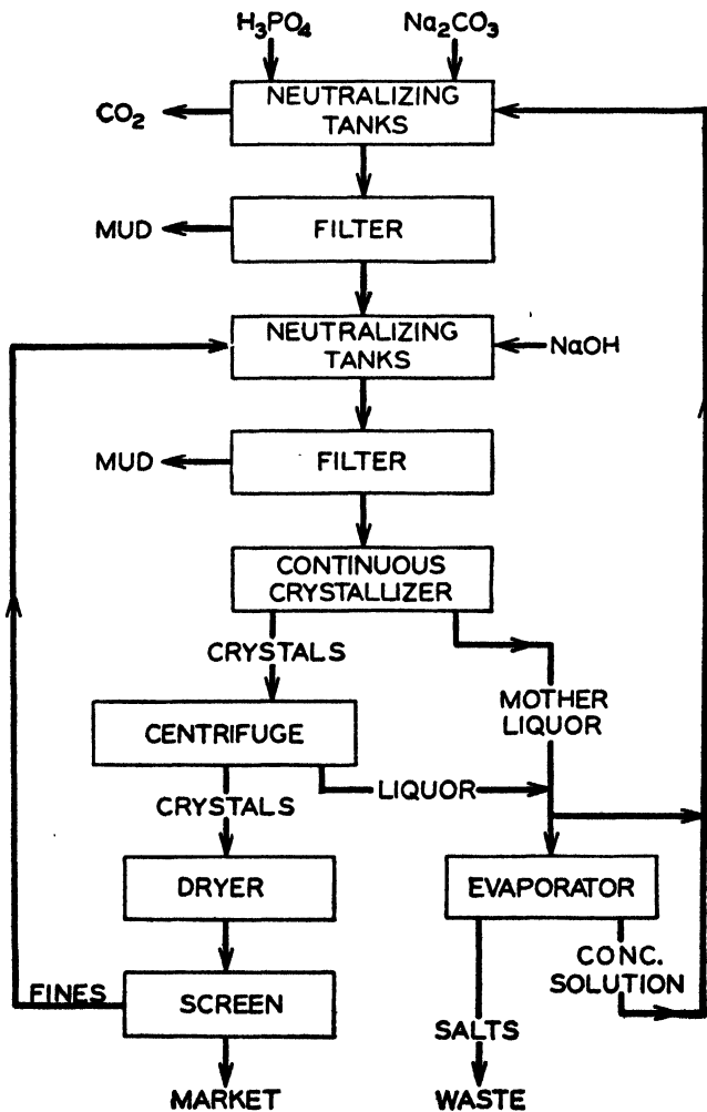
Fig. 52.—Flow sheet of manufacture of trisodium phosphate.
