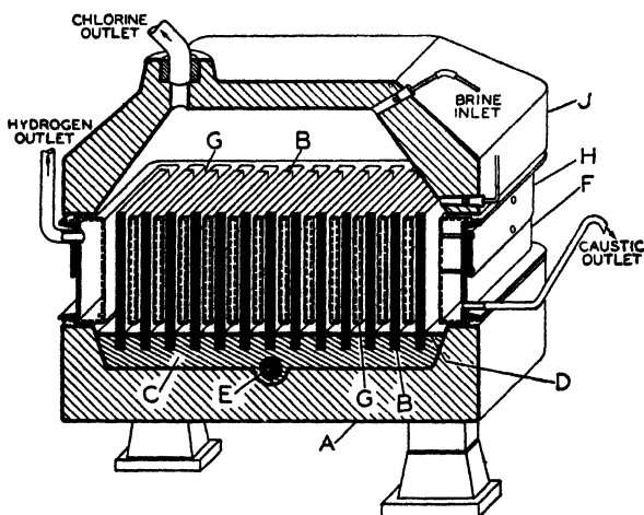
FIG. 45.—Hooker Type-S cell.
