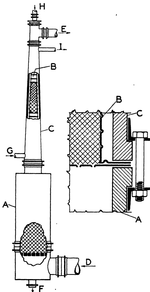
FIG. 36.—Tantalum absorber for hydrochloric acid. (Courtesy of Fansteel Metallurgical Corporation.)
