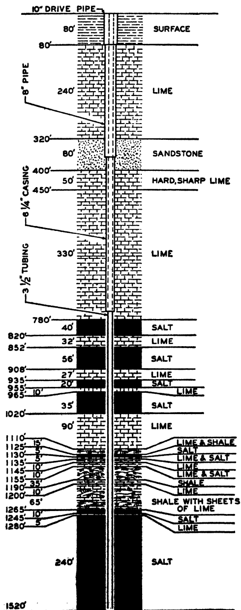
FIG. 2.—Section of salt well.
