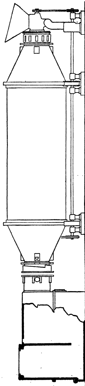
Fig. 13.—Glens Falls sulfur burner.
