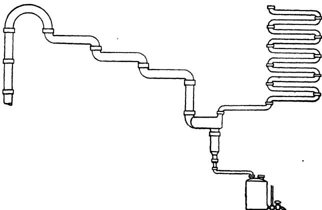
FIG. 23.—Condensing system for nitric-acid vapors.
