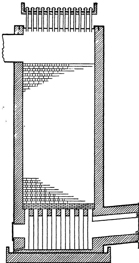
FIG. 15.—Details of chamber-plant construction: Glover tower.
