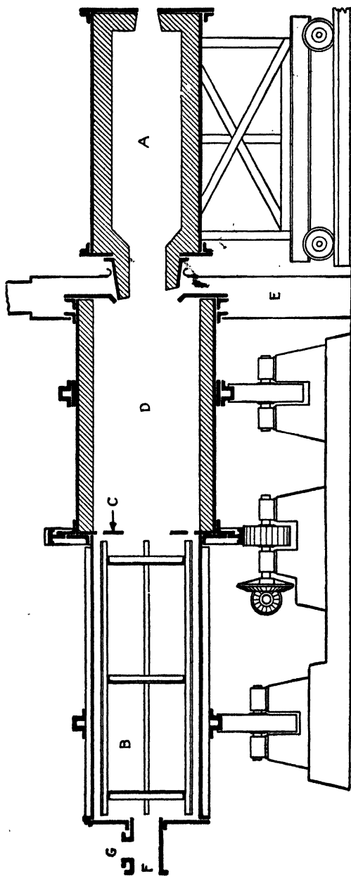
FIG. 32.—Laury furnace.
