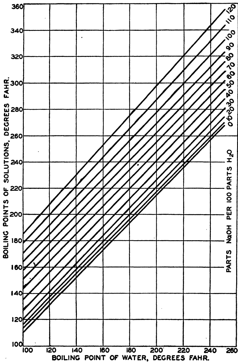
FIG. 47.—Boiling points of electrolytic-caustic solutions.
