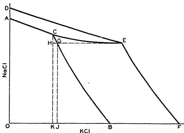
FIG. 54.—Mutual solubilities of sodium chloride and potassium chloride at 110 and 20°C.
