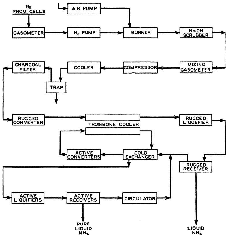
FIG. 24.—Flow sheet of ammonia-synthesis process.
