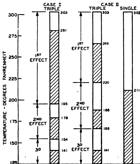
Fig. 48.—Effect of elevation in boiling point on multiple-effect evaporator capacity.
