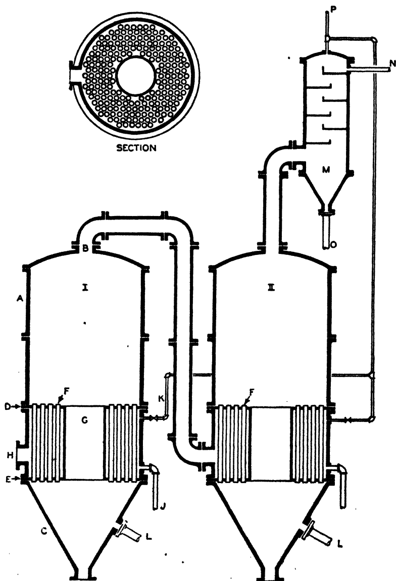
FIG. 6.—Double-effect salt evaporator.
