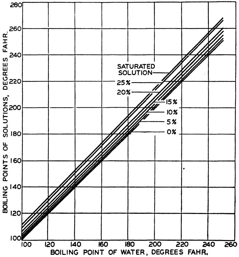
Fig. 58.—Boiling points of salt solutions.
