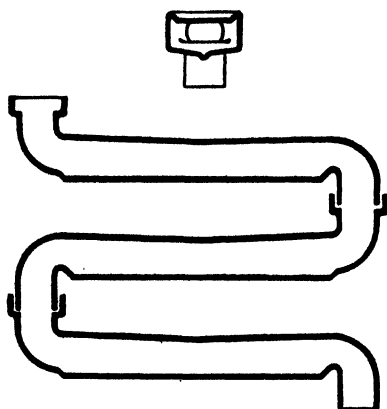
FIG. 35.—Tyler S-bend absorbers.
