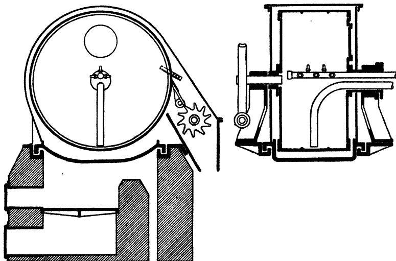
FIG. 50.—Caustic flaker.
