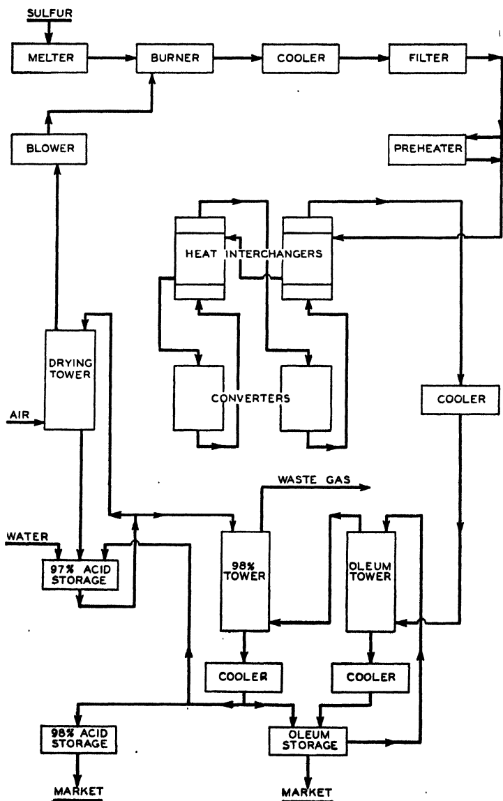
Fig. 20.—Flow sheet of contact process.
