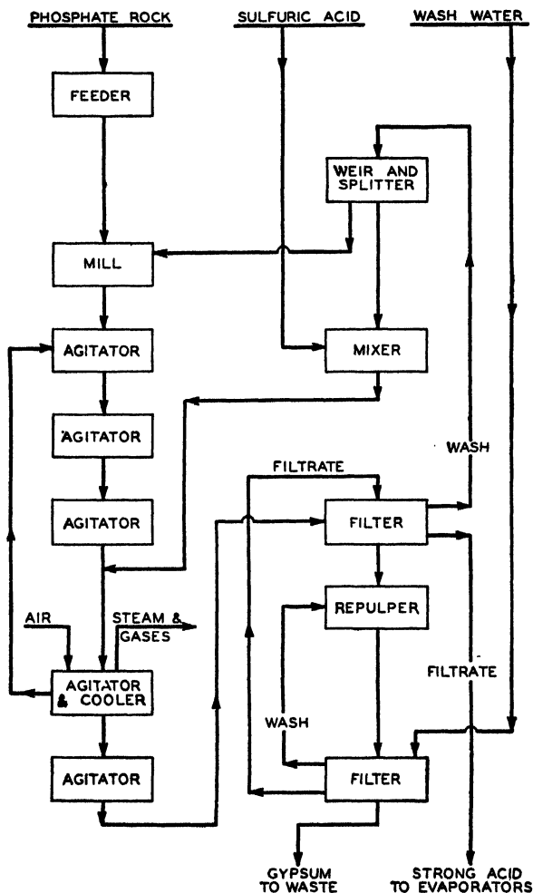
Fig. 37.—Flow sheet for phosphoric-acid manufacture by wet process.
