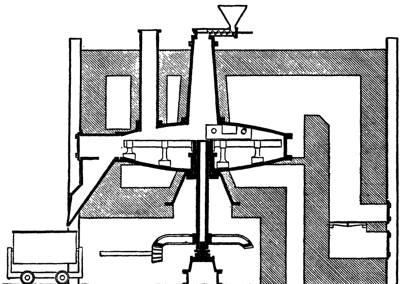
FIG. 31.—Mannheim furnace.
