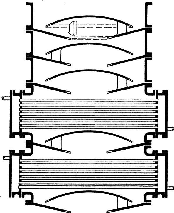
FIG. 40.—Solvay-tower construction.
