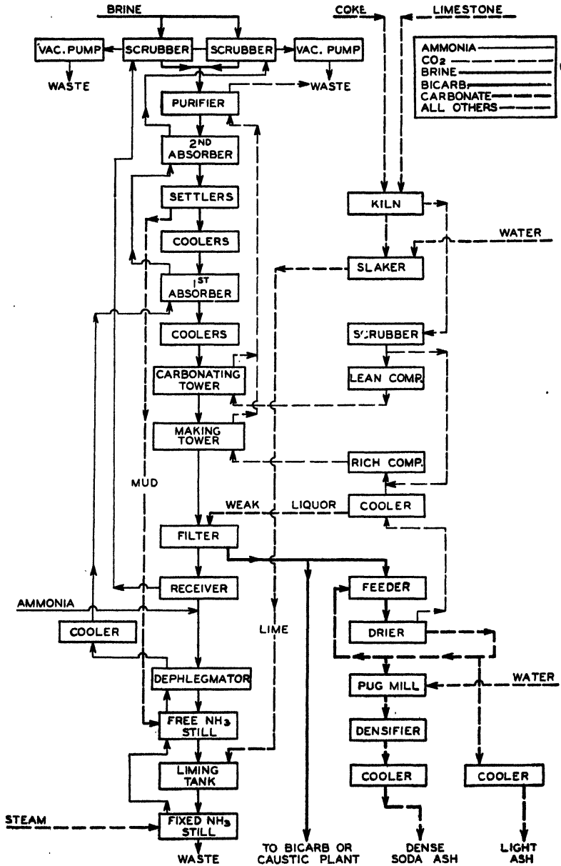
Fig. 39.—Flow sheet of Solvay process.
