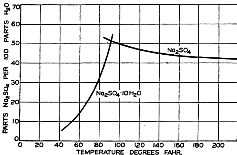
FIG. 51.—Solubility of sodium sulfate.
