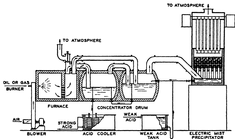
FIG. 19.—Concentrator for sludge acid. (Courtesy Chemical Construction Company.)
