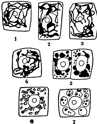
FIG. 130. — Pea root. Vacuolar system. Method of da Fano. 1-4, network strongly impregnated with silver. 5, fusion to uniformly stained vacuoles, which later (6) appear like dictyosomes, then (7) become larger with silver-impregnated precipitates.
