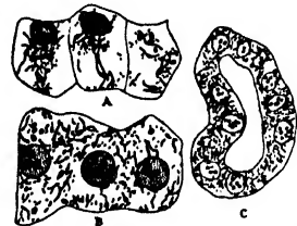
FIG. 21. — The chondriome. A. frog's liver. B. salamander's liver. C. frog's kidney. Regaud's method.
