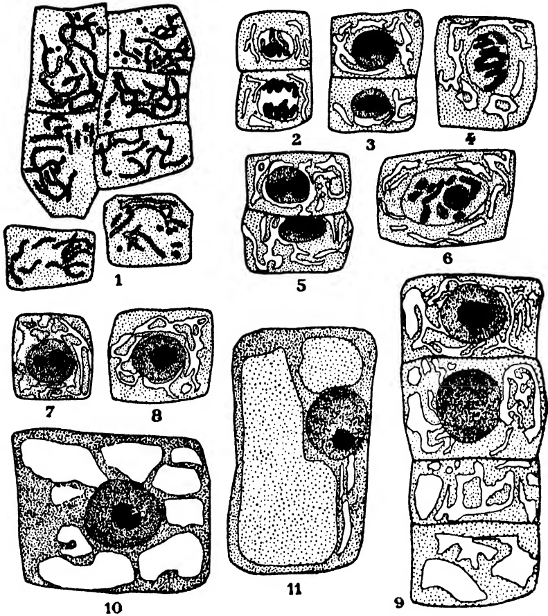
FIG. 129. — Barley root. 1, meristem vitally stained with neutral red; vacuolar system deeply stained, more or less reticulate. 2-11 Benschley's method; 2-9, meristem; vacuolar system has the appearance of Holmgren's apparatus. 10, 11, differentiating cells; Holmgren's apparatus transformed into large vacuoles.
