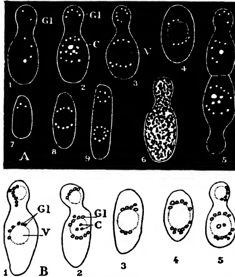
FIG. 110. — Saccharomyces . (A), under the ultramicroscope; (B), with direct light. A, 1-6 S. Ludwigii . Vacuoles (V) usually invisible; position marked by strongly lighted lipide granules (G1; A3, B5) surrounding them and corpuscles of metachromatin (C; A2, B2) which they contain. 4, contour of vacuole visible. 6, cytoplasm coagulated. 7-9, S. pastorianus . B, S. Ludwigii .
