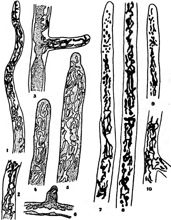
FIG. 132. — Saprolegnia . Vacuolar system. 1-3, vitally stained with neutral red; reticulate, tending to fuse into a vacuolar canal. 4-6, Bunsen's method; system appears as canaliculi of Holmgren. 7, 8, da Fano's silver impregnation method; system impregnated with silver, resembles Golgi's network. 9, 10, Kolatchev's osmic impregnation method; system strongly blackened.
