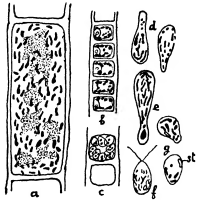
FIG. 103. — a , Cladophora ; vital staining of large central and small peripheral vacuoles. b , c , Ulothrix pseudo-flocca ; arrangement of vacuoles in b vegetative cells and in c zoosporangium. d , e , Cladophora ; zoospores which have ceased swarming. f , Bryopsis plumosa ; zoospore. g , Ulva Lactuca ; zoospore which has just come to rest. st , stigma. (After DAN-GEARD).
