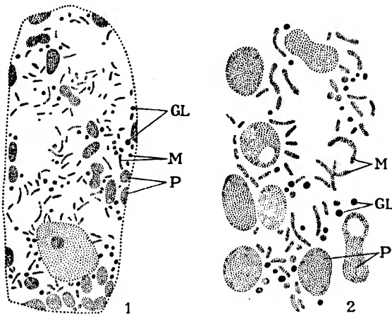
FIG. 140. — Elodea canadensis . 1, Cell from the leaf fixed with Meves' method, stained with acid fuchsin, which colors the chloroplasts (P) and chondriosomes (M) red; lipide granules (GL) colored dark brown by the osmic acid. 2, detail; some chloroplasts are dividing.
