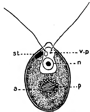
FIG. 11. — Motile cell of Chlamydomonas surrounded by a cell wall which forms a beak between the flagella at the anterior pole. Stippled region shows chloroplast. st , stigma. p , pyrenoid surrounded by a , starch. n , nucleus. v.p. , pulsating vacuole whose rôle is imperfectly known. ( \times 1650 ).
