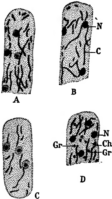
FIG. 141. — Endomyces Magnusii . A-C, Regaud's method; D, Meves' method; stained with haematoxylin. C, Ch, chondrioconts; Gr, lipide granules, brown with osmium; N, nucleus, sufficiently destained in A and C to show structure.
