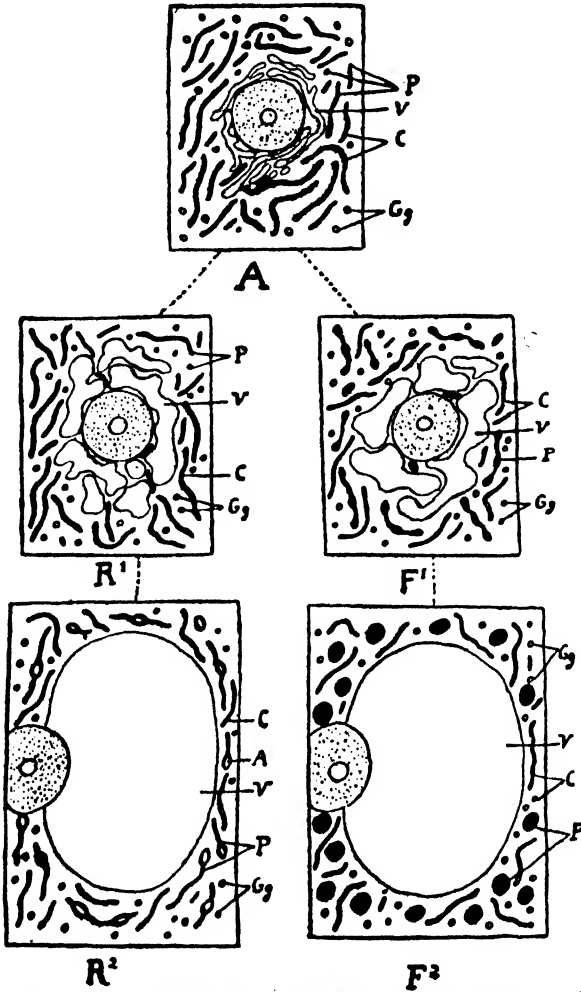
FIG. 151. — Diagrammatic representation of the structure of phanerogam cells during development, based upon the author's investigations. A , embryonic cells; colorless plastids ( P ) shaped like filaments, rods, and granules, indistinguishable from the genuine chondriosomes ( C ); chondriosome-shaped vacuoles ( V ) looking like canaliculi of Holmgren; G g , lipide granules (microsomes of other authors) which do not stain with mitochondrial techniques. R 1 , cell at the beginning of differentiation in root; vacuoles enlarging and coalescing; plastids and chondriosomes unchanged. R 2 , mature cell of root; a single large vacuole; plastids show vesicles with starch ( A ) which mitochondrial techniques do not stain. F 1 , cell of leaf primordium; vacuoles enlarging and coalescing; plastids form swellings which increase in size, separate and become chloroplasts. F 2 , mature cell of leaf; a single vacuole; large chloroplasts easily distinguishable from the chondriosomes.
