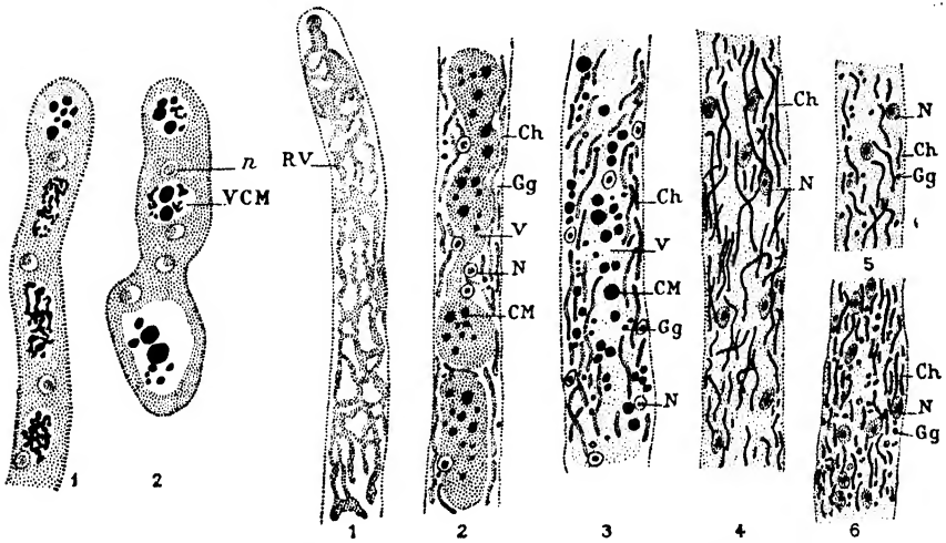
FIG. 107 (left). — Dematium . Bouin's method, stained with hemalum. 1, filament. 2, germinating conidium. VCM, vacuole containing metachromatin precipitates. n, nucleus. FIG. 108 (right). — Saprolegnia . Chondriome and vacuolar system. 1-3, Vital staining with neutral red. 1, tip of filament; reticular vacuole (RV); other elements omitted. 2, older filament; tendency of network to become a diffusely stained canal (V) containing deeply stained bodies (CM), other elements visible but unstained. 3, still older filament; vacuolar canal (V) loses its stain, other bodies as in (2). 4, mature filaments. Regaud's method with iron haematoxylin; vacuolar canal unstained, lipide granules dissolved, chondriosomes (Ch) strongly stained. 5, 6, mature filament. Meves' method with acid fuchsin; chondriosomes (Ch) red, lipide granules (Gg) brown. Ch, chondriosomes. N, nucleus.
