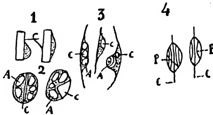
FIG. 15. — Inclusions of the plastids. 1, chloroplasts in epidermal cells of Hedera leaves. 2, chloroplasts in palisade parenchyma of leaves of Achyranthes Verschaffeltii . 3, leucoplasts in young buds of Canna Warszewiczii . 4, chromoplasts in the flower of Neottia Nidus-avis . A, starch; C, protein crystalloids. C, carotinoid crystal; P, protein crystalloid. (After SCHIMPER).
