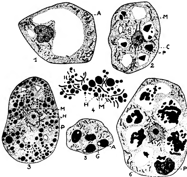
FIG. 118. — Ricinus . Endosperm. 1, young cell, starch (A) forms in chondriocysts. 2, just before maturation; starch is absorbed, the large vacuole is fragmented into small vacuoles containing protein crystals (C) and protein precipitates (P). 3, oil globules (H) blackened by osmic acid, protein crystals (P). 4, detail of (3). 5, dormant seed; A, aleurone grain, G, globoid. 6, during germination of the seed; aleurone grains (P) beginning to dissolve. M, chondriosomes. 1, 2, 5, 6, Regaud's method. 3, 4, Meves' method.
