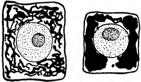
FIG. 138. — Vicia Faba . Golgi apparatus (vacuolar system) in meristem cells of the root. Osmic impregnation. (After Miss SCOTT).
