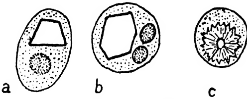
FIG. 117. — Aleurone grains in seeds. a, b, Ricinus ; one crystalloid and 1-2 globoids. c, Oenanthe Phelandrium ; sphaerocrystal of calcium oxalate in protein ground substance.
