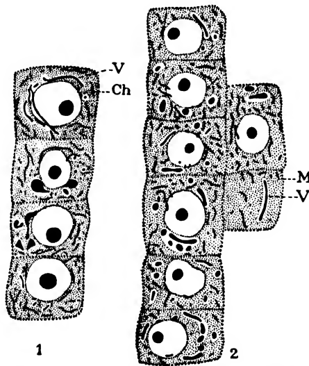
FIG. 105. — Ricinus root. Meristem fixed by Regaud's method. Black, filamentous or granular chondriosomes ( Ch ) and vacuoles ( V ), the latter distinguished by an external hyaline region due to a contraction of their colloidal contents during fixation.
