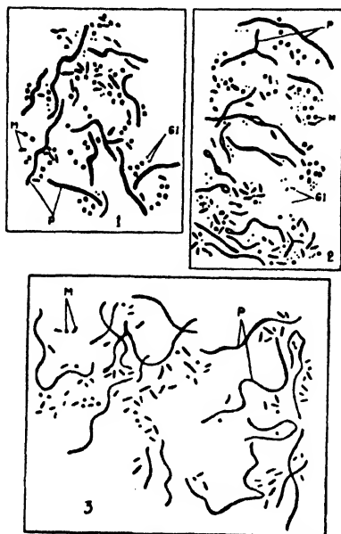
FIG. 143. — Iris germanica . Chondriosomes ( M ) and plastids ( P ) in the form of chondrioconts in epidermal cells of the leaf. 1, living material. 2, Meves' method with acid fuchsin. 3, Regaud's method. Lipide granules ( Gl ) very refractive in 1, blackened by osmium in 2, not preserved in 3.
