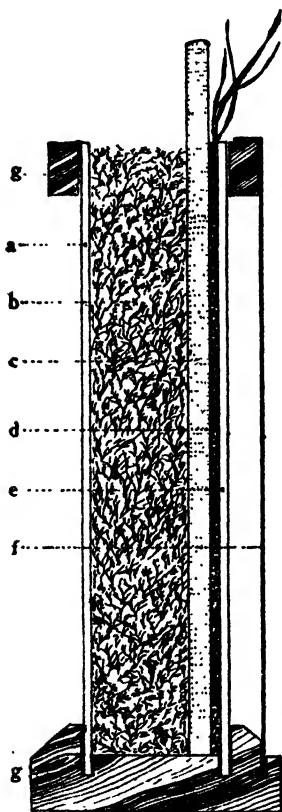
FIG. 296.—A sectional view of a root cage.
