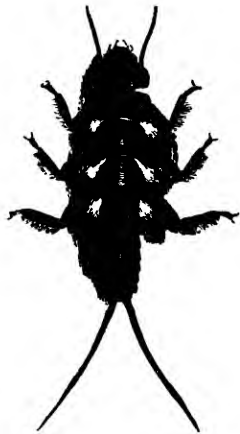
FIG. 116.—Nymph of stone-fly.
