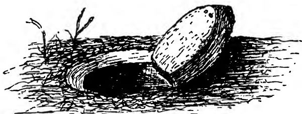
FIG. 200.—Entrance to nest of a trap-door spider.
