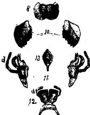
FIG. 5.—The mouth-parts of a locust: 8, labrum; 10, mandibles; 11, maxilla; 11 d, maxillary palpi; 12, labium; 12 d, labial palpi; 13, hypopharynx.
