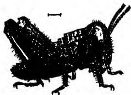
FIG. 11.—Nymph of Melanoplus , first stage. (After Emerton.)
