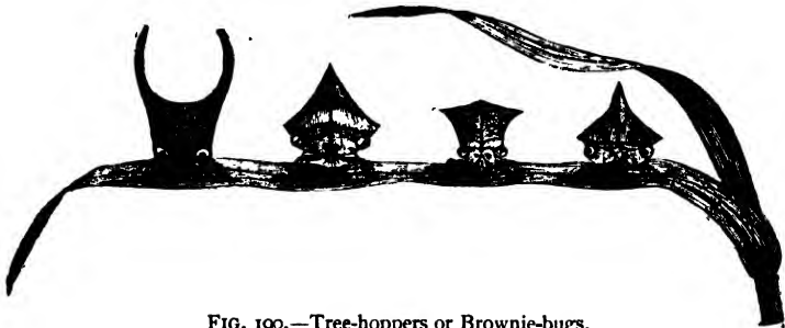
FIG. 190.—Tree-hoppers or Brownie-bugs.
