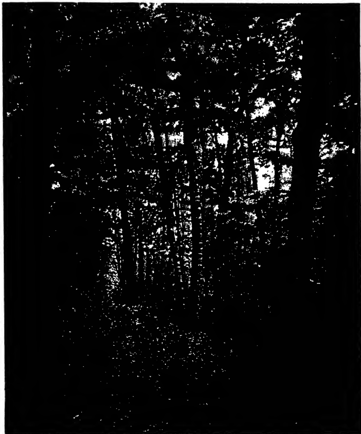
A FOREST AISLE.
