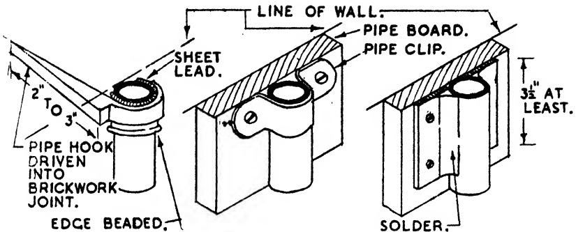
PIPE HOOK FIXING DIRECT TO WALL.
