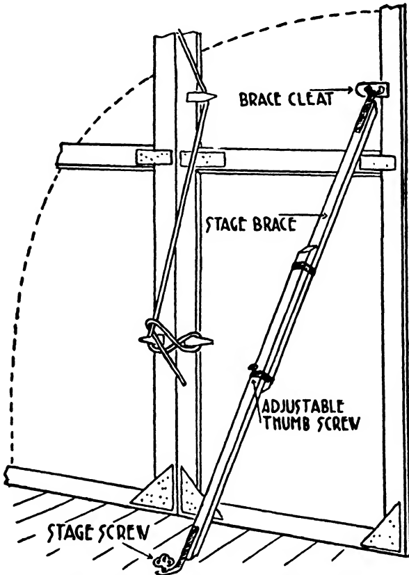
METHOD OF BRACING FLATS
