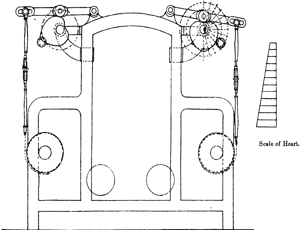
ELEVATION PASS END SHOWING HEART MOTION ARRANGEMENT FOR TRAVERSE OF BOBBIN.
