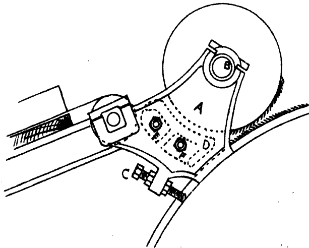
End Elevation.
