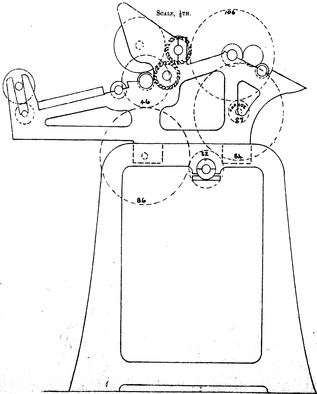
ARRANGEMENT OF DRAFT GEARING.
