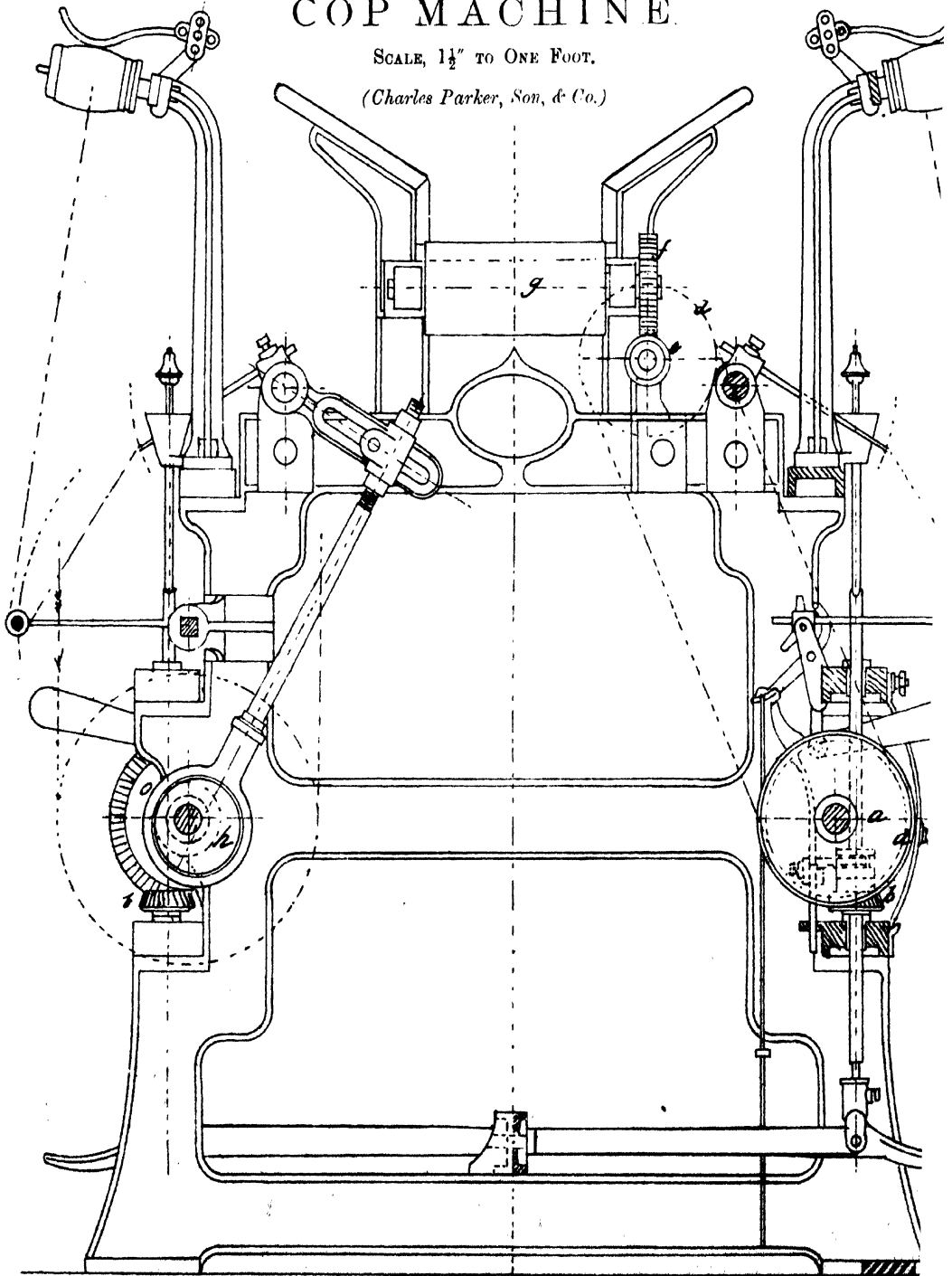
HALF SECTIONAL ELEVATION
