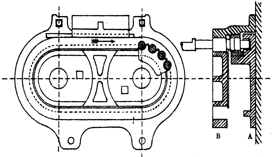
Sectional Elevation.
