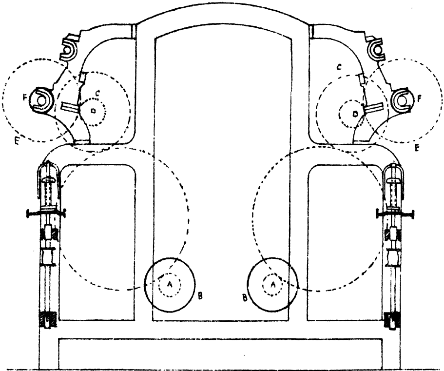
ELEVATION DRIVING END SHOWING TWIST GEARING.*
