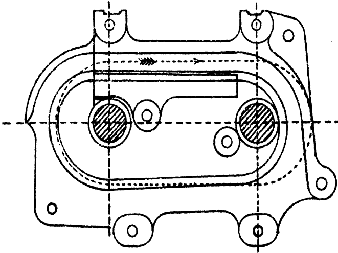
Elevation of Guide Plate "A" for pins on gill bar cranks.
