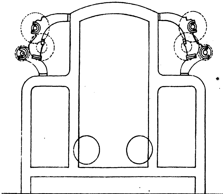
ELEVATION PASS END SHOWING GRIST GEARING.
