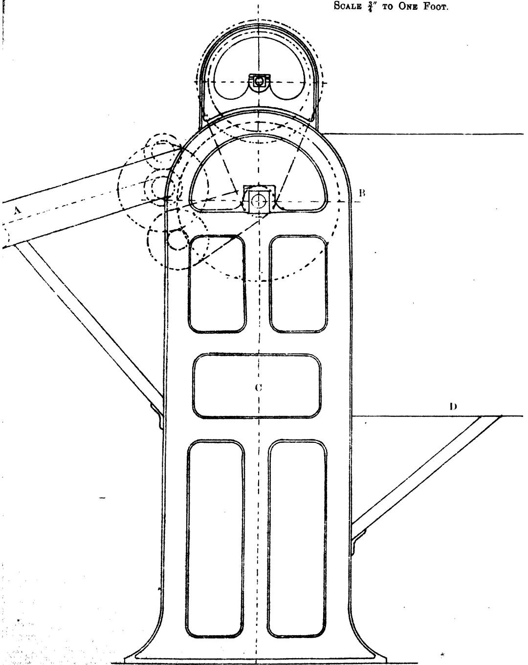
End Elevation.
