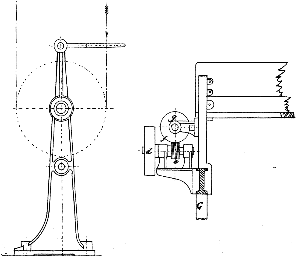
SIDE VIEW OF OUTER CARRIER B.
