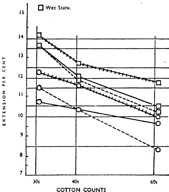
FIGURE 18 EXTENSION-AT-BREAK OF YARNS SPUN FROM— ○——○ Standard "Fibro" 1½" Staple 1.5 Denier Dry State. ○- - - -○ Strong "Fibro" " " " " " " ○- - - -○ Strong "Fibro" 1½" " " 1.25 " " " " RING SPUN YARNS
