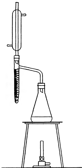
FIG. 23. Dean and Stark distilling apparatus.
