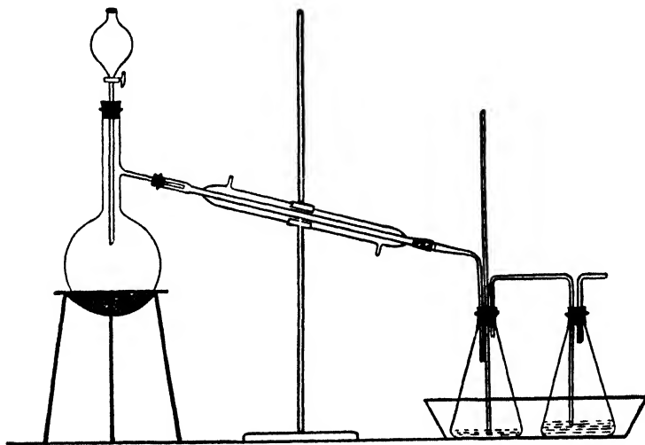
FIG. 21. Arsenic distillation apparatus.
