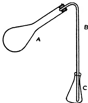
FIG. 25. Bromate distillation apparatus.
