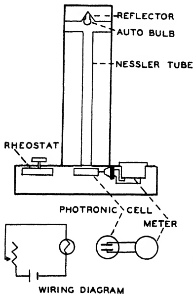
Fig. 27. Diagram of the Frear-Haley photoelectric colorimeter.
