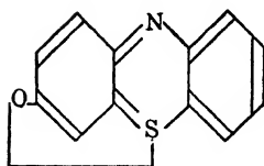
Phenothiazone (a)
