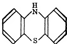
Phenothiazine
