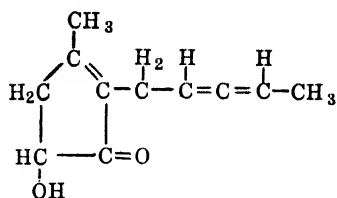
Pyrethrolone (A) *
