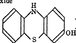
Leuco-phenothiazone
