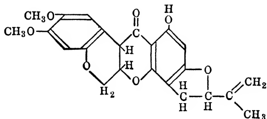
Sumatrol
