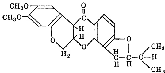
Dihydrorotenone
