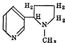
\beta -nicotine
