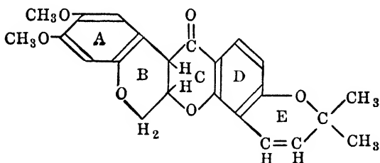
Deguelin
