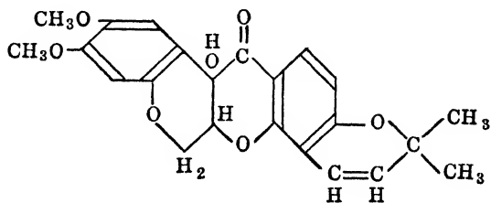
Tephrosin
