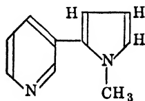
Nicotyryne
