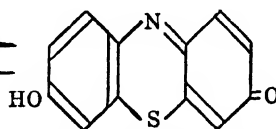
Hydroxyphenothiazone
