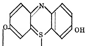
Thionol
