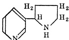
\beta - nornicotine
