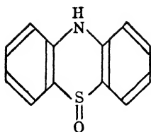
Phenothiazine Sulfoxide
