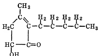
Tetrahydropyrethron (B) *
