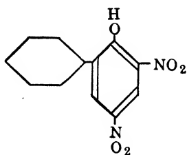
2,4-dinitro-6-cyclohexylphenol
