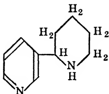
Anabesine (Neonicotine)
