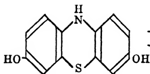
Leuco-hydroxy- phenothiazone
