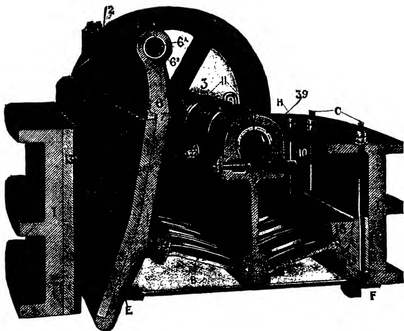
FIG. 20.—Blake Crusher.
