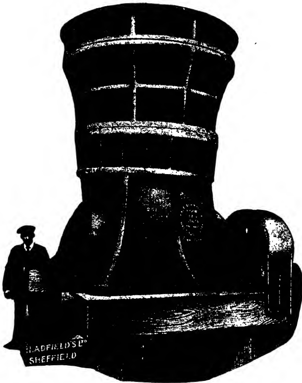
FIG. 21.—Gyratory Crusher.
