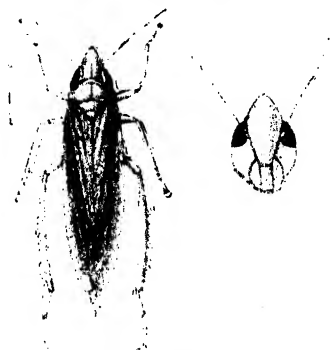
Fig. 36.— Campbellinella illustrata .
