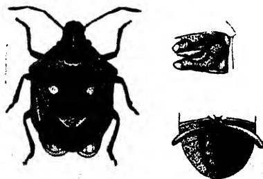
Fig. 69.— Bainbriggeanus fletcheri .
