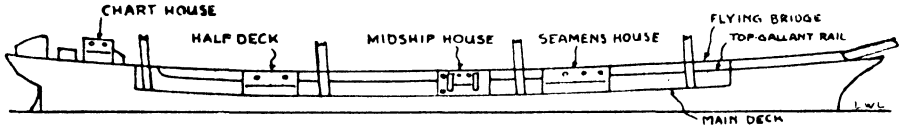
Fig. 30. Diagram of deckhouses
