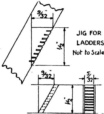
Fig. 48. Companion ladders
