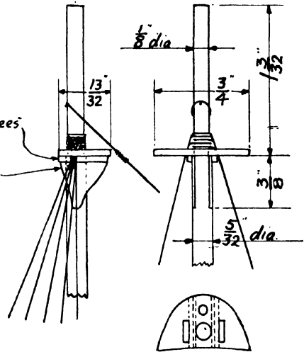
Fig. 58. Top for mizzen main and foremasts
