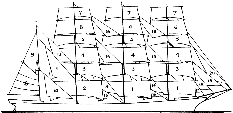
Fig. 76. Diagram of sails
