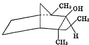
"Exo" structure
