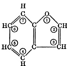
Coumarone
