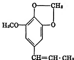
Isomyristicin
