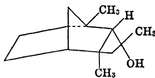
"Endo" structure
