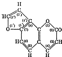
Angelicin (angular type)
