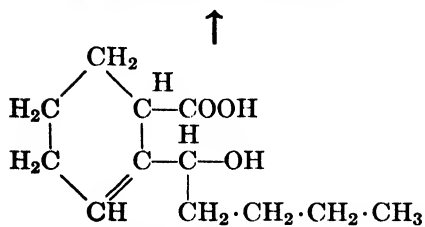
Sedanolic Acid C 12 H 20 O 3 1- \alpha -Hydroxy amyl- \Delta^2 -tetrahydrobenzoic acid
