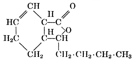
"Cnidium Lactone"
