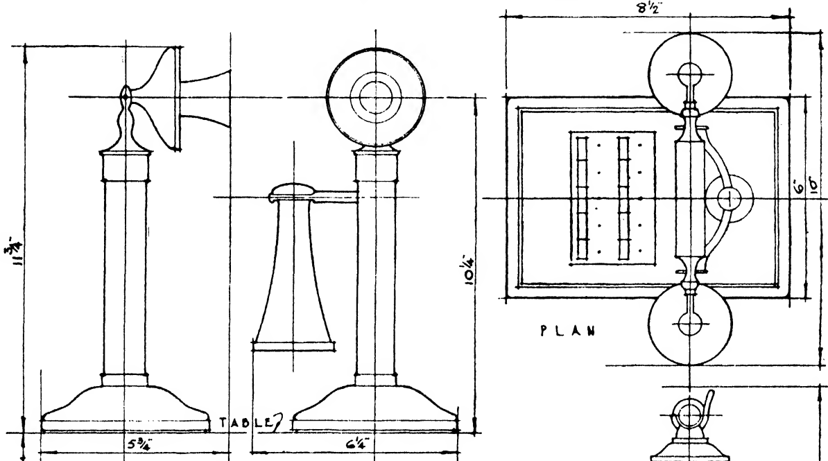
PEDESTAL PATTERN TABLE TELEPHONE. STANDING WALL PATTERN MOUTHPIECE TO FLOOR 5 0"
