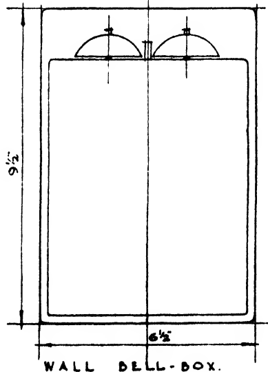
WALL BELL-BOX.
