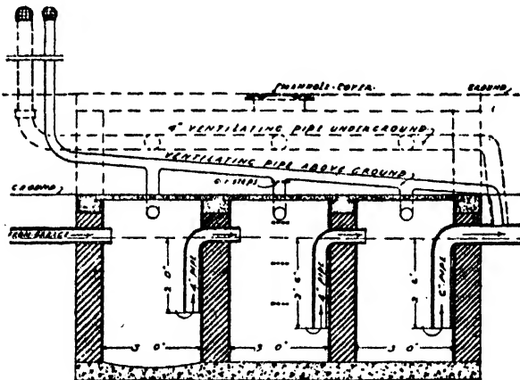
Section of Intercepting Tank.
