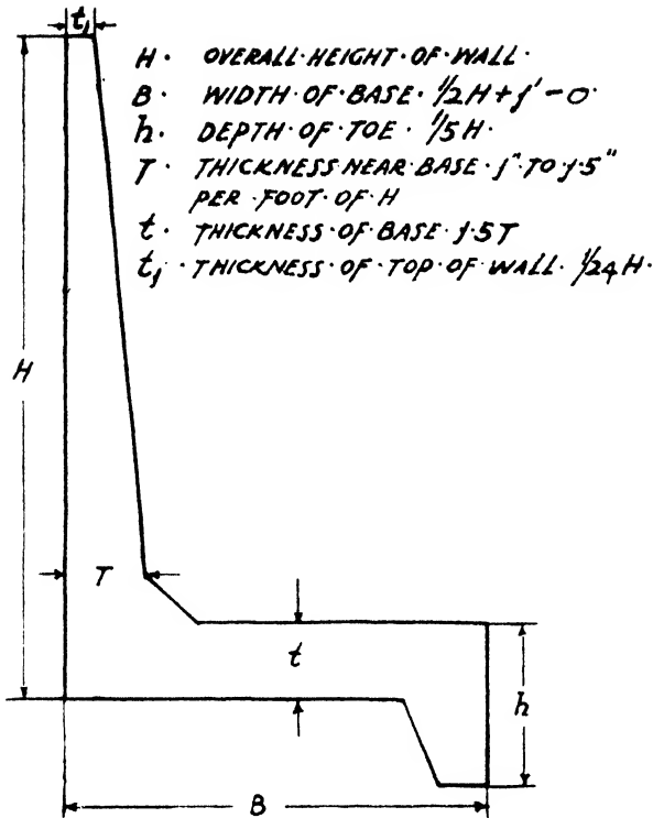
TYPICAL SECTION R.C. RETAINING WALL.
