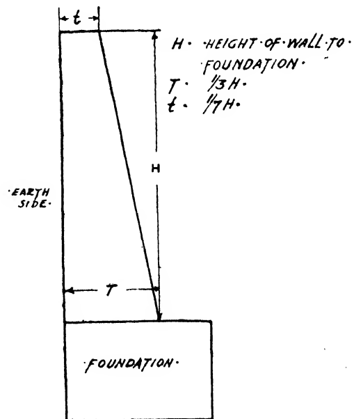
TYPICAL GRAVITY SECTION RETAINING WALL
