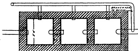
Plan of Intercepting Tank.
