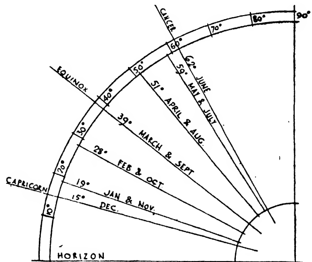
Fig. 2. Sun altitudes for London on N.S. aspect.
