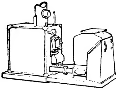
THE BABY ROBOT STOKER attached to a domestic Boiler
