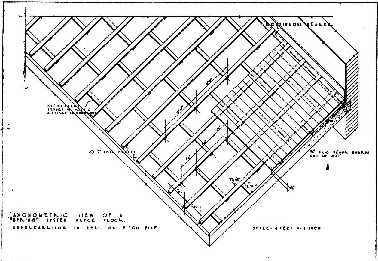
The above diagram shows a type of floor often used for dancing where a true spring floor would be too costly.
