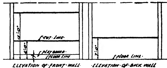
ELEVATION OF FRONT WALL · ELEVATION OF BACK WALL
