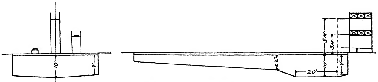
Sections of narrow bath with 5-metre diving board.
