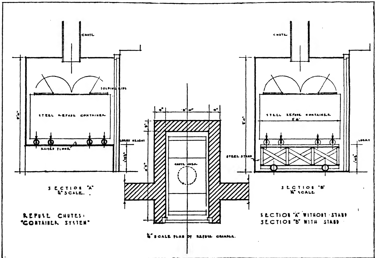
Details of Dust Chutes
