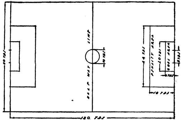
ASSOCIATION FOOTBALL GROUND
