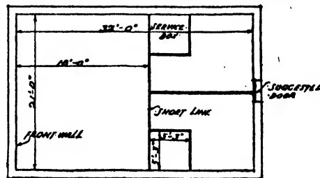
· PLAN OF SQUASH RACKETS COURT ·
