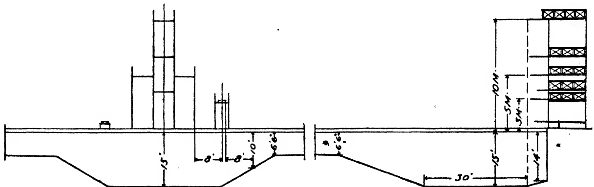
Sections of wide bath with 10-metre diving board.
