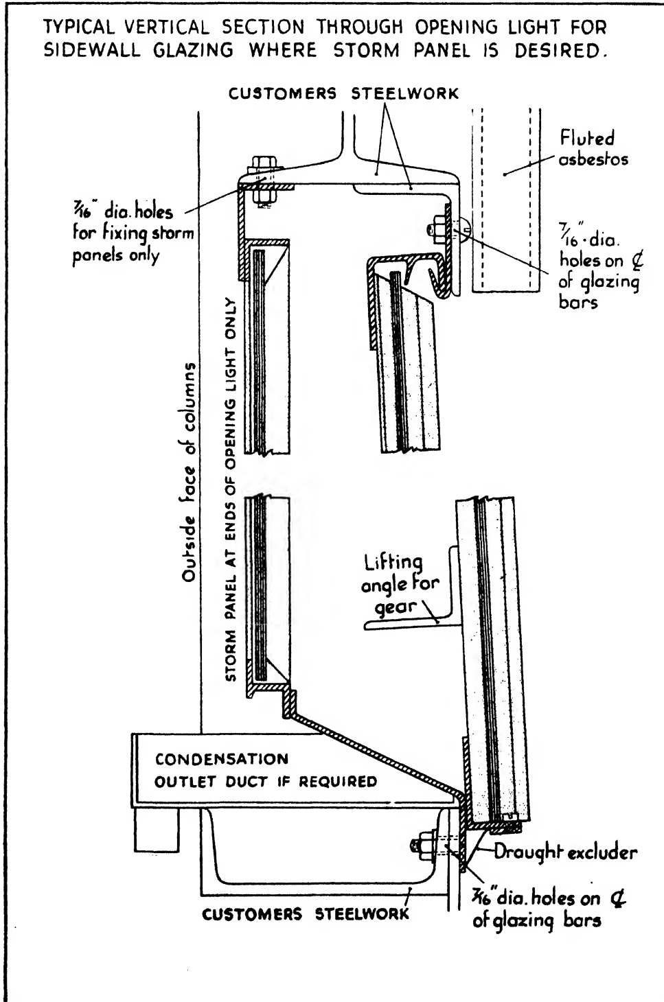
Typical section of OPENING LIGHT for SIDEWALL GLAZING
