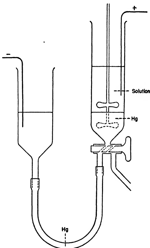
FIG. 14. Apparatus for Electrodeposition with Mercury Cathode.
