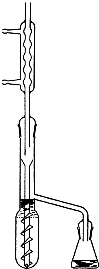
FIG. 13. Continuous Extractor.
