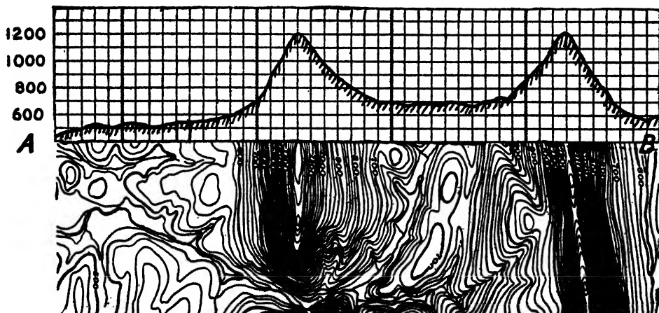
Fig. 98 Construction of profile along the line A-B.
