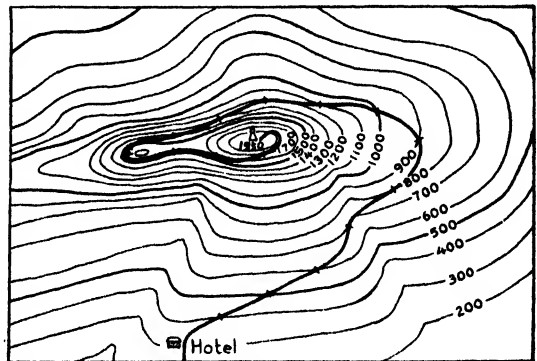
Scale 0 \frac{1}{4} \frac{1}{2} 1 Mile Gradient of road 400' per mile Fig. 100 The layout of a motor road of even grade. Several alternatives are possible.
