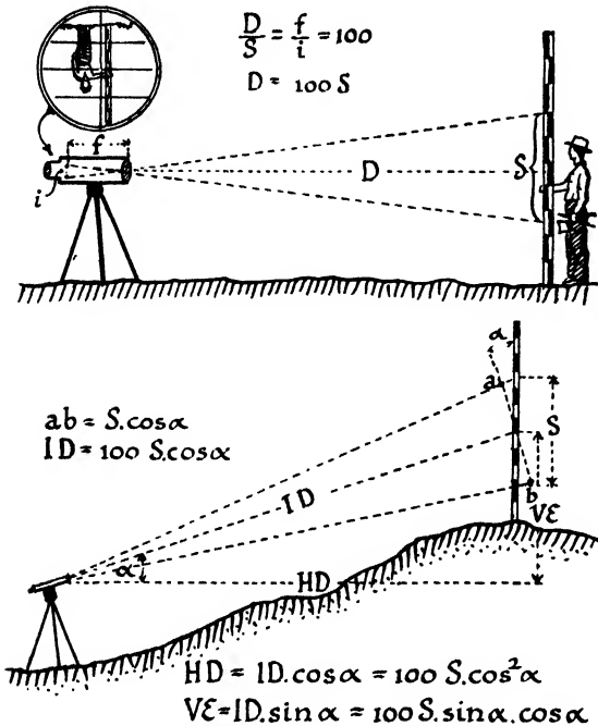
Fig. 145 In the stadia method distances are observed by reading the length of the part of the rod's image that appears between the cross hairs.
