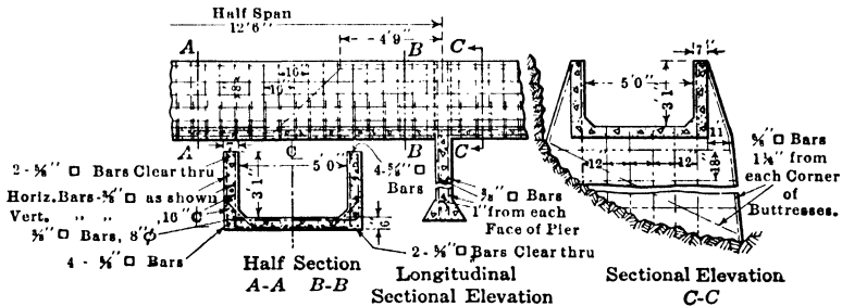
FIG. 45.—Reinforced concrete elevated flume. Yakima Valley Canal, Wash.
