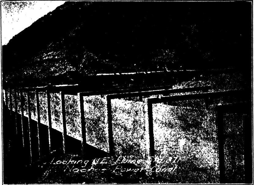
FIG. A.—Reinforced concrete flume. Naches Power Canal, Wash.
