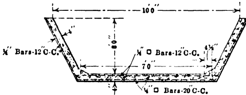
FIG. 23.—Reinforced concrete lining. Yakima Valley Canal, Wash.
