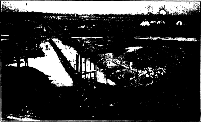
FIG. A.—Clay Creek Siphon during construction. American Sugar Beet Co., Colo.
