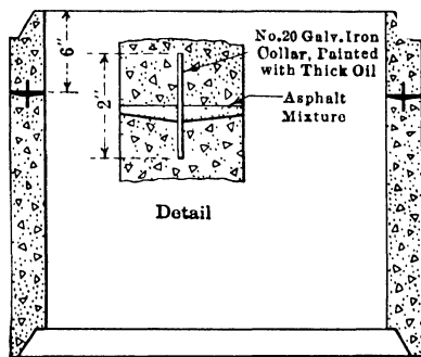
FIG. 70.—Contraction joint for hand-tamped cement pipe.
