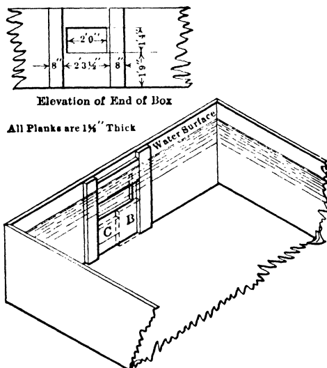
FIG. 10.—Isometric sketch of box. Forms of free discharge gate opening, to accompany results given by Unwin.
