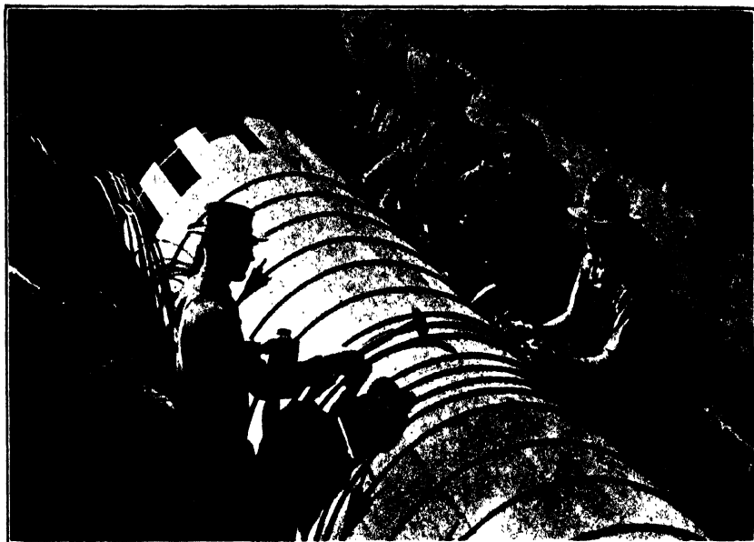
FIG. C.—Constructing a 45½-inch continuous wood stave pipe. Whittier, Calif. Pacific Tank & Pipe Co.
