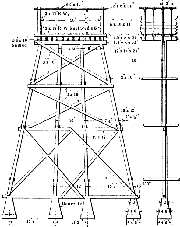
FIG. 34.—Delaney flume. Turlock main canal, Calif.
