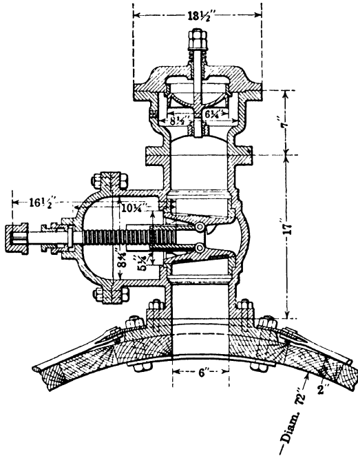
FIG. 62.—Air valve used on pipe line of Pioneer Power Plant, Ogden, Utah.
