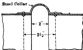
Section of Steel Tube Joint
