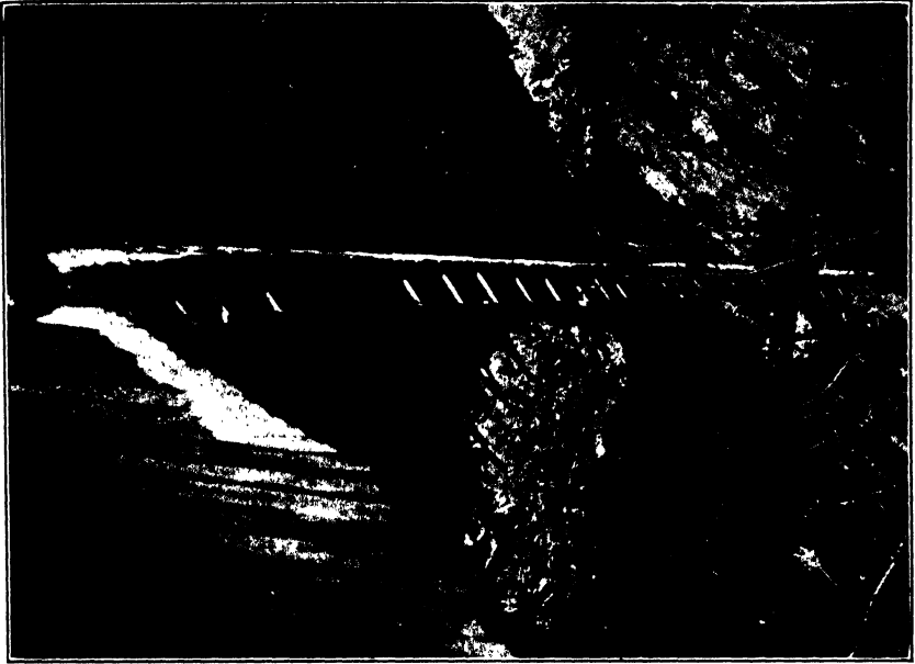
FIG. A.—Small wooden flume on rocky bluff. Penticton System, B. C.
