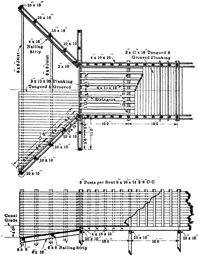
FIG. 50.—Inlet to wooden flume. Southern Alberta Land Co., Can.
