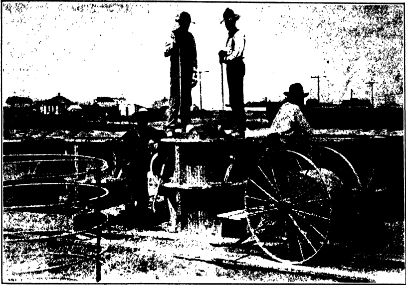
FIG. A.—Placing mixture in moulds, for 30-inch reinforced concrete pipe. Umatilla Project, Ore.
