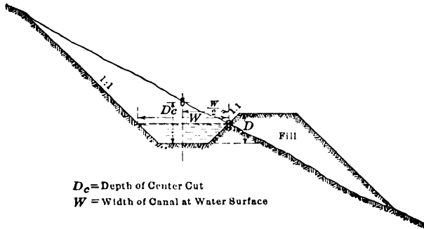
FIG. 2.—Location of Side-hill Canal with water cross section all in cut.
