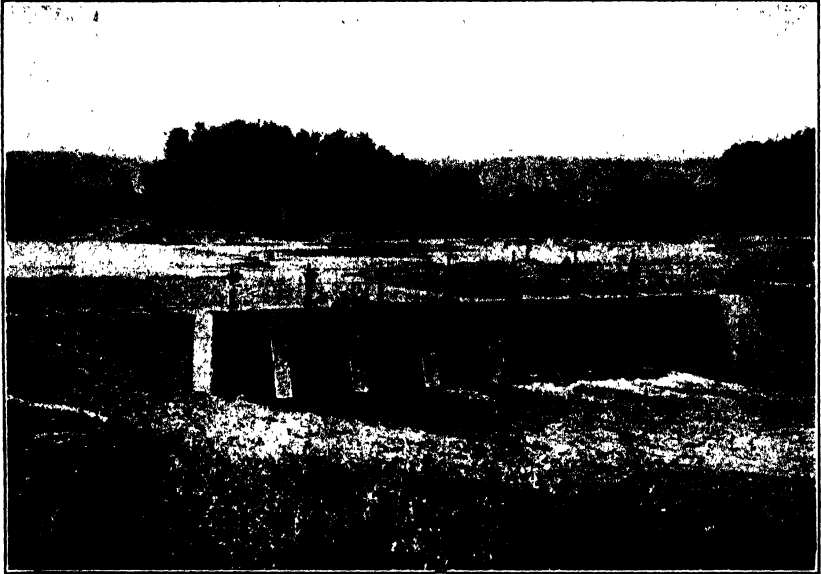
FIG. C.—Low diversion weir and headworks for main feed canal, Umatilla Project, Ore.
