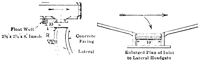
FIG. 11.—Type of lateral headgate on Punjab System, India, used in determination of coefficient of discharge.
