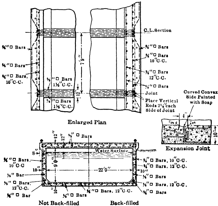
Fig. 32.—Bench flume of Big Fork Power Plant, Mont.
