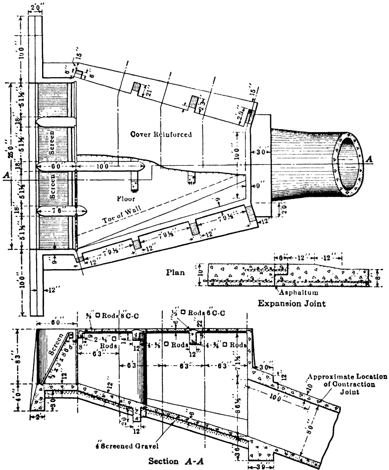
FIG. 79.—Inlet structure of Anderson Siphon. Belle Fourche Project, S. D.
