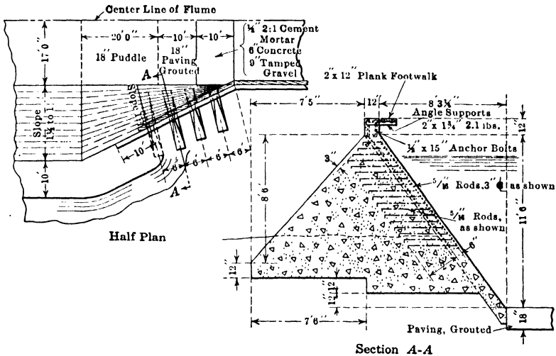
FIG. 49.—Inlet to flume, at Spring Canyon Draw. Interstate Canal, North Platte Project, Wyo., Neb.
