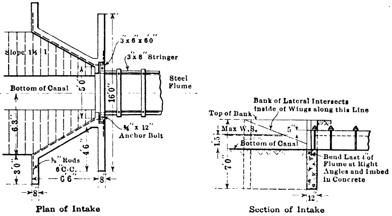
FIG. 53.—Inlet to steel flume on Sunnyside Project, Wash.
