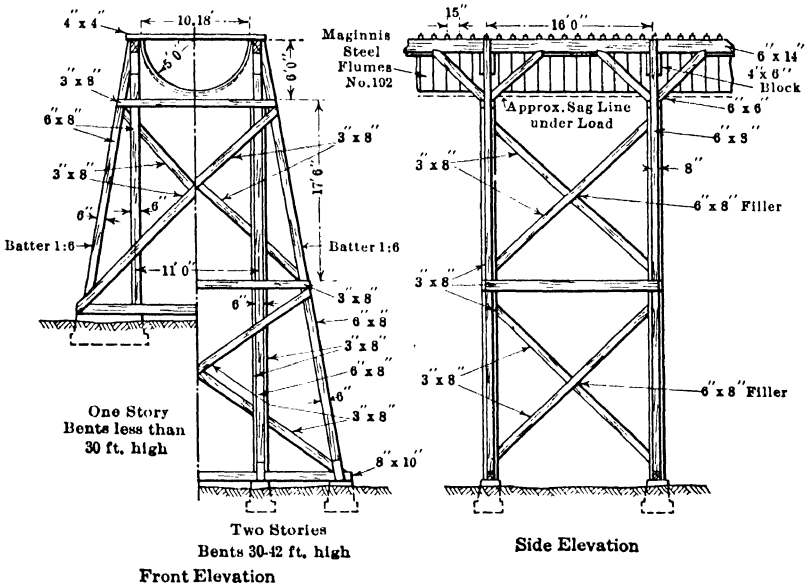
FIG. 44.—Steel flume. Twin Falls, Salmon River Land & Water Co., Idaho.
