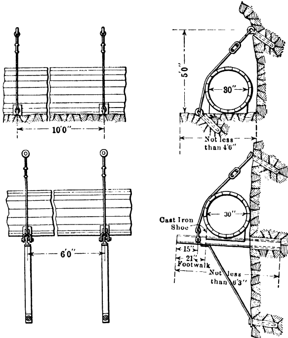
FIG. 68.—Method of supporting Canyon City pipe line on rock bench and vertical bluff. Colo.
