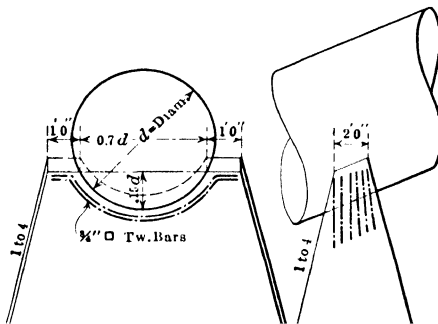
FIG. 57.—Standard piers for steel pipe. Jawbone Siphon, Los Angeles Aqueduct, Calif.
