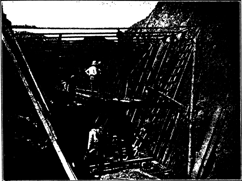
FIG. A.—Building forms for concrete lining. Truckee Carson Project, Nev.
