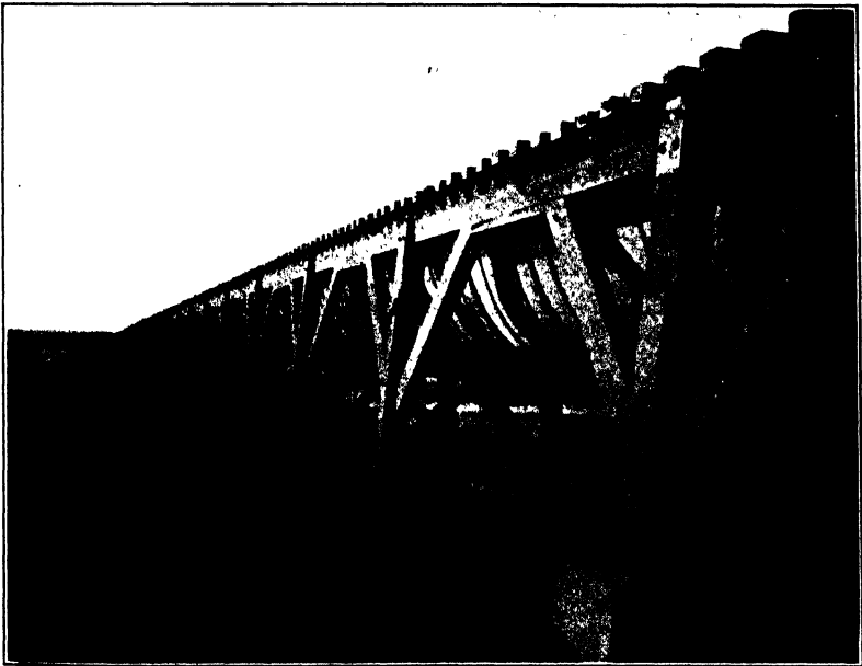
FIG. B.—Hess steel flume, 10 feet 10 inches diameter. Belle Fourche Project, S. D.
