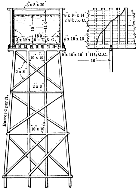
FIG. 36.—Flume of South Alberta Canal Co., Province of Alberta, Can.
