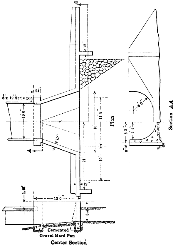
FIG. 54.—Inlet structure for steel flume. Twin Falls, Salmon River Land & Water Co., Idaho.
