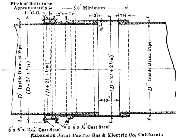
FIG. 56.—Standard type of expansion joint, developed by Pacific Gas & Electric Co., Calif.
