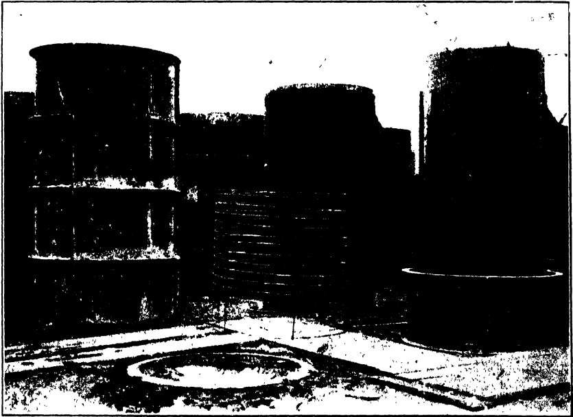
FIG. B.—Moulds for casting 47-in. reinforced concrete pipe. Umatilla Project, Ore.
