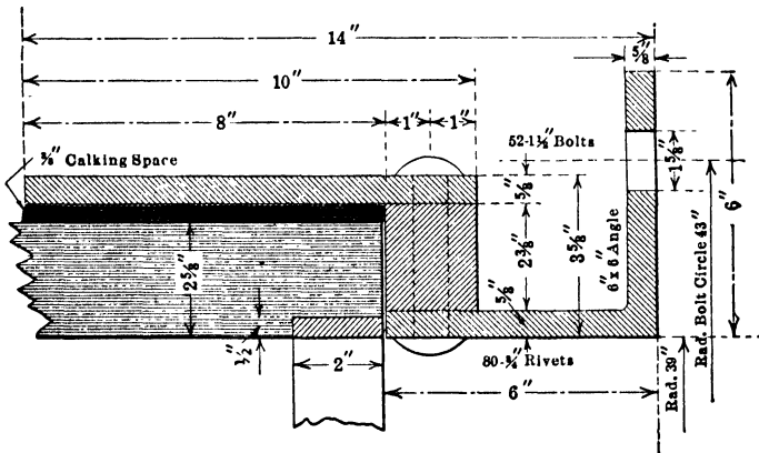
FIG. 66.—Riveted steel coupling collar to connect wood stave pipe with steel pipe. From Bull. No. 155, U. S. Dept. of Agr.
