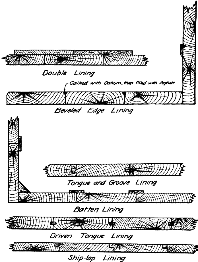
FIG. 33.—Types of lining for wooden flumes.
