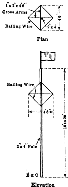
FIG. 4.—Signal for plain table work. Truckee-Carson Topographic Survey.
