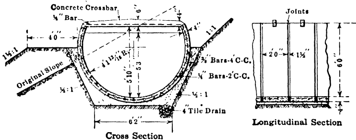
FIG. 24.—Reinforced concrete sectional lining. Tieton Project, Wash.
