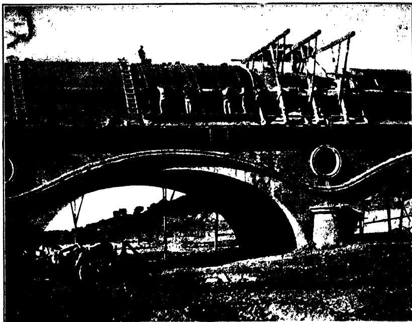
FIG. C.—Construction of concrete shell around steel tubes on bridge. Sosa Siphon, Spain.
