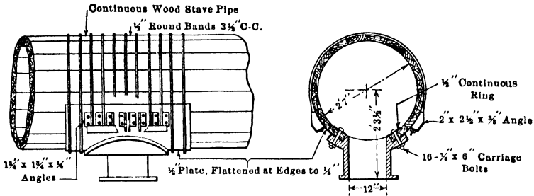
FIG. 65.—Saddle connection for blow-off. Prosser Siphon, Sunnyside Project, Wash.
