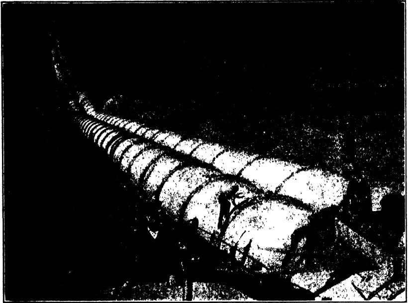
FIG. C.—Sosa Siphon, nearly completed. Spain.
