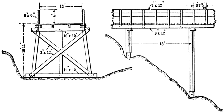
FIG. 37.—Flume on extension of North Poudre Canal, Colo.
