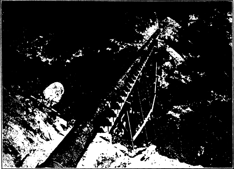
FIG. A.—24-inch machine banded wooden stave pipe on trestle. Southern Oregon (Washington Pipe & Foundry Co.).
