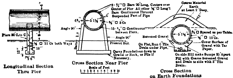
FIG. 76.—Sections of reinforced concrete pipe of Simms Creek Siphon, Sun River Project, Mont.
