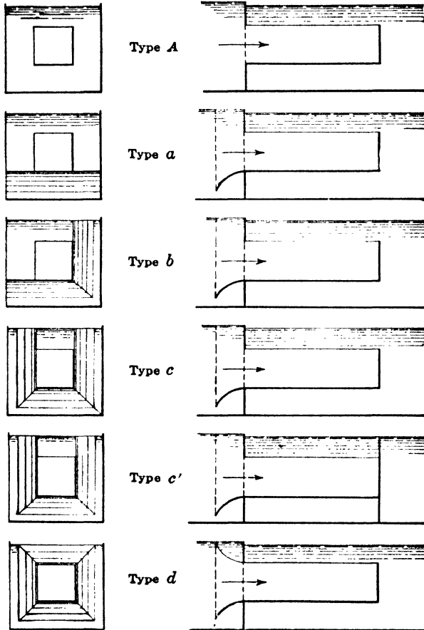
FIG. 12.—Forms of entrance of submerged tubes, 4 feet square, used in experiments made at University of Wisconsin.
