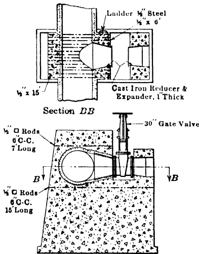
FIG. 81.—Blow-off, originally designed for Simms Creek Siphon. Sun River Project, Mont.
