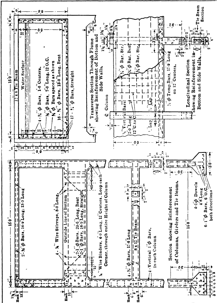
FIG. 46.—Reinforced concrete elevated flume, Naches Power Canal, Wash.
