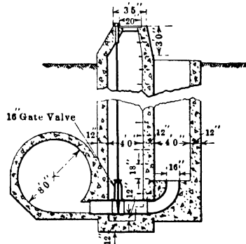
FIG. 82.—Blow-off for Anderson Siphon. Belle Fourche Project, S. D.
