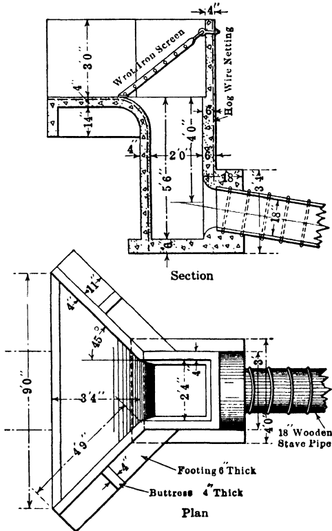
FIG. 77.—Inlet structure of Wolf Creek Siphon. American Beet Sugar Co., Colo.
