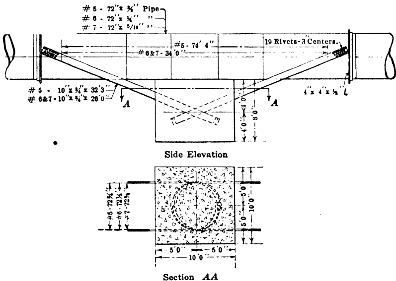
FIG. 59.—Anchorage on Drum pipe line. Pacific Gas & Electric Co., Calif.
