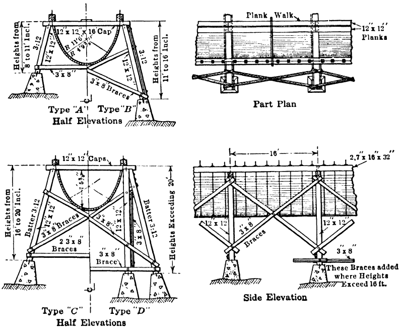
FIG. 41.—Wood stave flume. Puntledge River Power Canal, Vancouver Island, B. C.
