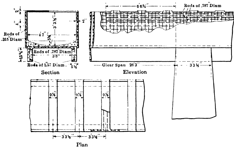
FIG. 47.—Reinforced concrete flume of Hamiz, Algeria.
