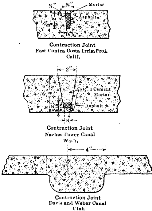
FIG. 20. --Contraction joints for concrete canal linings.
