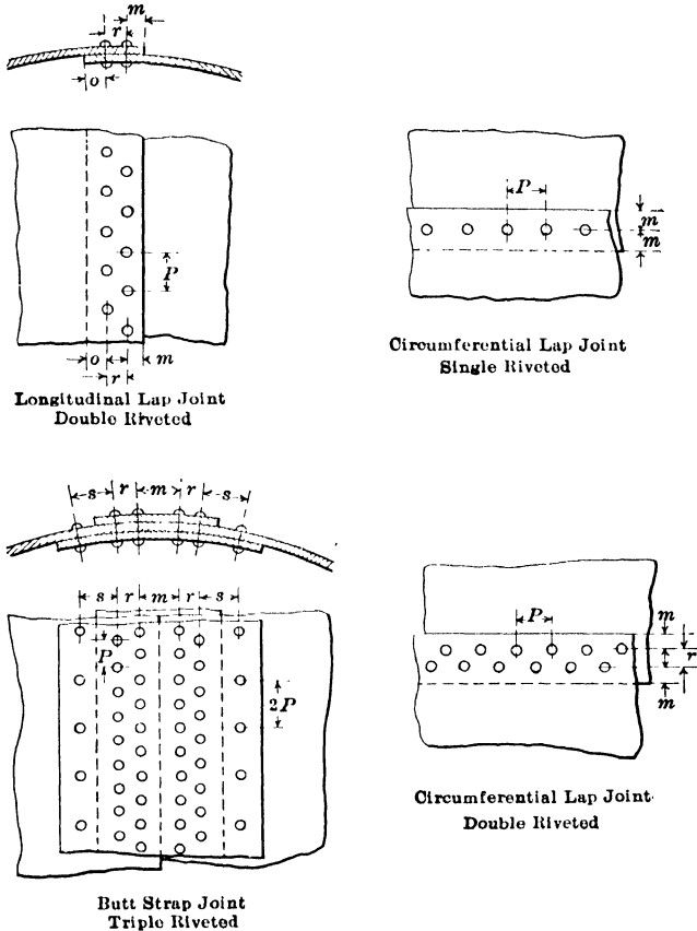
FIG. 55.—Details of types of riveted joints for steel pipes.
