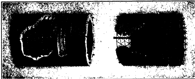
FIG. C.—Reinforced concrete pipe and lock joints made by Reinforced Concrete Pipe Co. of Los Angeles, Calif.
