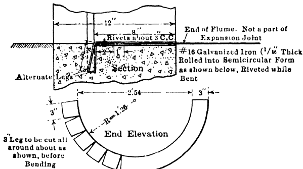
FIG. 42.—Expansion joint for Maginnis steel flume. Boise Payette project, Idaho.
