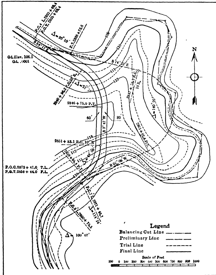
FIG. 3.—Details of paper location.
