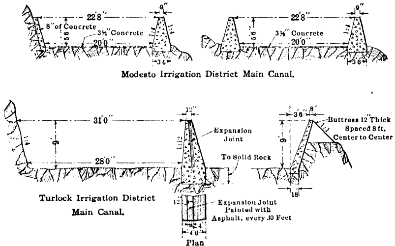
FIG. 28.—Concrete retaining wall, canal sections.
