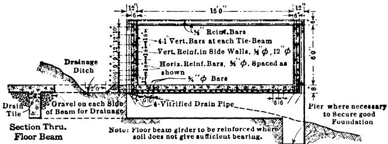
FIG. 31.—Reinforced concrete bench flume. Naches Power Canal, Wash.
