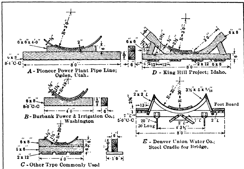
FIG. 67.—Supporting sills and cradles for wood stave pipe.
