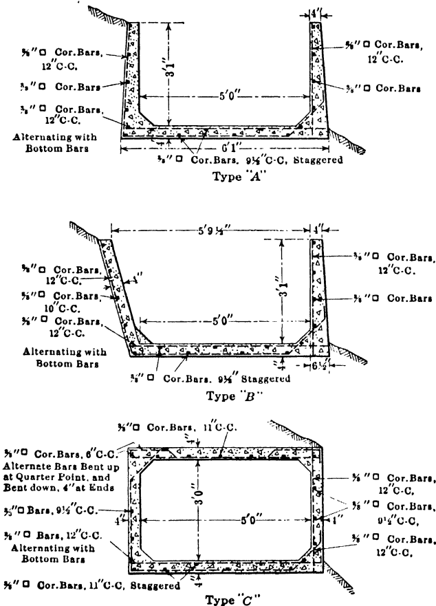
FIG. 30.—Reinforced concrete bench flumes. Yakima Valley Canal Co., Wash.
