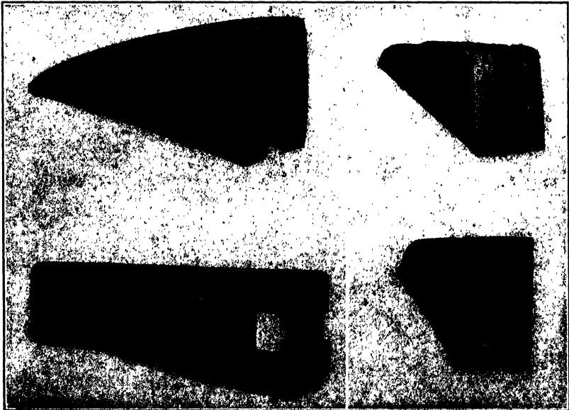
FIG. D.—Three types of shoes for wooden stave pipe. Marion Malleable Iron Works, Marion, Ind.
