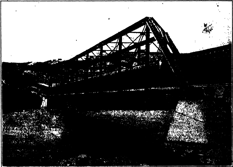
FIG. B.—60-inch continuous wooden stave pipe on bridge over Bear River, Oneida Irrigation District, Idaho. 300-foot head, \frac{3}{4} -inch bands, \frac{5}{8} -inch center to center. (Pacific Tank & Pipe Co.)
