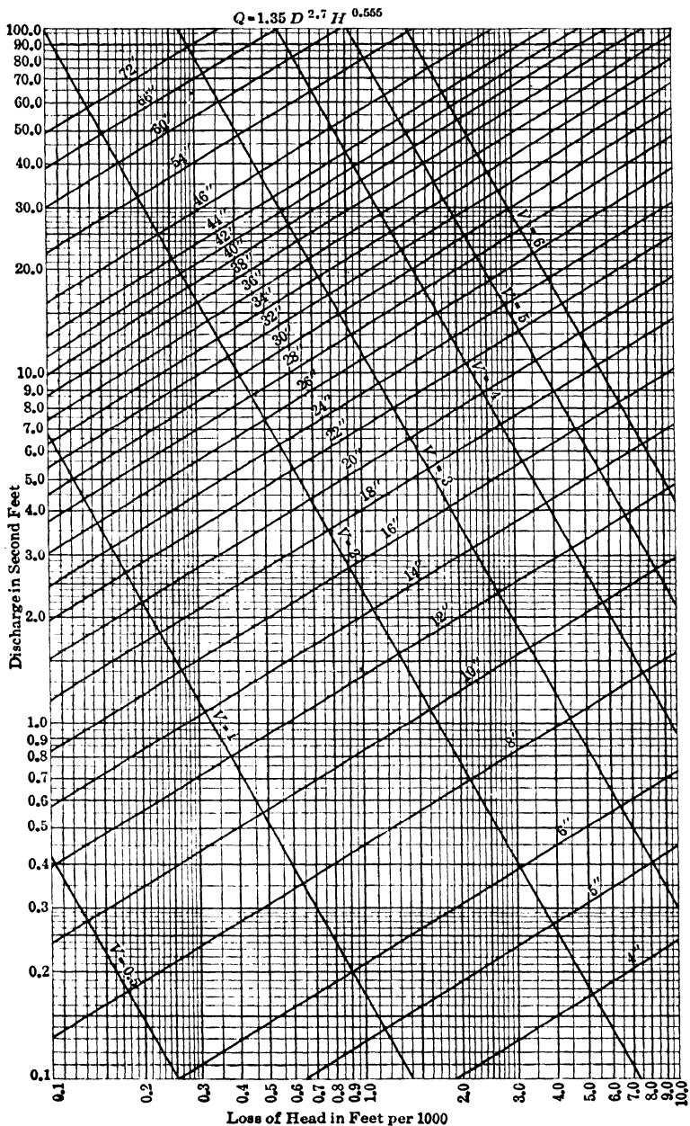
FIG. 8.—Diagram for the flow of water in wood-stave pipes, by E. A. Moritz.
