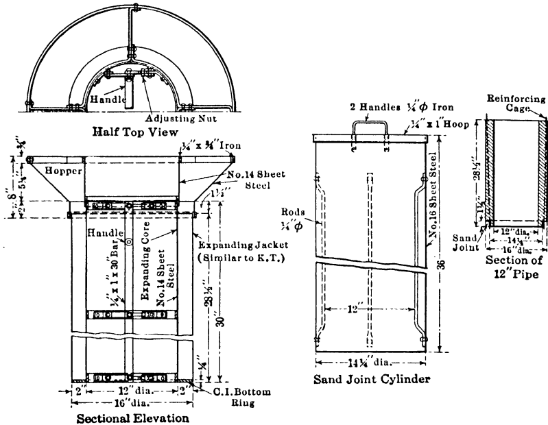
FIG. 69.—Moulds for making 12-inch reinforced concrete pipe. Tieton Project, Wash.
