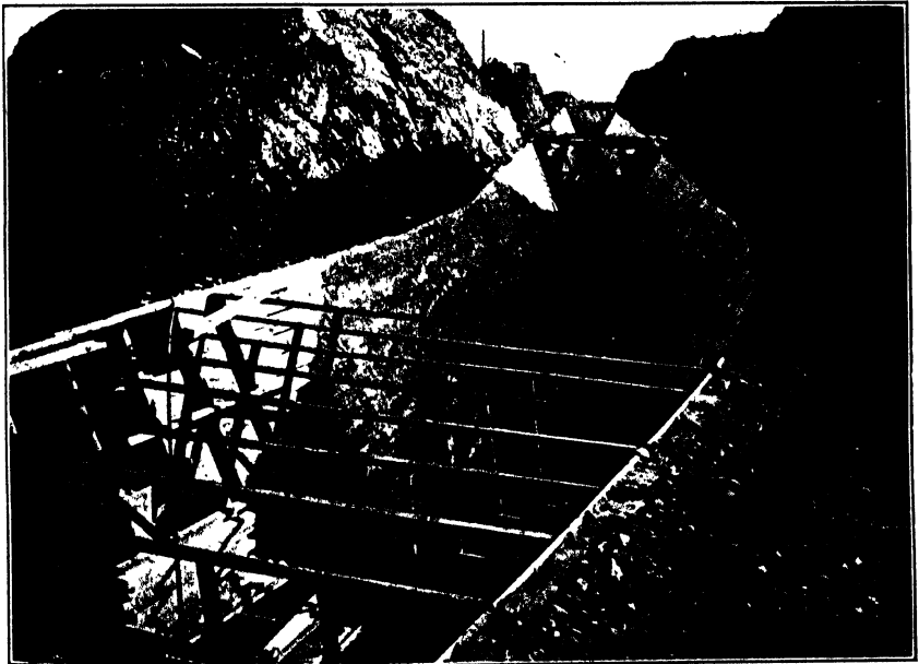
FIG. B.—Partly completed concrete-lined canal. Truckee Carson Project, Nev.
