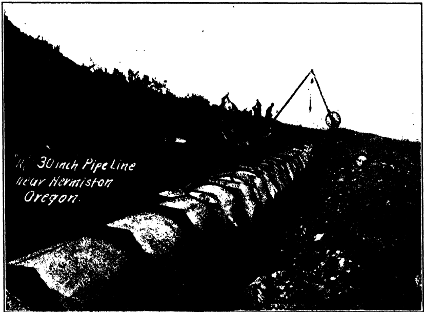
FIG. B.—Cast collars on 30-inch reinforced concrete pipe. Umatilla Project, Ore.
