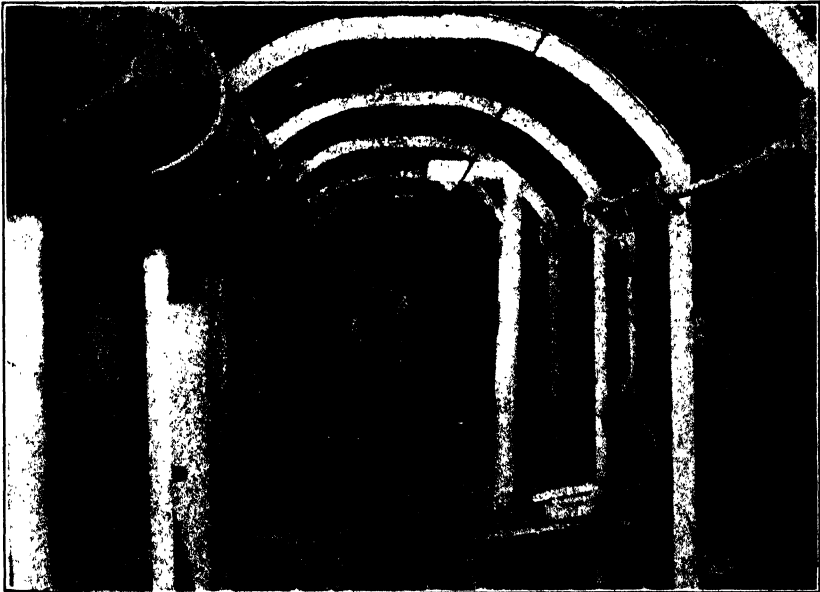
FIG. B.—Interior of Strawberry Valley Tunnel, in timbered section; steel ribs in place for supporting concrete forms; tramway and trolley; ventilation pipe. Strawberry Valley Project, Utah.
