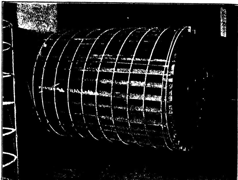
FIG. C.—Reel for making wire spiral reinforcement. Umatilla Project, Ore.
