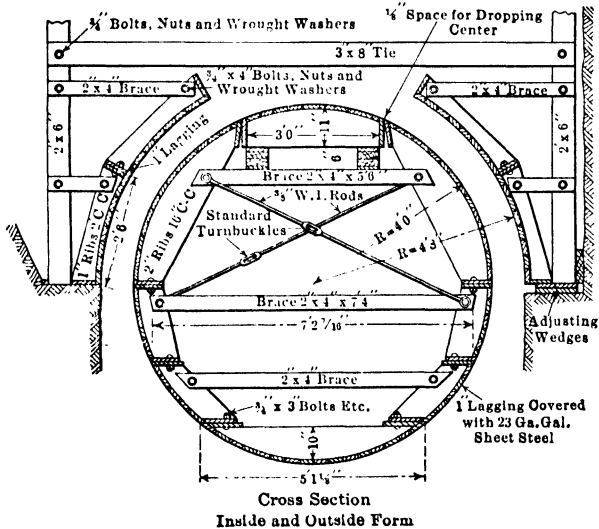
FIG. 72B.—Collapsible inside and outside forms for the construction of Anderson Siphon. Belle Fourche Project, S. D.
