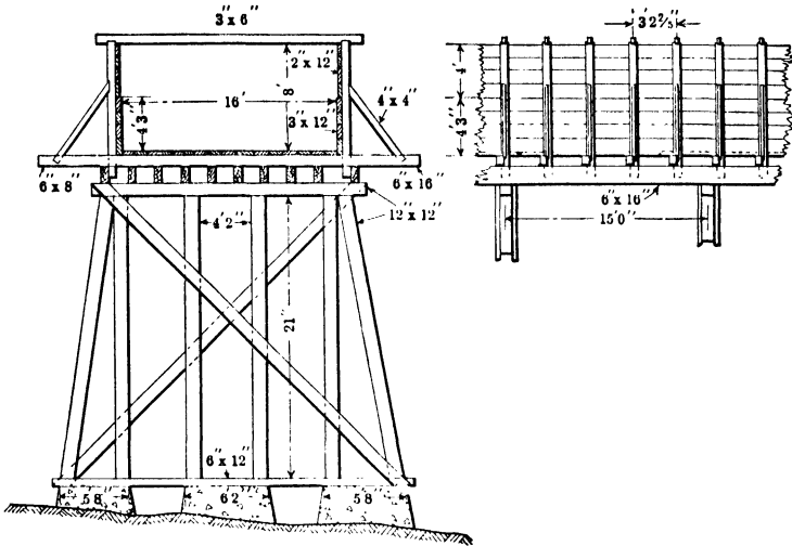
FIG. 35.—Flume of Kern River Power Co., Calif.
