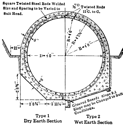
FIG. 72A.—Cross section of Anderson Siphon. Belle Fourche Project, S. D.
