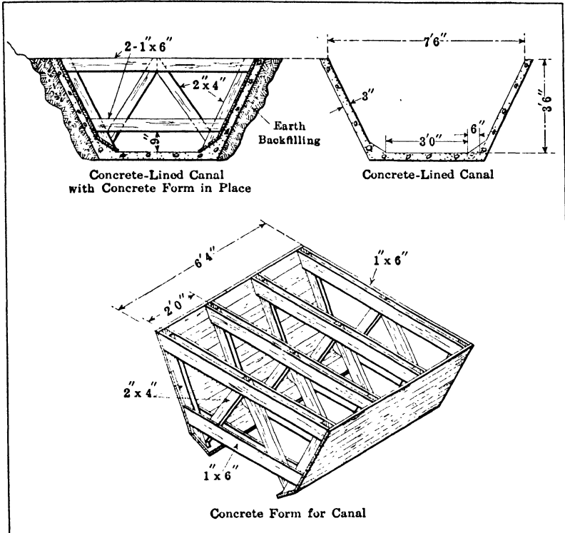
FIG. 21.—Method of concrete lining canals with forms. As used by Fruitlands Irrigation & Power Co., B. C.
