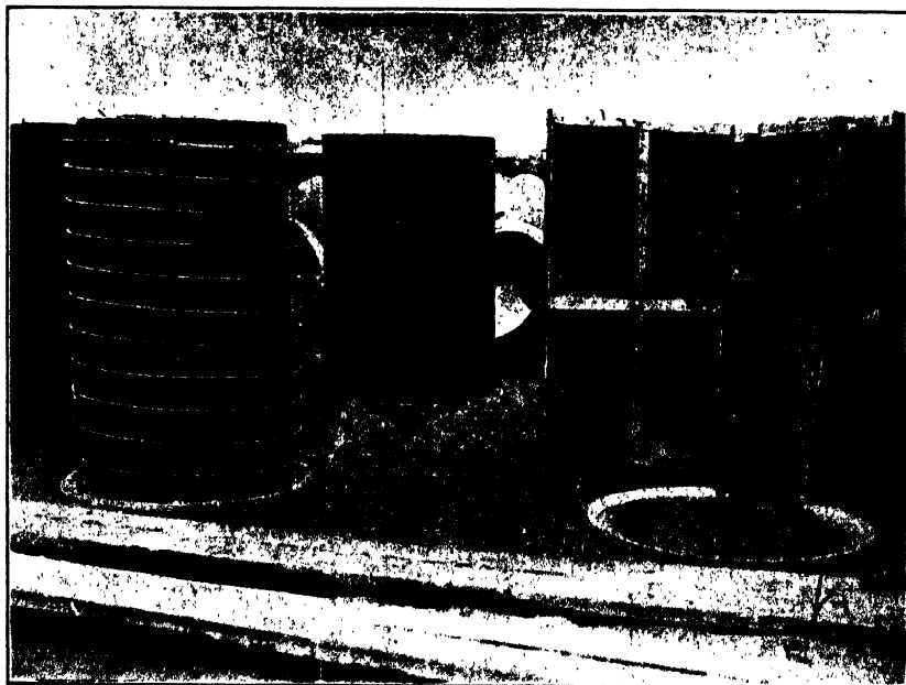
FIG. D.—Moulds for casting 30-inch reinforced concrete pipe. Umatilla Project, Ore
