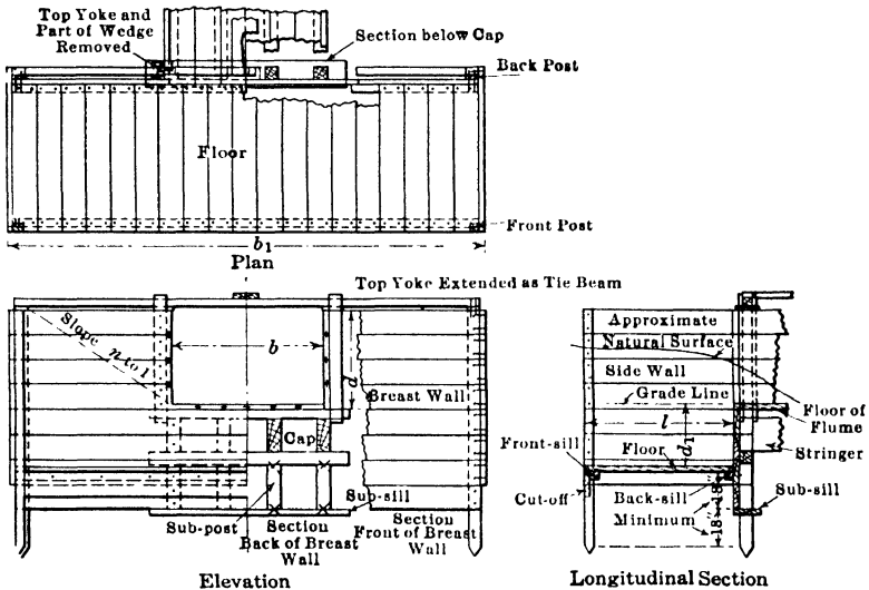
FIG. 51.—Standard design for inlet and outlet for wooden flume. U. S. Reclamation Service.
