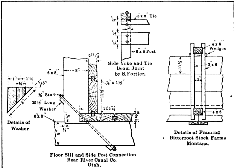
FIG. 38.—Details of framing for wooden flume box.
