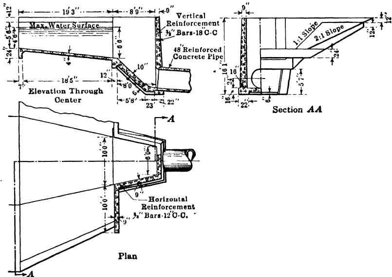
FIG. 78.—Inlet to reinforced concrete wasteway chute. Boise Project, Idaho.
