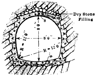
Tunnel in Untimbered Shale Bellefourche Project
