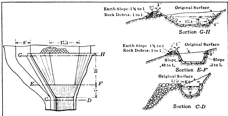
FIG. 19.—Transition from earth to concrete-lined section. Umatilla Project, Ore.
