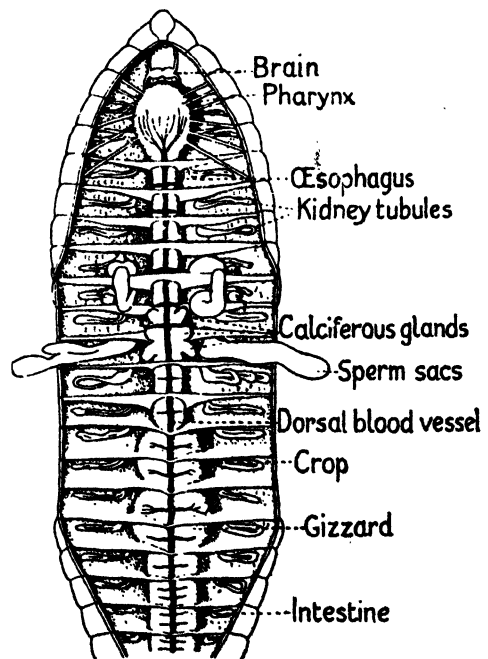
FIG. 55. DISSECTED EARTHWORM
