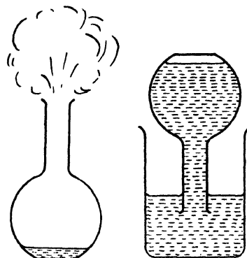
FIG. 44. SHOWING CONTRACTION WHEN VAPOUR CHANGES TO WATER
