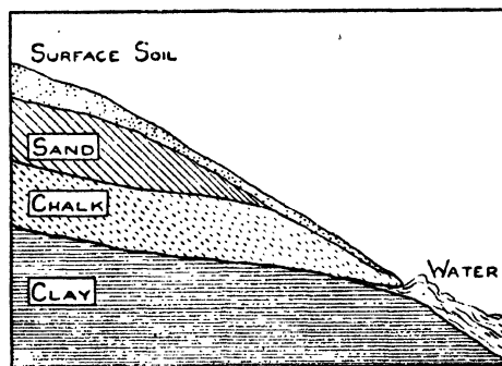
FIG. 56. FORMATION OF A SPRING
