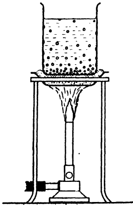
FIG. 39. AIR DRAWN FROM WATER
