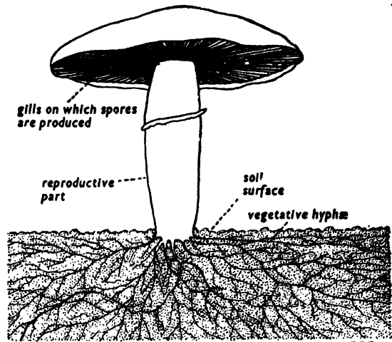
FIG. 96. MUSHROOM
