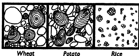
FIG. 76. STARCH GRAINS
