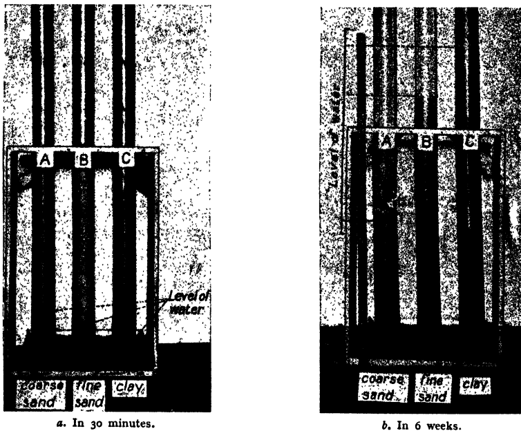
FIG. 100. TO SHOW RISE OF WATER IN TUBES PACKED WITH CLAY AND SAND
