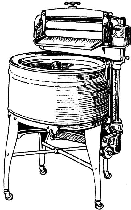
FIG. 91. AN ELECTRIC WASHER
