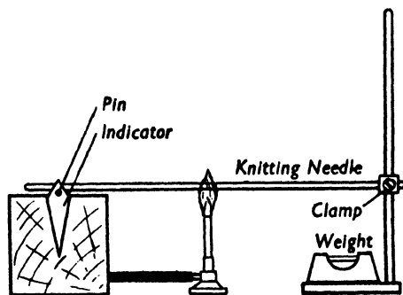
FIG. 11. EXPANSION OF STEEL
