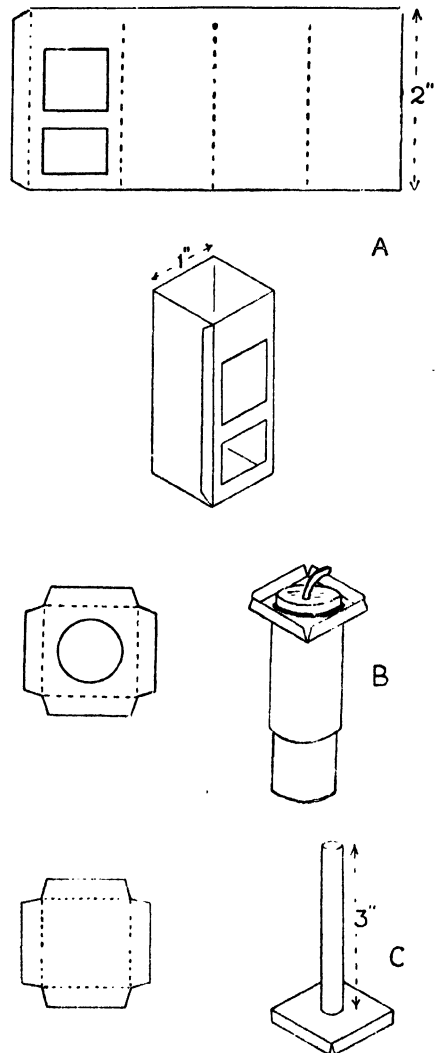
FIG. 1. COMPONENTS OF MODEL FIREPLACE (Dotted lines indicate bends in the tinplate.)
