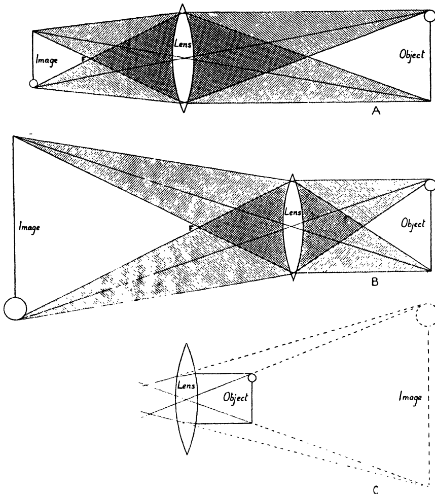
FIG. 69. IMAGES PRODUCED BY A CONVEX LENS
