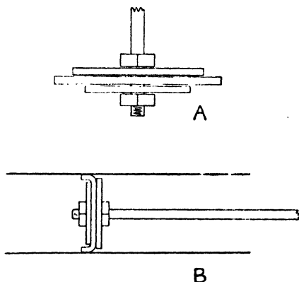
FIG. 28. MODEL TYRE PUMP A. PISTON ASSEMBLY B. PISTON IN BARREL
