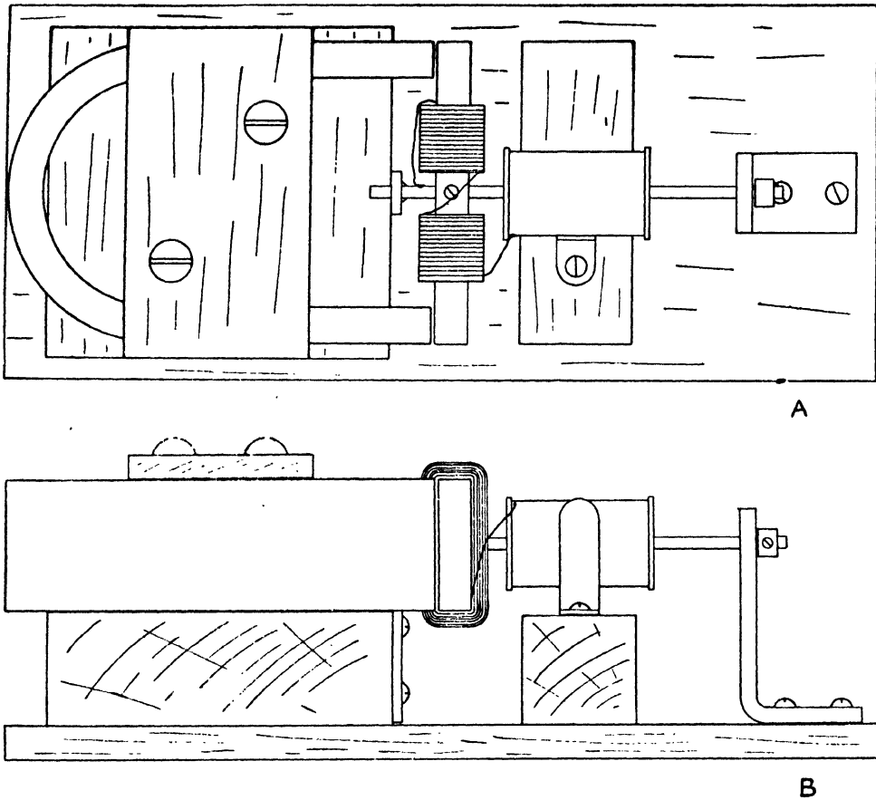
FIG. 33. SIMPLE SCHOOL-MADE MAGNETO DYNAMO
