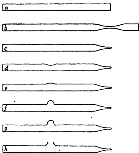
FIG. 8. STAGES IN BLOWING A NECK ON A GLASS TUBE
