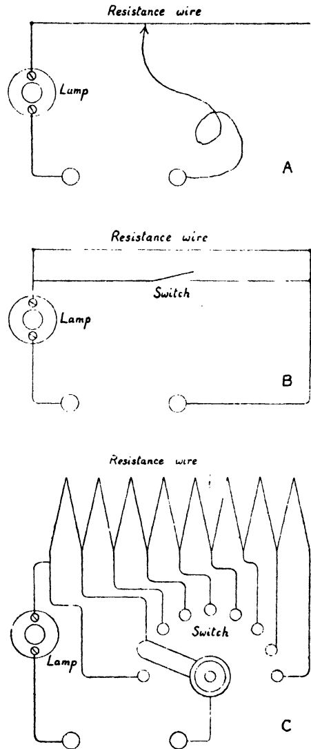
FIG. 41. A. CIRCUIT FOR SLIDING CONTROL DIMMER B. CIRCUIT FOR SWITCH DIMMER C. CIRCUIT INCORPORATING RHEOSTAT CONTROL
