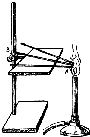
FIG. 21. TESTING THE BEST CONDUCTOR OF HEAT
