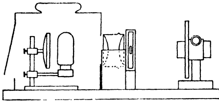
FIG. 76. ARRANGEMENT OF SIMPLE OPEN STAGE OPTICAL LANTERN
