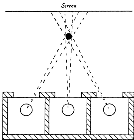
FIG. 44. PLAN OF COLOURED SHADOW APPARATUS
