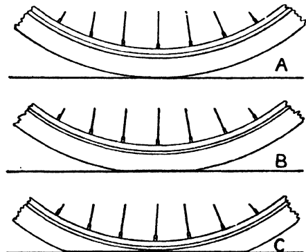
FIG. 22. A. NORMAL TYRE CONTACT B. HARD TYRE AT MAXIMUM COMPRESSION C. SOFT TYRE AT MAXIMUM COMPRESSION
