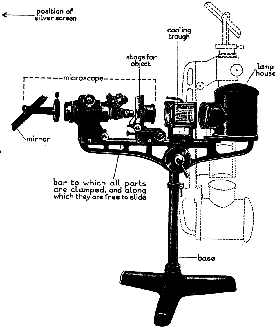
PLATE XXVIII. MICROPROJECTOR
