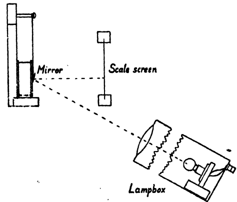
FIG. 31. OPTICAL ARRANGEMENT OF MIRROR GALVANOSCOPE
