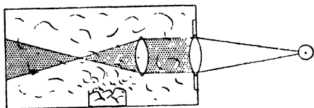
FIG. 65. ARRANGEMENT OF THE OPTICAL SMOKE BOX
