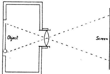
FIG. 68. DIAGRAM SHOWING THE ESSENTIAL DIFFERENCE BETWEEN THE CAMERA AND THE EPISCOPE
