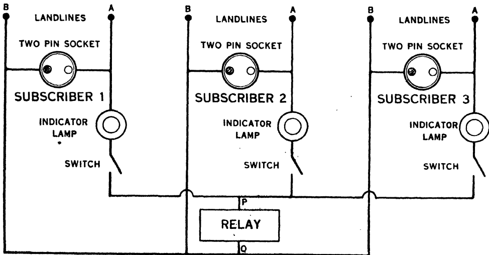
FIG. 3 CIRCUIT OF EXCHANGE APPARATUS FOR THREE SUBSCRIBERS.
