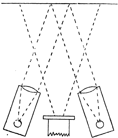
FIG. 45. PLAN OF THE THREE COLOUR PROJECTOR APPARATUS
