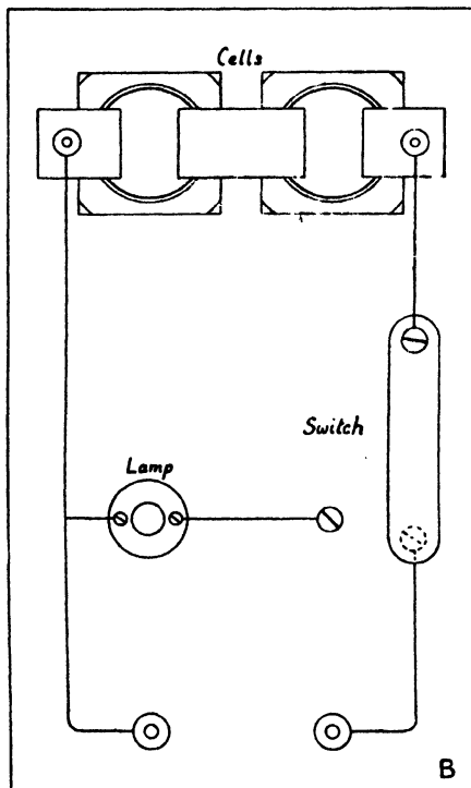
FIG. 36. ACCUMULATOR APPARATUS A. ARRANGEMENT OF LEAD STRIPS B. CIRCUIT
