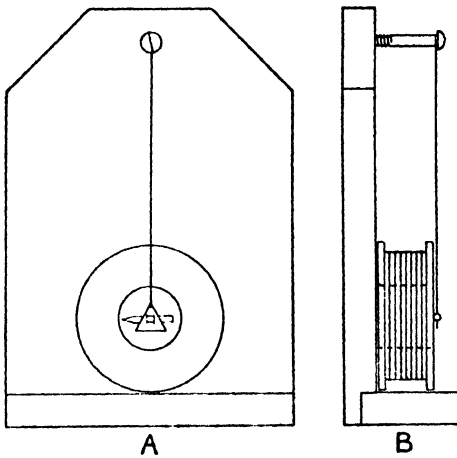
FIG. 30. CONSTRUCTIONAL DETAILS OF THE GALVANOSCOPE A. FRONT VIEW B. SIDE VIEW
