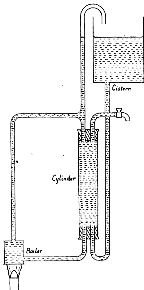
FIG. 4. ARRANGEMENT OF MODEL HOT WATER SYSTEM
