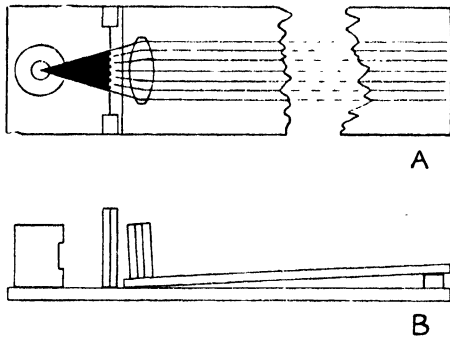
FIG. 61. ARRANGEMENT OF RAY APPARATUS A. PLAN, SHOWING A CONVEX LENS PRODUCING A PARALLEL BEAM B. SIDE ELEVATION
