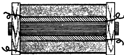
FIG. 10 THE MICROPHONE TRANSFORMER
