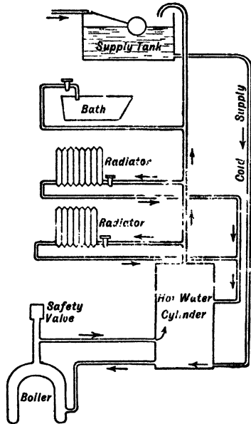
FIG. 3. COMMERCIAL TYPE OF HOT WATER SYSTEM, FITTED WITH PIPES WHICH PROVIDE A SECONDARY CIRCULATION THROUGH RADIATORS
