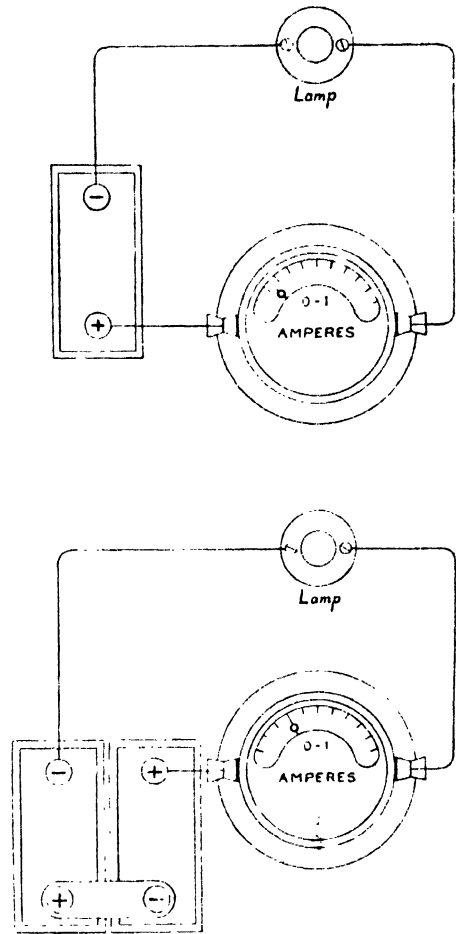
FIG. 37. EFFECT OF INCREASING THE VOLTAGE APPLIED TO A CIRCUIT
