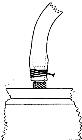
FIG. 24. HOW THE ADDITIONAL TYRE VALVE IS ASSEMBLED
