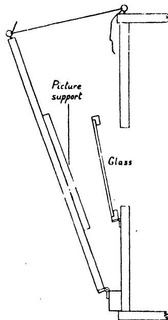
FIG. 74. ARRANGEMENT OF THE GLASS, FRAME AND PICTURE SUPPORTING DEVICE AT THE BACK OF THE EPISCOPES
