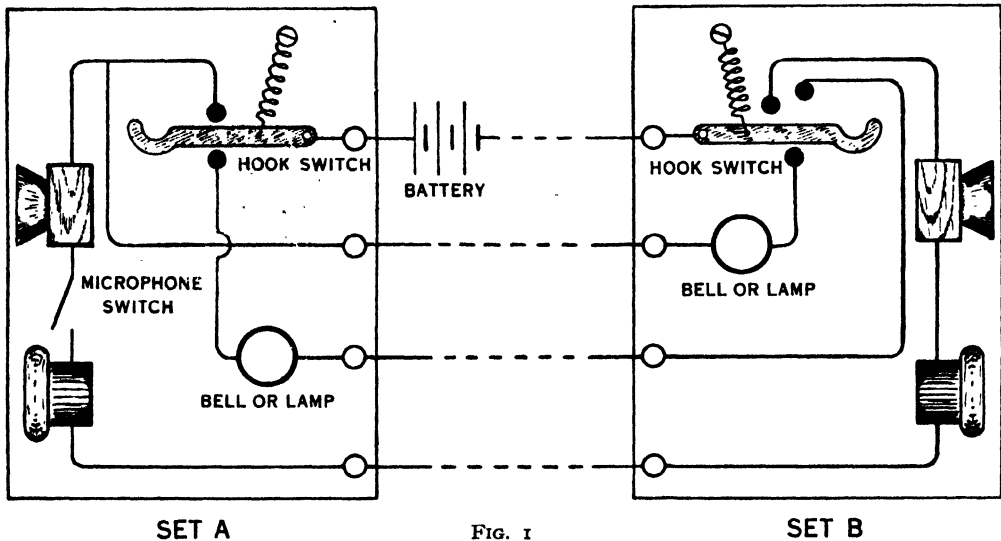
FIG. 1 A SIMPLE TELEPHONE INSTALLATION, INCORPORATING ALTERNATIVE FORMS OF MICROPHONE SWITCH Set A: Manually operated press switch. Set B: Automatically operated spring hook switch.
