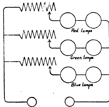
FIG. 47. CIRCUIT DIAGRAM FOR LAMPS AND RHEOSTATS
