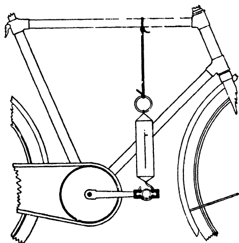
FIG. 18. EXPERIMENTAL ARRANGEMENT USED FOR MEASURING THE FORCE APPLIED BY A CYCLIST ON THE PEDALS
