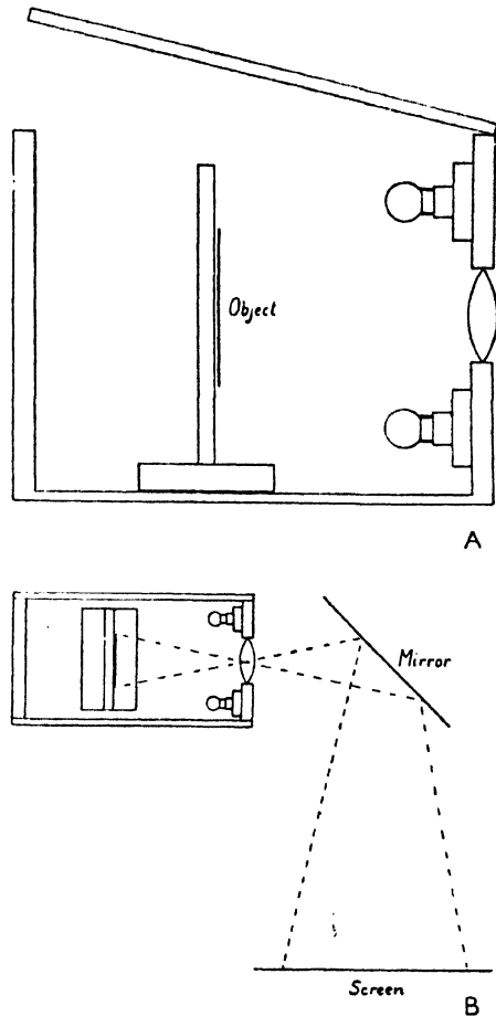
FIG. 70. A. SIMPLE MODEL EPISCOPES B. EPISCOPES PROJECTION, USING A REVERSING MIRROR
