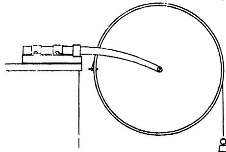
FIG. 14. ARRANGEMENT OF APPARATUS DESIGNED TO COMPARE THE EFFICIENCY OF BALL AND PLAIN BEARINGS
