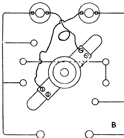
FIG. 43. A. SERIES PARALLEL CIRCUIT, USING TUMBLER SWITCHES B. SERIES PARALLEL CIRCUIT, USING DOUBLE ENDED ROTARY STUD SWITCH
