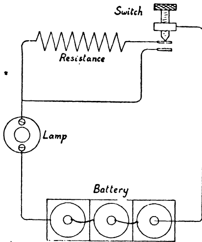
FIG. 40. CYCLE LAMP CIRCUIT, WITH DIMMING SWITCH
