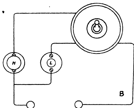
FIG. 42. A. HIGH AND LOW POWER LAMP CIRCUITS WITH SIMPLE CHANGE-OVER SWITCH B. ALTERNATIVE ARRANGEMENT WITH TWO WAY TUMBLER SWITCH
