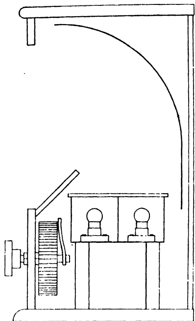
FIG. 48. ARRANGEMENT OF RHEOSTAT CONTROLLED COLOUR EFFECTS APPARATUS
