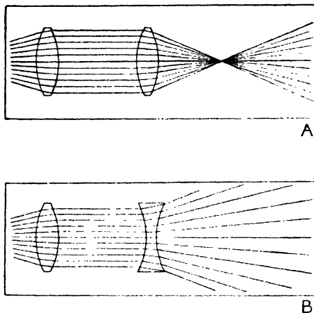
FIG. 64. RAY APPARATUS IN USE
