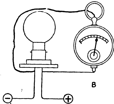
FIG. 39. VOLTAGE MEASUREMENTS ON BULBS A. SIDELAMP B. HEADLAMP
