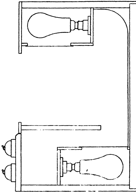
FIG. 46. ARRANGEMENT OF MODEL STAGE LIGHTING APPARATUS
