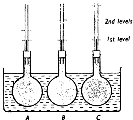
FIG. 14. EXPANSION COMPARED OF WATER, TURPENTINE AND ALCOHOL.
