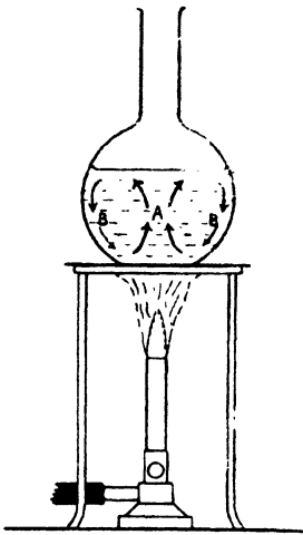
FIG. 24. CONVECTION CURRENTS IN HEATED WATER
