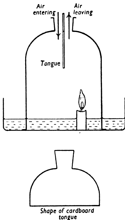
FIG. 26. A CANDLE BURNING THROUGH CONVECTION CURRENTS
