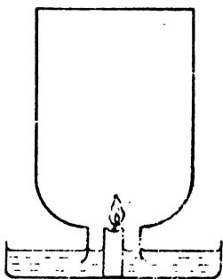
FIG. 69. FLAME GOING OUT WITH- OUT AIR
