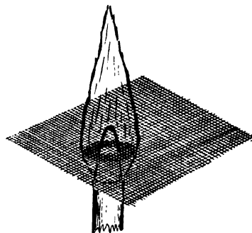
FIG. 62. HOT AND COOL ZONES SHOWN IN GAUZE
