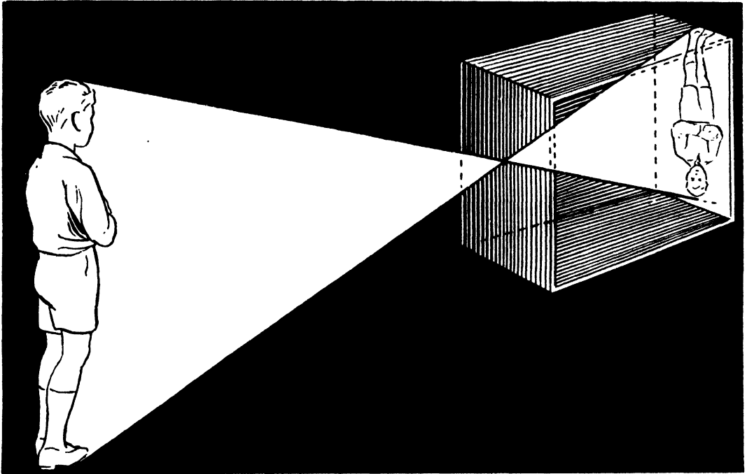
DIAGRAM SHOWING HOW INVERTED IMAGES ARE FORMED ON THE RETINA OF THE EYE
