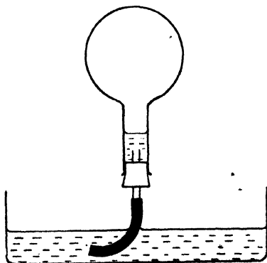
FIG. 32. SHOWING HOW MUCH AIR WEIGHS
