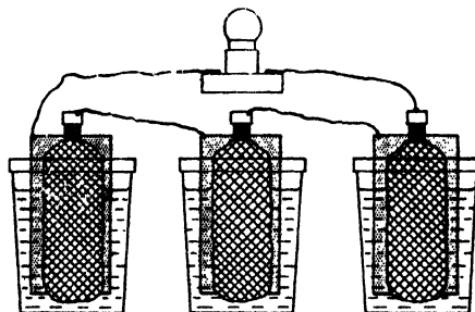
FIG. 35. REVIVED CELLS IN SERIES WITH A FLASHLAMP BULB
