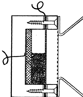
FIG. 7 THE CARBON DISC MICROPHONE
