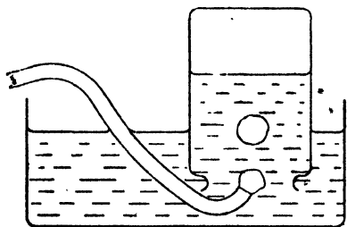
FIG. 25. MEASURING THE AIR IN A PNEUMATIC TYRE
