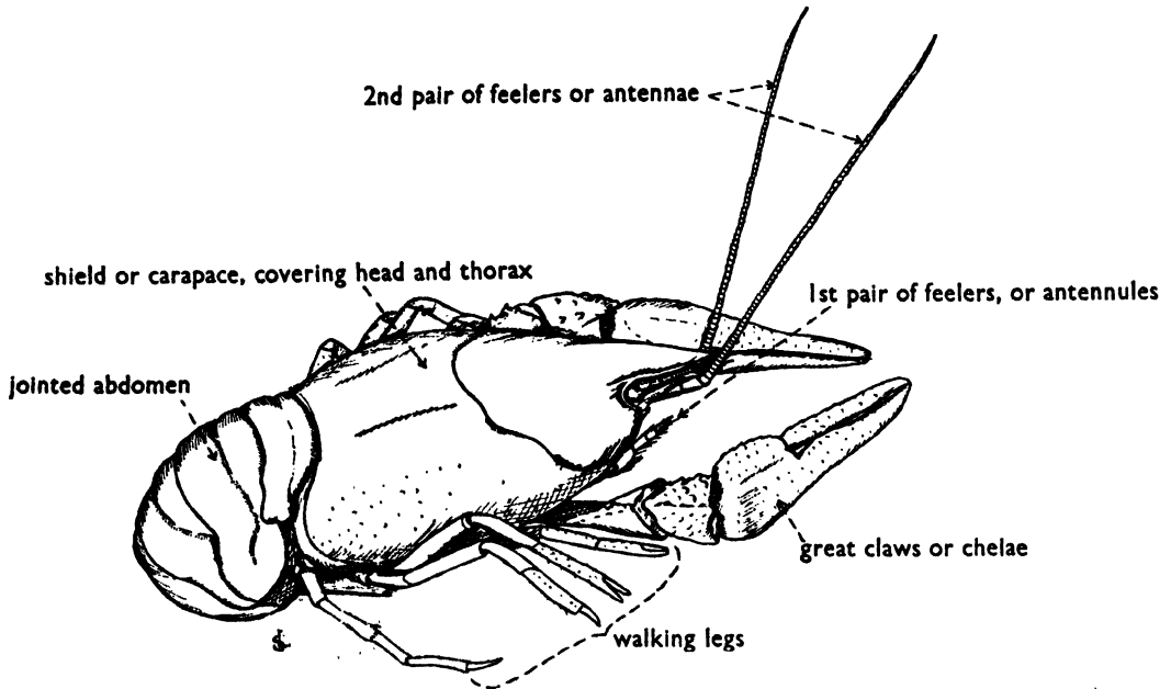
FIG. 68. CRAYFISH
