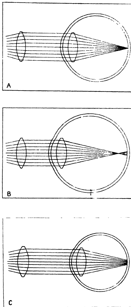
FIG. 78. EYE DEFECTS DEMONSTRATED ON THE RAY BOARD A. A NORMAL EYE B. A SHORT-SIGHTED EYE C. A LONG-SIGHTED EYE
