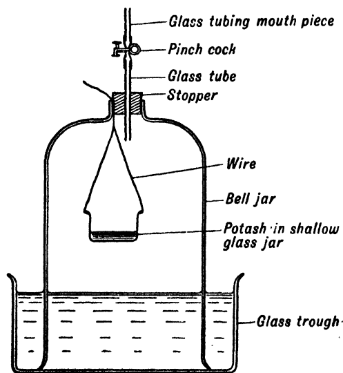
FIG. 79. TO SHOW THAT OXYGEN IS REMOVED FROM AIR WHICH HAS BEEN BREATHED
