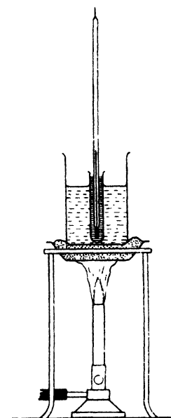
FIG. 8. BOILING POINT OF ALCOHOL
