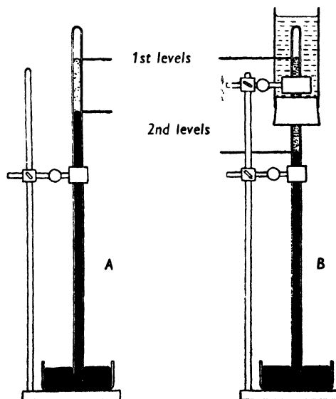
FIG. 45. WATER VAPOUR EXERTS PRESSURE
