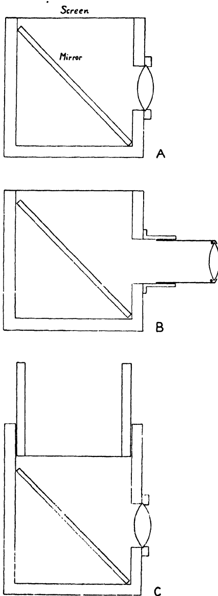
FIG. 67. A HAND CAMERA VIEW FINDER
