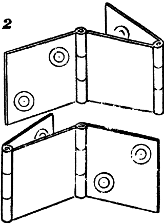
EVERYDAY HINGES
