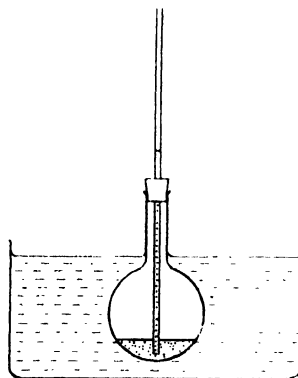
FIG. 15. EXPANSION OF AIR
