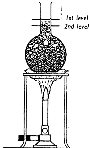
FIG. 40. ICE CONTRACTING ON MELTING
