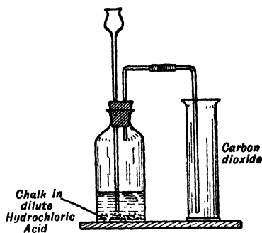
FIG. 78. PREPARATION OF CARBON DIOXIDE
