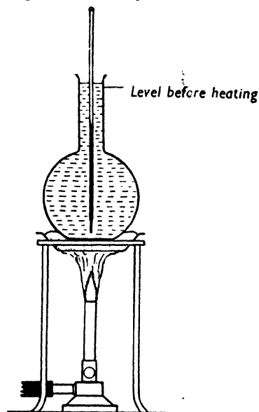
FIG. 13. EXPANSION OF WATER
