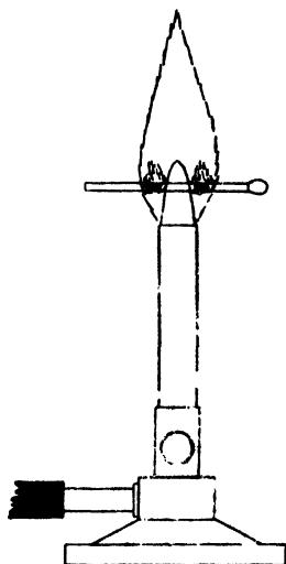
FIG. 61. A MATCHSTICK BURNS IN THE OUTER ZONE OF A BUNSEN FLAME BUT NOT IN THE CENTRAL PART
