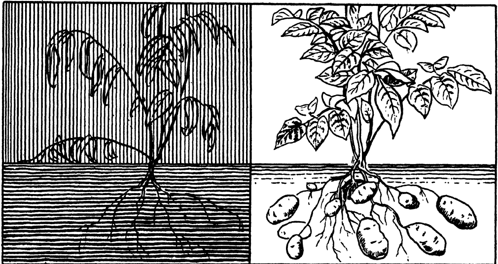
DIAGRAM OF SPECTRUM; DIAGRAM OF SPECTRUM AND PRISM; THE VALUE OF SUNLIGHT
