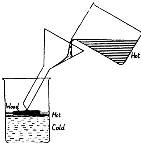
FIG. 6. FLOATING HOT WATER ON COLD
