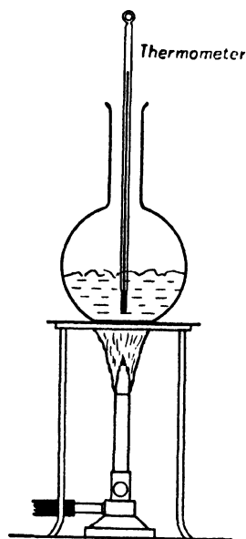
FIG. 5. FINDING THE BOILING POINT OF WATER
