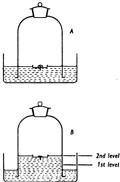
FIG. 70. SHOWING RESULT WHEN PHOSPHORUS IS BURNT
