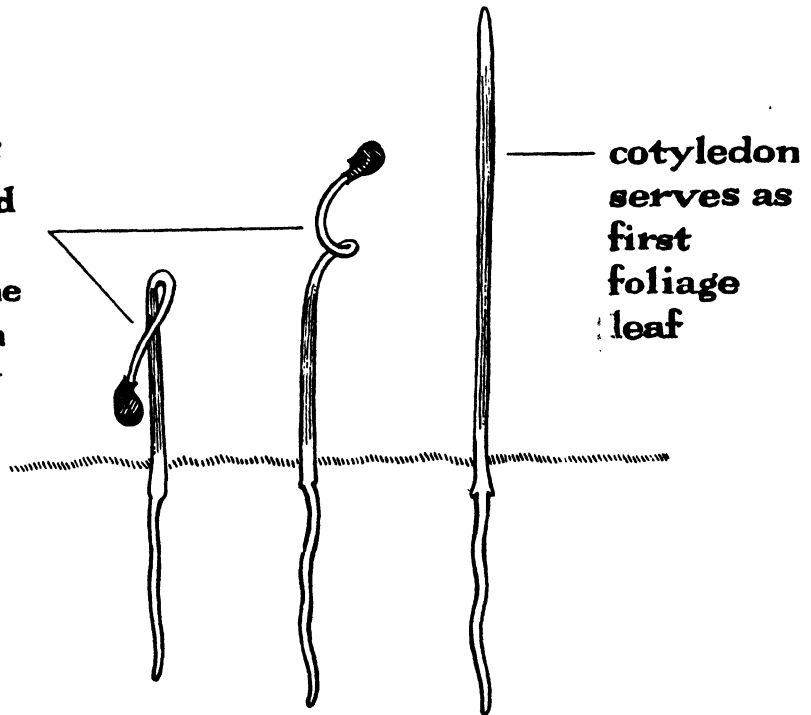
FIG. 83. ONION SEEDLINGS
