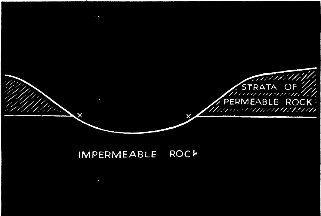
FIG. 27. HOW A SPRING MAY GIVE RISE TO A POND
