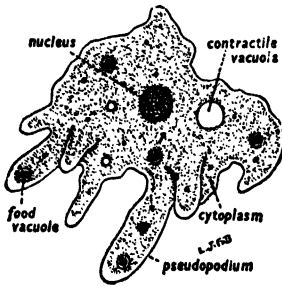
AMOEBA
