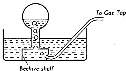
FIG. 1. FILLING A FLASK WITH COAL GAS
