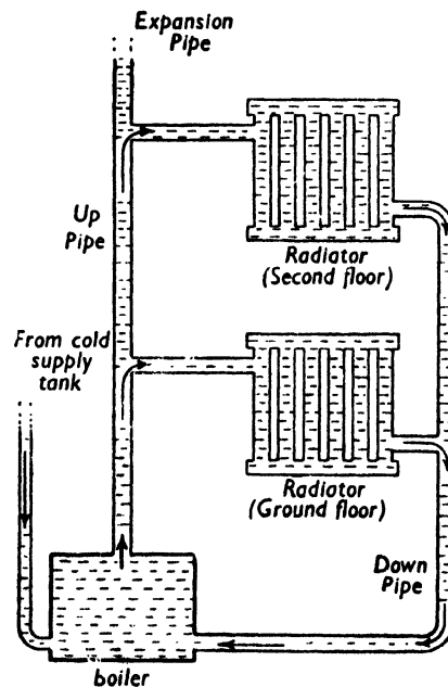
FIG. 25. HEATING A BUILDING
