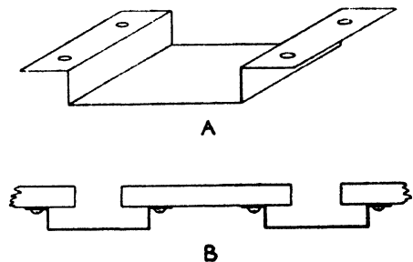
FIG. 73. A. TINPLATE LIGHT Baffle FOR EPISCOPE VENTILATORS B. DIAGRAM SHOWING Baffles IN POSITION
