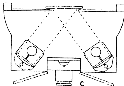
FIG. 72. A. PLAN OF EPISCOPIC FITTED WITH ORDINARY FILAMENT LAMPS B. PLAN OF EPISCOPIC WITH SINGLE PROJECTOR LAMP C. PLAN OF EPISCOPIC WITH TWIN PROJECTOR LAMPS
