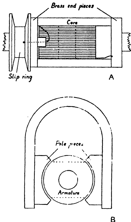
FIG. 34. THE MAGNETO DYNAMO A. DETAILS OF ARMATURE ASSEMBLY AND WIRING B. END VIEW, SHOWING MAGNET, POLE PIECES AND ARMATURE
