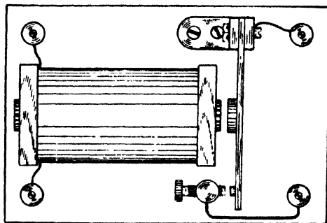
FIG. 12 THE EXCHANGE BELL RELAY
