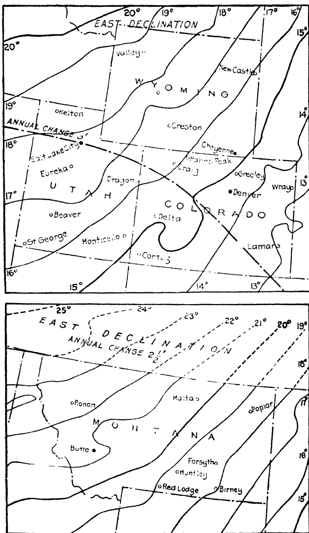
FIG. 266 —Magnetic declinations (1915).—(Continued.)
