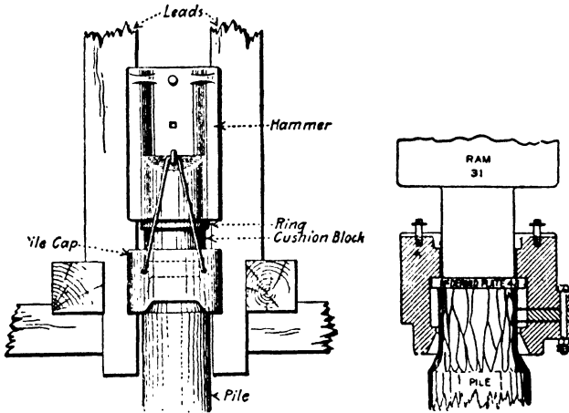
FIG. 359.—Pile caps.
