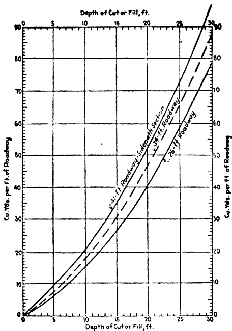
Graphic for estimating road approach earthwork grade crossing eliminations.
