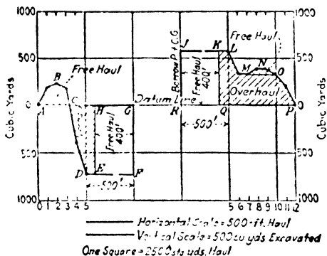
FIG. 319.—Mass diagram, Case II.
