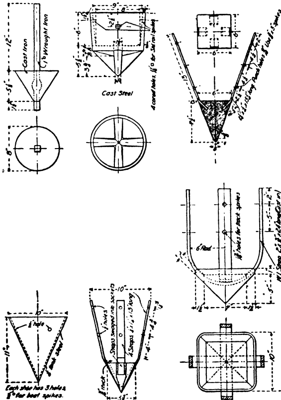
FIGS. 13d, e and f.—Shoes for Timber Piles.
