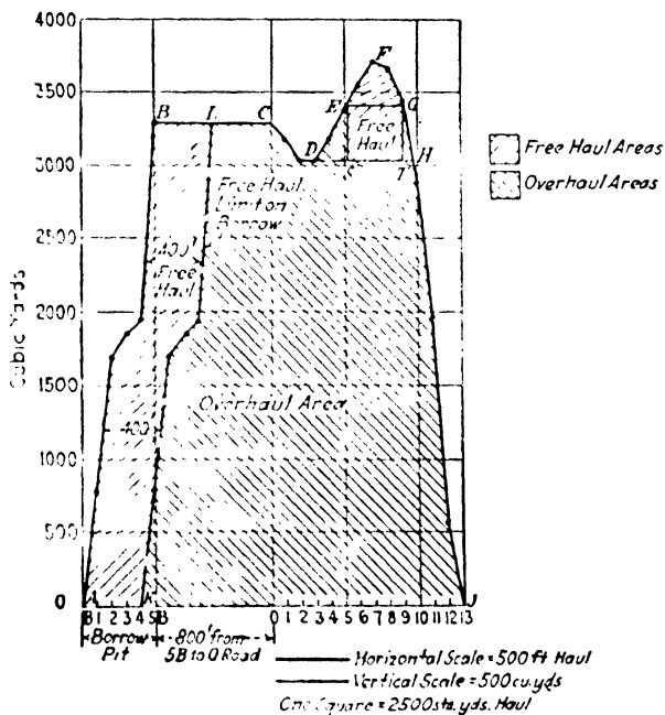
FIG. 320.—Mass diagram, Case III.
