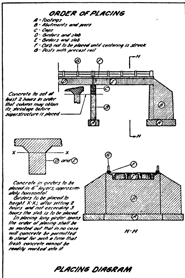
FIG. 355.—Order of placing concrete.
