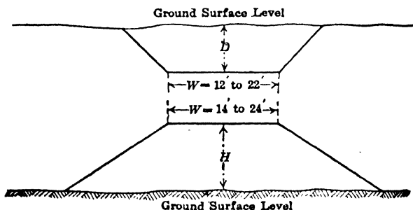
APPROXIMATE AMOUNTS OF EMBANKMENT AND EXCAVATION FOR DIFFERENT CENTER-LINE CUTS AND FILLS, GROUND SURFACE ASSUMED LEVEL
