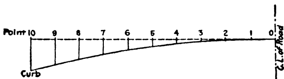
Parabolic crown ordinates.
