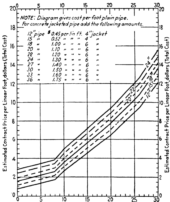
Average cost sewers. (Lima, Ohio, 1921.)
