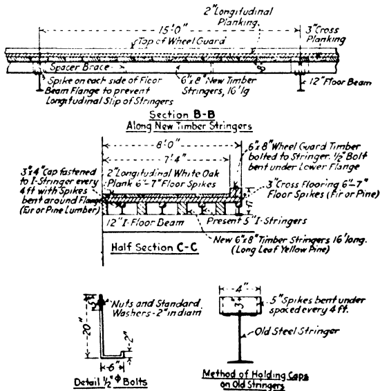
Typical bridge floor repair and strengthening road 485.
