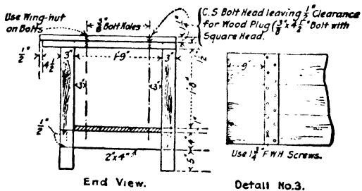
FIG. 288.—Folding kitchen camp table.
