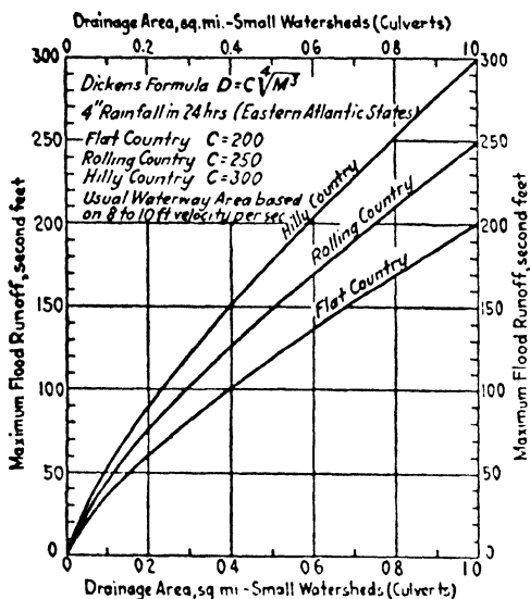
DIAGRAM 1.—Flood runoff for small streams. N. Eastern States (See Table 47, page 189.)
