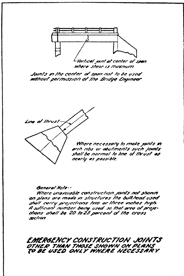
FIG. 356.—Emergency construction joints.
