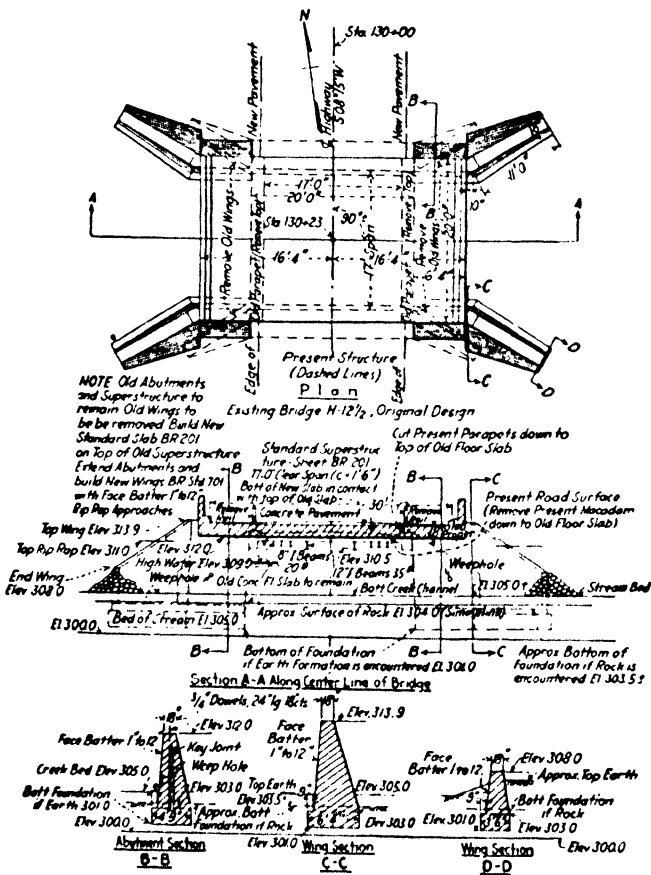
FIG. B.—Utilization of old structures, Case 2. Saved $1500 over entire new structure.
