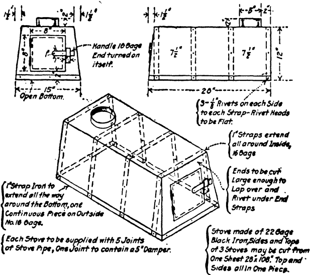
FIG. 287.—Tent heater
