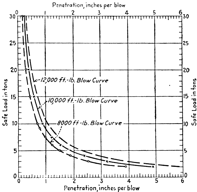
FIG. 346B.—Safe pile loads. Double acting steam hammer test penetrations.
