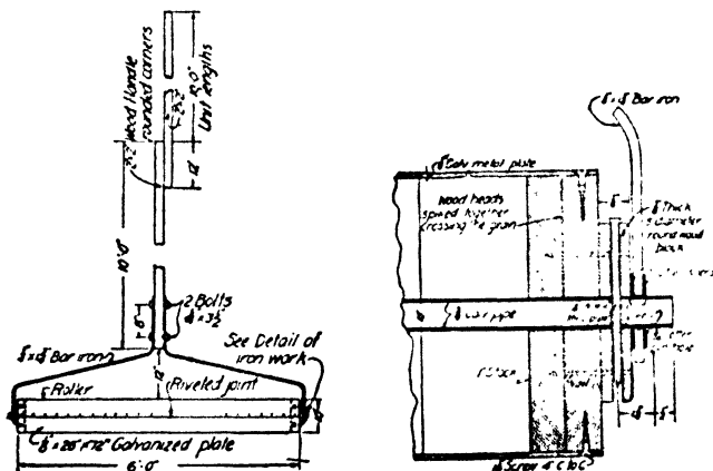
FIG. 340.—Detail of roller.
