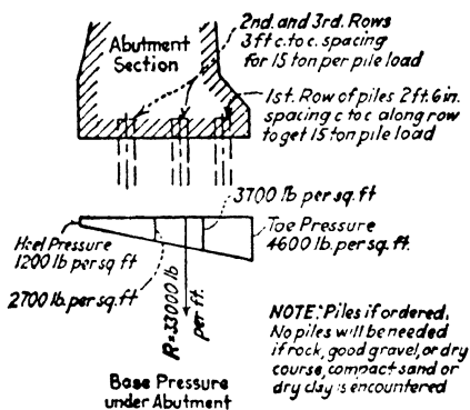
FIG. 321.—Typical base pressure diagram.
