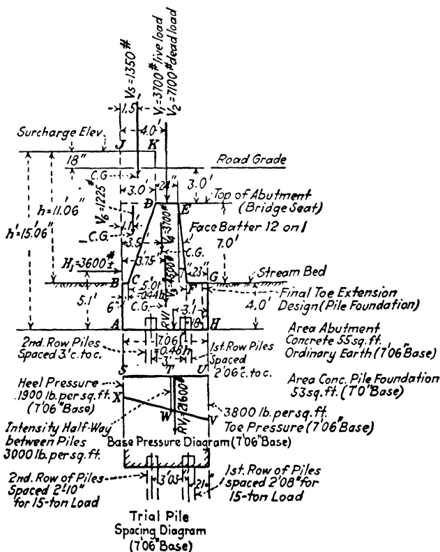
Trial design bridge 2, Road 191, New York State.
