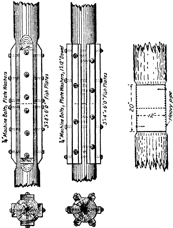
FIG. 357.—Pile splices.
