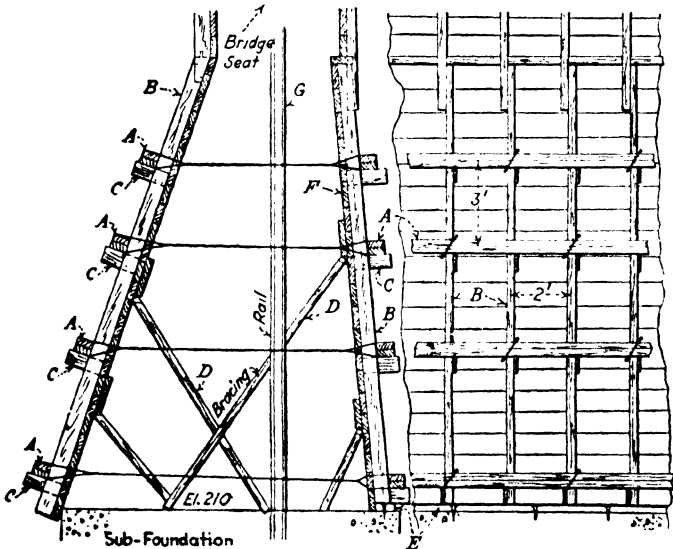
FIG. 353.—Typical form. High abutment Ry. elimination project. New York State.
