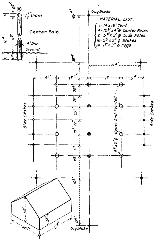
FIG. 285.—Layout diagram.
