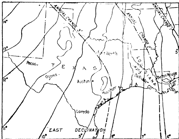
FIG. 266.—Magnetic declinations (1915).—(Continued.)
