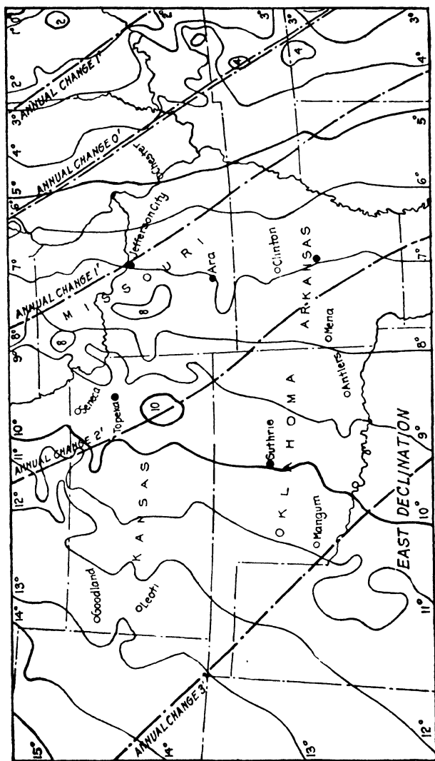
FIG. 266.—Magnetic declinations (1915).—(Continued.)
