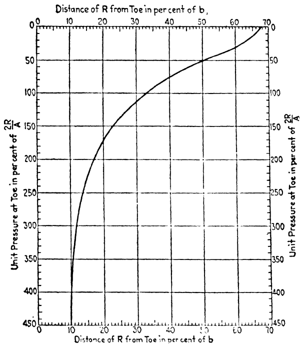
Base pressure distribution. (Toe pressures.)
