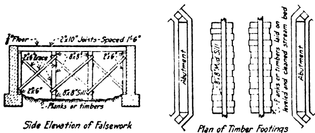
FIG. 348B.—Falsework for small concrete bridges.*
