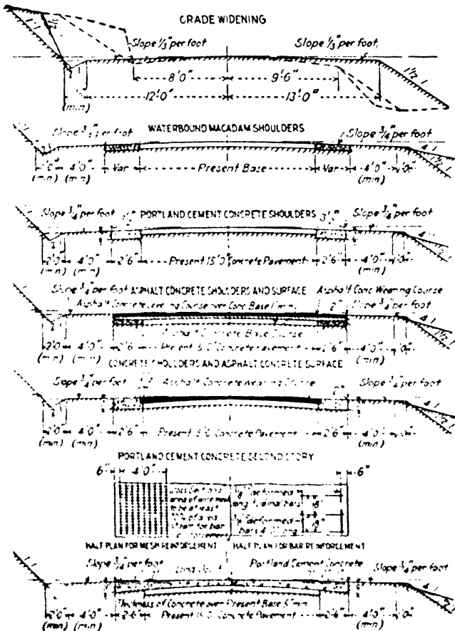
FIG. 308D.—Reconstruction sections, state of California 1926. Widening and thickening old state roads.
