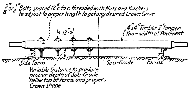
Sub-grade tester.
