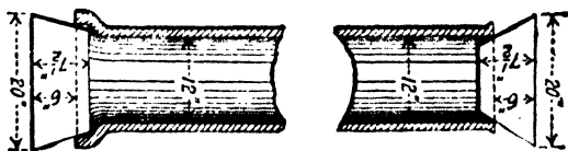
FIG. 333.—Headwall plug extension forms.
