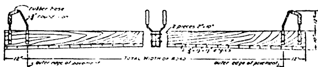
FIG. 339.—Screed strike board.
