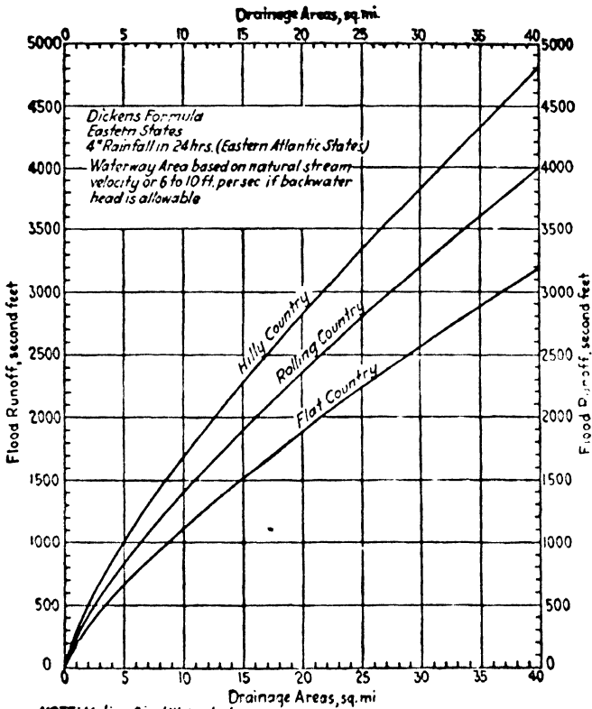
DIAGRAM 2.—Flood runoff for streams. Medium size watersheds. N. Eastern States.
