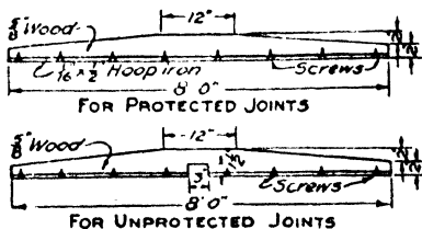
FIG. 343.—Testing straight edge.
