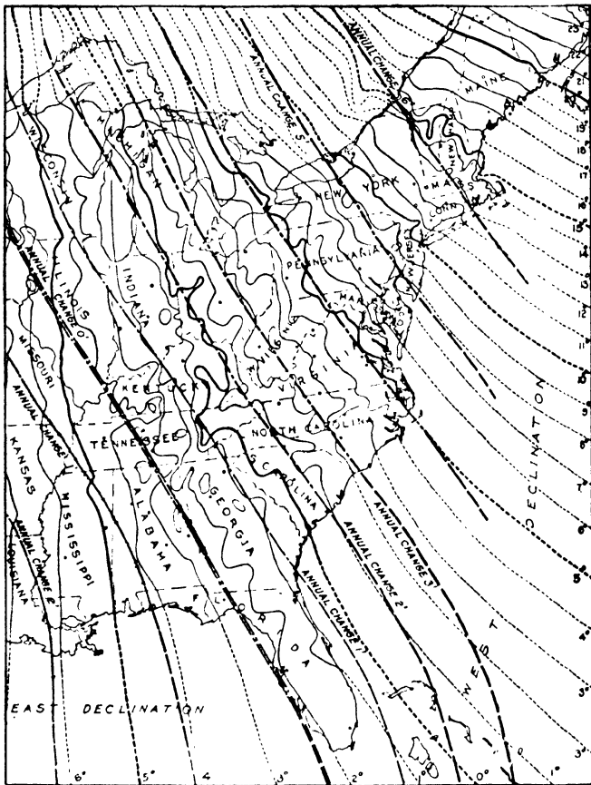
FIG. 266.—Magnetic declinations (1915).—(Continued.)
