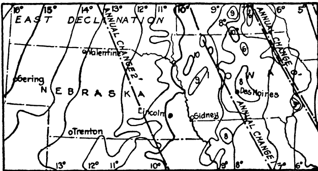
FIG. 266.—Magnetic declinations (1915).—(Continued.)
