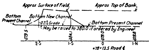
New Channel Profile
