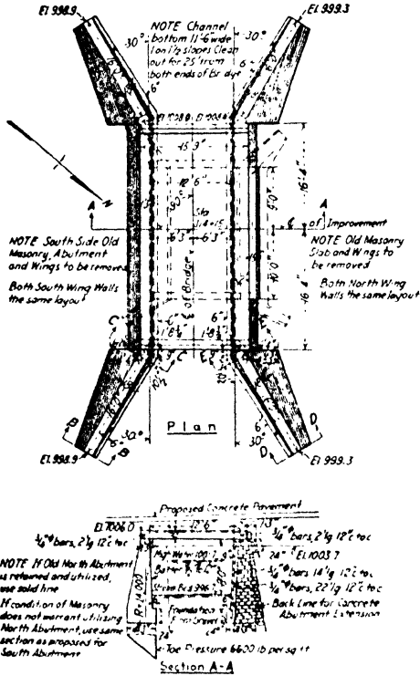
FIG. D.—Utilization of old structures, Case 3. Face and extend one abutment.
