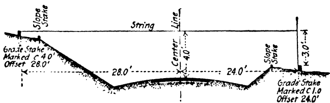
FIG. 330.—Showing suggested method of staking out.
