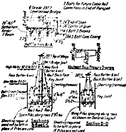
Typical plans (4). Bridge details.
