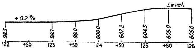
FIG. 313A. - Actual profile road 5046 New York State, illustrating maximum abutness in short roll which is satisfactory for traffic.
