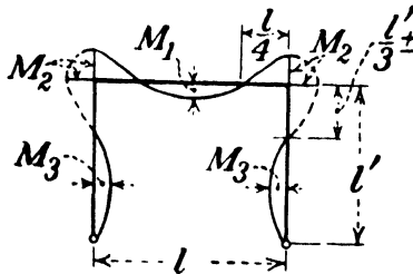
Approximate moment diagram.
