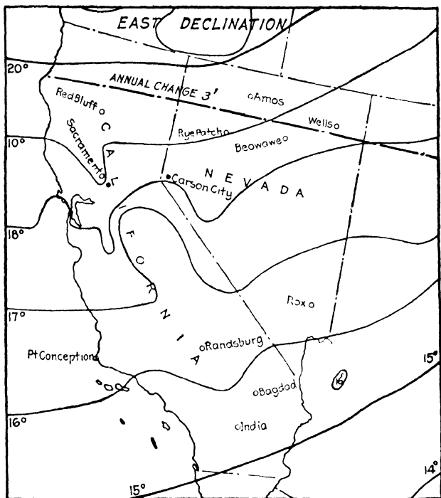
FIG. 266.—Magnetic declinations (1915).—(Continued.)
