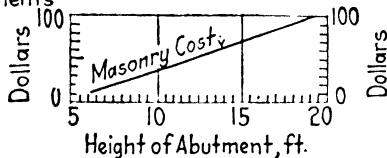
FIG. 260.—Approx. cost curves. Abutment masonry for slab type bridges. Spans 6' to 25' (unit price of concrete $18 per c.y.).
