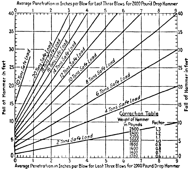
FIG. 346A.—Safe pile loads drop hammer test with free fall. (Shear release.) Use 80% of safe loads for drop hammer with usual cable and drum rig.
