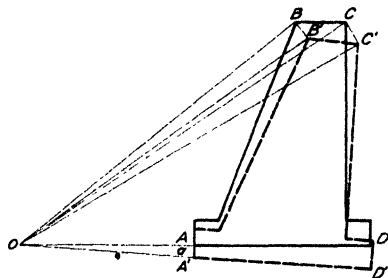
FIG. 225.—Movement of a structure caused by settlement.
