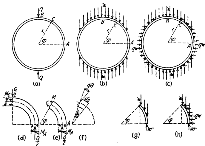
FIG. 168.—Stresses in a pipe conduit due to external loads.
