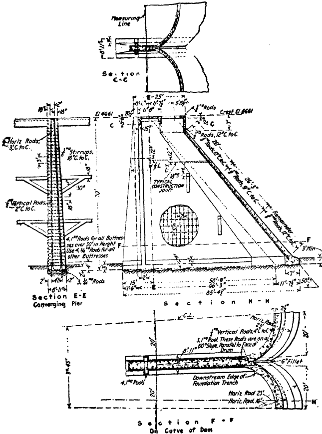
FIG. 91.—Details of Lake Eleanor multiple arch dam.
