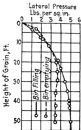
FIG. 179.—Observed lateral pressures of wheat in a bin.
