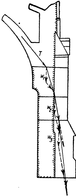
FIG. 10.—Line of thrust in a buttressed wall.
