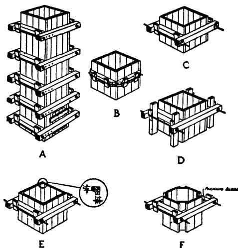
FIG. 197.—Typical column forms.
