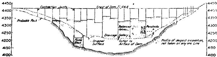
FIG. 83.—Contraction joints in Elephant Butte dam.
