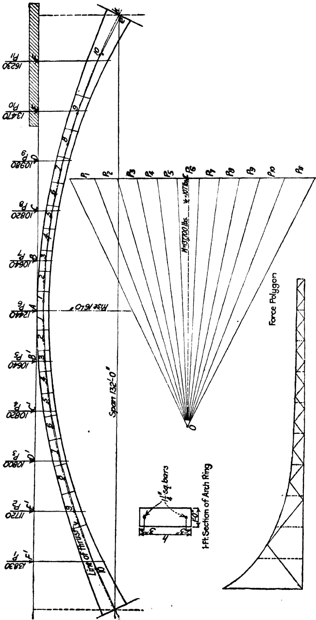
FIG. 45.—Stress analysis of a masonry arch.
