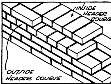
FIG. 7(b).—Manner of laying brick with common bond.
