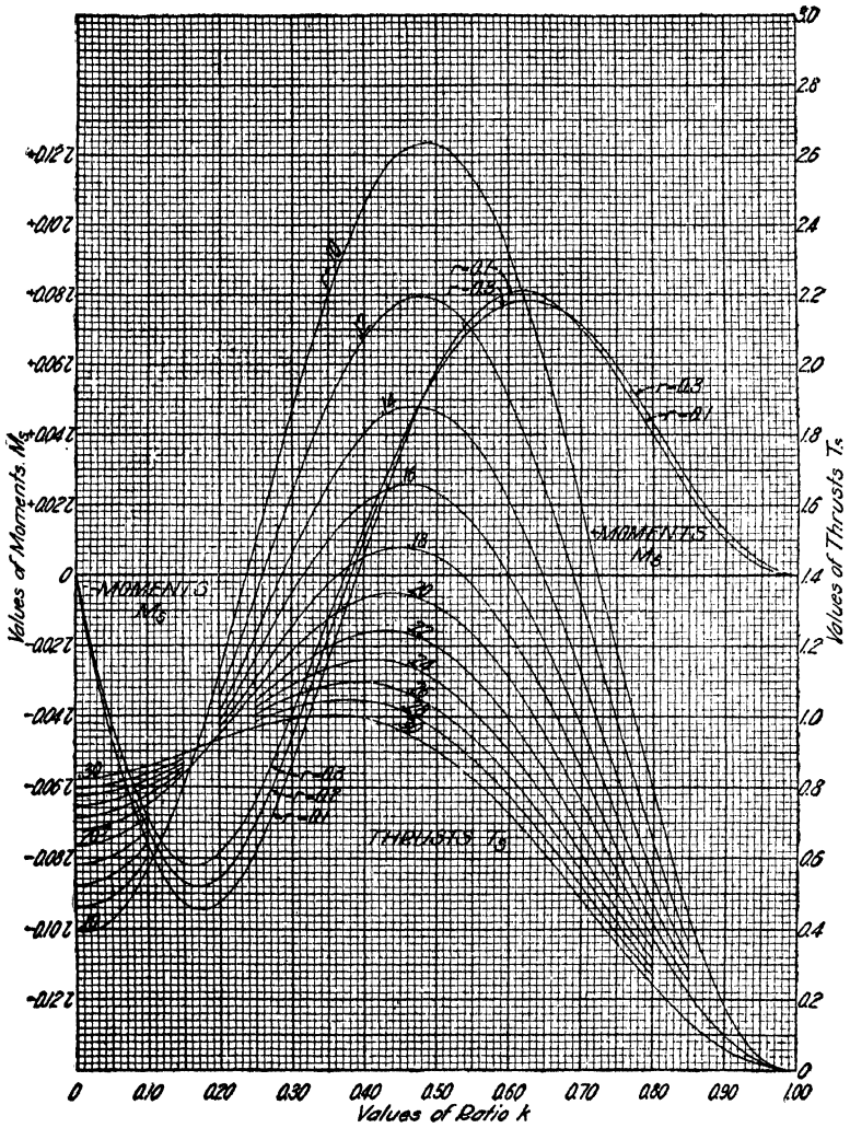
FIG. 52.—Influence lines for moments and thrusts at springing; open spandrel arch, type A_{2,0} .
