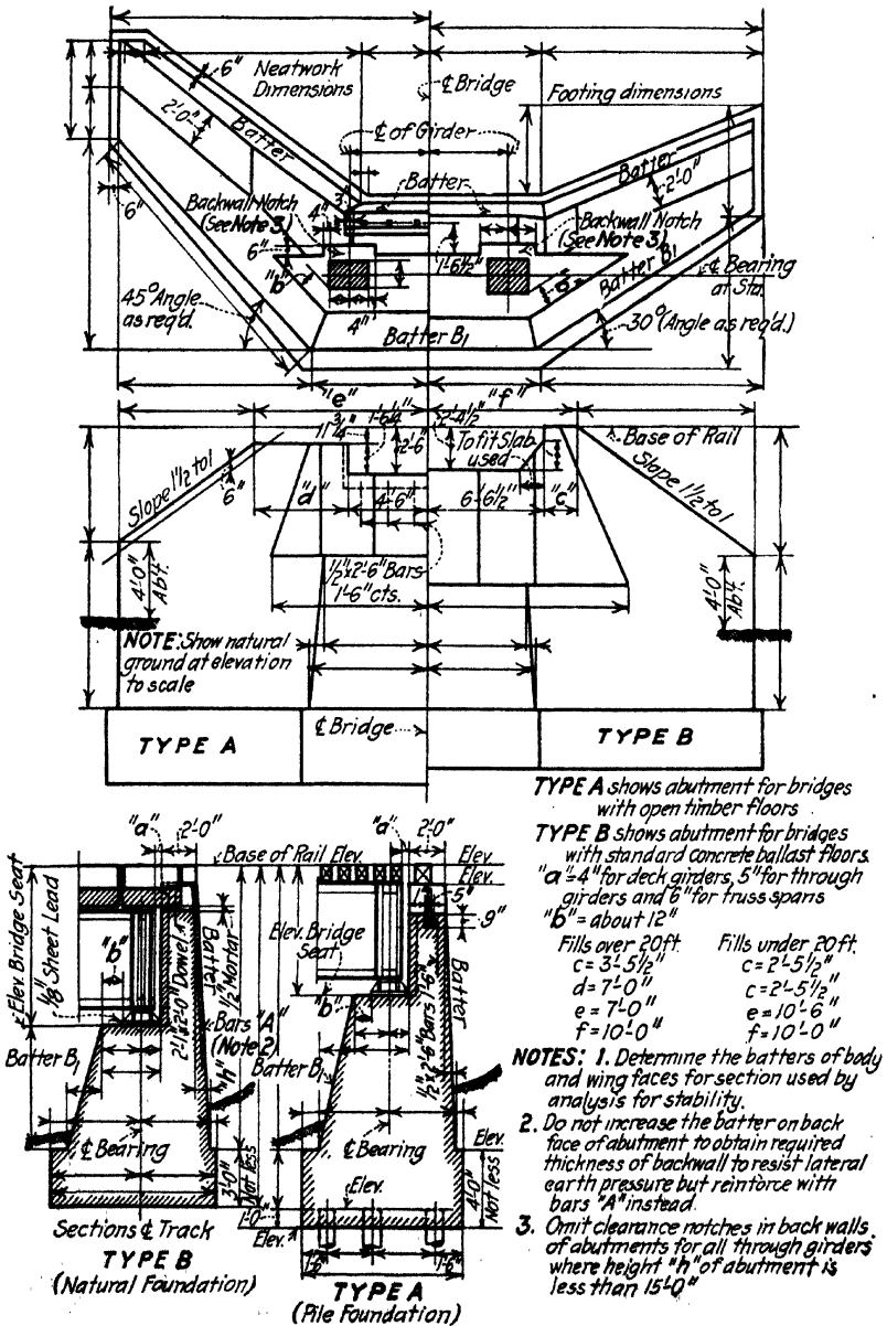
FIG. 128.—Standard bridge abutment of C. M. & St. P. Ry.
