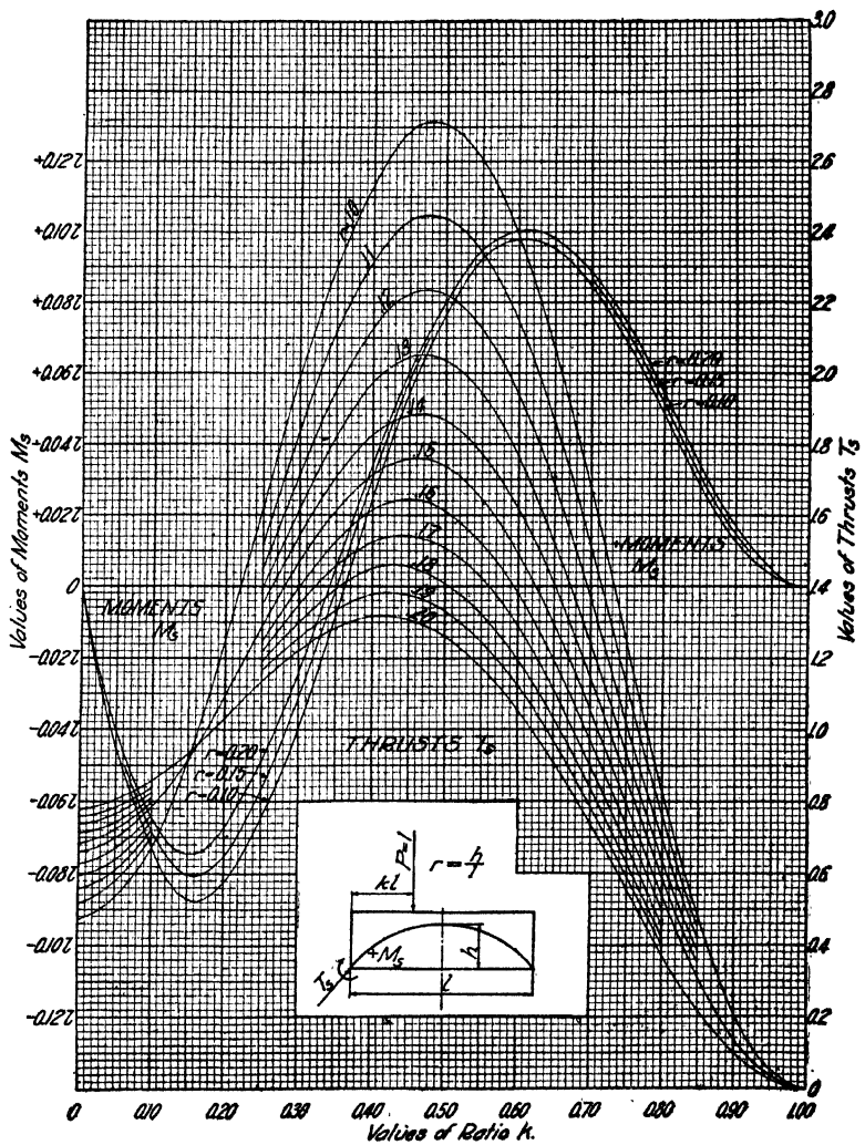
FIG. 55.—Influence lines for moments and thrusts at springing; filled spandrel arch, type A 2.0 .
