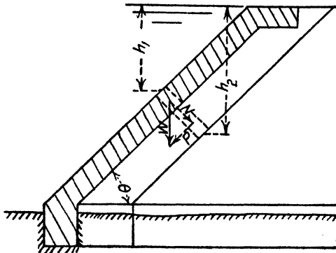
FIG. 90.—Stress distribution in a multiple arch dam.
