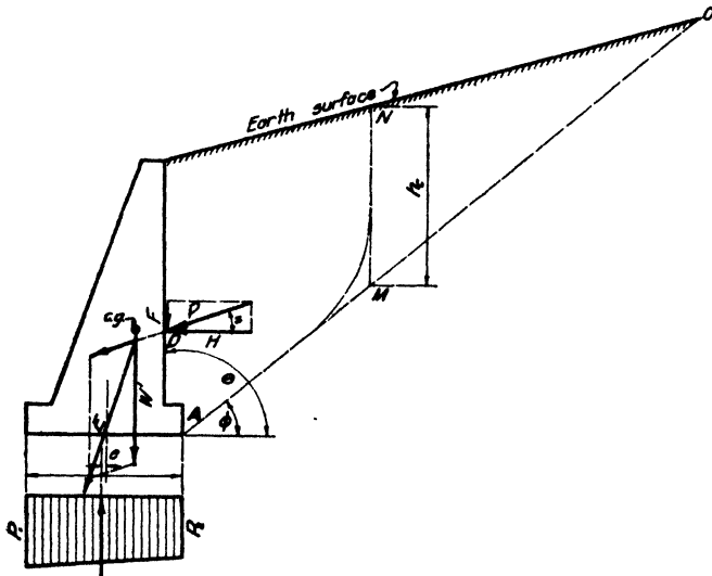
FIG. 99.—Forces acting on a retaining wall.
