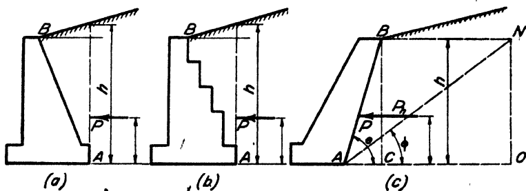
FIG. 102.—Effect of sloping back.
