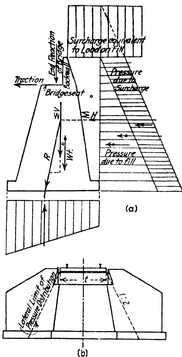
FIG. 118.—Forces acting on a bridge abutment.
