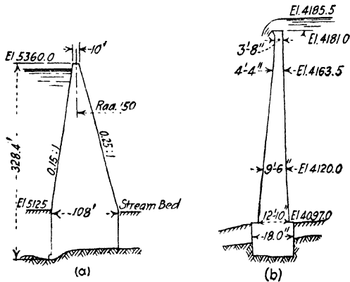
FIG. 86.—Sections of arch dams (a) Shoshone, (b) Huacal.
