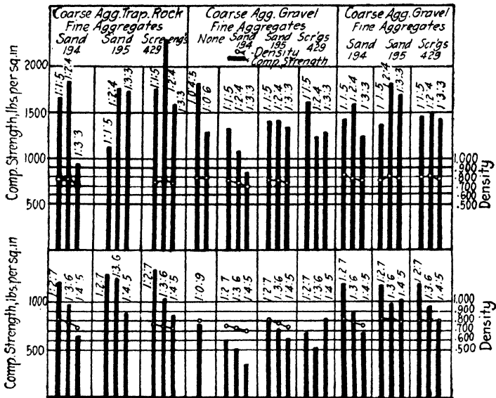
FIG. 15.—Relation between strength and density of concrete.
