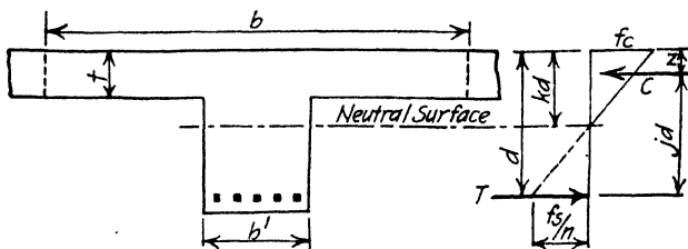
FIG. 29.—Stress distribution in a T-beam.
