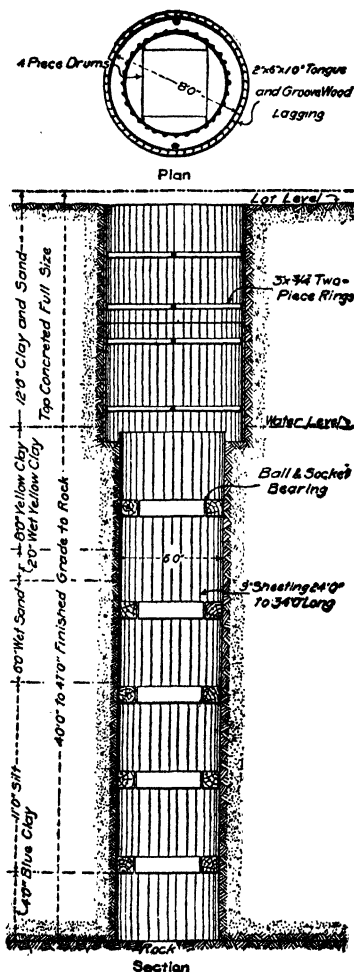
FIG. 232.—Open well for pier under the Railway Exchange Building, St. Louis.
