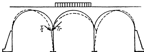
Fig. 57. Deformation of arches with elastic piers.
