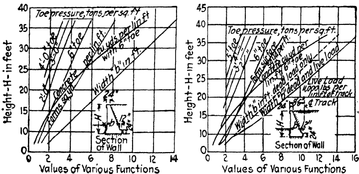
FIG. 105.—Chart for preliminary design of gravity retaining walls.
