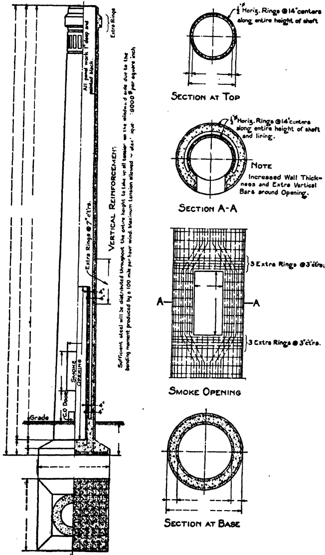
FIG. 195.—Reinforced concrete chimney built by the Weber Chimney Co.
