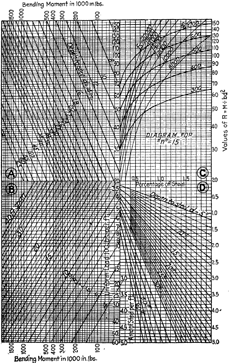
Fig. 35.—Diagrams for design of reinforced concrete beams.
