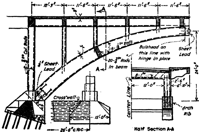
FIG. 162.—Three-hinged reinforced concrete arch.
