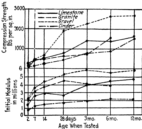
FIG. 22.—Effect of age on the properties of concrete.
