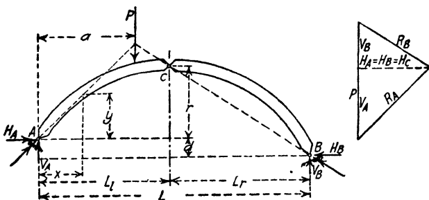
FIG. 160.—Reactions for a three-hinged arch.
