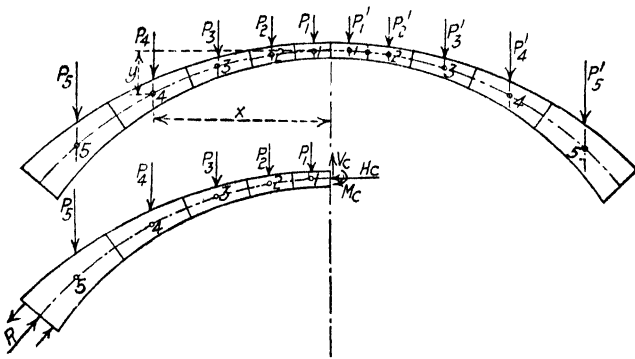
FIG. 41. Loads and forces on an elastic arch ring.
