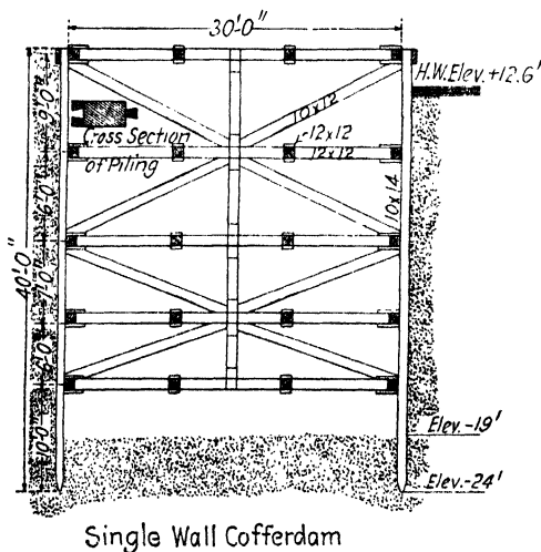
FIG. 241.—Internal traming of a timber cofferdam.
