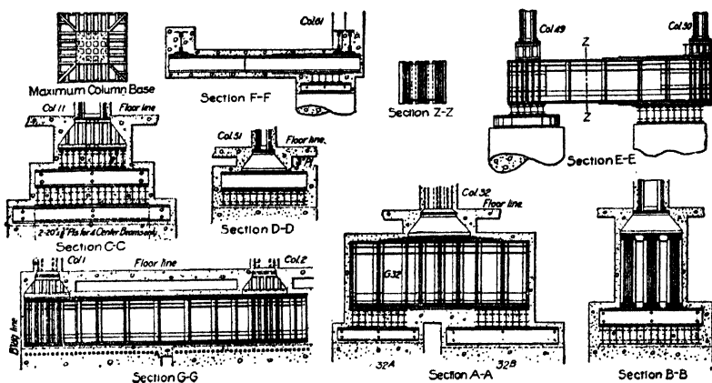
FIG. 227(b).—Grillage foundation of the Woolworth Building, New York.
