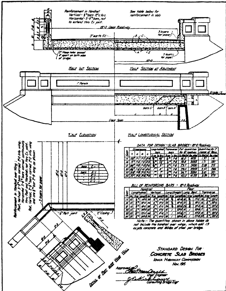
FIG. 153.—Reinforced concrete slab bridge of the Iowa Highway Commission.
