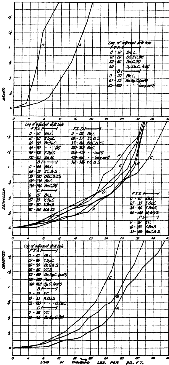
FIG. 224(a).—Test graphs of various soils.
