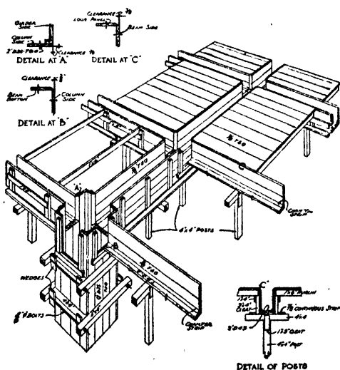
FIG. 199.—Beam and girder forms, bottom detached.
