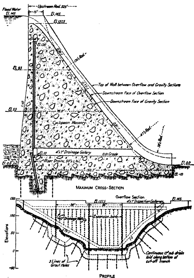
Fig. 77.—Section of the lower Otay dam (proposed).
