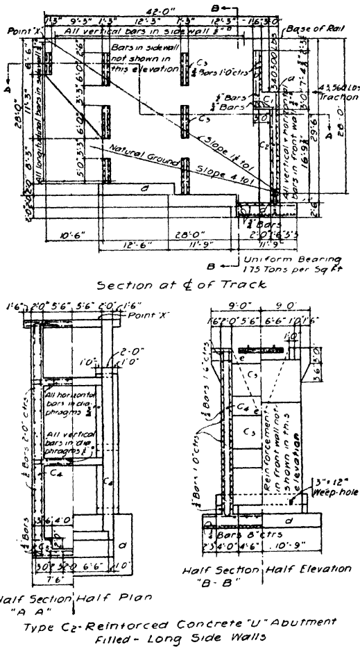
FIG. 123.—Details of a reinforced concrete U-abutment, C. M. & St. P. Ry.
