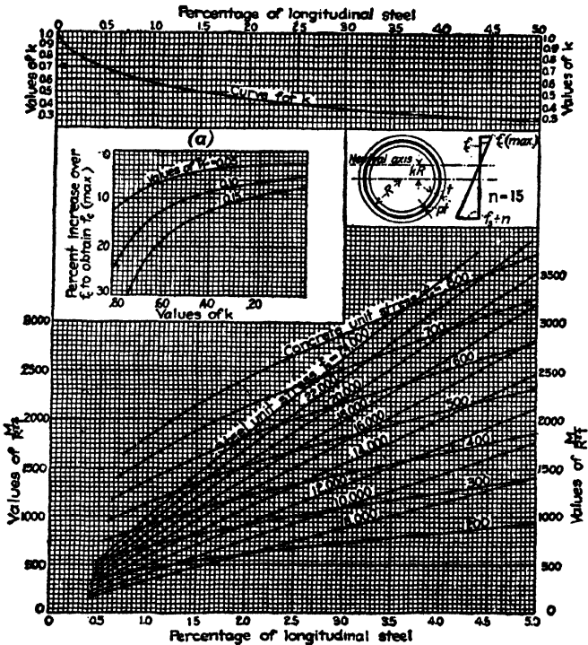
Fig. 192.—Diagram for designing a reinforced concrete chimney.
