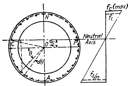
FIG. 191.—Stresses in a reinforced concrete chimney.
