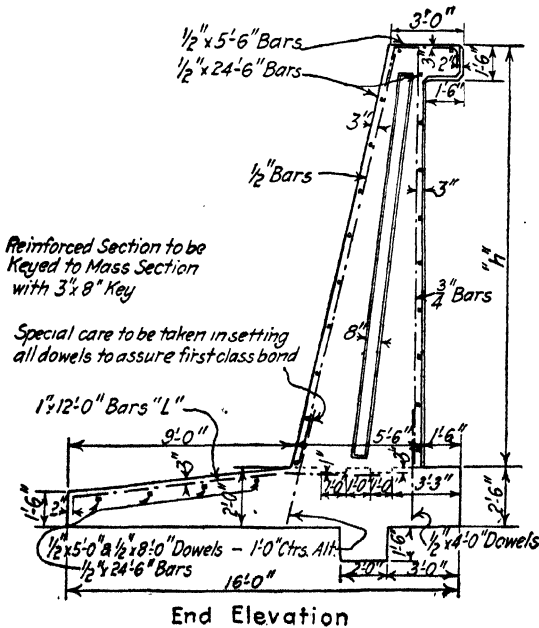
FIG. 116.—Compromise section of a retaining wall of the C. M. & St. P. Ry.
