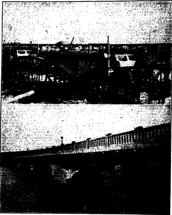
FIG. 164.—Platte river bridge at Douglas, Wyoming.
