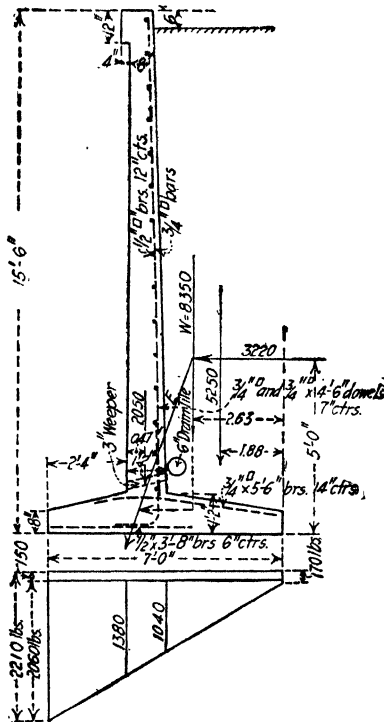
FIG. 106.—Section of a cantilever retaining wall.
