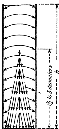
FIG. 175.—Distribution of pressure in a deep bin.
