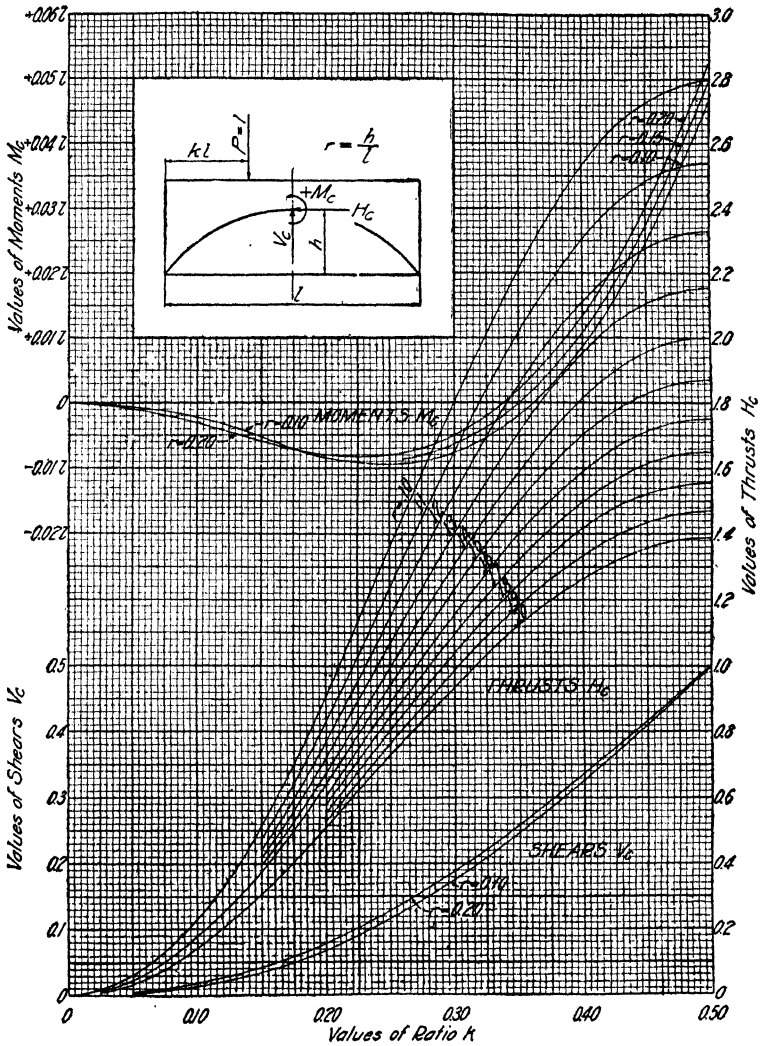
FIG. 54.—Influence lines for moments, thrusts and shears at crown; filled spandrel arch, type A 2.0 .
