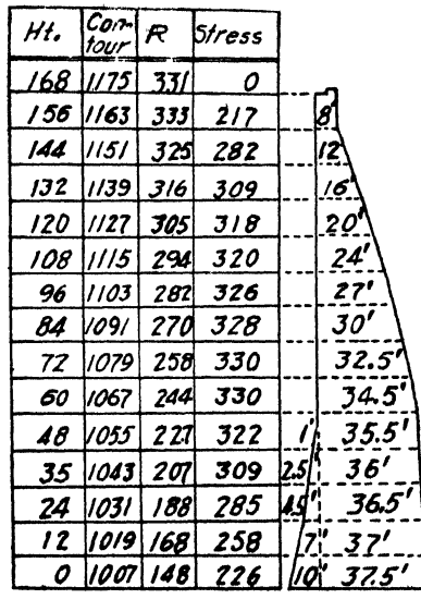
FIG. 88.—Section of Salmon River constant angle arch dam.
