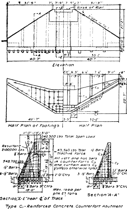
FIG. 122.—Details of a counterfort abutment, C. M. & St. P. Ry.
