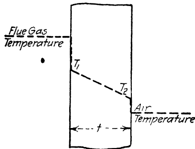
FIG. 188.—Temperature drop in a chimney wall.
