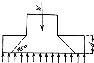
FIG. 226(b).—Diagram of column footing.
