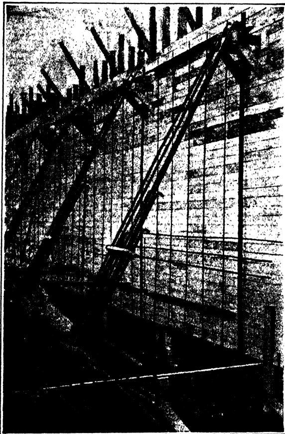
FIG. 108.—Reinforcement in counterfort retaining wall.
