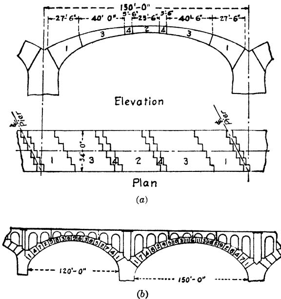
FIG. 61.—Order of placing masonry in arch rings.
