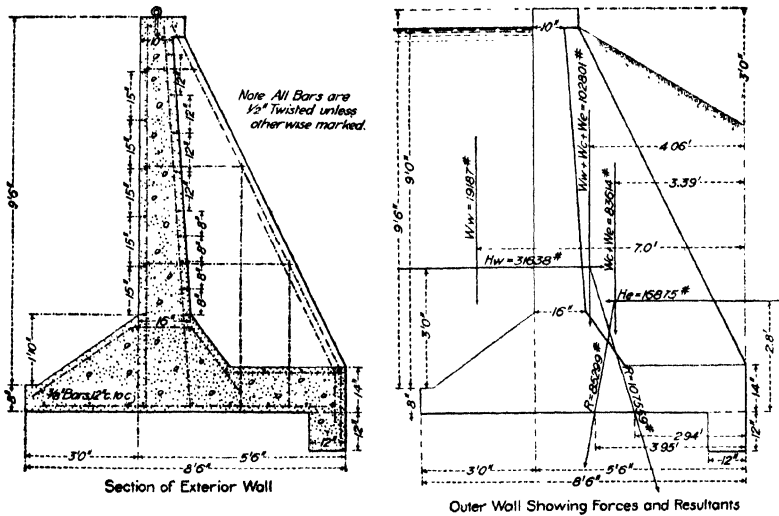
FIG. 112.—Section of reservoir wall at Webb City, Mo.
