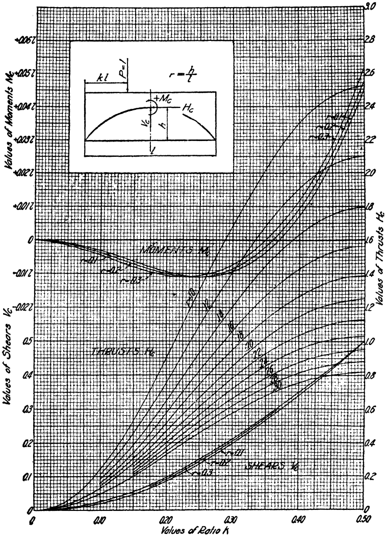
FIG. 48.—Influence lines for moments, thrusts and shears at crown; open spandrel arch, type A_{1.5} .
