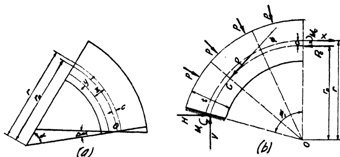
FIG. 85.—Elementary section of an arch dam.
