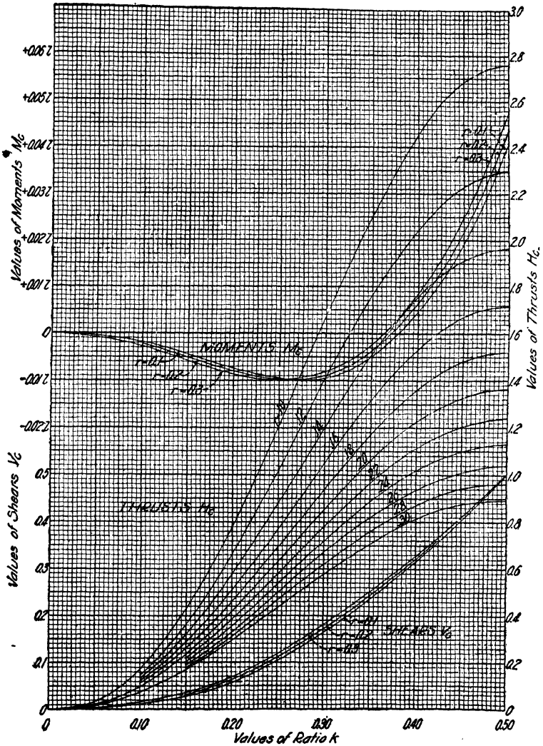
FIG. 50.—Influence lines for moments, thrusts and shears at the crown; open spandrel arch, type A 2.6 .
