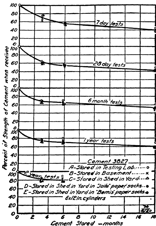
FIG. 11.—Effect of storage of cement on the strength of concrete.
