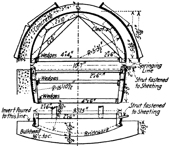
FIG. 204.—Forms for a large concrete sewer.
