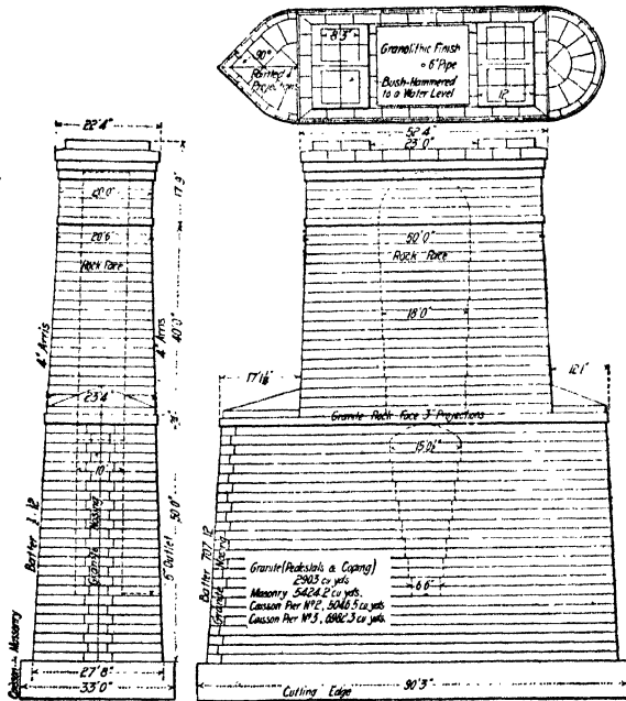
FIG. 137.—Hollow pier of the municipal bridge of St. Louis.
