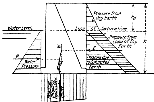
FIG. 110.—Forces acting on a quay wall.
