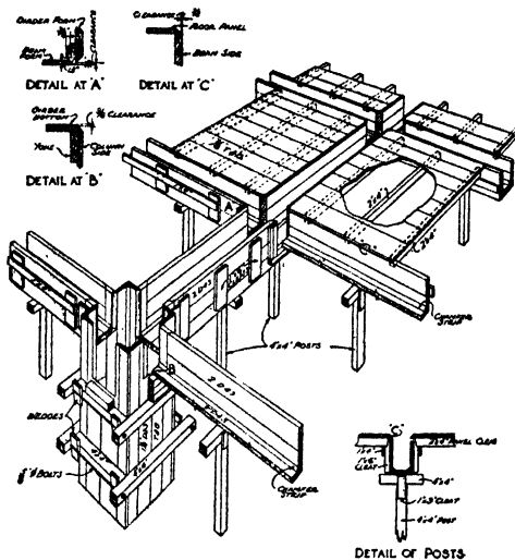
FIG. 198.—Beam and girder forms, bottom attached.
