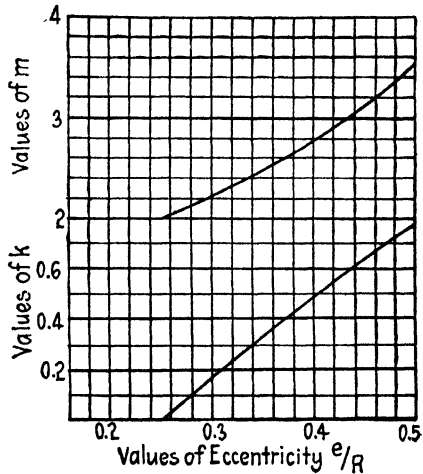
FIG. 194.—Diagram for calculating soil pressure under a chimney.
