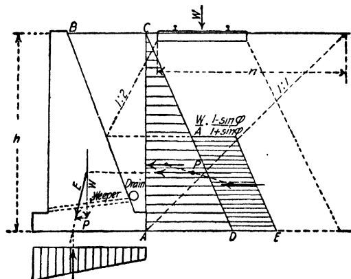
FIG. 103.—Pressure on a retaining wall due to loaded fill.
