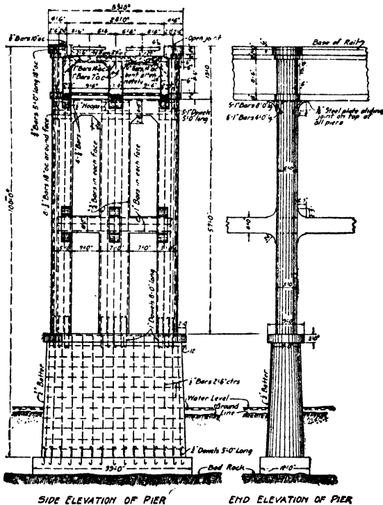
FIG. 138.—Divided reinforced concrete pier.
