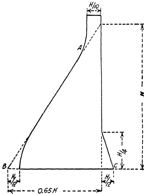
FIG. 78.—Approximate section for a gravity dam.
