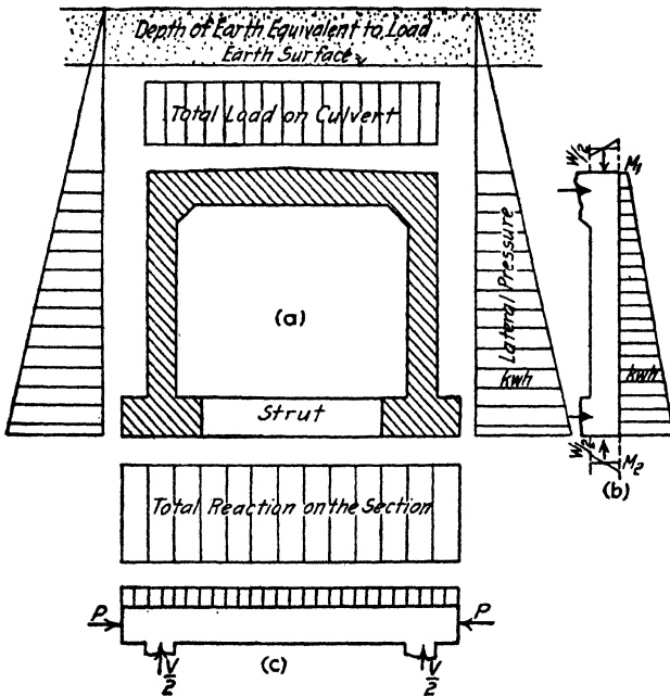
FIG. 166.—Forces acting on a rectangular culvert.
