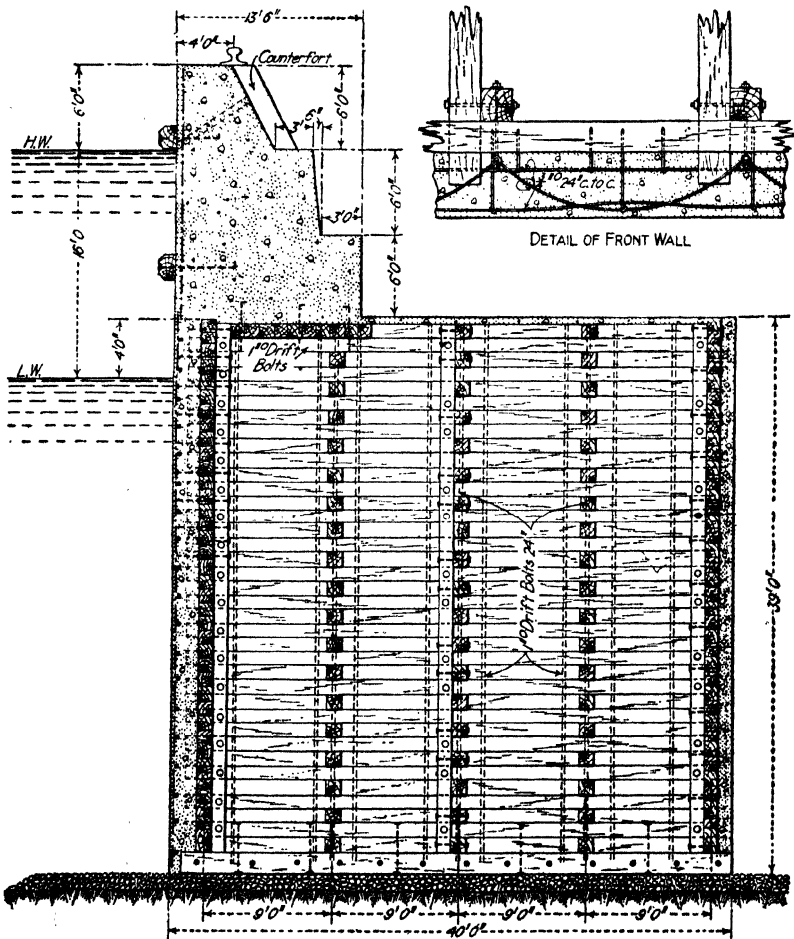
FIG. 111.—Section of Vancouver dock wall.
