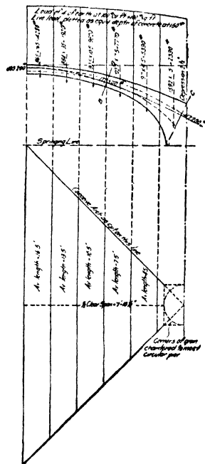
FIG. 70(b).—Stresses in a groined arch.
