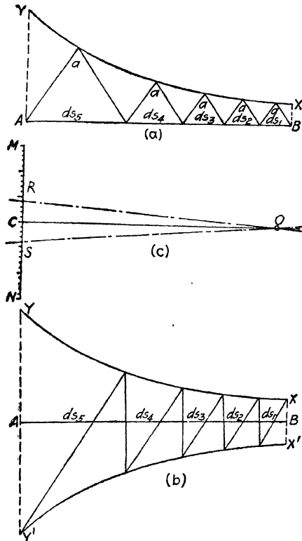
FIG. 43.—Dividing an arch ring by graphical methods to make \frac{ds}{I} constant.
