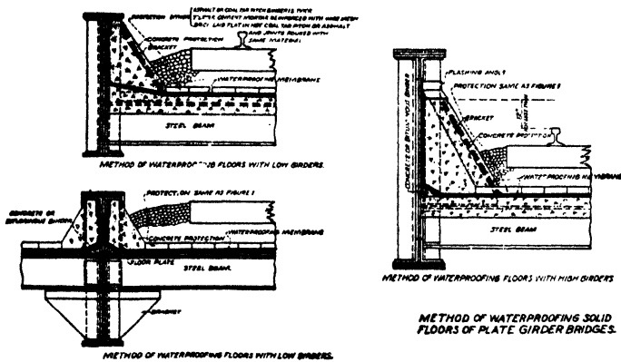
Fig. 165.—Methods of water-proofing bridge floors.
