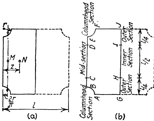
FIG. 34.—Diagram of a flat slab panel.
