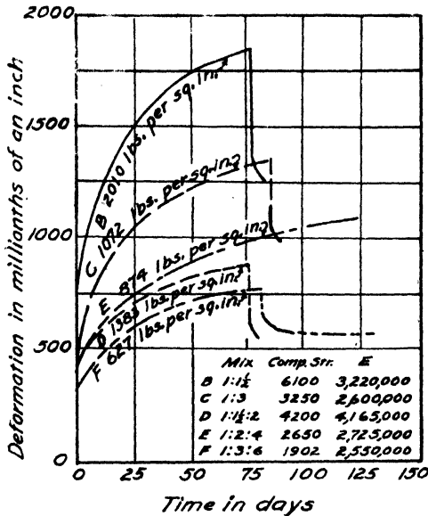
FIG. 25.—Plastic flow of concrete under stress.
