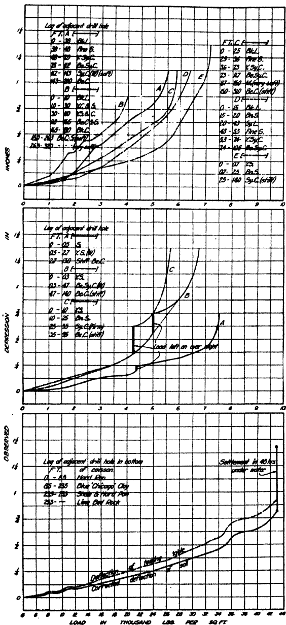
FIG. 224(b).—Test graphs of various soils.
