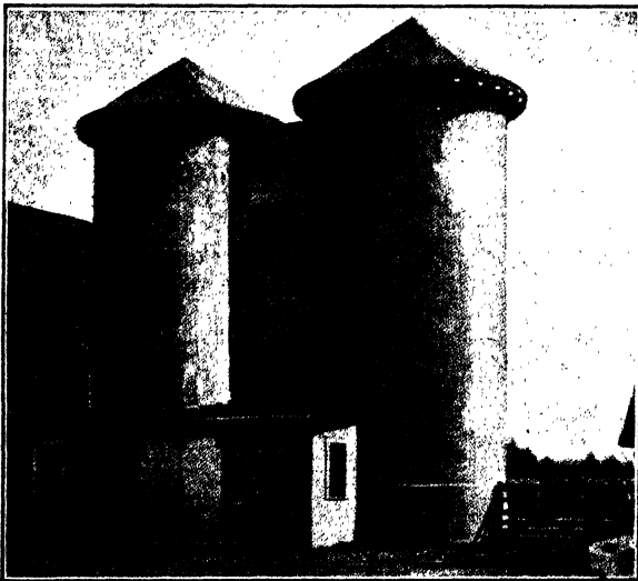
FIG. 187.—Reinforced concrete twin silos.
