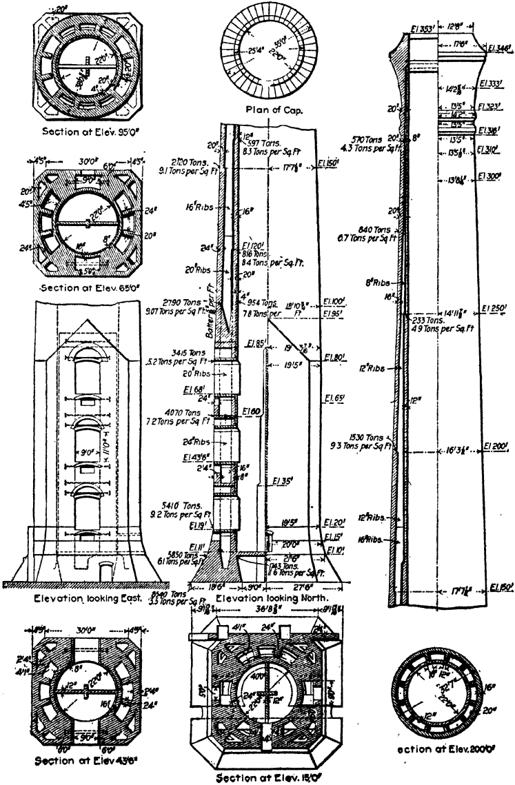
FIG. 189.—Details of a chimney of common brick.
