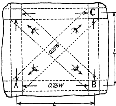
FIG. 70(a).—Assumed stress distribution in a groined arch.
