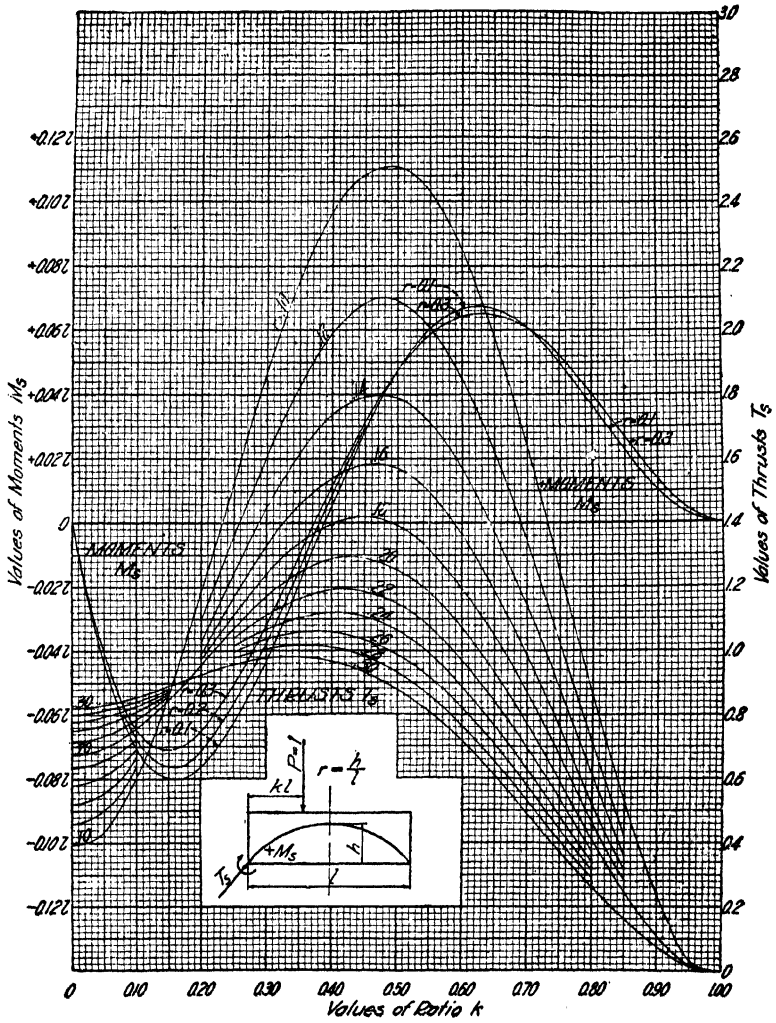
FIG. 51.—Influence lines for moments and thrusts at springing; open spandrel arch, type A1.5.
