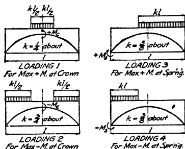
FIG. 39.—Position of live loads for maximum stresses.
