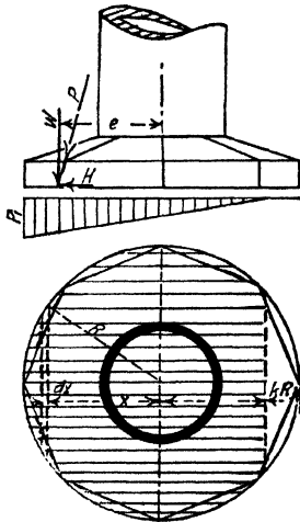
FIG. 193.—Soil pressure under a chimney base.
