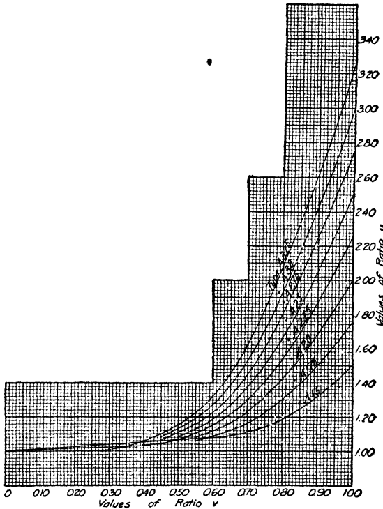
FIG. 38.—Diagram for thickness of typical arch rings.
