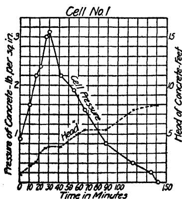
FIG. 196.—Effect of time on the pressure of concrete on forms.
