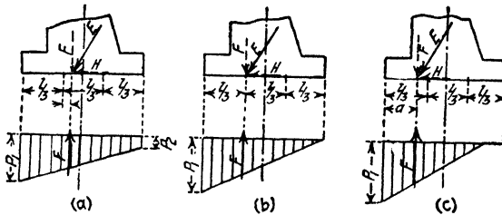
FIG. 104.—Distribution of pressure under a retaining wall.
