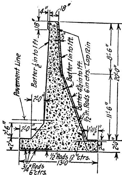
FIG. 115.—Section of a fillet retaining wall.
