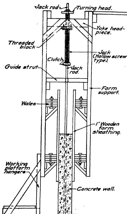
FIG. 206.—Sliding forms for a wall.
