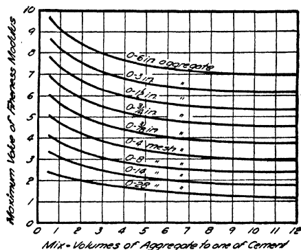
FIG. 21.—Maximum permissible value of fineness modulus.
