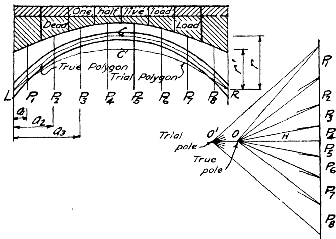
FIG. 36.—Loading and equilibrium polygon for economic arch.
