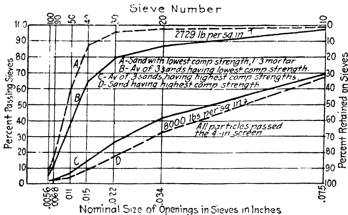
FIG. 12.—Effect of gradation of sand on the strength of mortar.
