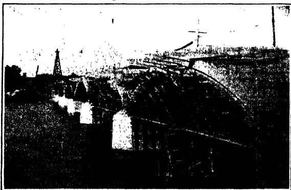
FIG. 211.—Timber centers on steel trusses used in constructing Lawrence, Kansas, bridge.
