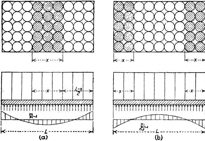
FIG. 184.—Moments in slab under a bin cluster.
