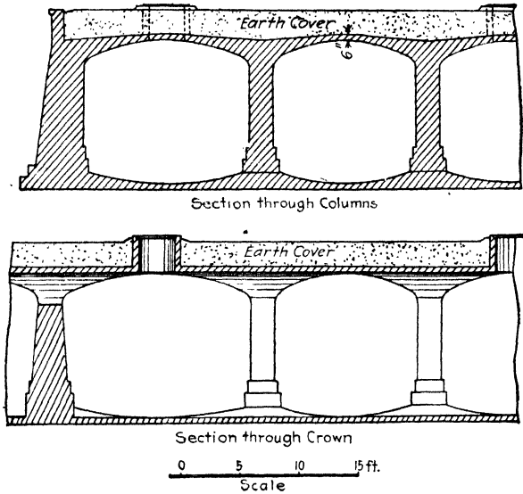
FIG. 71.—Section through groined arches at Washington.
