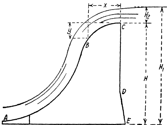
FIG. 73.—Head on an overflow dam.
