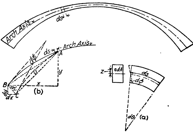
FIG. 40.—Elastic deformation of a curved beam.
