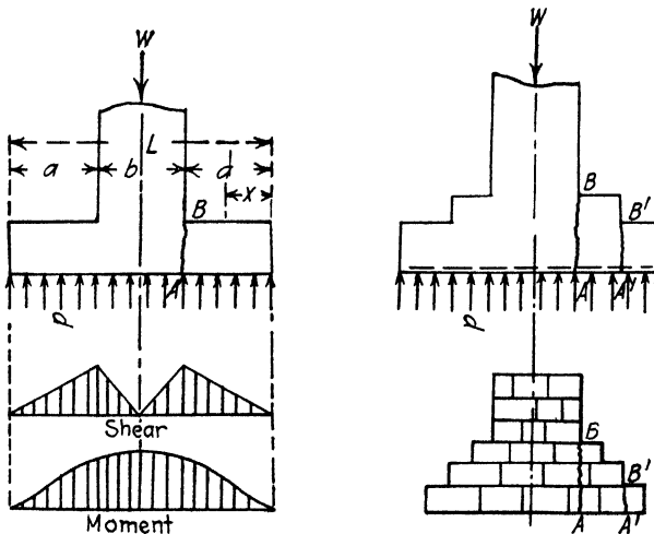
FIG. 226(a).—Diagrams of wall footings.
