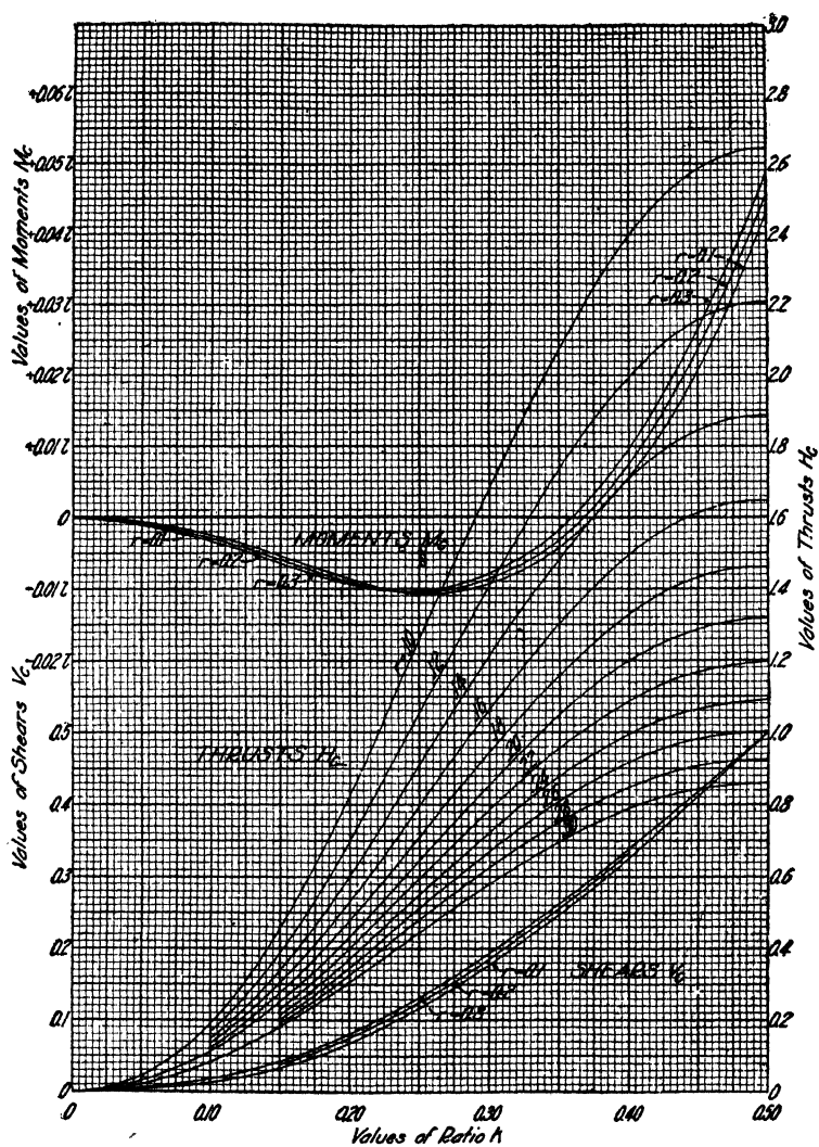
FIG. 49.—Influence lines for moments, thrusts and shears at the crown; open spandrel arch, type A 2.0 .
