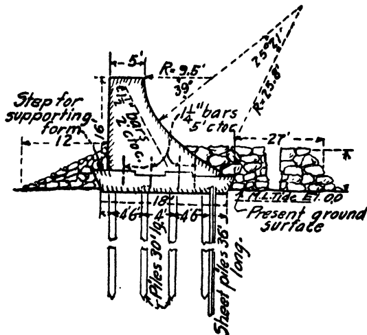
FIG. 98.—Section of sea wall at Galveston.
