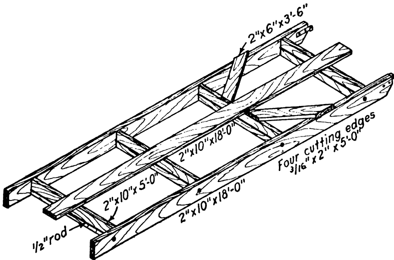
FIG. 61. — Land drag. (New Mexico Ext. Service Circular 92.)
