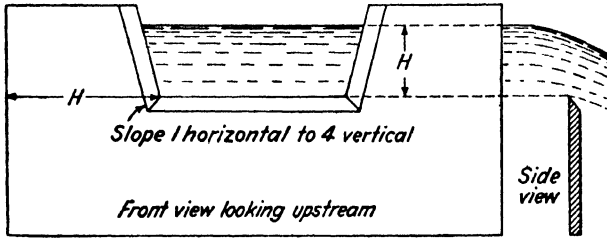
FIG. 15. — A trapezoidal, or Cipolletti weir.
