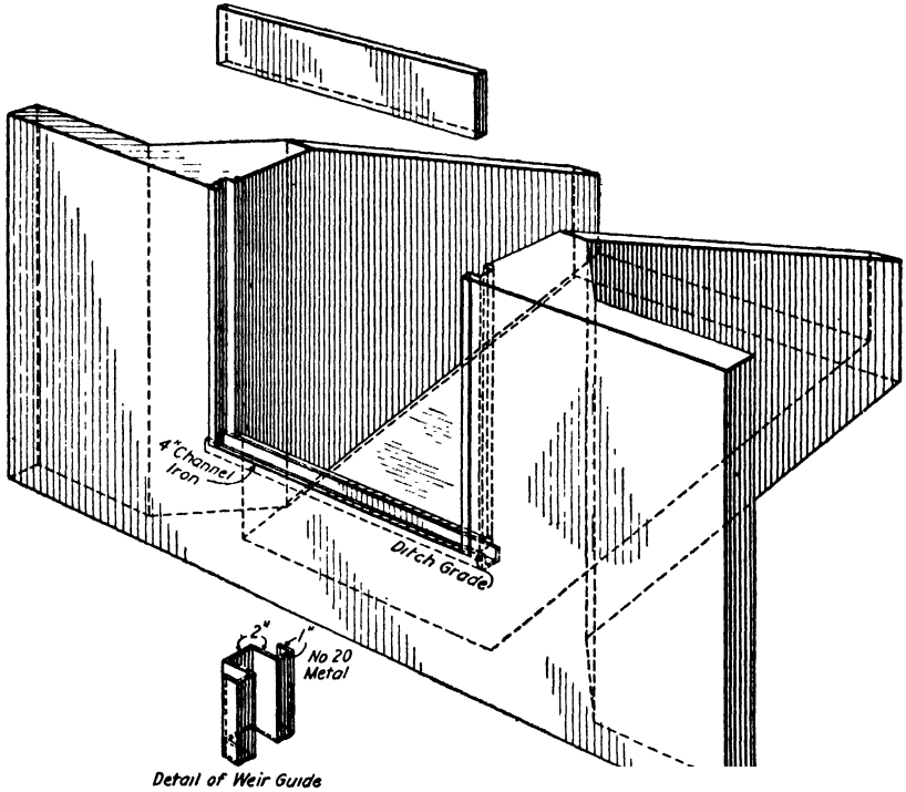
FIG. 75. — Concrete gate and wooden flashboard used on the Turlock Irrigation District. California.
