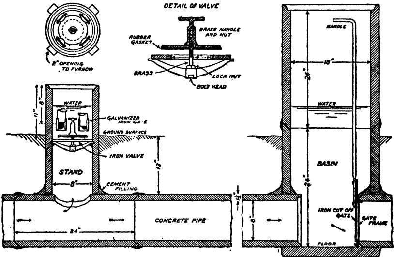
Fig. 163. — Design for concrete pipe and stand system for orchard irrigation. (U. S. Dept. Agr. Farmers' Bul. 882.)
