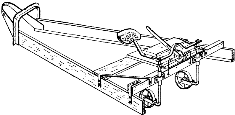
FIG. 67. — Bordering machine as designed and used in Salt River Valley, Arizona.
