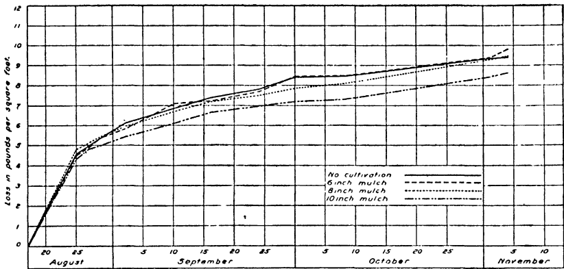
FIG. 108. — Loss of water by evaporation directly from the surface of bare soils in tanks at Mountain View. (Calif. Agr. Exp. Sta. Hilgardia Vol. II No. 6, 1921.)
