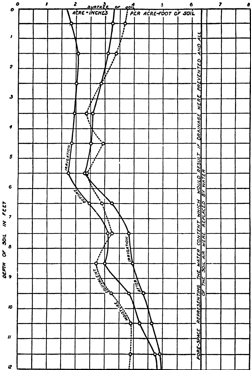
FIG. 98. — Graphs of the water content before and after irrigation, moisture equivalent, and pore space of yolo loam soils. Each water-content curve is the average of 6 plots for 1913, 1914, and 1915, and the average of 147 borings.
