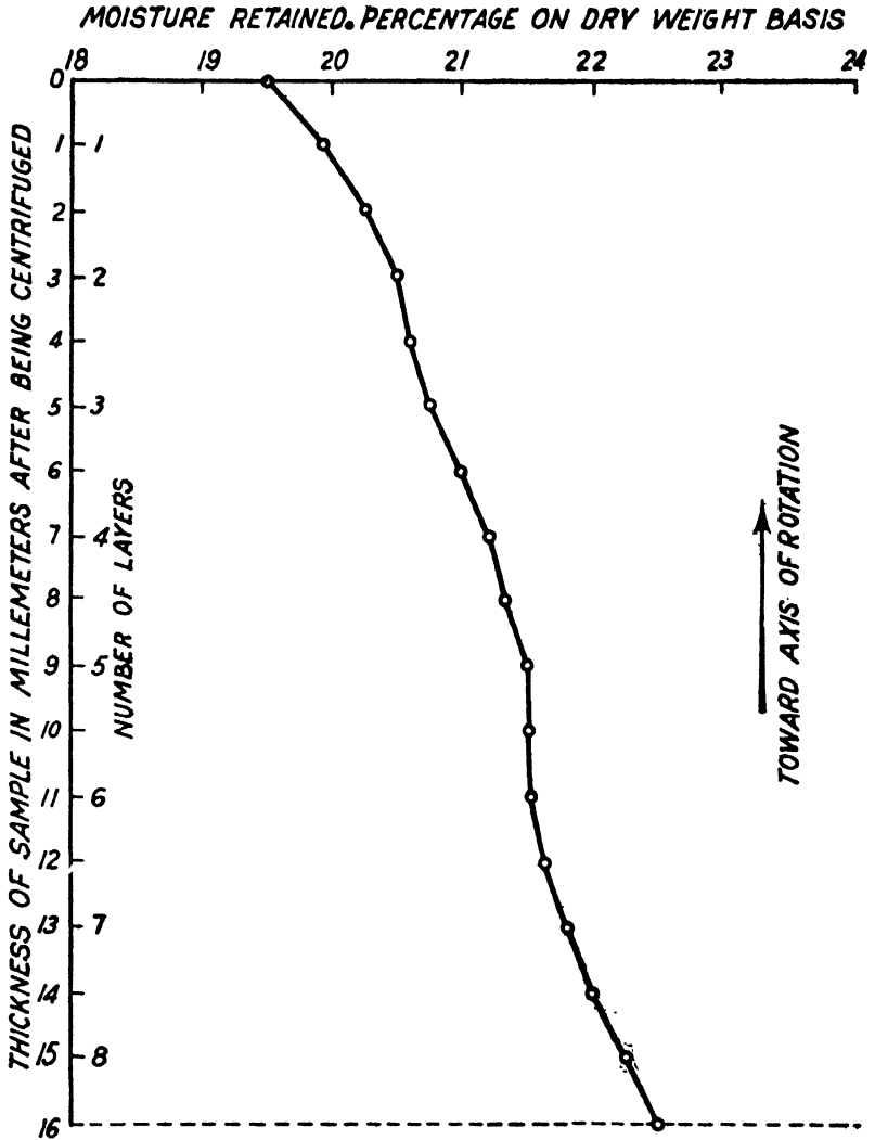
FIG. 86. — Moisture distribution in a 60-gram sample of yolo caly loam soil after being subjected to a centrifugal force of 1000 times gravity for a period of one-half hour. (Calif. Agr. Exp. Sta. Tech. Paper No. 16.)
