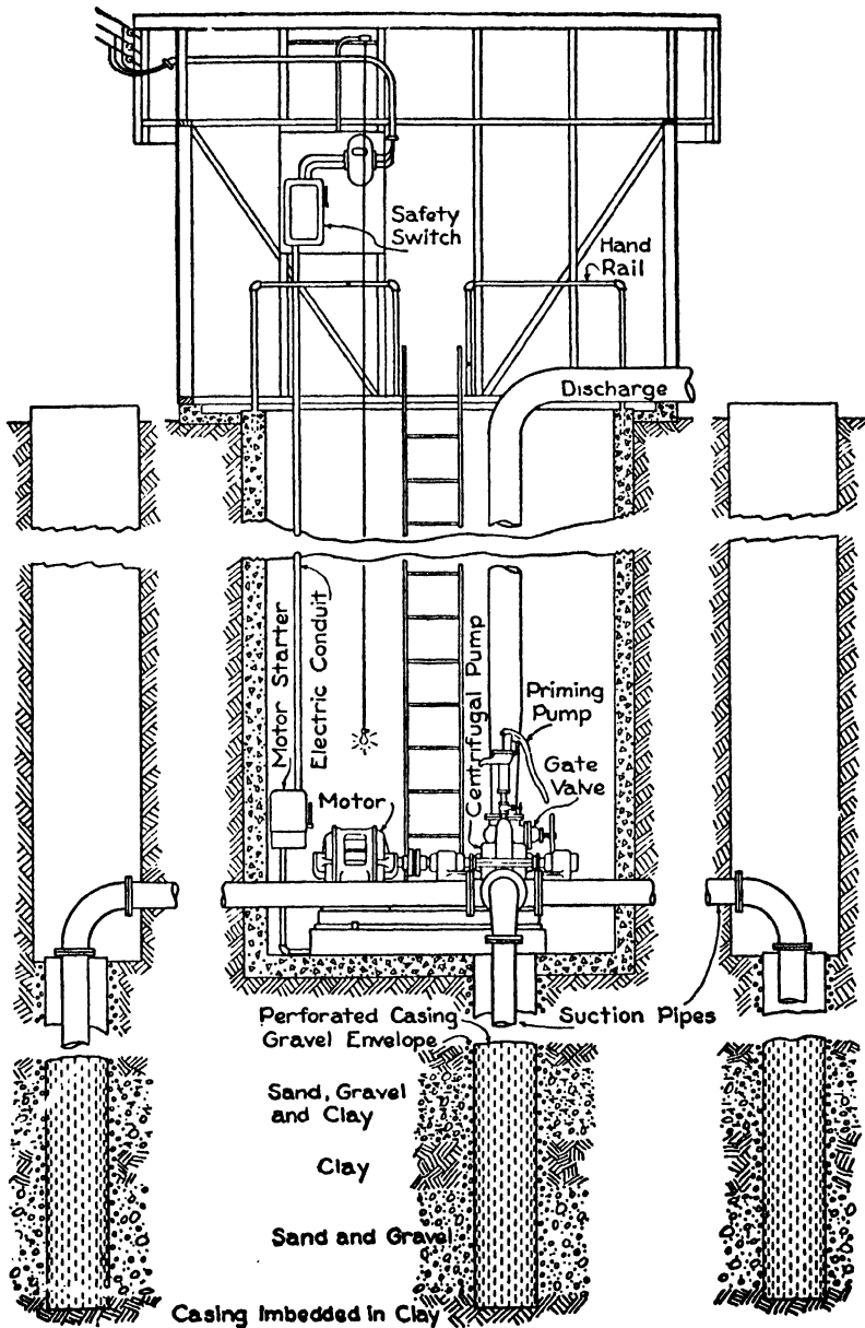
FIG. 44. — A horizontal centrifugal pump direct-connected to an electric motor in a pit, pumping from three wells simultaneously. (Colo. Agr. Exp. Sta. Bul. 350.)
