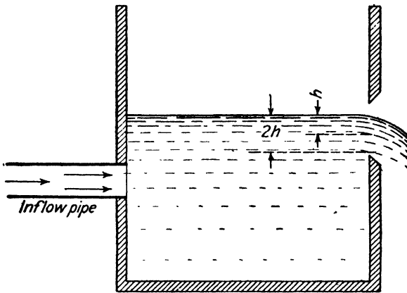
FIG. 13. — Showing that discharge through a partly-filled orifice is similar to the discharge over a weir.
