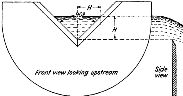
FIG. 16. — A 90°-notch triangular weir.
