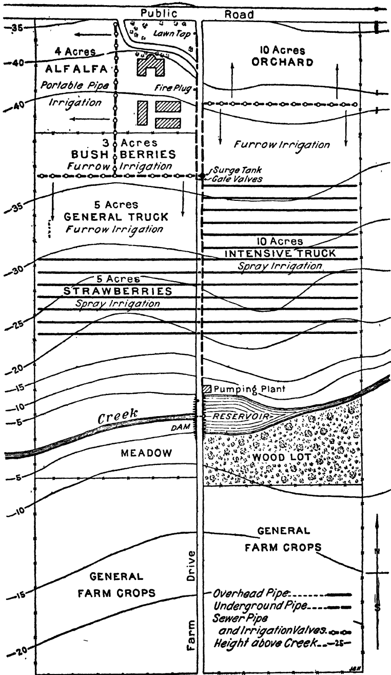
FIG. 174. — Typical 80-acre farm in humid regions, showing development of water supply by reservoir and a combination of spray and surface methods of irrigation and from one pumping plant (U. S. Dept. Agr. Bul. 495.) (387)
