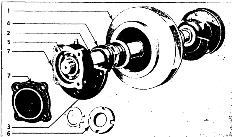
FIG. 36. — Impeller and shaft assembly of pumps showing: (1) enclosed impeller; (2) ground carbon-steel shaft; (3) water seal ring; (4) packing; (5) standard ball bearing; (6) lock nut and (7) ball-bearing housing and cover. (Courtesy: Fairbanks-Morse Company.)
