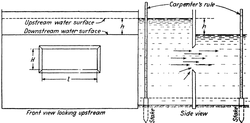
FIG. 17. — Submerged orifice.
