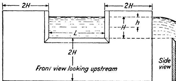
FIG. 14. — A rectangular weir with complete end contractions.
