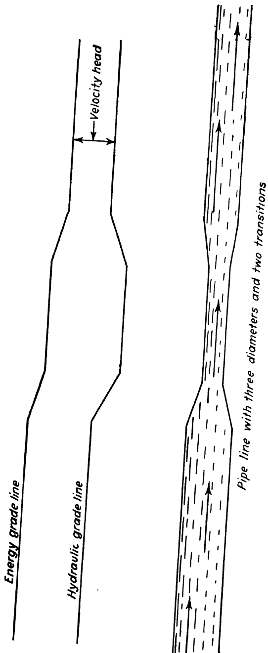
FIG. 10. — Showing that the energy grade line always falls in the direction of flow.
