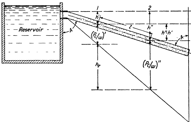
FIG. 107. — Illustrating the capillary flow of water through an inclined pipe, using engineering symbols to represent heads due to position and to capillary pressure.
