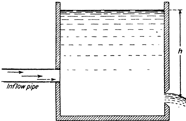
FIG. 12. — Illustrating the discharge of water through an orifice under a head, h .
