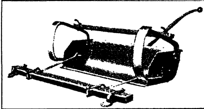
FIG. 62. — Fresno scraper.
