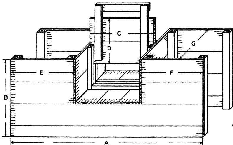
Fig. 73. — Standard single-wing wooden check gate. (Figs. 73 to 76 from U. S. Dept. Agr. Farmers' Bul. 1213.)
