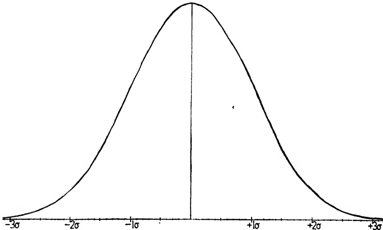
FIG. 153.—Normal curve of variation, with multiples of the standard deviation marked on the base line.
