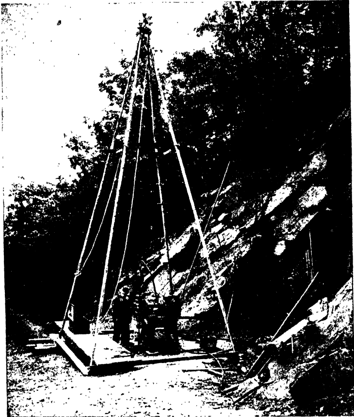
FIG. 8a.—Explorer diamond drill on surface mounting. (Courtesy of Ingersoll-Rand Company.)
