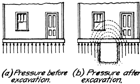
FIG. 2.—Length of arrows indicates relative intensities of soil loads.
