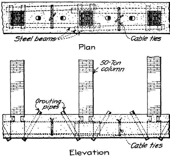
FIG. 8.—Foundation reinforced with grillage for underpinning.
