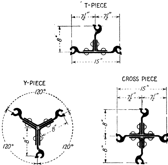
FIG. 52b.—Standard fabricated connections.
