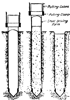
FIG. 45.—Method of constructing Simplex concrete piles.
