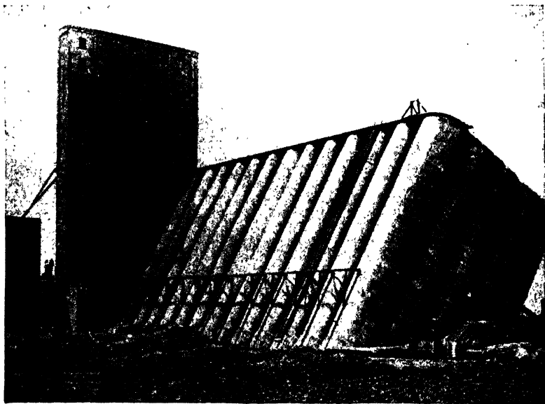
FIG. 18.—Winnipeg grain elevator after foundation failure. (Courtesy of Foundation Company.)
