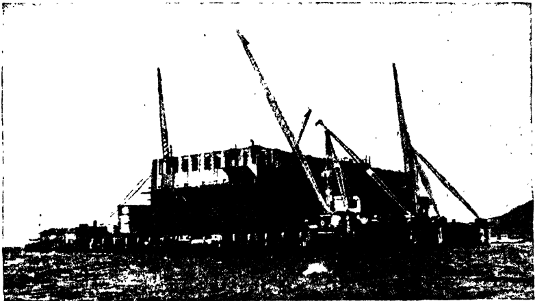
FIG. 18.—Caisson for San Francisco-Oakland Bay Bridge pier.
