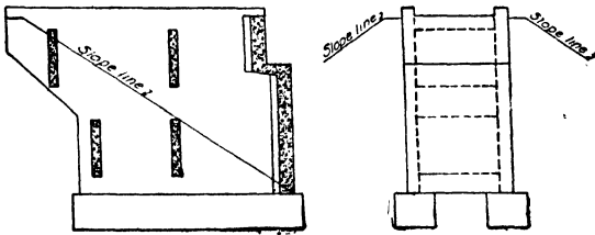
FIG. 11.—Hollow U abutment, cellular type.
