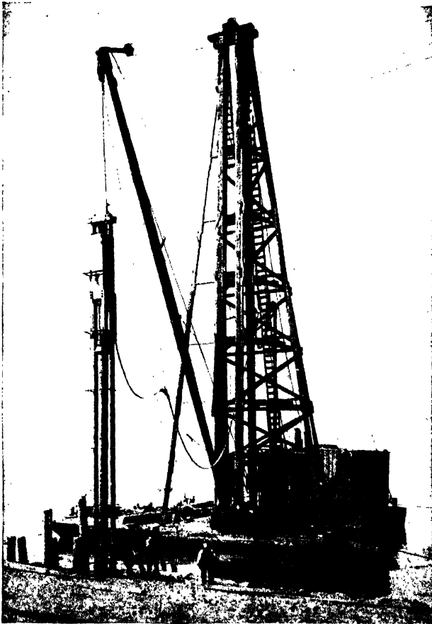
FIG. 31A. —Large double-acting steam hammer with pipe-sleeve attachment.
