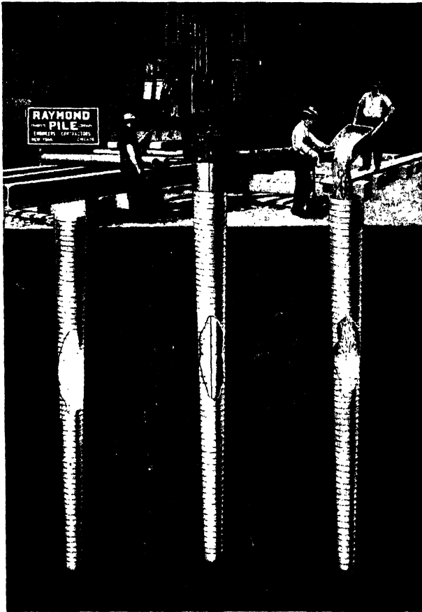
FIG. 40A.—Installing Raymond standard-taper piles.
