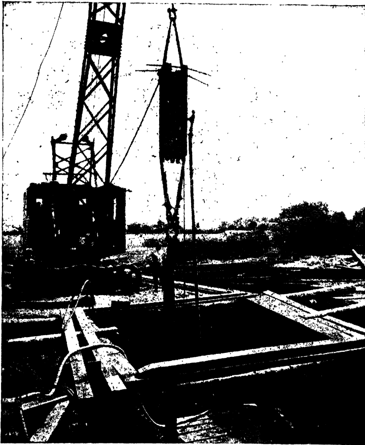
FIG. 17.—Inverted pile hammer.
