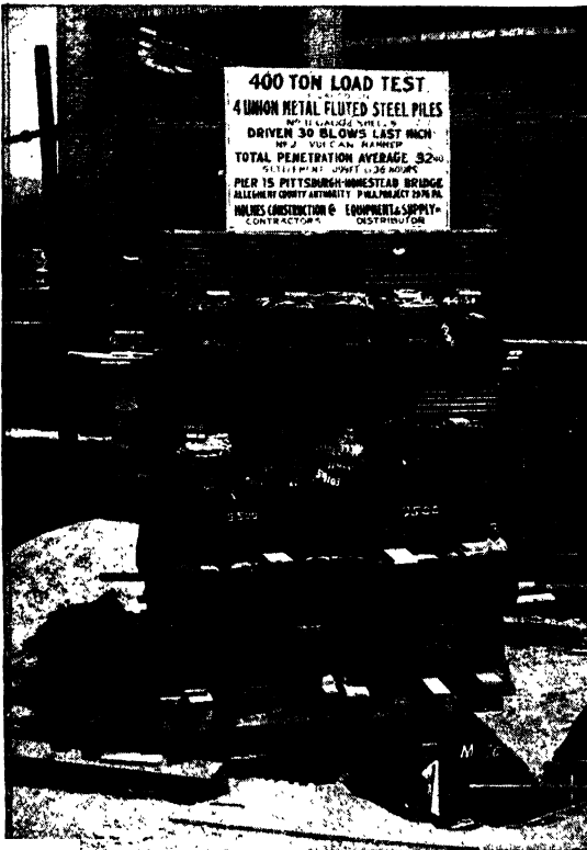
FIG. 49.—Pile-loading test on a pile group.
