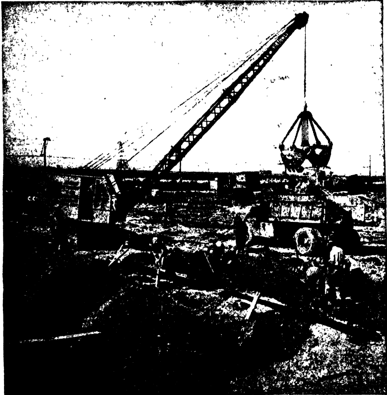
FIG. 13.—Clamshell bucket in trench excavation. ( Courtesy of Northwest Engineering Company. )
