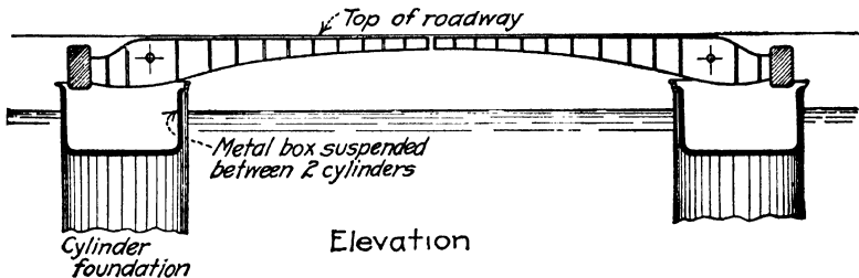
FIG. 21. —Old Knippels Bridge at Copenhagen, built 1869 (now removed).
