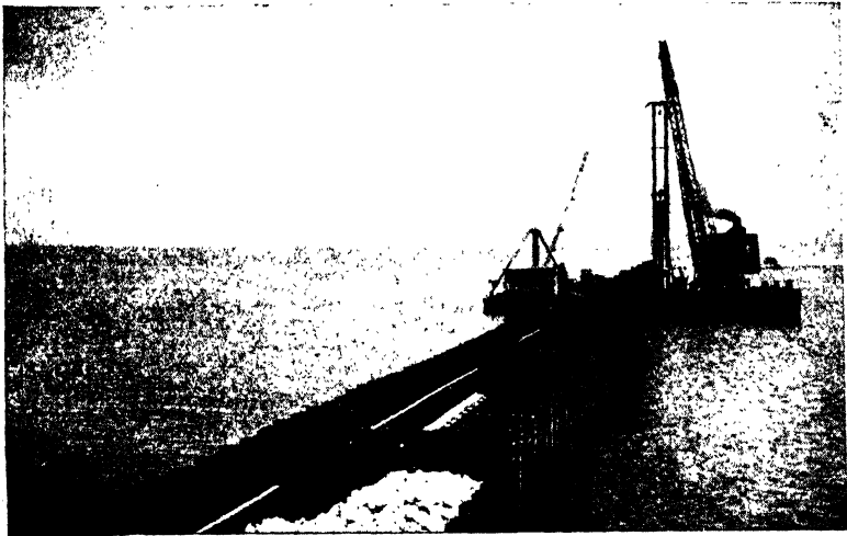
FIG. 29A.—Crane with wooden hanging leads.
