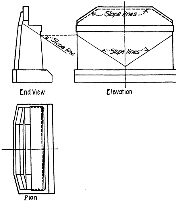
FIG. 3.—Breast abutment.
