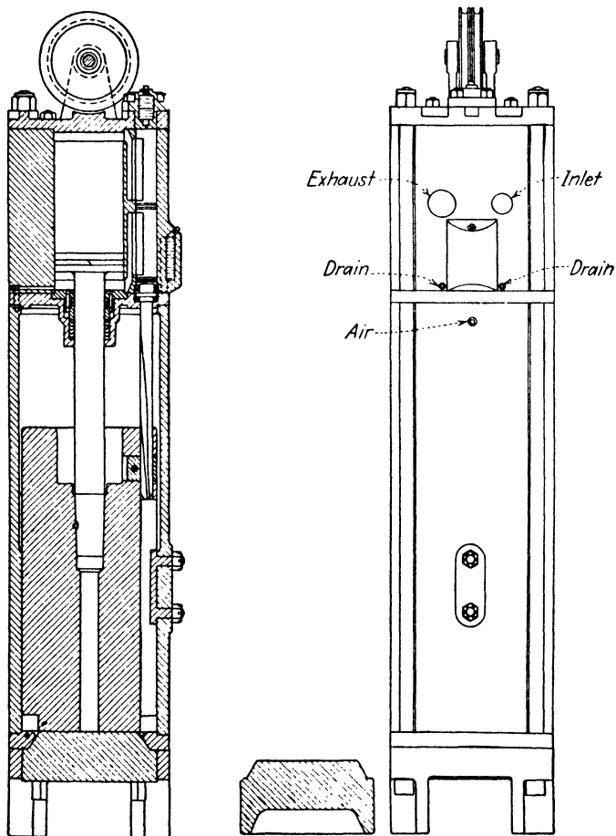
FIG. 30.—Cross section of a pile hammer.
