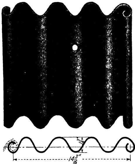
FIG. 56b.—Interlocking section, corrugated sheet piling.
