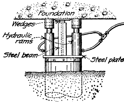
FIG. 15.—Method of driving pile by hydraulic rams. This illustration also shows method of wedging. "Pretest Method" (patented).
