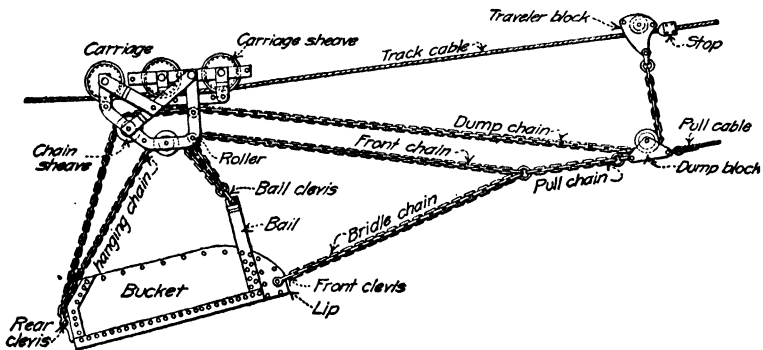
FIG. 14.—Dragline cableway bucket.
