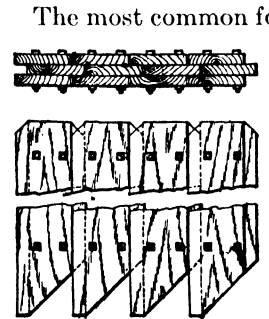
FIG. 51.—Wakefield sheet piling.
