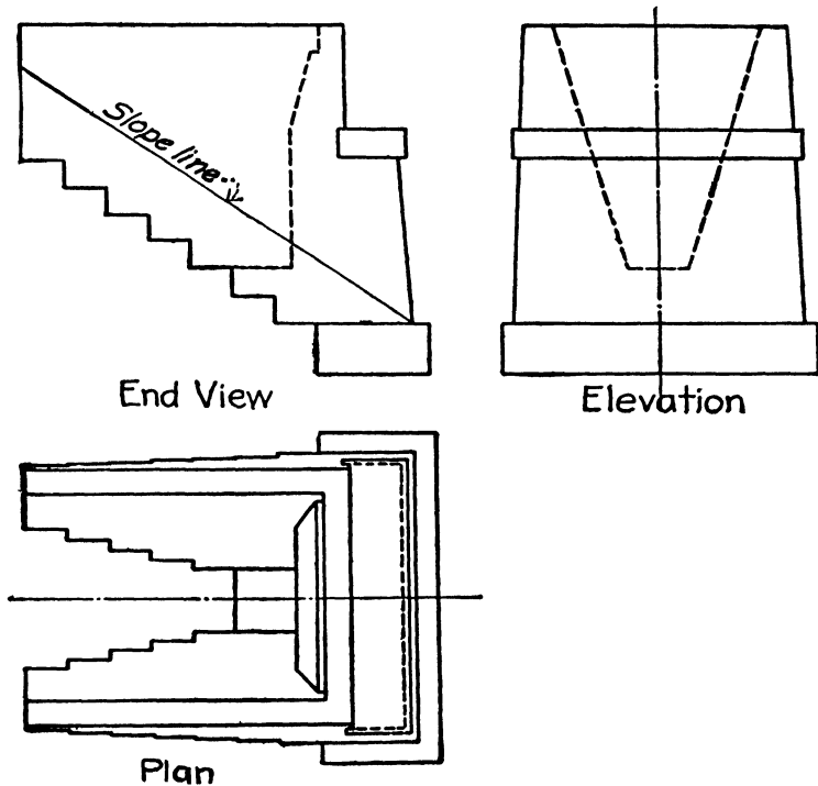
FIG. 5.—U abutment.
