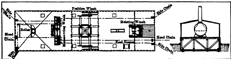
FIG. 27B.—Plan view of Lobnitz rock cutter.
