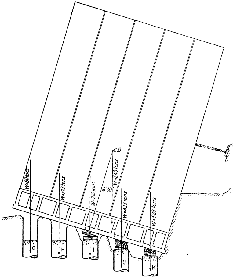
FIG. 19.—Section through the binhouse of the Winnipeg elevator. (Courtesy of Foundation Company.)
