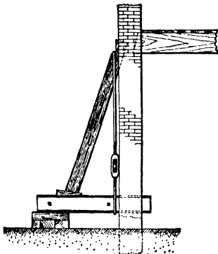
FIG. 4.—Shoring with support for wall below shore.
