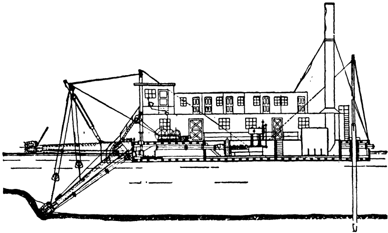
FIG. 31A.—Side view of hydraulic dredge. (Courtesy of Norbom Engineering Co.)
