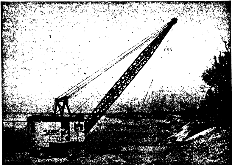
FIG. 11.—Dragline in moderate depth excavation. (Courtesy of Northwest Engineering Company.)
