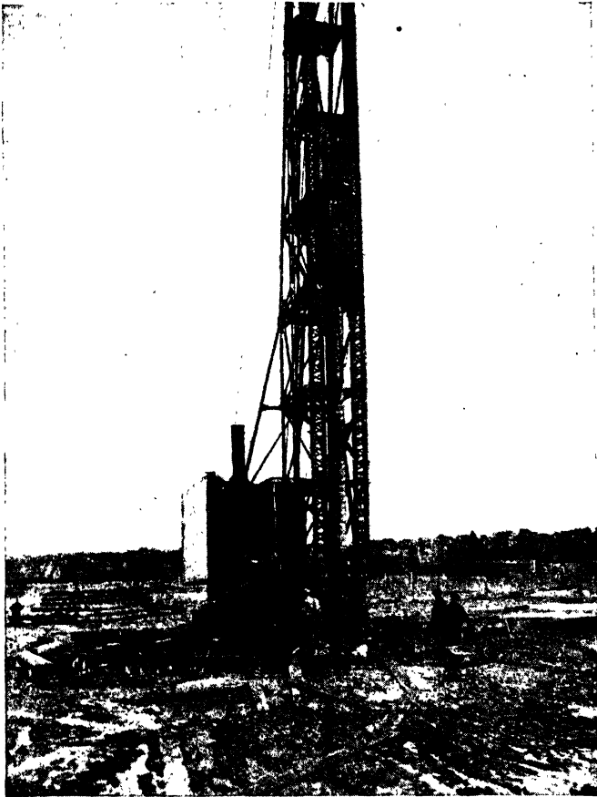
FIG. 41A.—Driving Raymond step-tapered piles.
