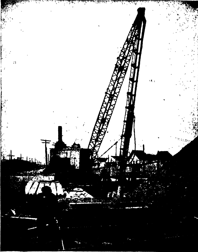
FIG. 29B.—Crane with steel hanging leads.
