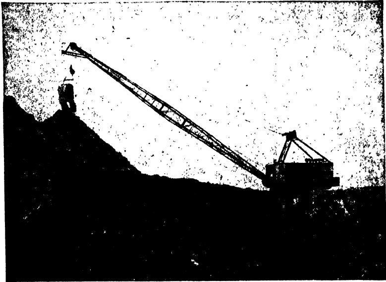
FIG. 16.—Walking dragline. (Courtesy of Bucyrus, Erie.)
