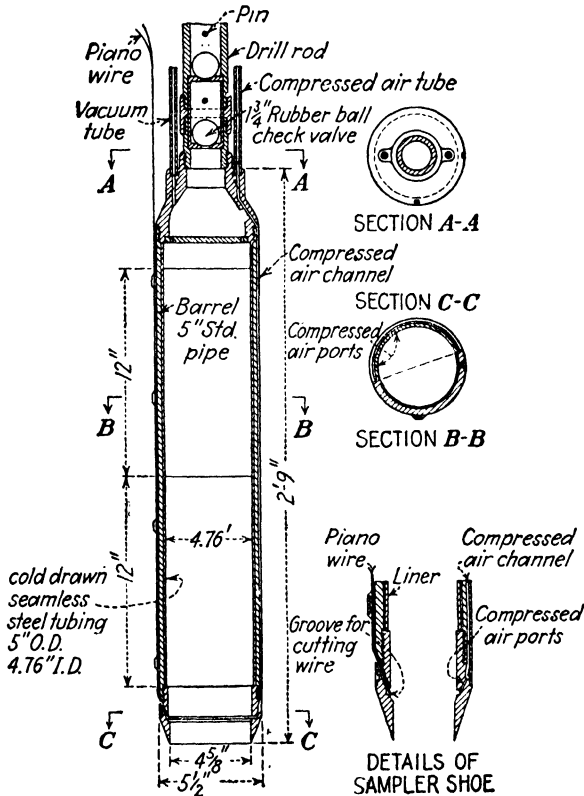
FIG. 4.—Casagrande-Mohr-Rutledge sampler. (Krynine, "Soil Mechanics.")
