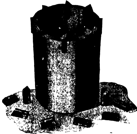
FIG. 6.—Calyx cutter. ( Jacoby and Davis, "Foundations of Bridges and Buildings," 3d Ed. )
