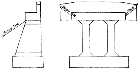
FIG. 12.—Buried abutment.
