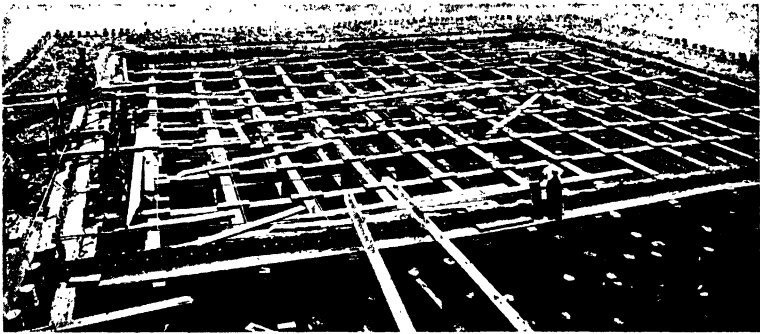
Fig. 22.—Cofferdam of the Boulevard Link Bridge in Chicago.
