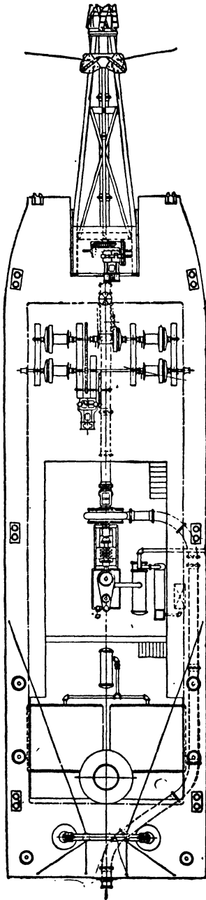
FIG. 31B.—Plan view of hydraulic dredge. (Courtesy of Norbom Engineering Co.)
