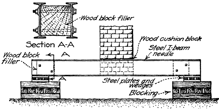
FIG. 5.—Simple needling operation.
