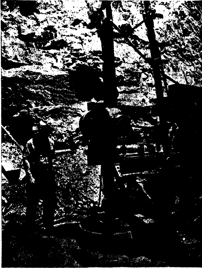
FIG. 11.—Mounting for 36-in. calyx drill. (Courtesy of Ingersoll-Rand Company.)
