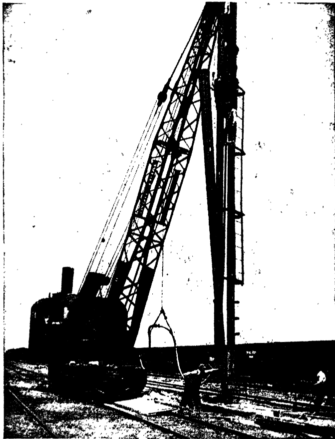
Fig. 28C.—Car-mounted crane with hanging leads.
