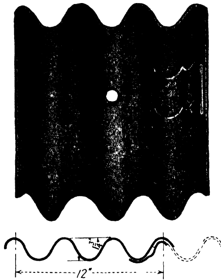
FIG. 56a.—Standard section, corrugated sheet piling.
