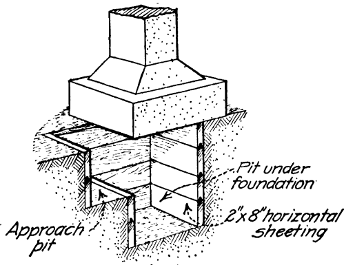
Fig. 11.— Foundation with underpinning pit.
