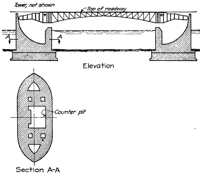
FIG. 15.—Tower Bridge, London, built 1892.
