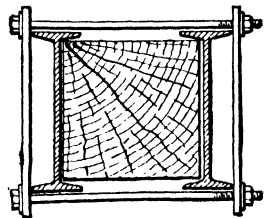
FIG. 3A.—Method of reinforcing wood shore for heavy loads.
