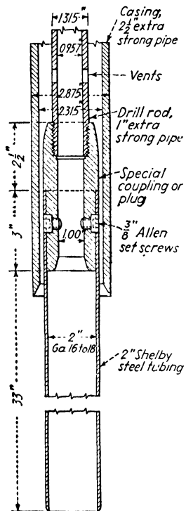
FIG. 2.—Shelby tubing sampler, by H. A. Mohr. (Jacoby and Davis "Foundations of Bridges and Buildings," 3d Ed.)
