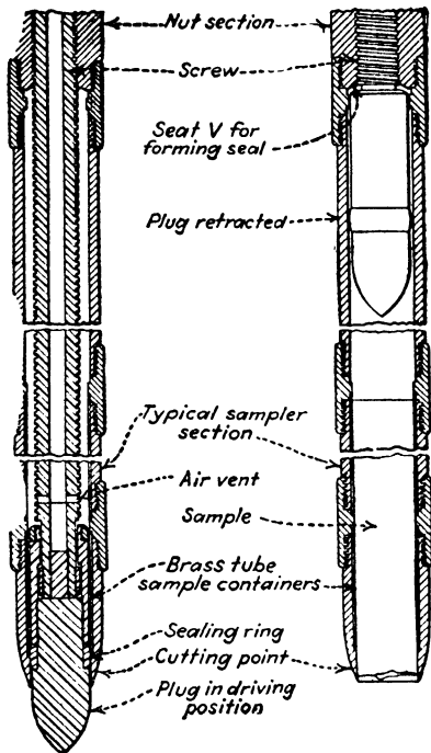
FIG. 1.—Lower end of Porter soil sampler. Jacoby and Davis, "Foundations of Bridges and Buildings," 3d ed. )
