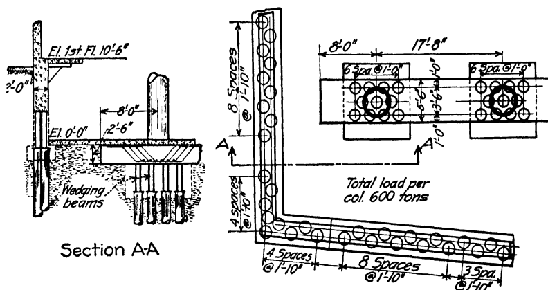
FIG. 17.—Typical pretest foundation (patented) as used for 17-story reinforced concrete building. Diameter of cylinders—14 to 20 in. Loading—350 to 500 lb. per sq. in. of cylinder cross section.
