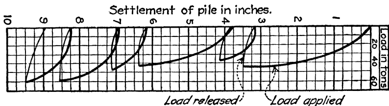
FIG. 16.—Loading test on jacked pile.
