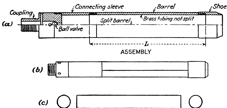
FIG. 3.—Moran and Proctor sampler. ( Krynine, "Soil Mechanics." )
