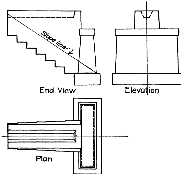
FIG. 4.—T abutment.
