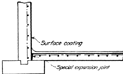
FIG. 2.—Surface waterproofing method.
