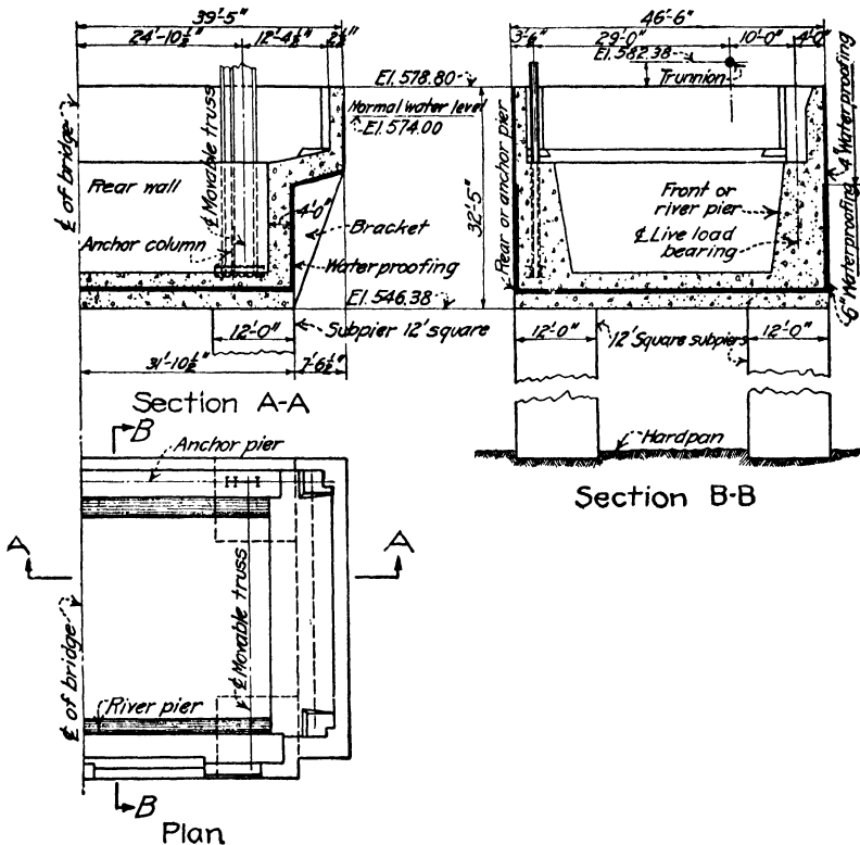
FIG. 16.—General design of Jefferson Avenue and Fort St. Bridge, Detroit; also the railroad bridge for the Detroit, Toledo & Ironton R. R. over the Short Cut Canal at Detroit.
