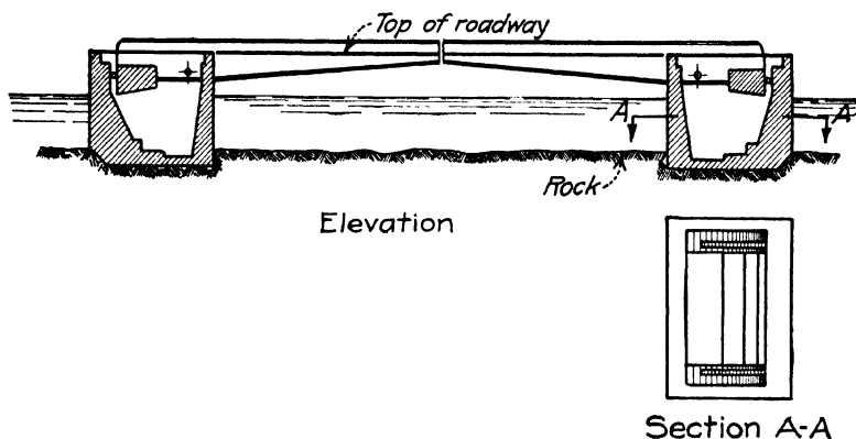
FIG. 17.—General design of Phoenix Bridge, built over the New York State Barge Canal; also 35th Street Bridge, Chicago, built 1914.
