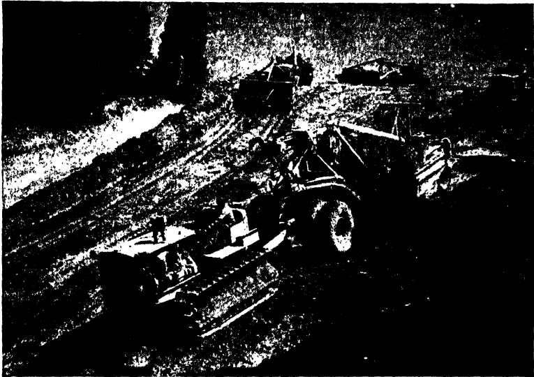
FIG. 3.—Carryall scraper. Loading operation. (Courtesy of R. G. LeTourneau, Inc.)
