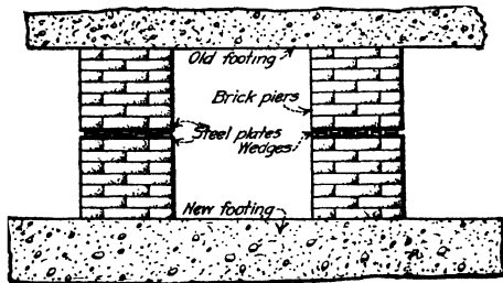
FIG. 12.—Wedging in brick underpinning piers.
