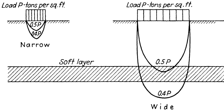
FIG. 13.—Isobars under a narrow and under a wide loaded area.
