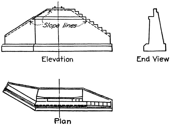
FIG. 7.—Wing abutment.
