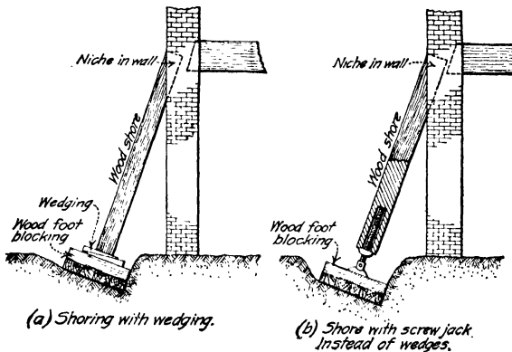
FIG. 3.—Typical shoring.
