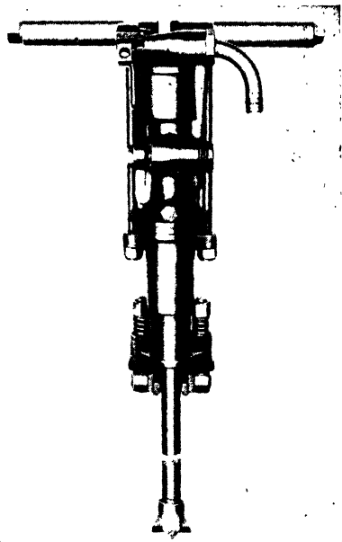
FIG. 22.—Front view of a jackhammer. (Courtesy of Ingersoll-Rand Company.)
