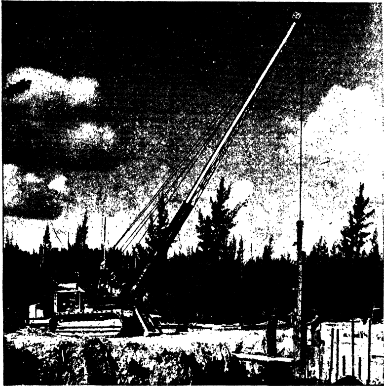
FIG. 55.—Caterpillar Diesel-powered speeder pile driver.
