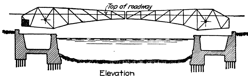
FIG. 19.—Erie Street Bridge, Chicago, built 1910.
