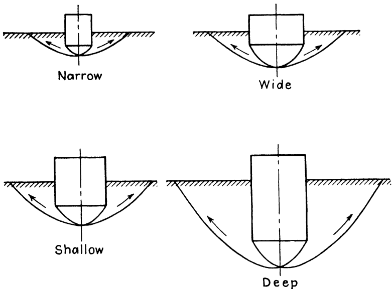
FIG. 14.—Possible shear planes under narrow, wide, shallow, and deep loaded areas.
