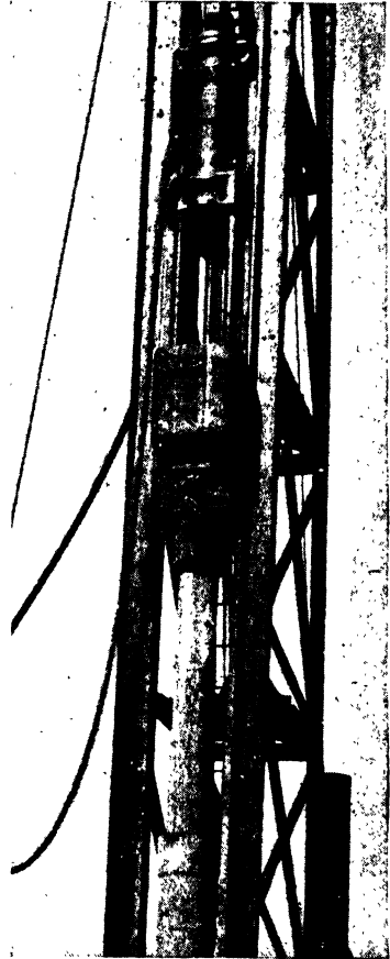
FIG. 46.—Withdrawing casing of the MacArthur pile.
