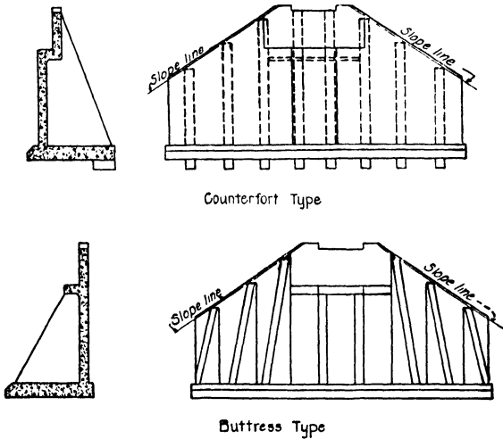
FIG. 13.—Reinforced concrete abutments.
