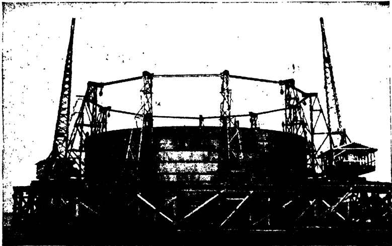
FIG. 25.—Lowering steel shell to provide sand island.
