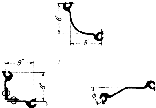
FIG. 52.—Standard rolled and fabricated corners.
