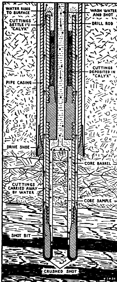
FIG. 10.—Shot drill showing calyx shot bit, drive shoe, and core sample. (Jacoby and Davis, "Foundations of Bridges and Buildings," 3d. ed.)
