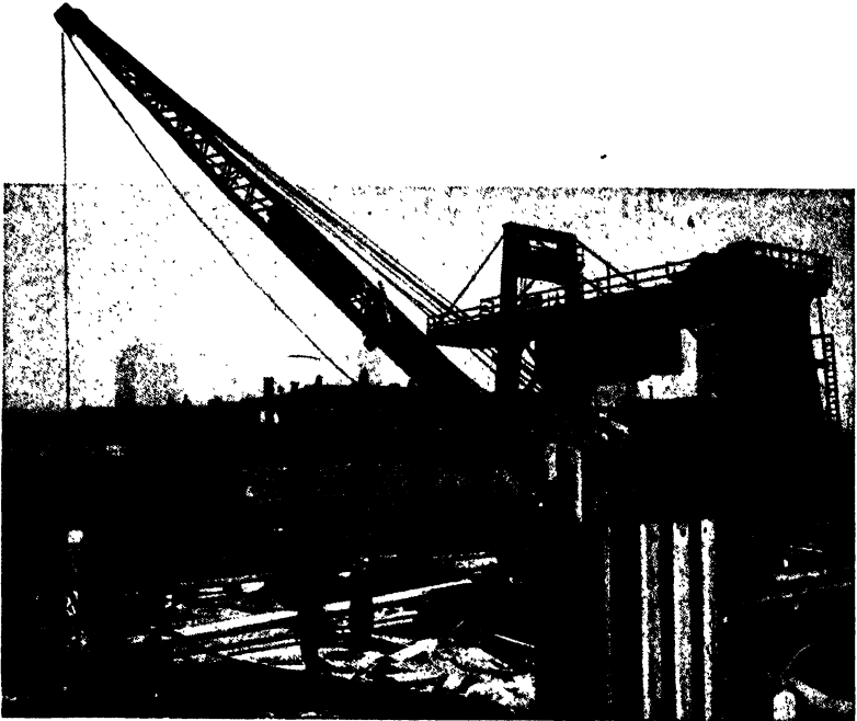
FIG. 16.—Pile extractor.
