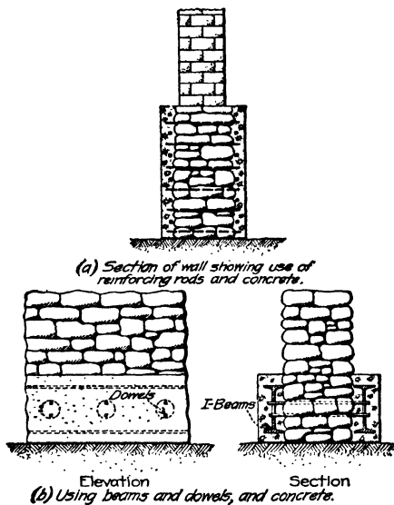
FIG. 7.—Strengthening old walls.
