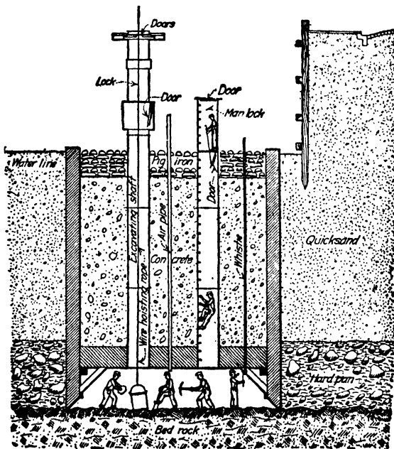
FIG. 26.—Pneumatic caisson sunk to bed rock.
