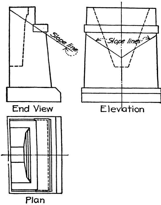
FIG. 6.—Pulpit abutment.
