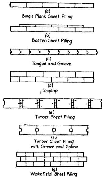
FIG. 50.—Types of timber sheet piling.
