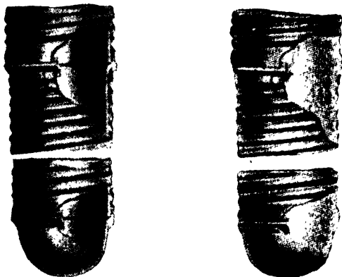
FIG. 41B.—Detail of step-tapered pile.
