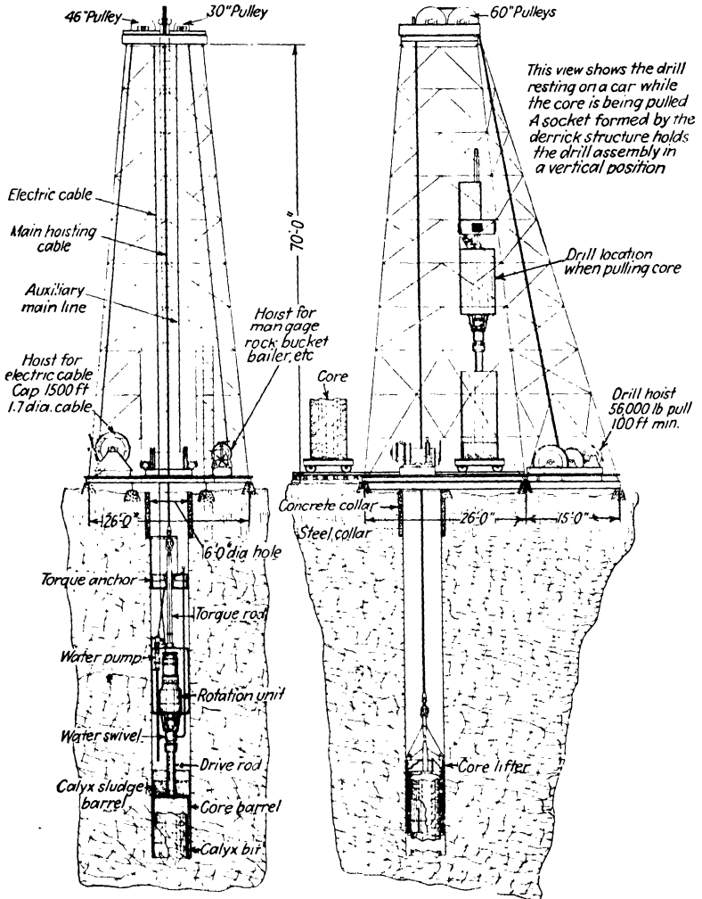
FIG. 25.—Rodless calyx bore unit. (Courtesy of Ingersoll-Rand Company.)
