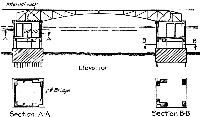
FIG. 20. —Bascule Bridge over Young's Bay, Astoria, Oregon, built 1920.
