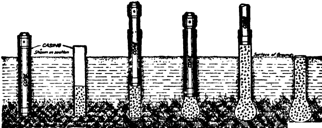
FIG. 47.—The process of forming a pedestal pile.
