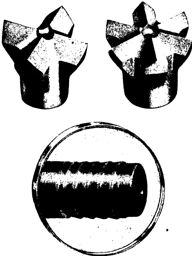
FIG. 23.—Jack bits and jack-rod thread. (Courtesy of Ingersoll-Rand Company.)
