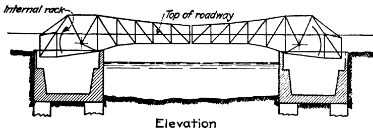
FIG. 18.—General design of Jefferson Avenue and Fort St. Bridge, Detroit; also the railroad bridge for the Detroit, Toledo & Ironton R. R. over the Short Cut Canal at Detroit.
