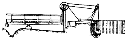
FIG. 42.—SUBBA RAO'S WATER-LIFT (SECTION).
