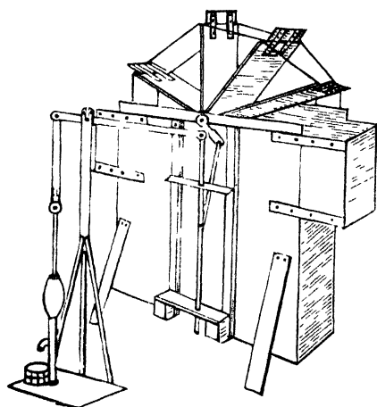
FIG. 7.—THE HOME-MADE WINDMILL.
