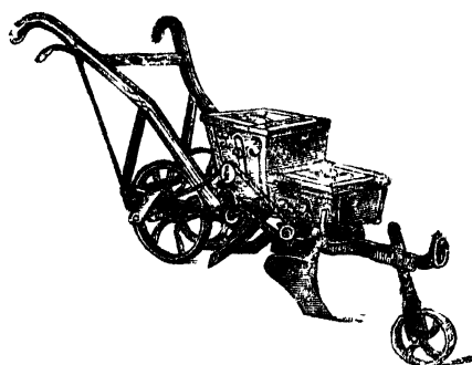
FIG. 31.—HENDERSON CORN PLANTER AND FERTILIZER DISTRIBUTOR.
