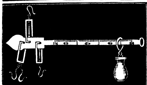
FIG. 60.—STEEL-YARD FOR WEIGHING 15 TO 50 lb. (60 RESERVED).
