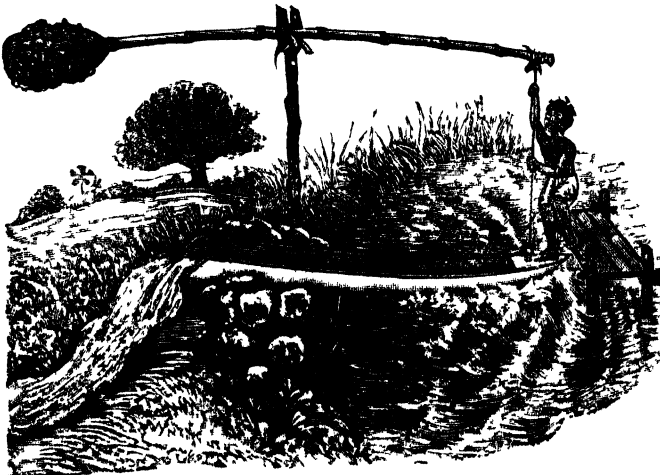
FIG. 51.—THE ORDINARY DON.
