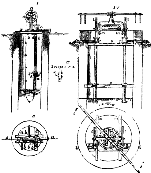
HAND-LIFT.
