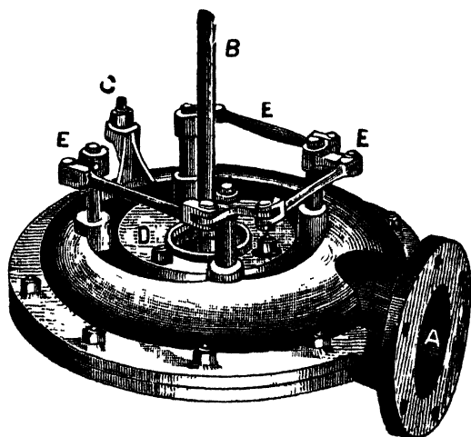
FIG. 12.—THE TURBINE.
