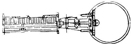
FIG. 41.—SUBBA RAO'S WATER-LIFT (PLAN).
