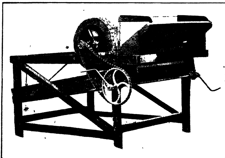
FIG. 37.—HAUSER'S WINNOWER AND GRAIN-CLEANER.
