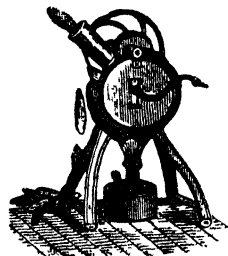
FIG. 58.—MAIZE-HULLER.
