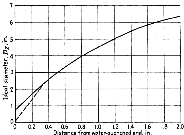
FIG. 6.9. Relation between ideal diameter and Jominy depth. (Asinow, Craig, and Grossmann, 12 as modified by Hodge and Orehoski. 73 )
