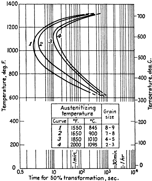
FIG. 3.11. Comparative time intervals for 50 per cent transformation in a single steel as influenced by austenite grain size. (Davenport) 41
