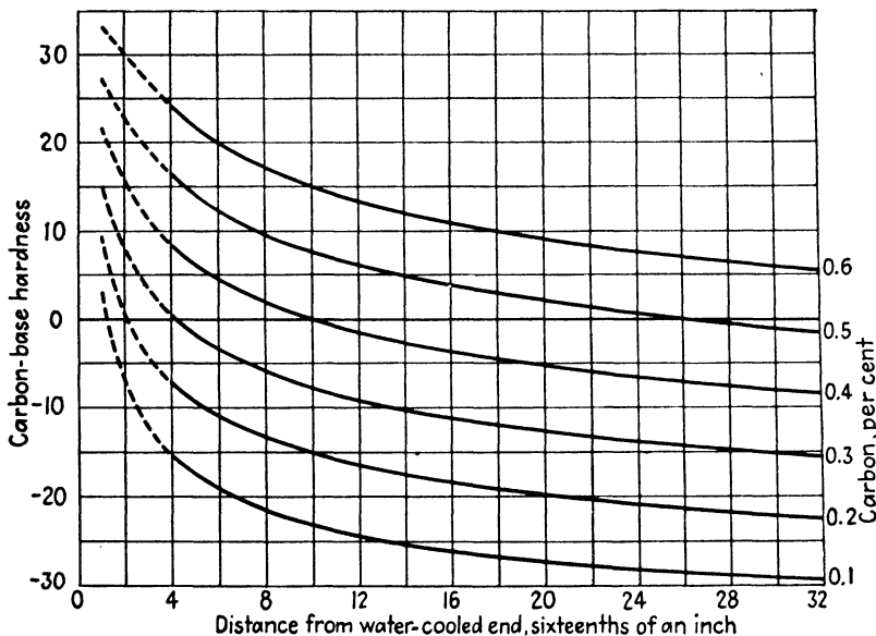
FIG. 7.7. Effect of cooling rate, expressed as Jominy distance, on carbon-base hardness (Rockwell C). ( Crafts and Lamont. ) 27
