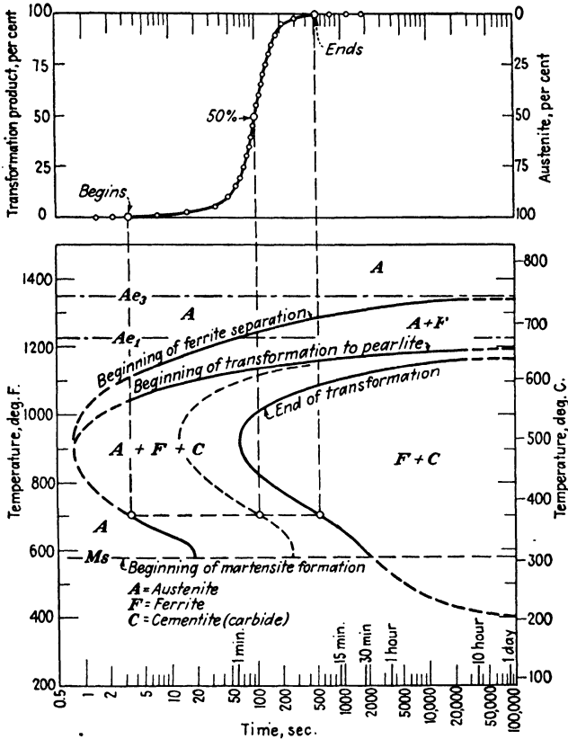
FIG. 3.4. Method of constructing a T-T-T diagram, and complete diagram for a medium-carbon nickel steel. (Atlas.) 115
