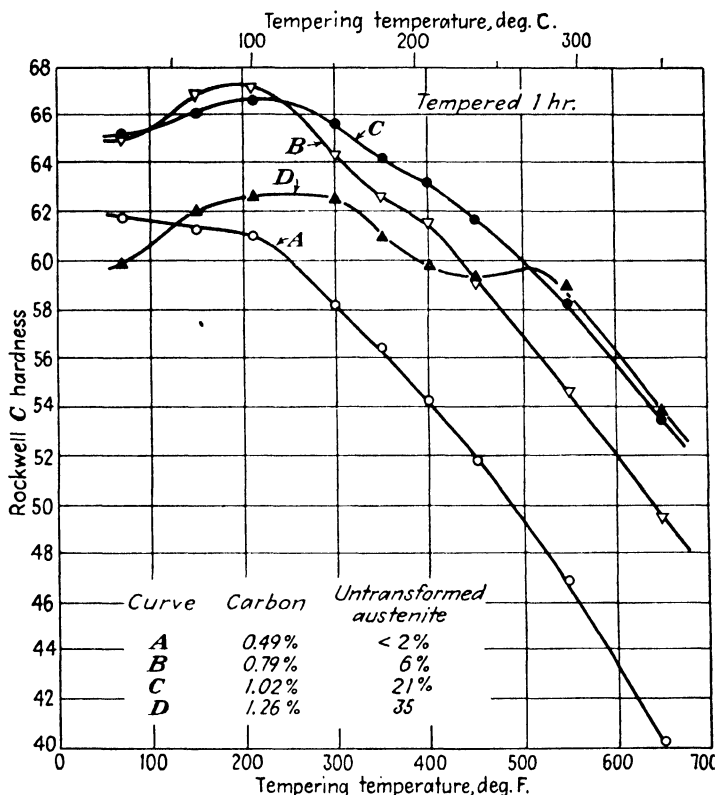
FIG. 8.3. Hardness-tempering curves for tempering for one hour at various temperatures steels containing 0.49 to 1.26 per cent carbon. (Fletcher and Cohen.) 60
