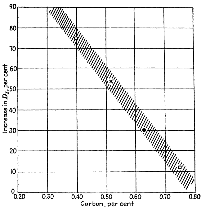
FIG. 5.18. Relation of carbon content to the ideal critical diameter in carbon steels containing an effective boron addition (0.001 per cent minimum). ( Grange and Garvey. ) 58
