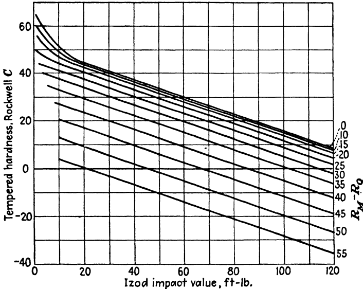
FIG. 9.14. Relation between Izod impact strength, tempered hardness, and degree of hardening of fine-grained alloy steels. (Crafts and Lamont.) 39
