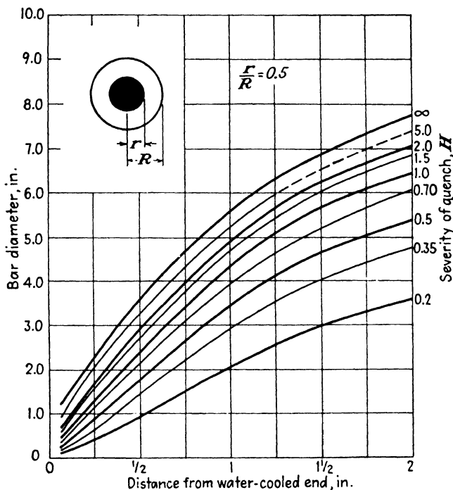
Fig. 4.19. Location on end-quenched Jominy hardenability specimen corresponding to 50 per cent from the center of round bars. (Lamont.) 96
