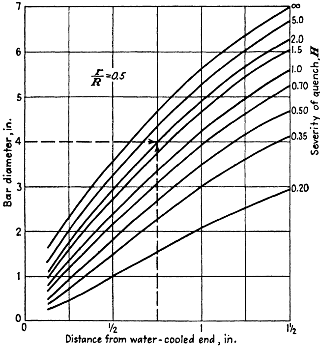
Fig. 4.12. Relation between severity of quench, Jominy depth, and bar size at a fractional depth r/R=0.5 . (Lamont.) 96
