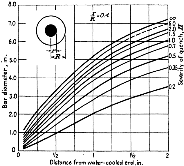
FIG. 4.18. Location on end-quenched Jominy hardenability specimen corresponding to 40 per cent from the center of round bars. (Lamont.) 98
