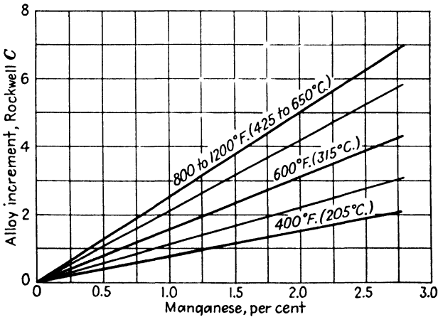
FIG. 8.13. Effect of manganese on resistance to softening at various tempering temperatures. (Crafts and Lamont.) 38
