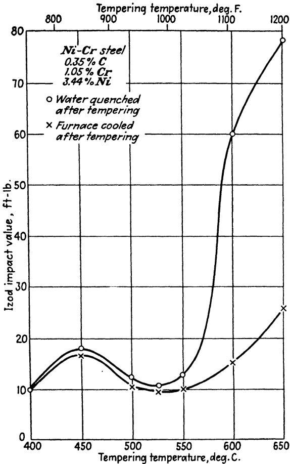
FIG. 9.16. Effect of cooling rate in avoiding temper brittleness after tempering a susceptible steel in the critical temperature range. (Hollomon.) 27
