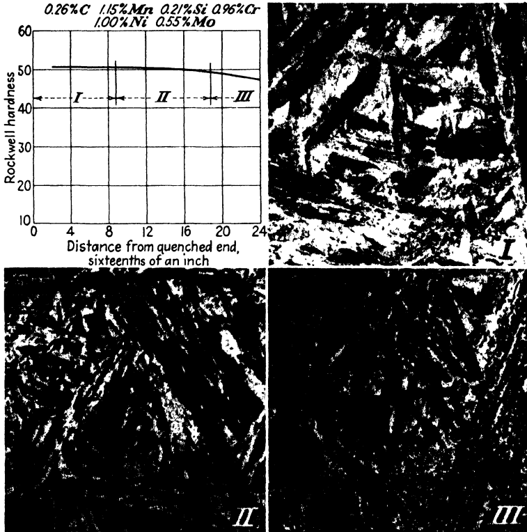
FIG. 8.4. Types of martensite in hardened Jominy specimens. Original magnification 2000 \times ; reduced \frac{1}{8} .
