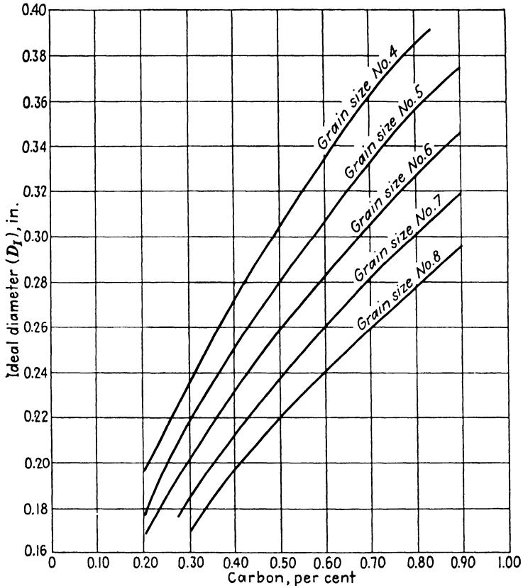
FIG. 5.13. Relation between ideal diameter ( D_I ), carbon content, and grain size. (Boyd and Field, 24 after Grossmann. 86 )
