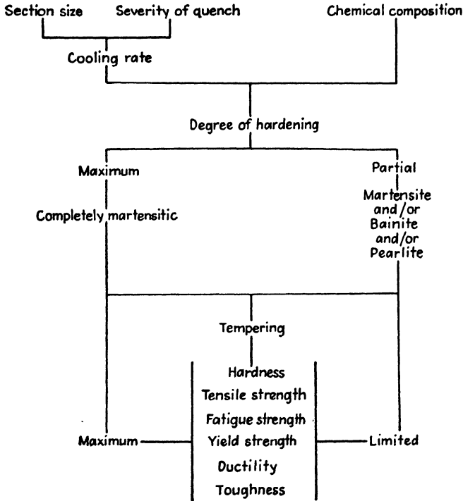
FIG. 1.1. Schematic representation of factors to be considered in the heat treatment of carbon and low-alloy steels.
