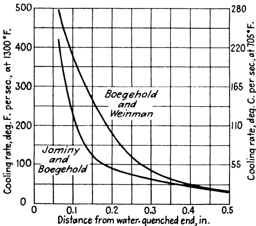
FIG. 6.6. Cooling rates along the Jominy test specimen determined originally by Jominy and Boegehold 97 and later by Boegehold and Weinman, according to Kopecki. 93
