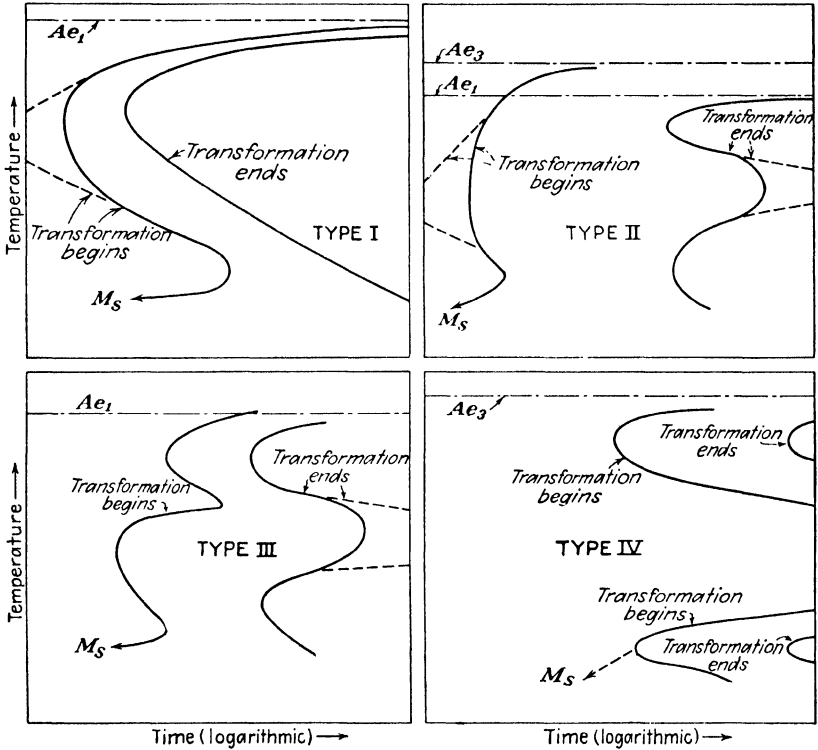
FIG. 3.13. General types of T-T-T diagrams for alloy steels. (Morral) 106
