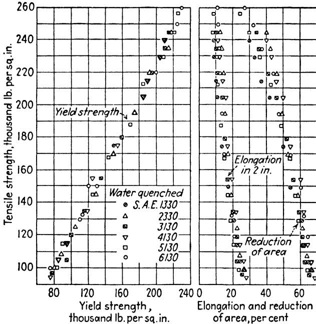
Fig. 9.4. Tensile properties of water-quenched and tempered SAE low-alloy steels containing about 0.30 per cent carbon. (Janitzky and Baeyertz.) 55
