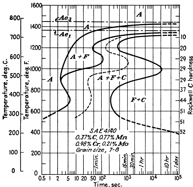
FIG. 3.5. T-T-T diagram of SAE 4140 steel austenitized at 1550°F. (845°C.), indicating time for beginning of transformation (left-hand lines) and for complete transformation (right-hand lines). Phases: A = austenite; F = ferrite; C = carbide. ( Atlas. ) 115
