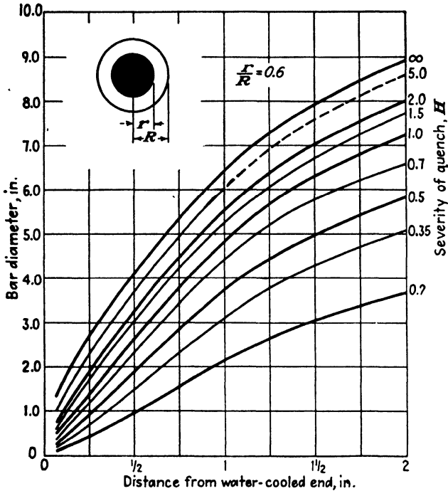
FIG. 4.20. Location on end-quenched Jominy hardenability specimen corresponding to 60 per cent from the center of round bars. (Lamont.) 96
