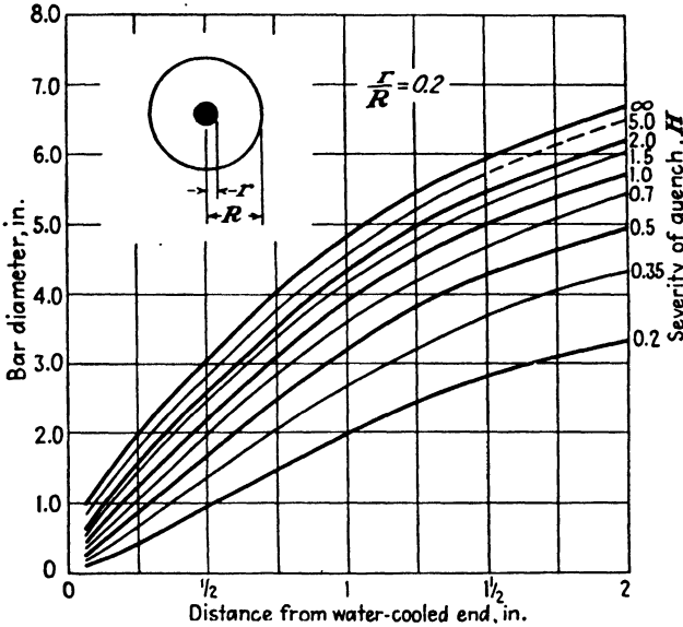
Fig. 4.16. Location on end-quenched Jominy hardenability specimen corresponding to 20 per cent from the center of round bars. (Lamonl.) 98
