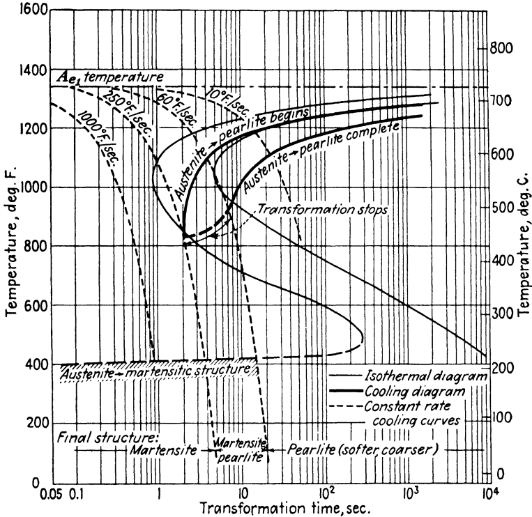
FIG. 3.16. Relation between continuous cooling rates and the T-T-T diagram for a eutectoid steel. (Grange and Kiefer.) 87
