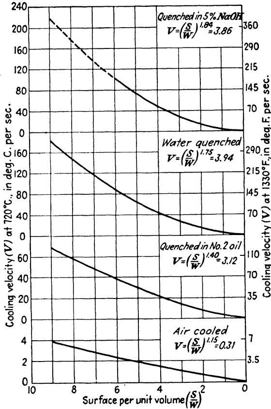
FIG. 4.4. Relation between center cooling velocity at 1330°F. (720°C.) and the surface per unit volume of steels quenched from 1610°F. (875°C.) in different coolants. (French.) 82
