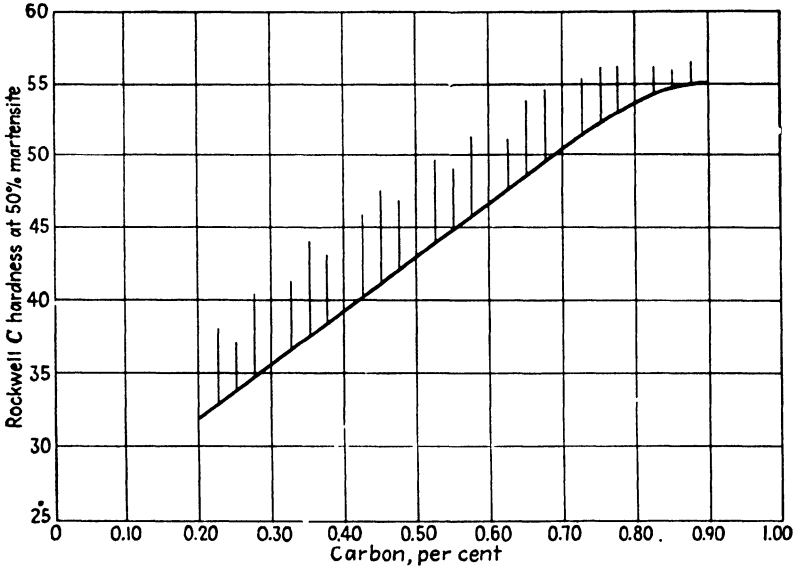
FIG. 5.16. Effect of carbon on the hardness of 50 per cent martensite. (Solid line for plain carbon steel; hatched portion for low- and medium-alloy steels.) (Grossmann.) 98
