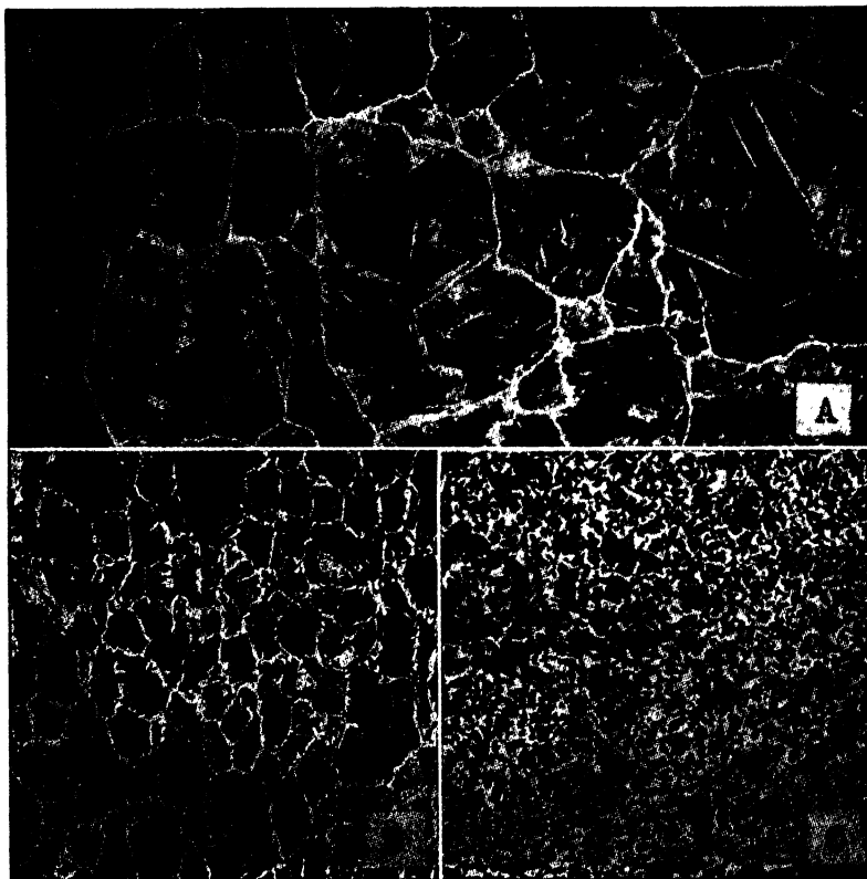
FIG. 2.8. Typical structure of slowly cooled carbon steel having (A) grain size 2; (B) grain size 5; and (C) grain size 8. Etched; 100 \times . ( Sisco ). 132
