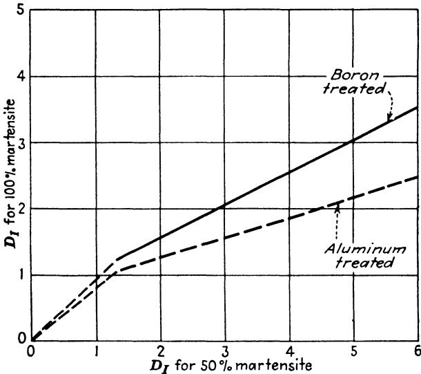
FIG. 5.19. Effect of boron on the relation between the ideal critical diameter for 50 per cent martensite and that for 100 per cent martensite.
