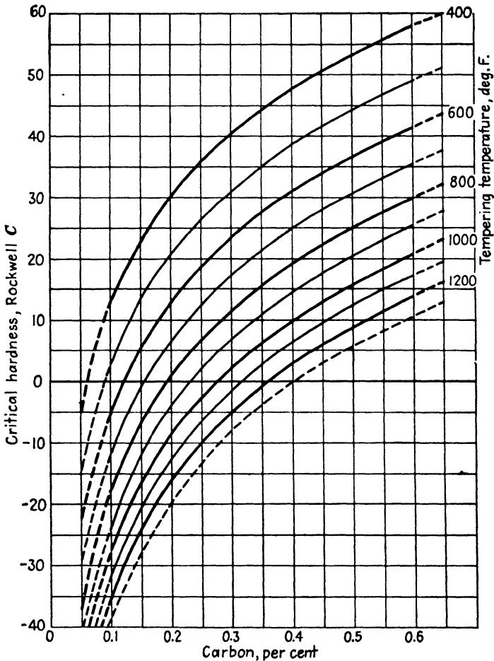
FIG. 8.19. Critical hardness (B) for alloy-free steel as affected by carbon content and tempering temperature. (Crafts and Lamont.) 28
