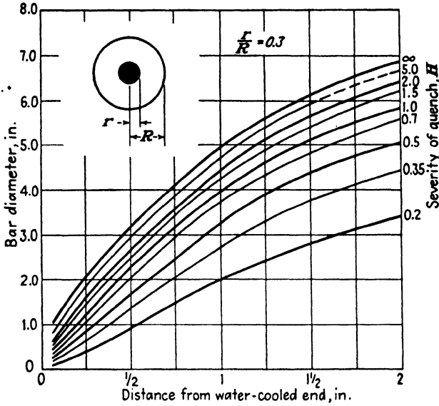
FIG. 4.17. Location on end-quenched Jominy hardenability specimen corresponding to 30 per cent from the center of round bars. (Lamont.) 98
