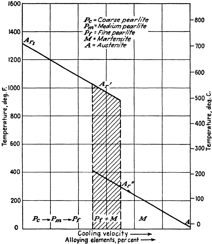
FIG. 3.2. Effect of cooling velocity and alloying elements on the location of the lower transformation point ( A_{r1} ) in cooling. (Sauveur.) 173
