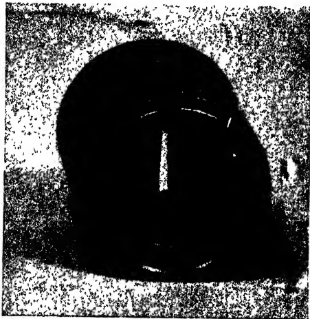
FIGURE 2. Photograph of transparent cell used in ultracentrifuges of the vacuum type. Diam. of cell, 25.4 mm; capacity, 0.6 cc; thickness of solution column in direction of light path, 1 cm. Quartz windows permit passage of ultraviolet light. Evaporation through the small filling hole is prevented by a rubber gasket and a screw plug.
