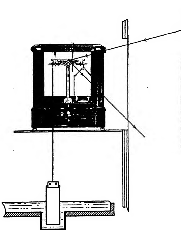
FIGURE 17. Vertical type of film balance for the measurement of the film pressure of soluble and insoluble films. (The balance is kept on the closed top of the thermostat, while the trough and film are inside.)
