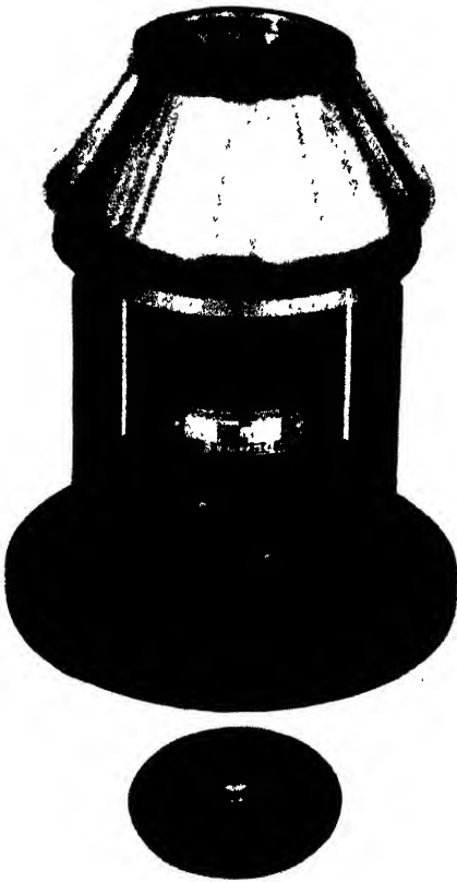
FIGURE 11. High-speed preparative angle centrifuge of the type designed by the author (see Ref. 90). Rotor fits directly on shaft of universal electric motor, which is flexibly mounted. For rotor illustrated: diameter, 20 cm; number of tubes, 18; capacity, 166 cc; speed, 18,000 rpm; maximum centrifugal force on fluid, 34,800 times gravity. Other rotors accommodate up to 610 cc of liquid.
