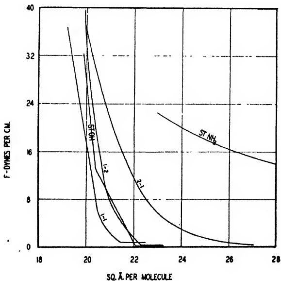
FIGURE 46. Effect of proportions in mixed stearyl alcohol and amine films ( \text{pH} = 3 ). The first figure gives the number of molecules of amine and the second of alcohol. The 1:1 mixture exhibits the greatest condensation.
