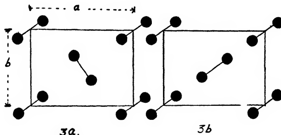
FIGURE 3. Relative Orientation of the Molecules in (a) the Rhombic Crystal, (b) Layer Structure of Paraffin Hydrocarbons. \bullet — \bullet represents the projection of a hydrocarbon molecule on the a-b crystal face. [After A. Muller, Proc. Roy. Soc. London , A127 , 417 (1930).]
