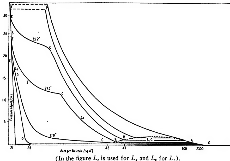
FIGURE 6. General phase diagram of a monolayer at a temperature below the critical temperature for the formation of a liquid expanded ( L_s ) film. Phases: FE or S , solid; ED or L_s , liquid condensed; DC or I , intermediate; CB or L_s , liquid expanded; BA or L_sG , gaseous film and L_s film in equilibrium; G gaseous film. The temperatures given are those for pentadecylic acid. For longer chain acids and for an alcohol of the same chain length the temperatures are higher, etc. The scale of molecular areas is much shortened (above about 47 Å) and the pressure scale is much expanded.
