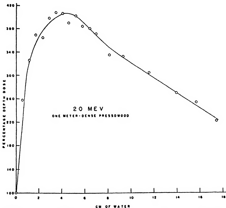
FIGURE 5. The distribution of ionization in a heavy Presswood phantom having a density equal to that of water.
