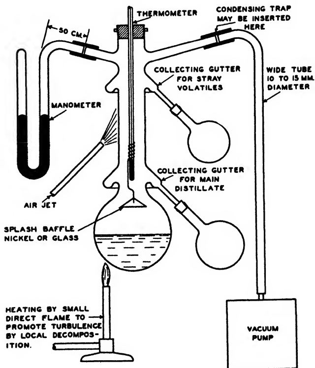
FIGURE 3. High-vacuum pot still assembly.
