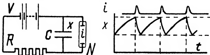
FIGURE 1. Figure from Fessard 12 showing at left a neon tube, N, in circuit with a condenser, C, battery, V, and resistance, R. The tube fires intermittently, as shown on the right; x is voltage across the condenser and i is current across the tube.
