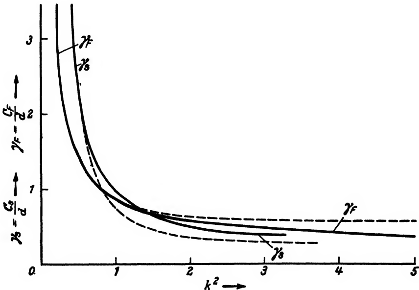
FIGURE 6. Spherical C_s and chromatic C_p aberration constants of magnetic lenses as a function of k^2 . Curve \gamma_s (full) — calculated ratio C_s/d for unsaturated pole pieces; curve \gamma_s (dotted) — calculated ratio C_s/d for saturated pole pieces; curve \gamma_p (full) — calculated ratio C_p/d for unsaturated pole pieces; curve \gamma_p (dotted) — calculated ratio C_p/d for saturated pole pieces. 57
