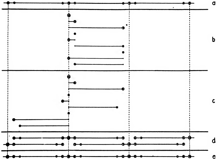
FIGURE 4. Relation between a hypothetical one-dimensional structure of point atoms (a) and its Patterson vector structure (e).
