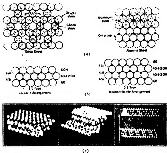
FIGURE 17. The crystal structure of the clay minerals. (a) Arrangement of atoms in the sheets; (b) arrangement of atoms in a single crystal plate; (c) in the models of kaolinite (left), montmorillonite (center) and the expanded lattice of montmorillonite (right). 81
