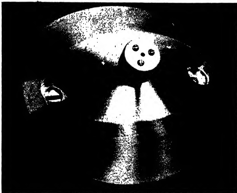
FIGURE 4. Oval-shaped Duralumin rotor of vacuum-type ultracentrifuge with cell and counterbalance shown in position. Maximum diameter of rotor is 18 cm. It withstands routine operation at 60,000 rpm, with an average centrifugal force in the cell 260,000 times that of gravity.
