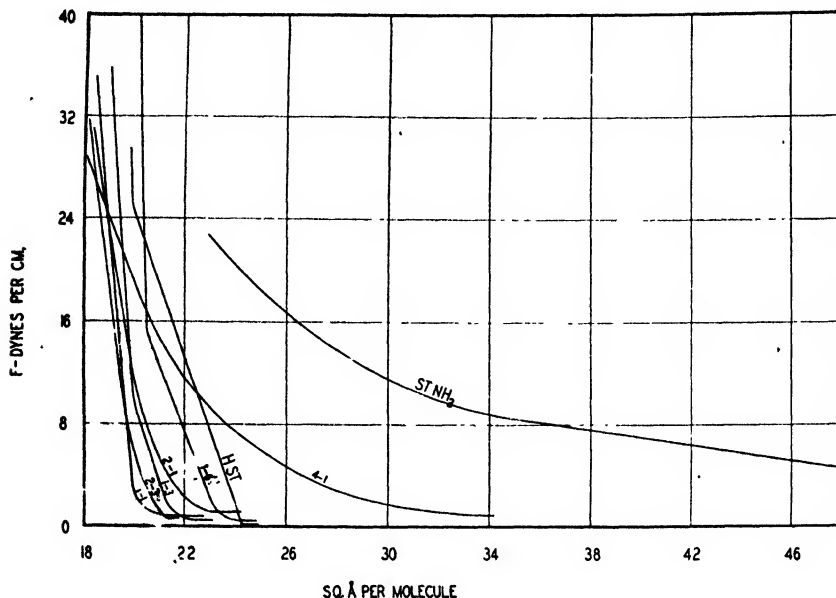
FIGURE 48. Effect of proportions in mixed films of stearyl amine and stearic acid ( \text{pH} = 3 ). The numbers on the curves give the ratio mole of amine to acid. The 1:1 mixtures exhibits the greatest condensation with very low molecular areas, and above 3 dynes the low compressibility 0.0023 (at \pi = 0 extrapolated) or a Type S film, while the similar value for one component stearyl alcohol I film is 0.0024. With 75 molar per cent of acid the sharp transition II I or liquid to solid is preserved, but seemingly not with 66 \frac{2}{3} per cent.
