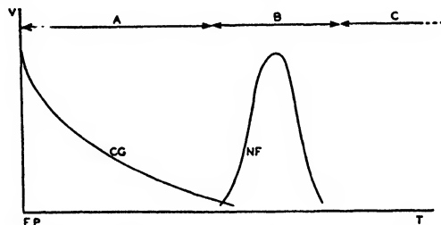
FIGURE 1. Graph representing the velocity of crystal growth (curve CG) and of the formation of crystalline nuclei (curve NF) in terms of decreasing temperatures; V, velocity; T, temperature; F. P., freezing point. (Curves drawn from Tammann's 1 data.)
