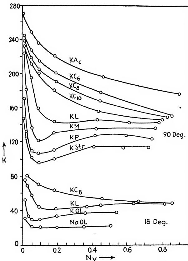
FIGURE 3. Equivalent Conductivity of Soap Solutions at 18° and at 90°.
