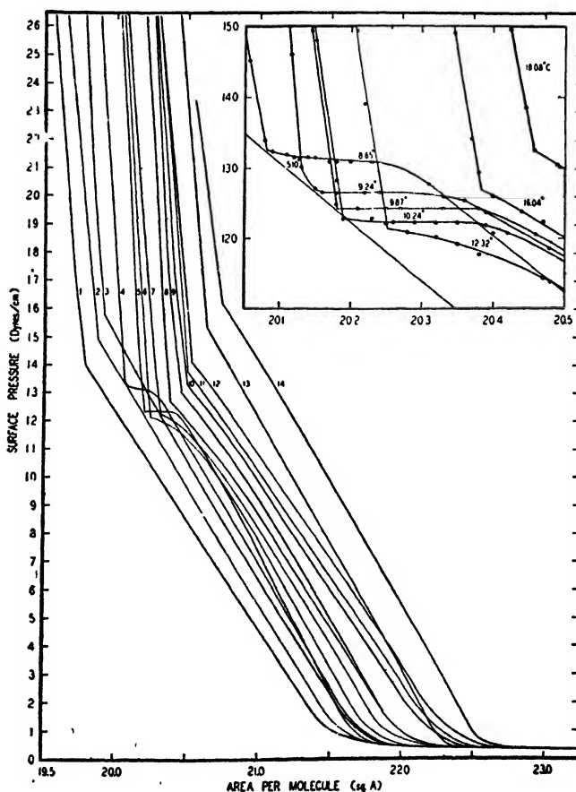
FIGURE 14a. Pressure-area temperature relations of condensed monolayers of octadecanol on water. The insert gives an enlarged section in the region of the first-order transition. Outside of this region all of the transitions are second-order. The temperatures ( ^{\circ}\text{C} ) for the curves in the principal diagram are: 1, 2.85; 2, 5.10; 3, 7.10; 4, 8.62; 5, 9.90; 6, 12.32; 7, 14.06; 8, 16.04; 9, 18.08; 10, 19.85; 11, 22.95; 12, 25.12; 13, 30.30; 14, 34.85. Curves for four other temperatures are given in the insert. Correction: Multiply Surface Pressures by 0.9315.
