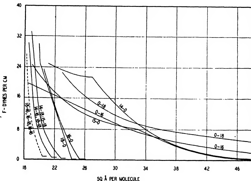
FIGURE 47. Mixtures (1:1) of acids and amines (pH = 3). The first figure gives the number of carbon atoms in the acid, and the second in the amine, molecule. All of the seven mixtures exhibit pressure-area curves of the same form, and with not very widely differing and very low areas. At the lower pressure all the mixtures give curves of the transition form.
