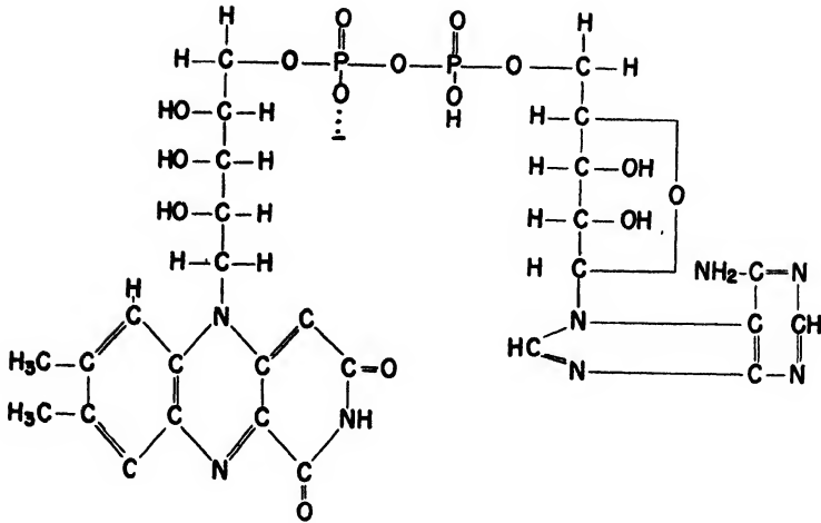
FIGURE 3. Flavin-adenine-dinucleotide.
