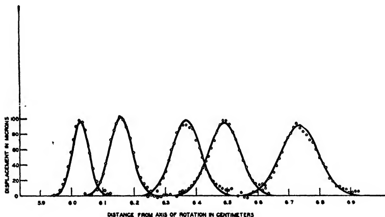
FIGURE 17. Theoretical vs. actual boundary spreading in sedimentation experiment on bushy stunt virus. Open circles are experimental points obtained by Lamm Scale method. Smooth curves are theoretical boundaries calculated from known diffusion constant. The times in minutes and scale cell distances in centimeters for the successive boundary curves, beginning at the left, are: 50, 2.1; 85, 3.1; 135, 4.1; 150, 4.6; 220, 5.6. (From Lauffer. 45 )
