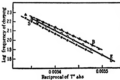
FIGURE 4. Data from three independent observers for the frequency of chirping of crickets as a function of temperature, from Crozier. 7
