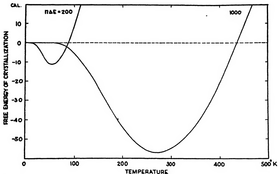
FIGURE 5. Dependence of the free energy of crystallization on the absolute temperature, according to Eq. (7), assuming n\Delta E = 200 cal and 1000 cal, with k' = k and n = Avogadro's number in both cases.
