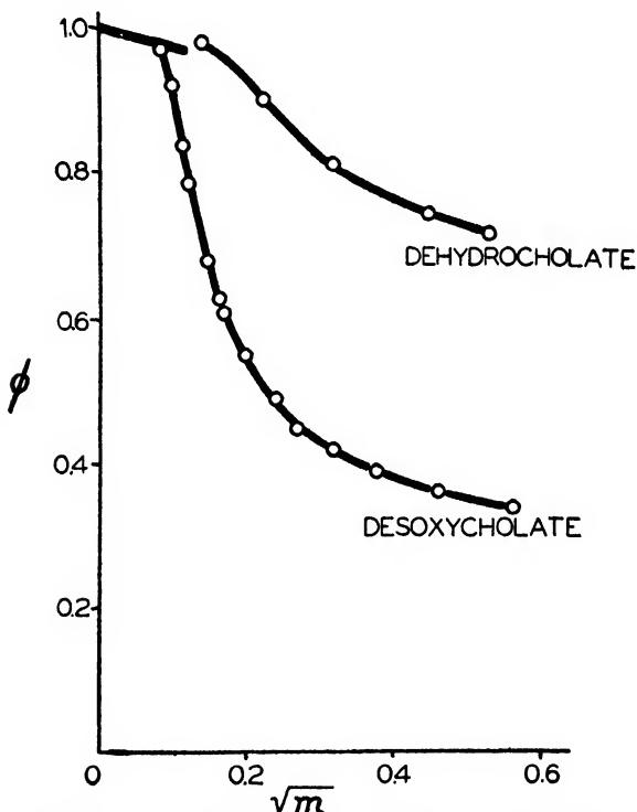
FIGURE 7. The Osmotic Coefficient of the Bile Salts; the detergent sodium desoxycholate, and the non-detergent sodium dehydrocholate.
