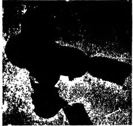
FIGURE 35. Partially cytolized Bacillus Megatharium cells under the action of sonic vibration, 123
