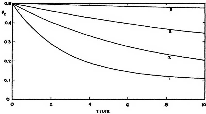
FIGURE 8. Variation with time (in arbitrary units) of the fraction of subsystems in the upper energy state (2), for various values of k'' (indicated by the numbers alongside the curves), according to Eq. (12).
