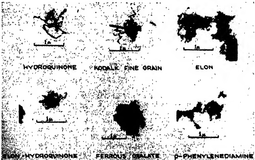
FIGURE 9. Electron micrographs of developing silver halide grains.
