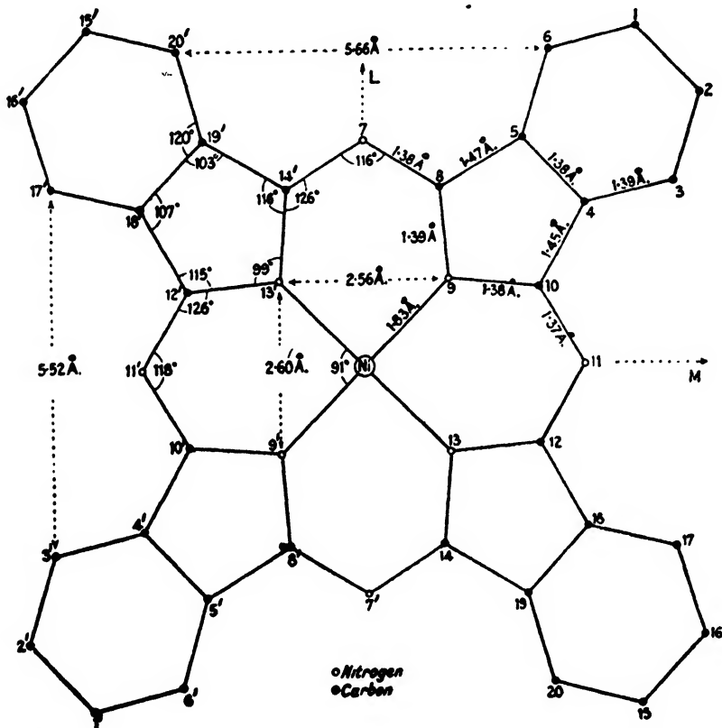
FIGURE 1. Dimensions of the Nickel Phthalocyanine Molecule (Robertson).
