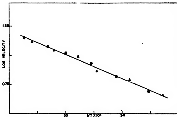
FIGURE 16. Arrhenius equation plot for oxidation of p -phenylenediamine. 1 \times 10^{-4}M p -phenylenediamine and 0.5 ml enzyme. ● = determinations made the day of preparation of enzyme. ▲ = determinations made the following day. \mu = 9,500 calories. From Hadidian and Hoagland. 18
