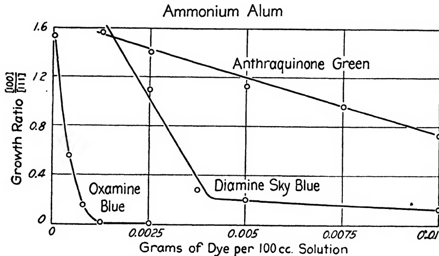
FIGURE 2. Growth ratio—concentration curves for ammonium alum.
