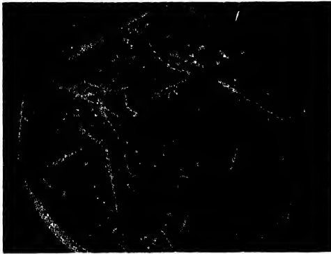
FIGURE 4. Ionization produced in a Wilson cloud chamber filled with a mixture of air, hydrogen and water vapor after bombardment with neutron rays and gamma-rays from the cyclotron. The thin tracks of ions were produced by secondary electrons liberated by the gamma-rays, while the thick and very dense tracks were produced by the recoil protons resulting from collisions of neutrons with the hydrogen atomic nuclei. This picture demonstrates the more localized and intense ionization produced in tissues by neutrons when compared with X-rays or gamma-rays.
