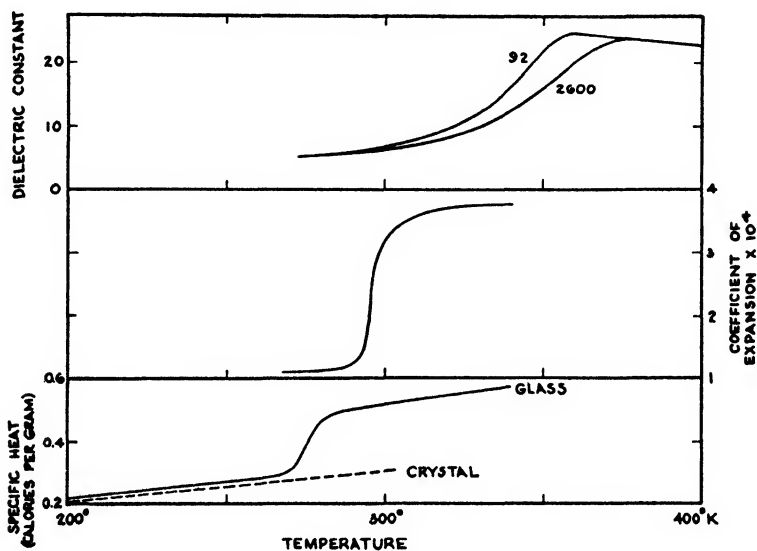
FIGURE 9. Variation with temperature of the specific heat at constant pressure, 81 coefficient of expansion, 81 and dielectric constant 39 (at 92 and 2600 kilocycles per second) of glucose. Data by Parks and co-workers.
