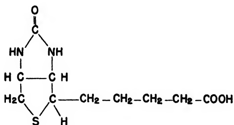
FIGURE 6. Biotin.
