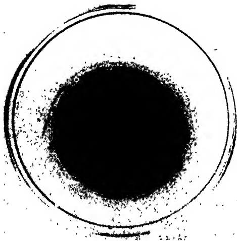
FIGURE 10. Liesegang rings produced on a gelatine film.
