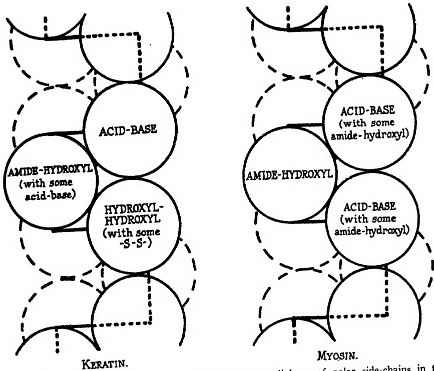
FIGURE 5. Proposed plan for the packing and cross-linkage of polar side-chains in the keratin-myosin series.
