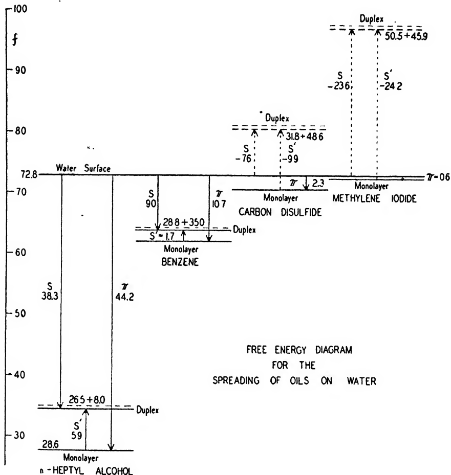
FIGURE 4. Free surface energy ( f ) diagram for the spreading of duplex films and of monolayers on the surface of water. The free surface energy of a duplex film is the sum of that for the interface ( \gamma_{wo} ) and for the surface of the oil ( f_o = \gamma_{wo} + \gamma_o ). The lower of the two energy levels of a duplex film represents oil saturated with water, while the upper level is that when no water is in the surface of the oil. S designates the semi-initial spreading coefficient S'_{i/o} , which may be positive (arrow pointing downward) or negative (arrow pointing upward). S' , which represents the final coefficient ( S'_{i/o} ) is always negative. Obviously if the free energy of a duplex film is above that of water, it will not form; if below that of water it may spread, but is always unstable with reference to the formation of a monolayer (and a lens). For the spreading of water on an oil, the free-energy levels for the duplex film are above that for water (usually by 40 to 110 erg \text{cm}^{-2} ), so water does not spread on an oil as a duplex film. Thus, except for the greater height of the duplex level the diagram is like that for methylene iodide.
