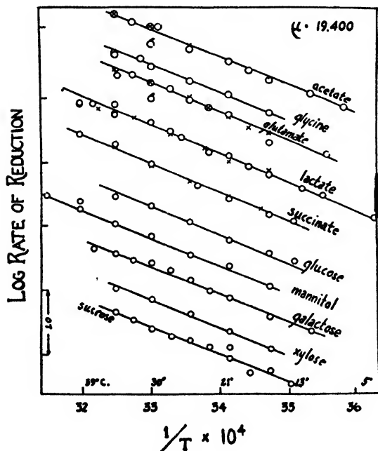
FIGURE 7. Log of rate of reduction (calculated from the time required for 75 per cent reduction of methylene blue) in presence of various substrates by a suspension of Escherichia coli plotted against 1/T . \mu in the Arrhenius equation = 19,400. \circ refers to the series of determinations made with a first bacterial preparation; \times to determinations made with second separate bacterial preparations. For lactate \times refers to determinations made with a preparation consisting of autolyzed cells. From Gould and Sizer. 16
