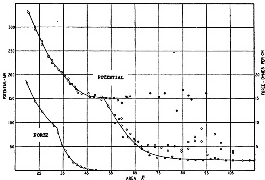
FIGURE 23. Pressure-area and potential-area of myristic acid monolayers. At areas greater than 52 \text{ \AA}^2 \text{ molecule}^{-1} the film is heterogeneous (gaseous and liquid-expanded).
