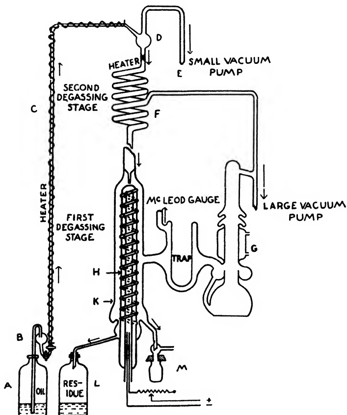
FIGURE 4. Laboratory falling-film still.
