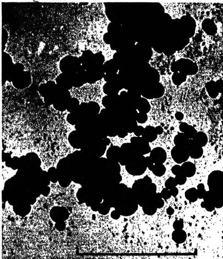
FIGURE 26. P-33 Carbon. Mean particle diameter, 74 \mu . (Magnification 50,000 diameters). 54 (Courtesy Columbian Carbon Co.)
