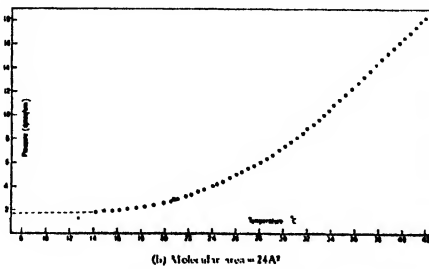
FIGURE 49b. Pressure-temperature relations of palmitic acid monolayers (condensed and intermediate phases).
