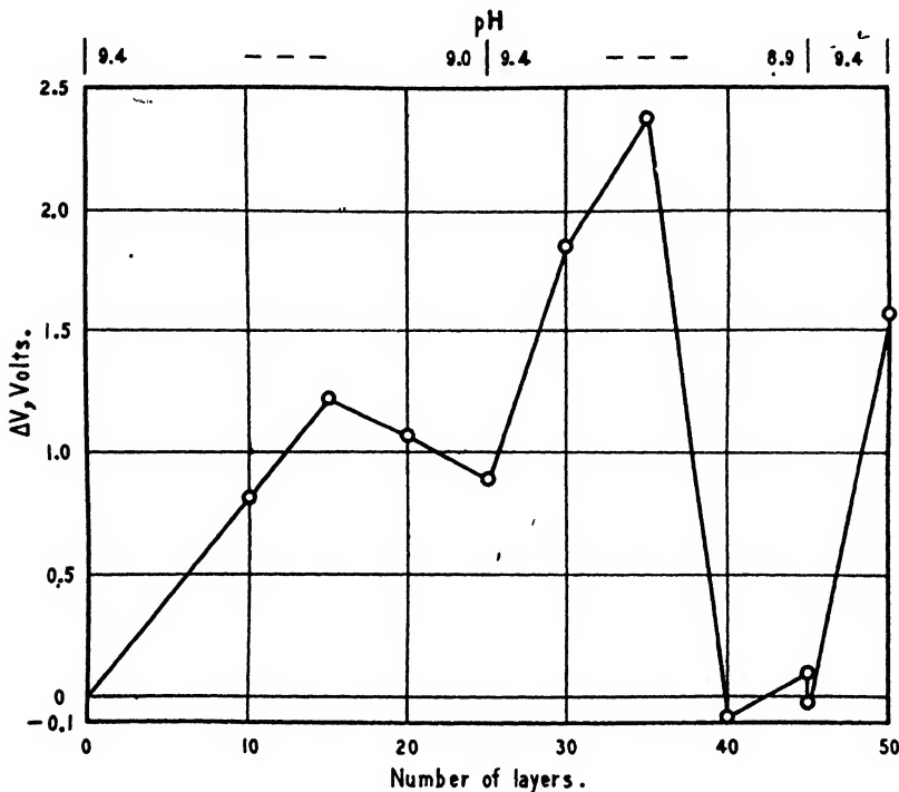
FIGURE 55. Effect of pH on film potentials.
