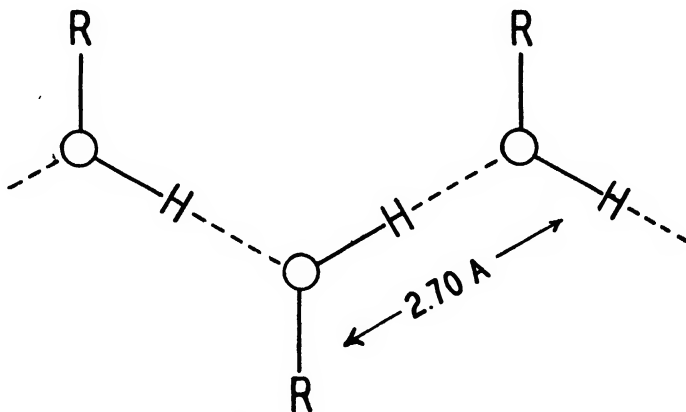
FIGURE 57. Hydrogen bonds in alcohol.
