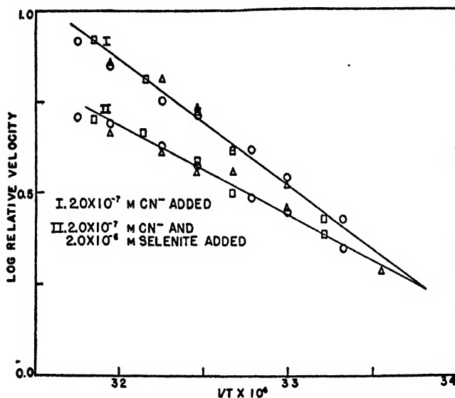
FIGURE 14. Arrhenius equation plot of a group of experiments on enzyme poisoned with cyanide and with cyanide plus selenite. From Hadidian and Hoagland. 17 I : \mu = 16,000 ; II : \mu = 11,400 .
