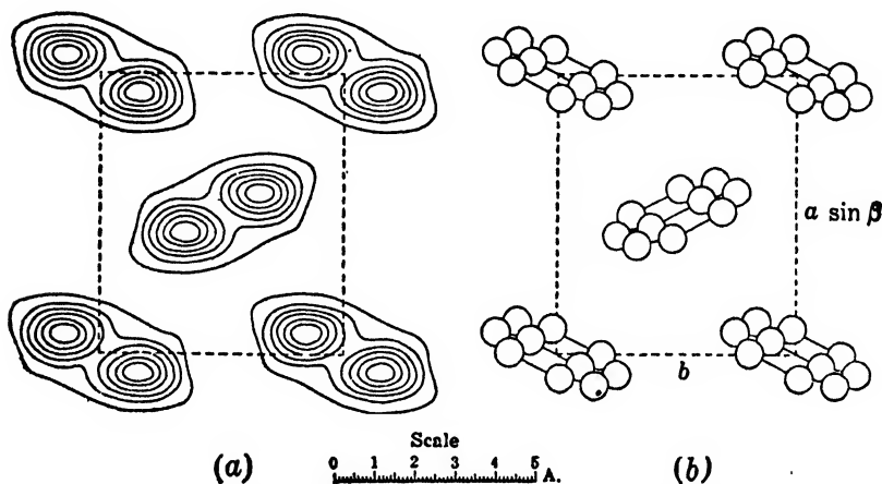
FIGURE 5. Projection of Naphthalene Along the c Axis. Each Contour Line Represents two Electrons per Å. 2 (J. M. Robertson.)
