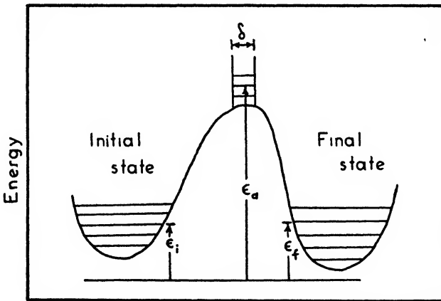
Distance along the reaction coordinate FIGURE 1. The energy relations of a reacting system.
