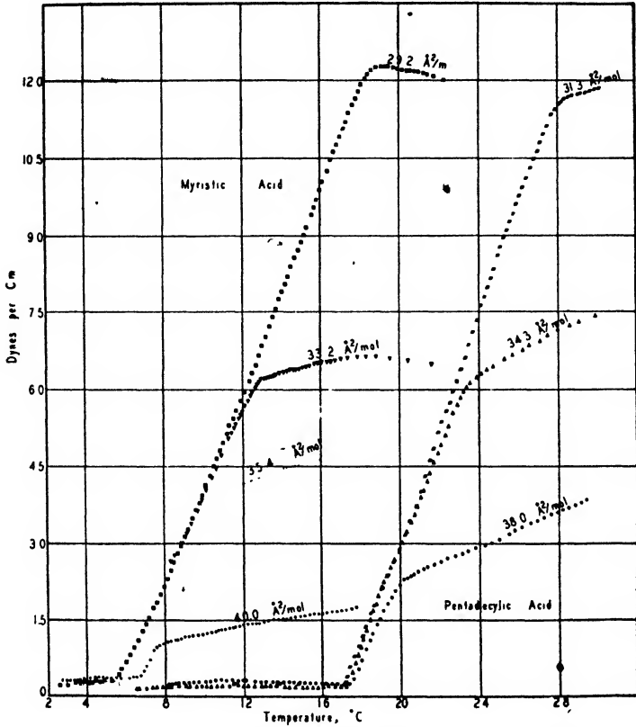
FIGURE 49a. Pressure-temperature relations of monolayers of myristic and pentadecylic acids. From left to right: L_c , I , and L_s phases. The upper part of the highest curve for myristic acid has a slope of incorrect sign, since at this high temperatures and pressures myristic acid monolayers are slightly soluble.
