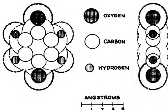
FIGURE 1. Van der Waals' projective areas of the dihydroquinonate ion (1) flat, (ii) oriented edge-on.
