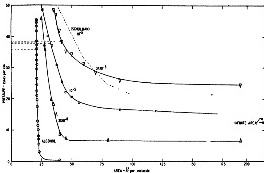
FIGURE 40. Pressure-area relations of equilibrium of monolayers of cetyl alcohol after penetration of molecules of sodium cetyl sulfate from aqueous solution of molal concentrations: 3 \times 10^{-6} ; 1 \times 10^{-5} ; and 3 \times 10^{-5} at 25^\circ \text{C} . Harkins, Gordon, and Copeland, with dotted curve by Schulman at 1 \times 10^{-5} \text{ m} for comparison. Schulman's values do not represent equilibrium, but only "one minute points."
