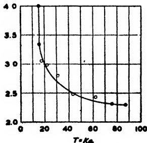
FIGURE 6. Lateral distance between parallel tobacco mosaic virus rods in an equilibrium gel plotted as a function of the (\text{NH}_4)_2\text{SO}_4 concentration. (From Bernal and Fankuchen. 11 )
