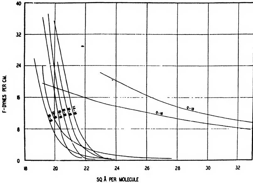
FIGURE 45. Mixtures (1:1) of condensed alcohol and vapor-expanded amine films ( \text{pH} = 3 ). For the one-component alcohol films see Fig. 42 and Fig. 43. The curves at the lower pressures are of the transition type. The first number gives the number of carbon atoms in the alcohol, and the second in the amine, molecule. The 14-16 and 18-16 mixtures have a high compressibility.
