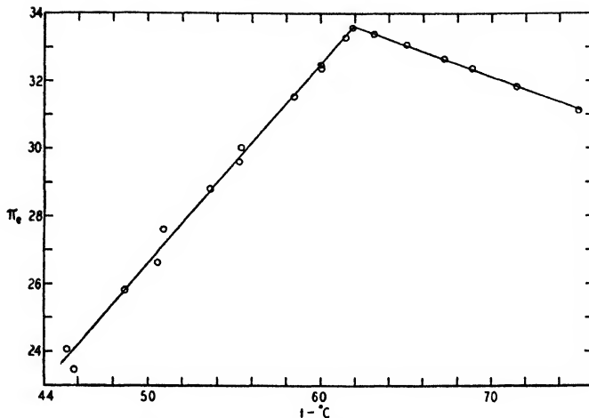
FIGURE 49b. Effect of Temperature on the equilibrium pressure of crystals ( t = 44^\circ to 61.8^\circ \text{C} ) and of Lenses ( t = 61.8 to 73^\circ \text{C} ) of palmitic acid.
