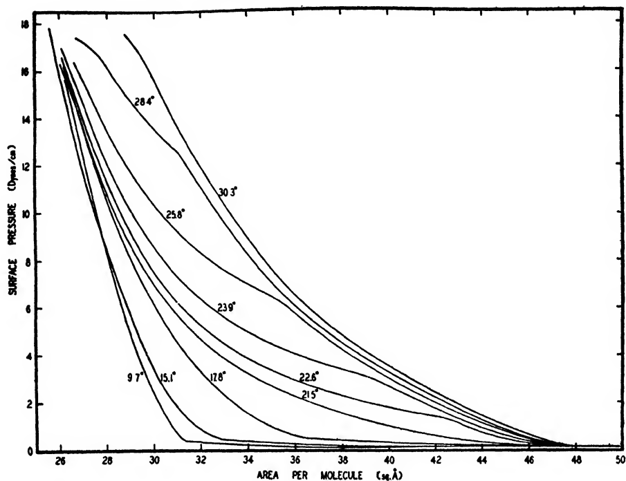
FIGURE 12. Monolayers of octadecane-nitrile on water. The intermediate phase exhibits a lower compressibility than that of the acids.
