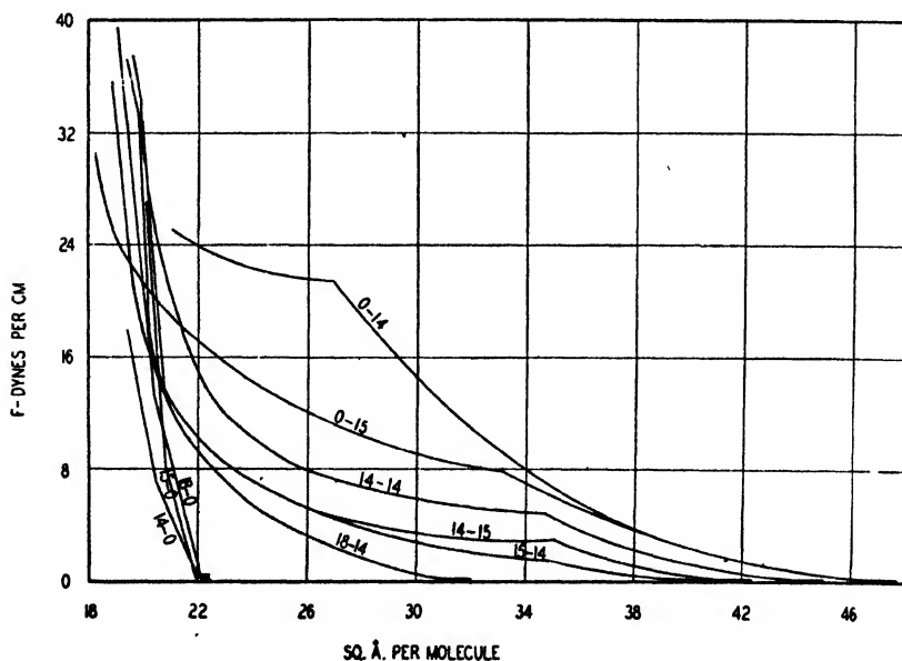
FIGURE 43. Mixtures (1:1) of condensed alcohol films and expanded films of myristic acid ( \text{pH} = 3 ). The curve for myristyl alcohol with pentadecylic (acid 14-14) is added for comparison with the effect produced with interchange of number of carbon atoms in the alcohol and acid). Stearyl alcohol does not condense the myristic acid, while it does the pentadecylic acid film (Figure 42).
