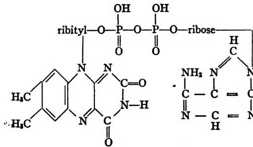
Riboflavin-adenine dinucleotide
