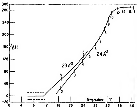
FIGURE 49d. Increase of the "Heat Content" for spreading h_s = (\partial H_s / \partial T)_{p, T, \sigma} as a function of temperature and pressure; numbers on curves give the film pressure \pi .
