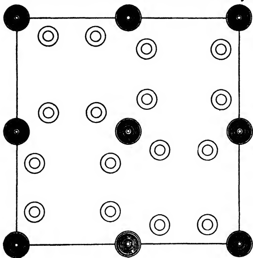
FIGURE 6B. Potassium dihydrogen phosphate ( \text{KH}_2\text{PO}_4 ). Contour map, 24 representing the electron density projection onto the XY plane, calculated from experimental F_{hkl} values by Equation 4.
