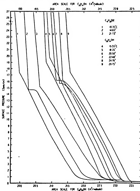
FIGURE 14b. Pressure-area temperature relations for the normal long-chain paraffin alcohols with 19 and 20 carbon atoms in the chain. The temperature of the first-order transition increases 5° while the pressure rises about 2 dyne cm -1 for each additional carbon atom. Correction: Multiply Film Pressures by 0.9315.
