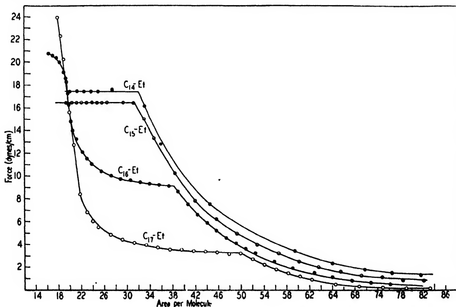
FIGURE 7. General phase diagram at temperatures above T_0 for the liquid expanded phase: ethylesters at 25° C.
