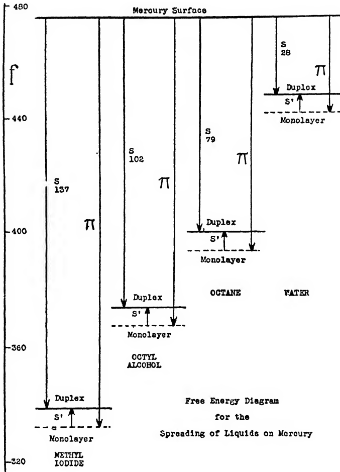
FIGURE 5. Water and all organic liquids have positive initial spreading coefficients on mercury, and thus may spread to form duplex films. The monolayers lie at a lower free energy level, so the duplex film, if formed, transforms into a monolayer and a lens. The free energy levels of the duplex films are known and are properly placed in the diagram. Those for the monolayers have not been determined, so only the sign of the final spreading coefficient ( S' ) is known. While the film pressure is larger than the initial spreading coefficient, it is probable that it is not very much larger, so the diagram gives the general location of the free-energy level for each monolayer.
