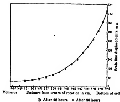
FIGURE 16. Sedimentation equilibrium experiment on bushy stunt virus. (From McFarlane and Kekwick. 62 )
