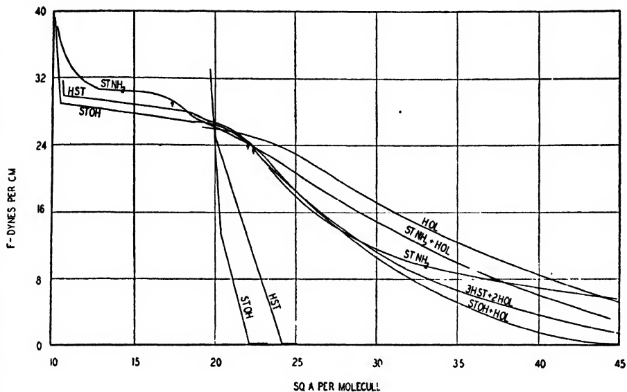
FIGURE 37b. Pressure-area relations of an oleic acid monolayer, and of mixtures of oleic acid (HOI) with stearyl alcohol (St(OH)), stearic acid (HSt), and stearyl amine ( \text{StNH}_2 ) on a subsolution of pH 3. The arrows represent the points at which lenses of oleic acid become visible in the ultramicroscope. Since at the extreme left all of the oleic acid has been squeezed out the figure has been drawn in such a way that the values of the area multiplied by two give the areas for the constituent left in the film: e.g. , the almost vertical line at 10.5 \text{ \AA}^2 for the mixture of oleic acid and stearyl alcohol indicates that the molecular area for the alcohol left alone in the film is 21 \text{ \AA}^2 .
