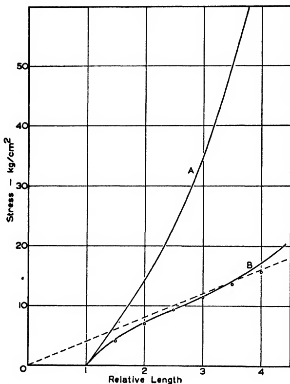
FIGURE 6. Curve A. True stress vs. nominal relative length for an accelerated pure gum stock. Curve B. Nominal stress vs. nominal relative length corresponding to Curve A. The circles are theoretical values according to Equation (31). The dashed line represents the asymptote of the theoretical curve.
