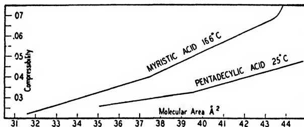
FIGURE 27. Variation of the compressibility of liquid-expanded ( L_e ) monolayers with molecular area.
