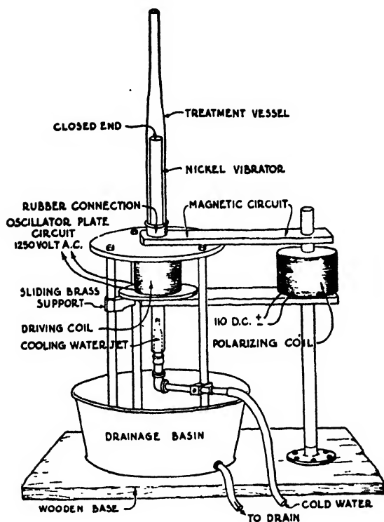
FIGURE 3. Magnetostriction sound generator.
