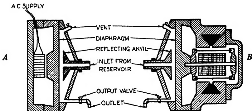
FIGURE 4. Two types of electromagnetic sound generators.
