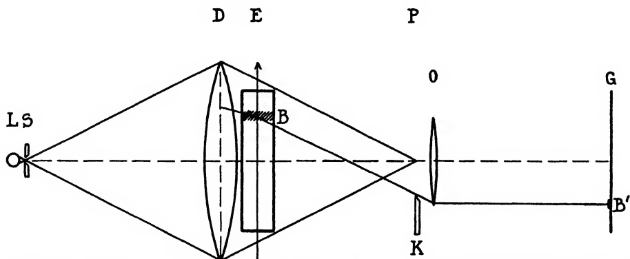
FIGURE 4. Arrangement for observation of the boundaries by the simple schlieren method.
