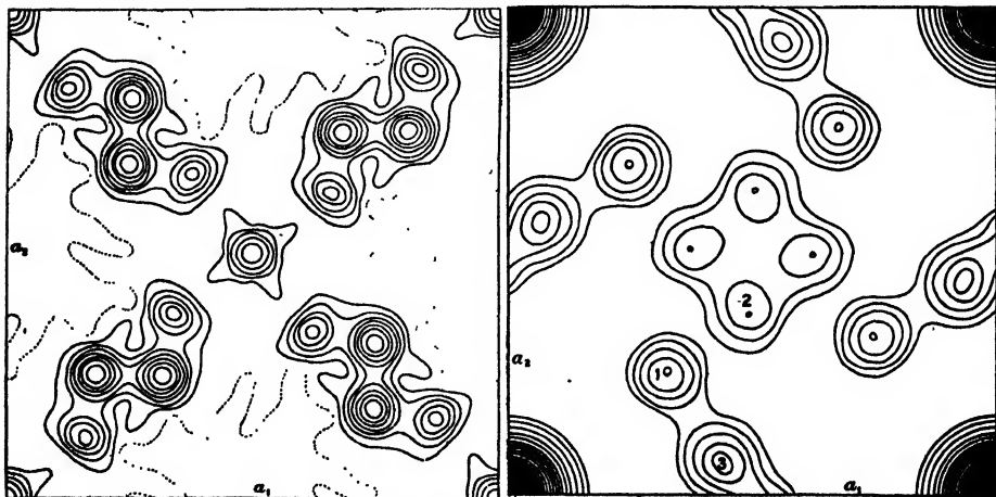
FIGURE 9C. Pentaerythritol. Contour map 17 representing the electron density distribution, projected onto the XY plane (Equation 4).
