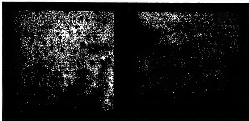
FIGURE 10. Electron micrographs of Lippmann emulsion, before and after development.
