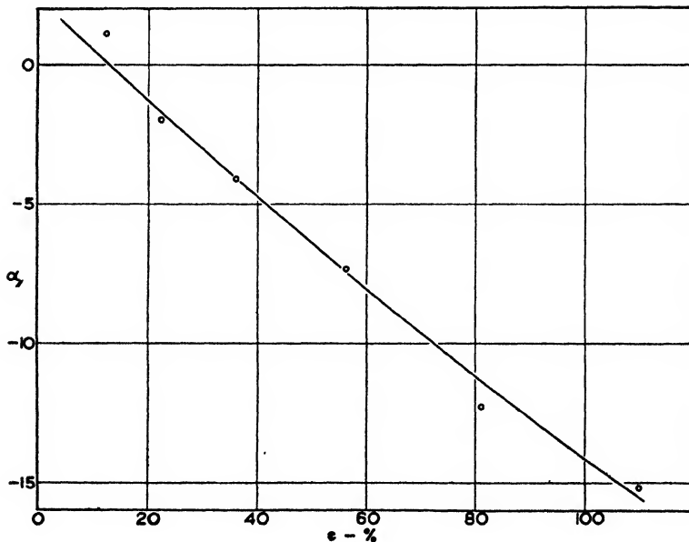
FIGURE 2. Linear thermal expansion coefficient \alpha_L , parallel to the direction of the stress as a function of the strain \epsilon according to Joule.
