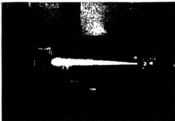
FIGURE 2. The 16 million electron-volt deuteron beam emerging from the cyclotron chamber into the air. An indication of its size may be gained from noting the meter stick placed below the beam.
