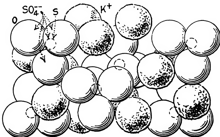
FIGURE 5. Model of potassium sulfate. Side elevation (100) plane.
