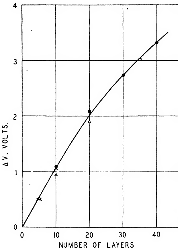
FIGURE 52. Film potentials of five different X multilayers on gold made from solutions 1(0, X), 2( \Delta , \square ), and 3( \bullet ). The potential increment is about 100 mv/layer up to 20 layers.
