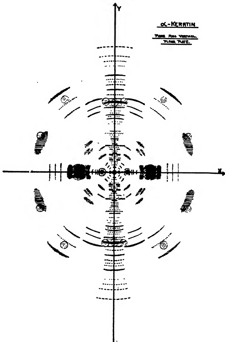
FIGURE 7. Composite diagram of the \alpha -keratin diffraction pattern given by porcupine quill (Cu K\alpha rays). The spacing of the most prominent arc on the meridian is 5.14, Å (MacArthur).
