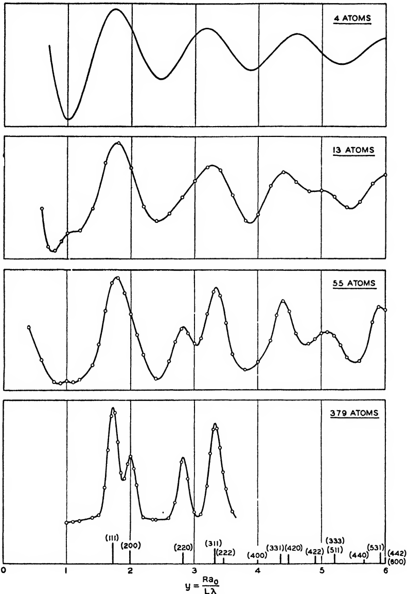
FIGURE 4. Theoretical scattering curves from randomly oriented face-centered cubic crystals made up of various numbers of atoms.
