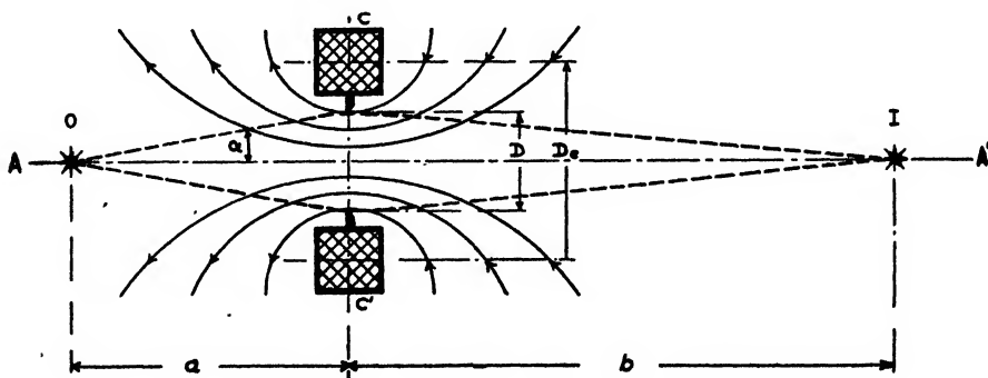
FIGURE 1a. Simple magnetic electron lens.
