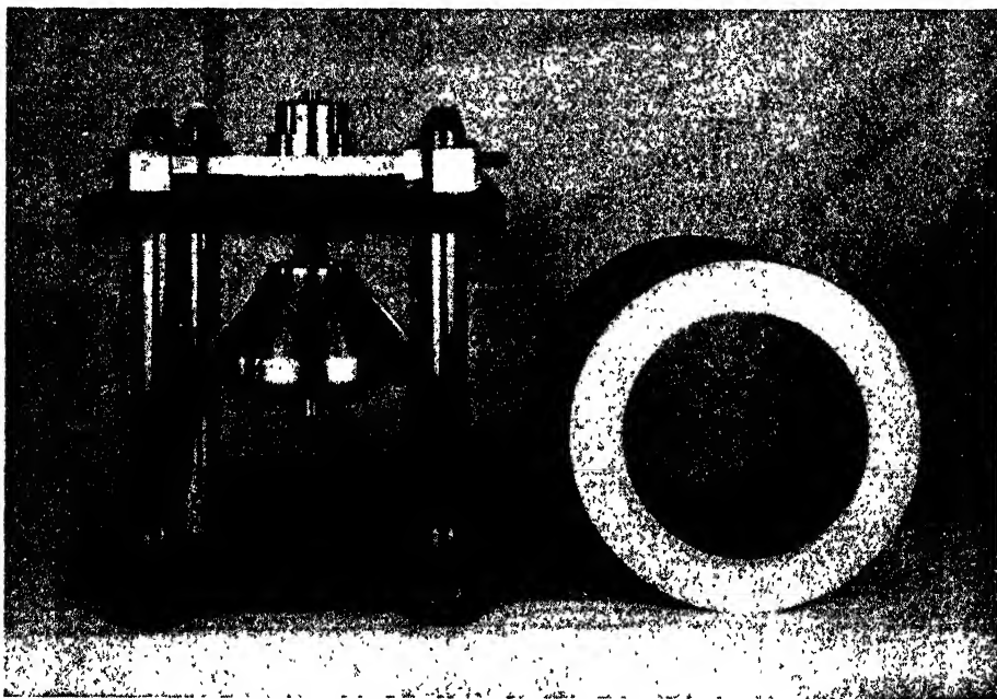
FIGURE 5. Photograph of a high-speed angle centrifuge of the vacuum type, with the cylindrical section of the steel vacuum chamber shown removed for the purpose of illustration. The turbine is driven and supported by compressed air. Rotors similar to the 20 cm one shown can be operated near 50,000 rpm. For the ultracentrifuge, top and bottom plates of the vacuum chamber are provided with windows to permit the passage of a light beam vertically through the revolving cell.
