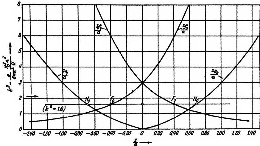
FIGURE 2. Principal points H_0 , H_1 and focal points F_0 , F_1 as functions of the parameter k^2 of strong magnetic lenses having the axial field distribution H(z) = H_0 \sqrt{1 + z^2/a^2} . The focal lengths are given by the relations: f_0 = z_{H_0} - z_{F_0} ; f_1 = z_{H_1} - z_{F_1} . 60
