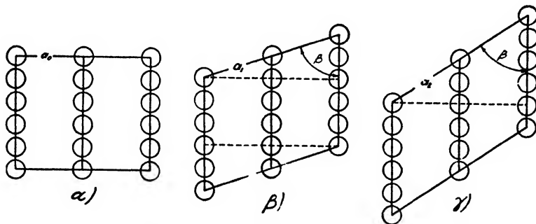
FIGURE 2. Alternative Methods of Packing of Hydrocarbon Chains: a = a_0/\sin \beta ; b = b_0 ; c = c_0 \sin \beta . [After Schoon, T., Z. physik. Chem. , B39, 385 (1938).]
