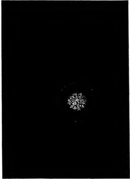
FIGURE 2. X-ray spectrogram of high quality carbonado (unfiltered Mo radiation; distance 5 cm) Courtesy G. L. Clark.
