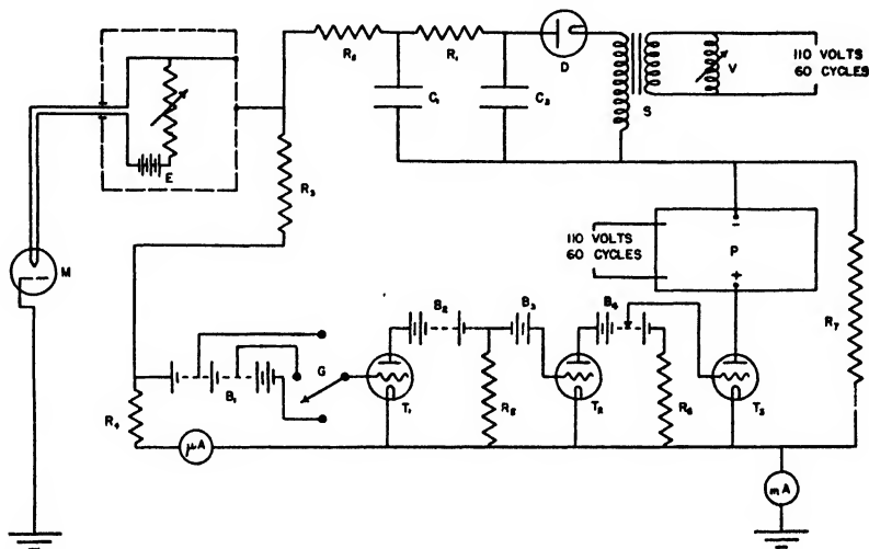
FIGURE 12. Circuit of the stabilized 60-cycle high-voltage power supply used with the Ohio State University electron microscope.
