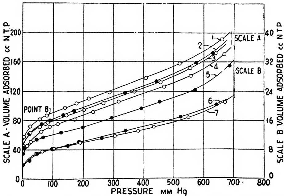
FIGURE 1. Adsorption of Nitrogen on Carbon Blacks at Liquid Nitrogen Temperatures.
