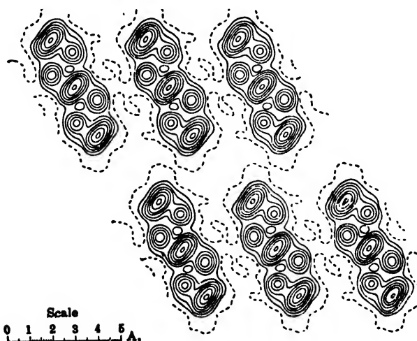
FIGURE 4. Projection of Naphthalene Molecules Along the b Axis, showing Mutual Relation of Molecules. Each Line Represents One Electron per \text{\AA}^2 (J. M. Robertson.)
