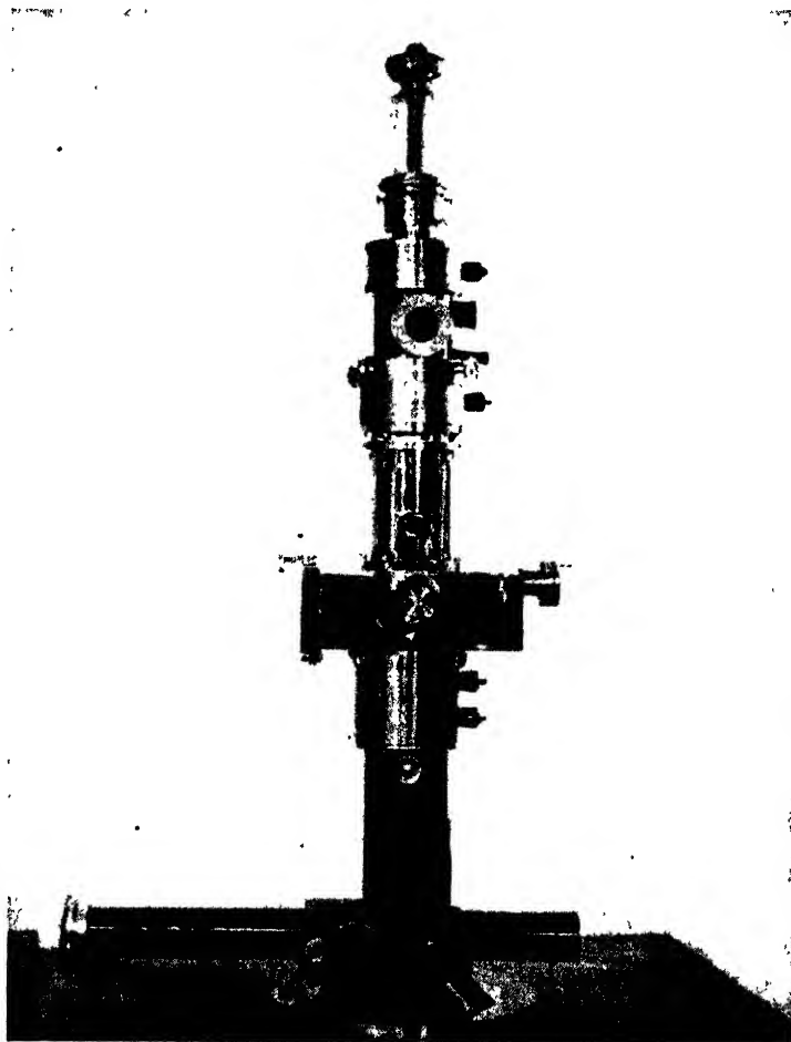
FIGURE 11a. Magnetic electron microscope constructed in the Radiation Laboratory of the Ohio State University in 1940.
