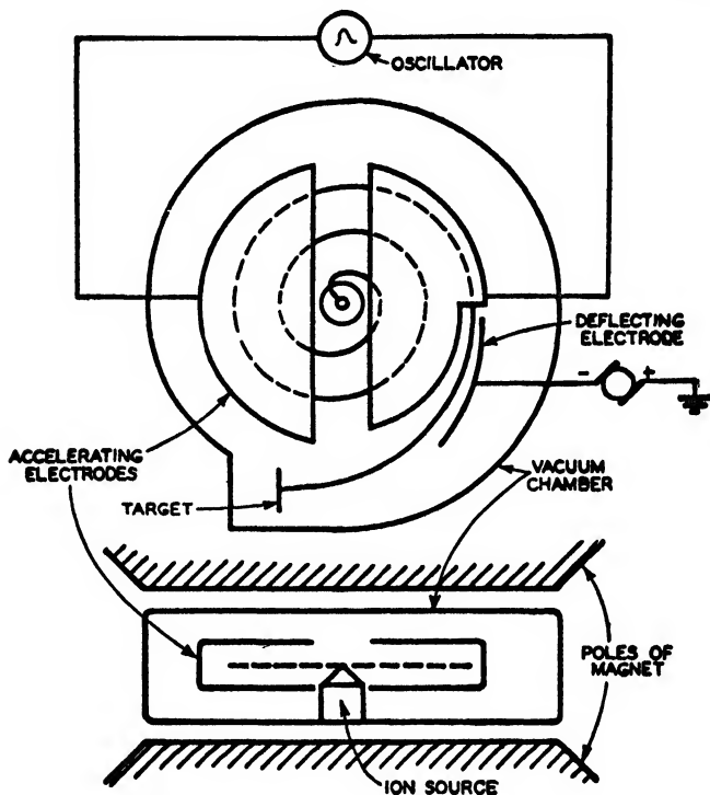
FIGURE 1. Schematic diagram of the cyclotron.
