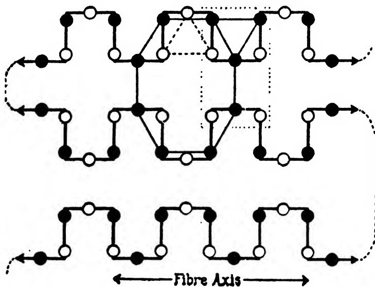
FIGURE 3. Packing of side-chains in the \alpha -fold of the keratin-myosin group. — represents the direction of the main-chains; ● represents a side-chain pointing up from the plane of the diagram; ○ represents a side-chain pointing down from the plane of the diagram.
