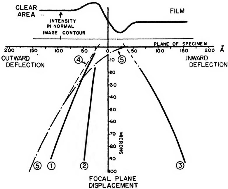
FIGURE 10b. Deflections of intensity extrema. Curve 1—normal image contour maximum (measured); curve 2—out-of-focus minimum (measured); curve 3—out-of-focus maximum (measured); curve 4—first maximum of Fresnel straight edge diffraction pattern displaced by spherical aberration; curve 5—theoretical deflection of first maximum of Fresnel diffraction pattern.
