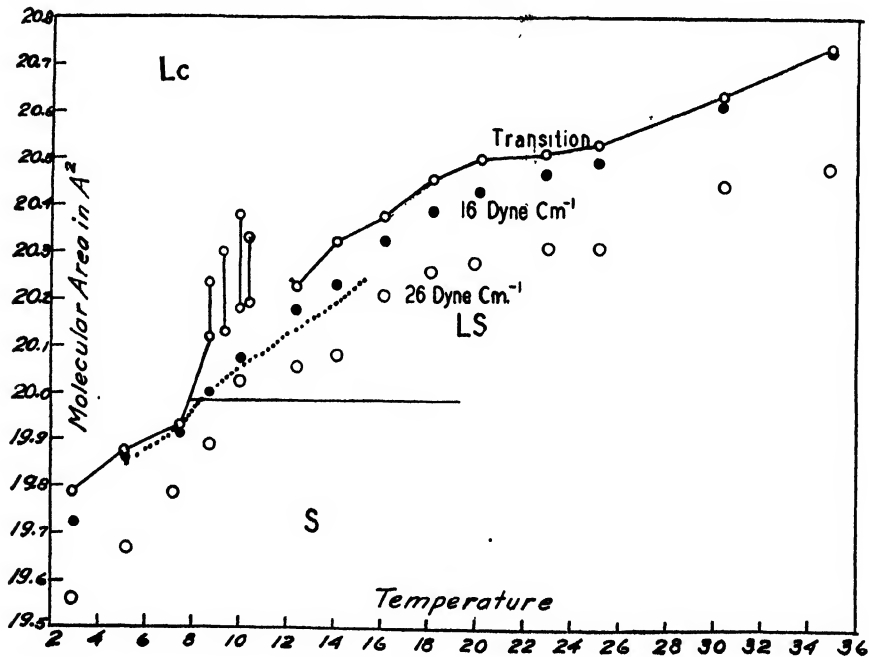
FIGURE 16. Molecular area-temperature values for the phase boundaries of condensed monolayers of octadecanol. The dotted line gives values at 16\text{ dyne cm}^{-1} as obtained by increase of the temperature of a monolayer. The black circles give values at the same pressure, from the isotherms. Multiply P by .93.
