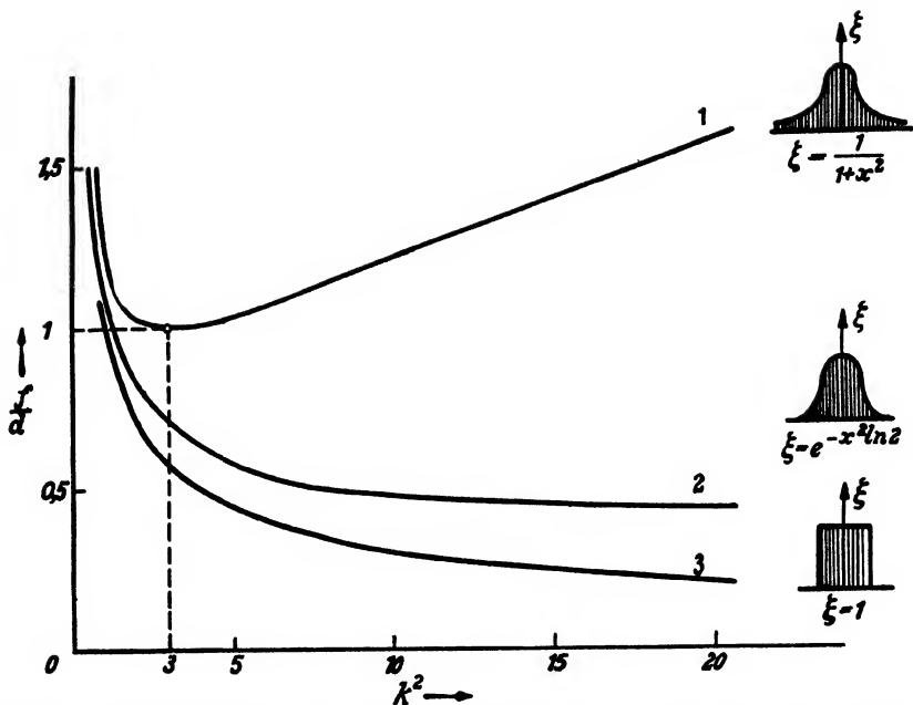
FIGURE 4. The focal length f ( f_o or f_i ) of a magnetic lens as a function of the parameter k^2 . Curve 1: with the field H(z) = H_o / (1 + z^2/a^2) ; curve 2: with the more sharply defined field H(z) = H_o \exp(-z^2/a^2) ; curve 3: with the ideal most sharply defined field H(z) = H_o ( -d < z < d ), H(z) = 0 ( z < -d , z > +d ). 57
