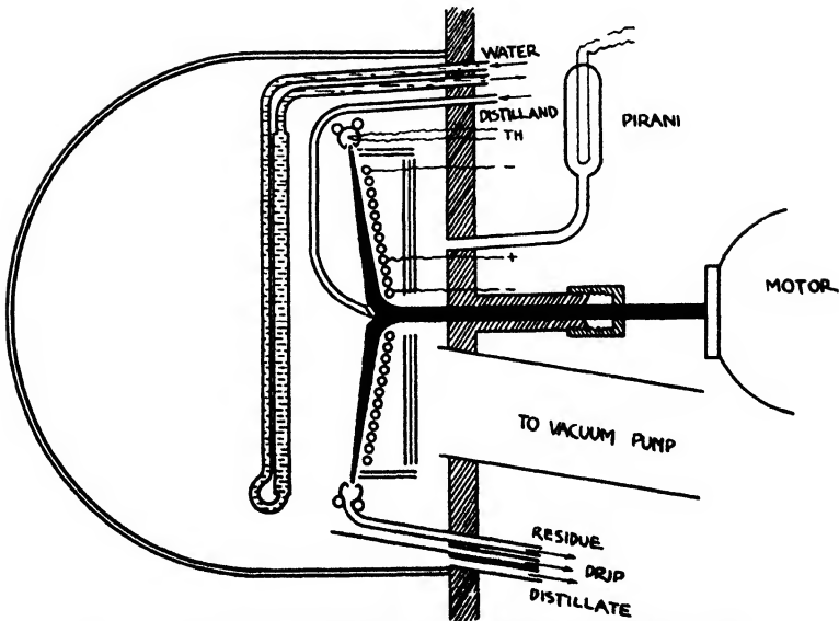
FIGURE 6. Sectional elevation of a centrifugal molecular still.
