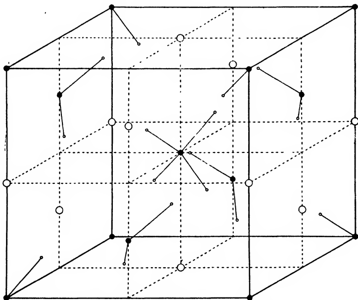
FIGURE 6A. Potassium dihydrogen phosphate ( \text{KH}_2\text{PO}_4 ). Distribution of atomic centers in the unit cell. Large open circles represent potassium; filled circles, phosphorus; small open circles, oxygen.
