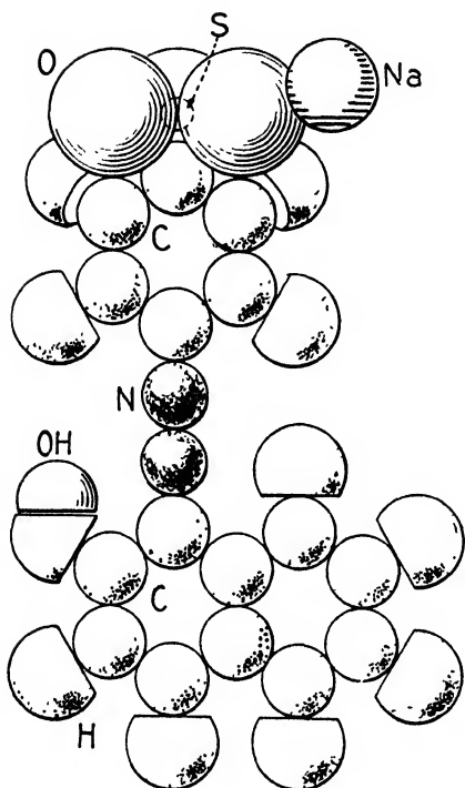
FIGURE 4. Model of dye P- \beta OH.
