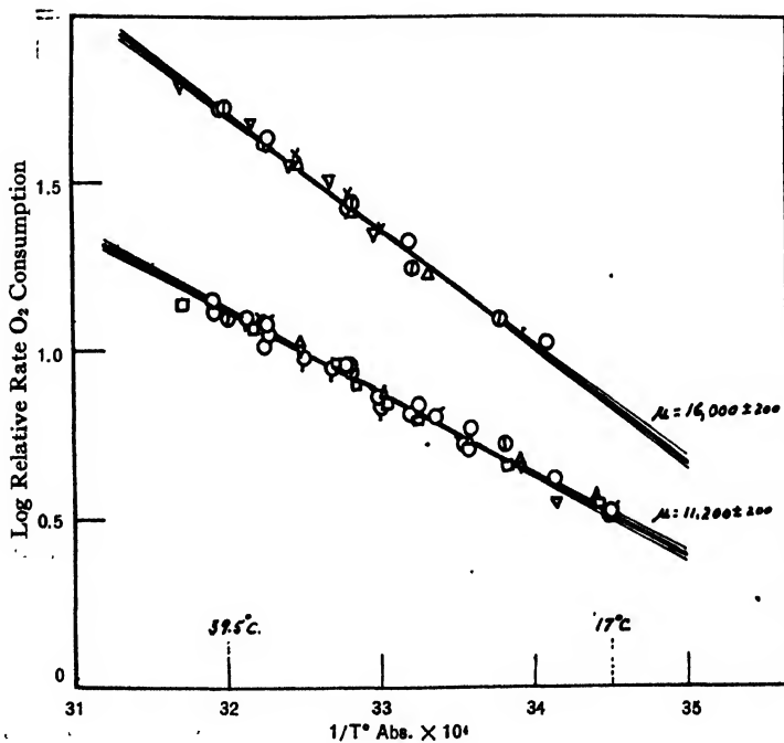
FIGURE 15. Composite massed plot for the enzyme experiments described in the text (compare with Fig. 10). Mean heavy lines are drawn by eye through the data; the lighter lines fanning out are for \pm 200 calories around the means.
