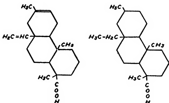
FIGURE 26. Structural formulas of the pimeric acids.
