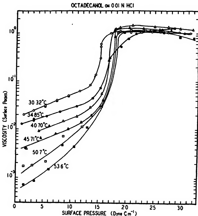
FIGURE 33. Viscosity relations of the liquid condensed and LS phases of octadecanol between 30^\circ and 54^\circ C. The extremely abnormal relations of Figures 31 and 32 have disappeared, since the viscosity again falls with rise of temperature. It is remarkable that identical values of viscosity and pressure occur at three different temperatures. Multiply all pressures for alcohols by 0.931.
