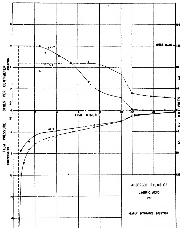
FIGURE 34. Effect of time on the film pressure and surface potential of solutions of lauric acid.
