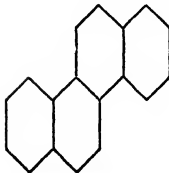
Chrysene
