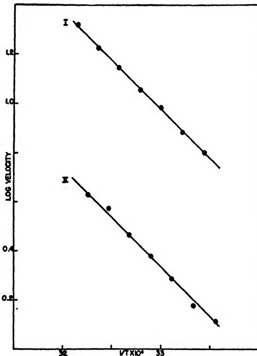
FIGURE 18. Curve I. Arrhenius plot for oxygen-consumption curves using dye-substituted enzyme as described in the legend to Fig. 17. Curve II. Arrhenius plot using one-tenth as much enzyme but the same amount of cresyl blue. From Hadidian and Hoagland. 18
