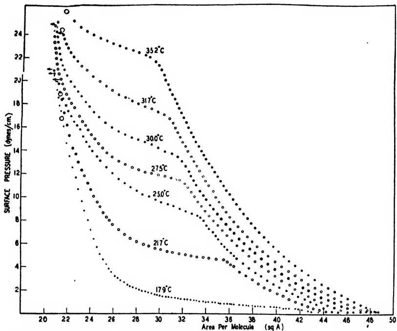
FIGURE 10. Liquid monolayers of pentadecylic (15-carbon) acid. The arrows indicate collapse.
