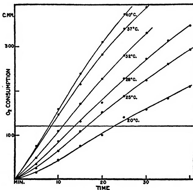
FIGURE 11. Reaction curves for a single experiment with unpoisoned enzyme at different temperatures. The horizontal line indicates the points at which velocities were measured. From Hadidian and Hoagland. 17
