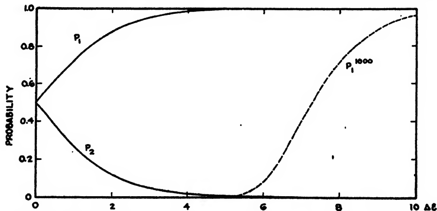
FIGURE 3. The probabilities of two states, in equilibrium with each other, as functions of \Delta\epsilon . The probability of the simultaneous existence of 1000 independent subsystems (all having the same value of \Delta\epsilon ) is also shown (dotted line).
