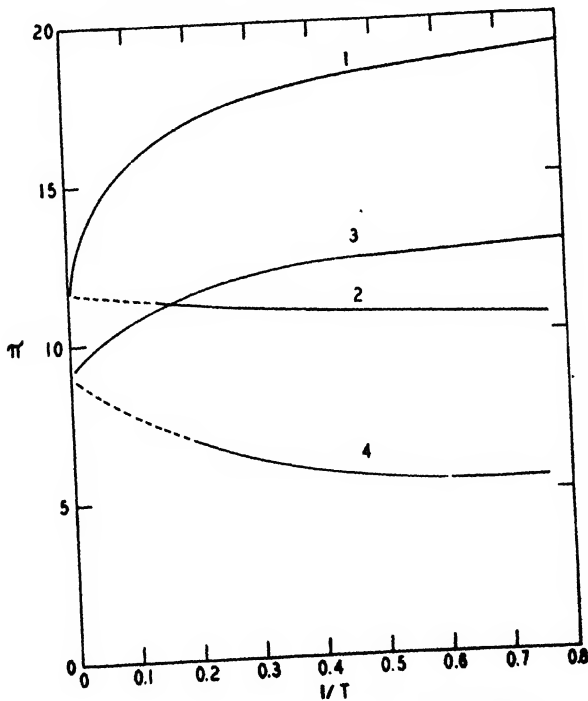
FIGURE 35c. Film pressure vs reciprocal of the time.
