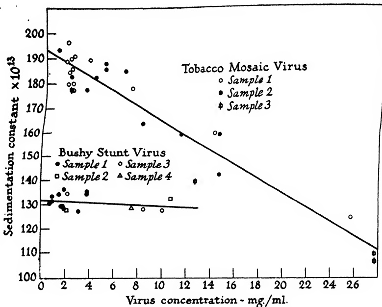
FIGURE 7. Sedimentation constant plotted as a function of tobacco mosaic virus concentration. (From Lauffer. 44 )
