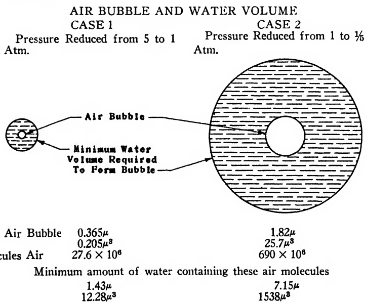
FIGURE 1. Relative size of the air bubbles and the water volume from which the molecules must come.
