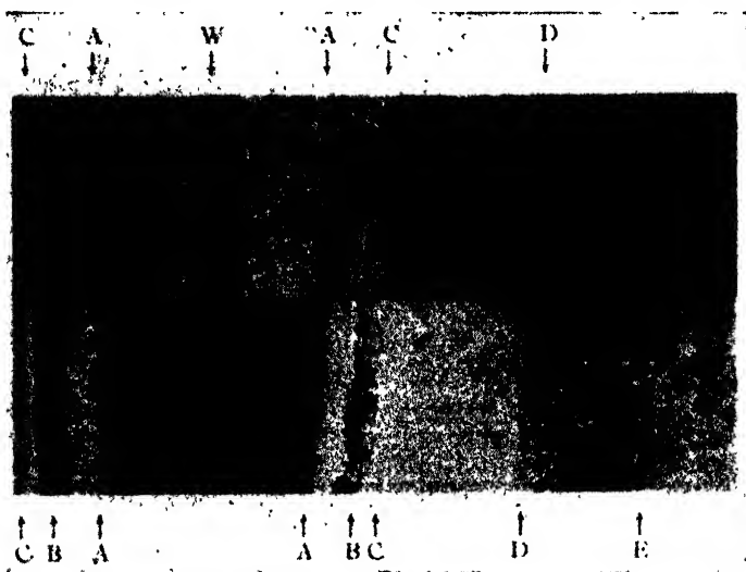
FIGURE 4. Photomicrographs of sodium stearate by the hot-wire technique. Five of the six phases of sodium stearate appear successively as the temperature falls from about 350^{\circ} near the wire (W) to about 140^{\circ} at the right-hand edge of the photograph. A, boundary between isotropic liquid and neat soap; C, boundary between neat soap and subneat soap; D, boundary between subneat soap and superwaxy soap; E, boundary between superwaxy soap and waxy soap. The upper photograph was taken with the Micropolychromar, the lower, showing an adjacent portion of the same field of view, with crossed polaroids. Magnification is about 20 fold. At B the neat soap has begun to become oriented, simulating the appearance of isotropic liquid. [From Vold, M. J., Macomber, M., and Vold, R. D., J. Am. Chem. Soc. , 63, 168 (1941).]
