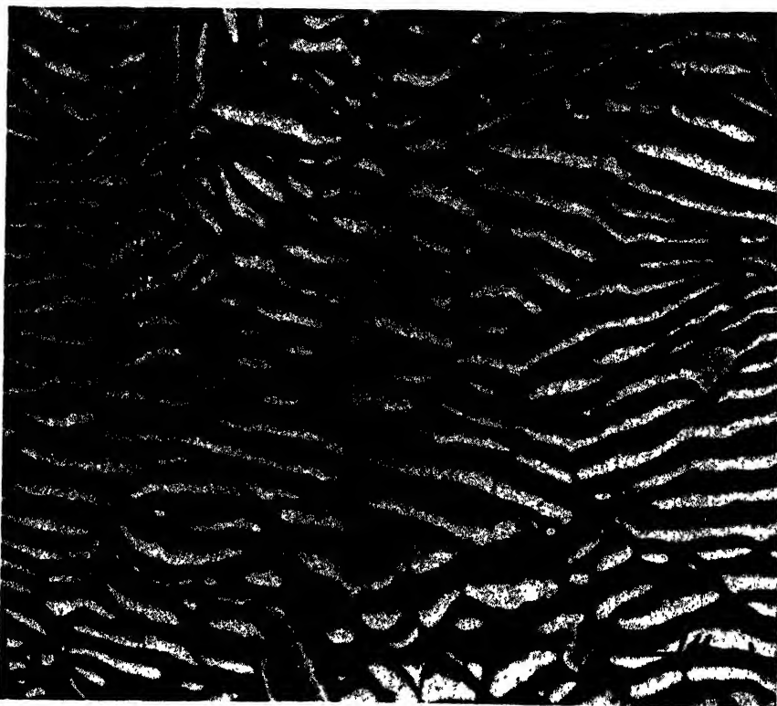
FIGURE 32. Replica of Pearlite structure prepared by initial single replica process of Schaeffer and Harker. 148 Opaque areas represent depressions; transparent areas represent elevations in original sample. The diffuse light lines are thought to represent strains in the replica. (Courtesy General Electric Co.)
