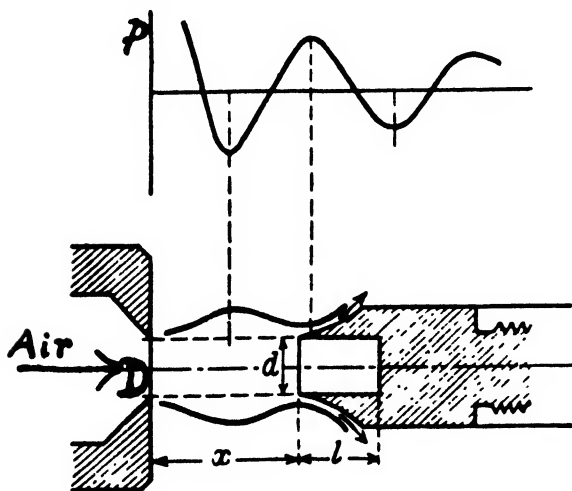
FIGURE 5. Gas-current sound generator.
