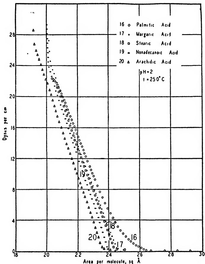
FIGURE 13. Effect of increasing chain length in decreasing the molecular area in liquid condensed ( L_c ) monolayers of the long chain acids of from 16 to 20 carbon atoms.
