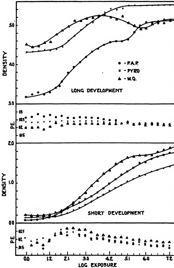
FIGURE 16. P.E.—photometric equivalent for different developers for long and short development.
