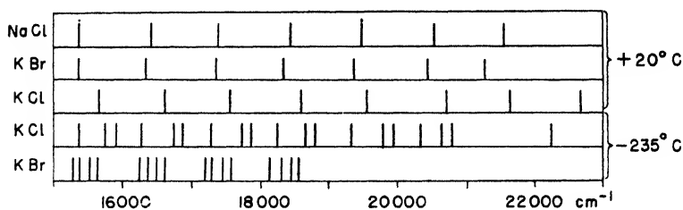
Fig. 209. Luminescence spectra of oxygen-activated alkali halides (Honrath).
