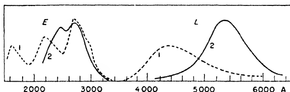
Fig. 211. Excitation and emission bands E and L of (1) calcium tungstate and (2) magnesium tungstate.
