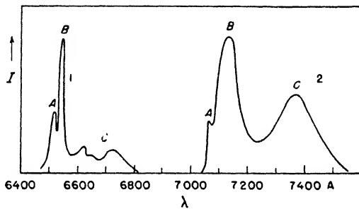
Fig. 210a. Fluorescence spectra of \text{Mg}_2\text{TiO}_4 activated (1) with \text{Mn}^{4+} and (2) with \text{Cr}^{+++} (Kroeger, Deutschbein).
