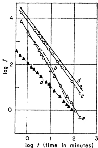
Fig. 188. Hyperbolic decay curves of various sulfide phosphors (Levshin, Randall).
