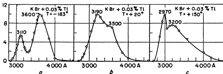
Fig. 205. Emission bands of a KBr(Tl)-phosphor at various temperatures (von Meyereren).
