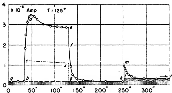
Fig. 175. Activating and deactivating photoelectric current in discolored NaCl at 125° C (Gudden and Pohl). Time in seconds.
