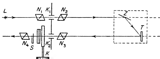
FIG. 3. Kerr-cell fluorimeter [Szymanowski (1623)].
