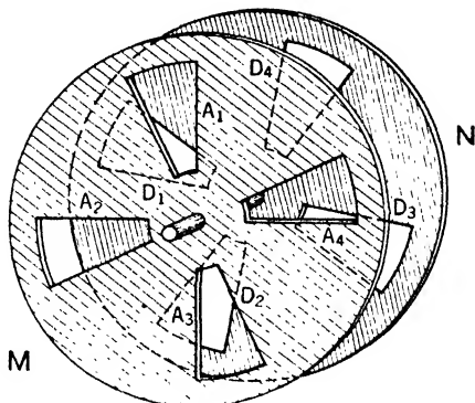
FIG. 2. Becquerel phosphoroscope.
