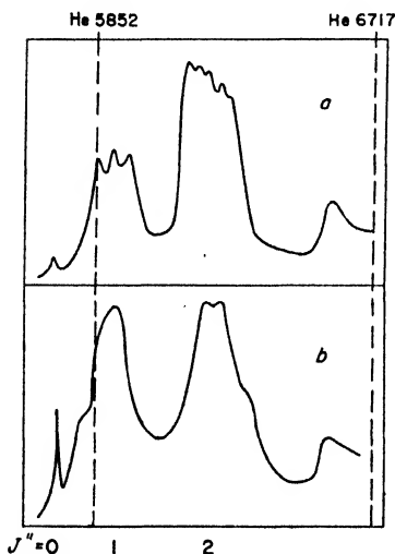
Fig. 158. Fluorescence band of trivalent europium (Tomaschek) a : in a glass. b : in aqueous solution.
