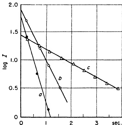
Fig. 97. Decay of the luminescence of tryptaflavine adsorbed on silica gel (Pringsheim and Vogels). a : green phosphorescence at +39^{\circ}\text{C} . b : the same at -18^{\circ} . c : orange slow fluorescence at -180^{\circ}\text{C} .
