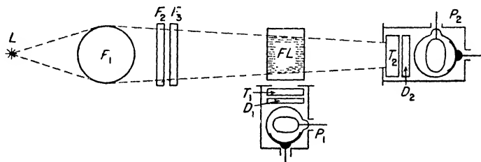
FIG. 6. Heterochromatic photometer (Bowen).
