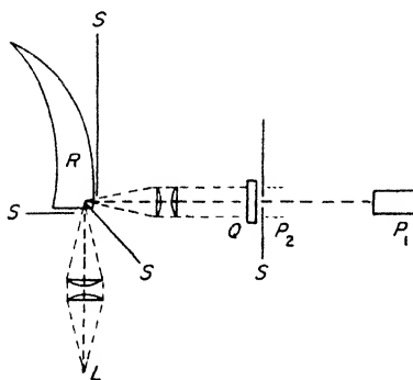
Fig. 47. Zemanski's apparatus for the determination of quenching cross sections.
