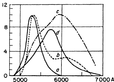
Fig. 201. Emission bands of zinc silicate phosphors (Kroeger; Leverenz).
