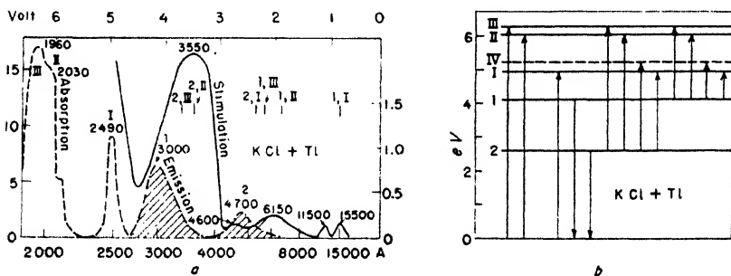
Fig. 180. Absorption, emission, and stimulation of a KCl(Tl)-phosphor (Buenger and Flechsig).
