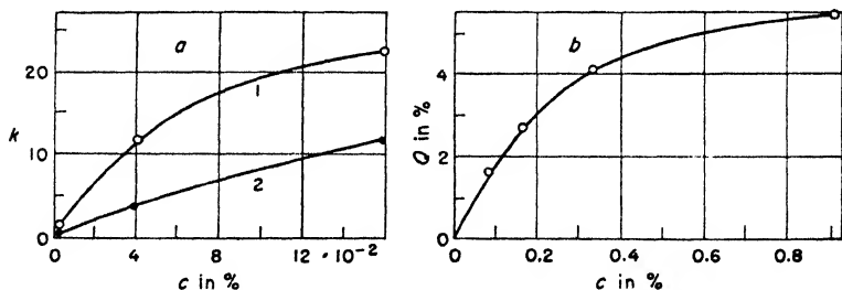
Fig. 192. Absorption coefficient k and phosphorescence yield Q of a KCl(Tl)-phosphor as a function of the Tl-concentration c .
