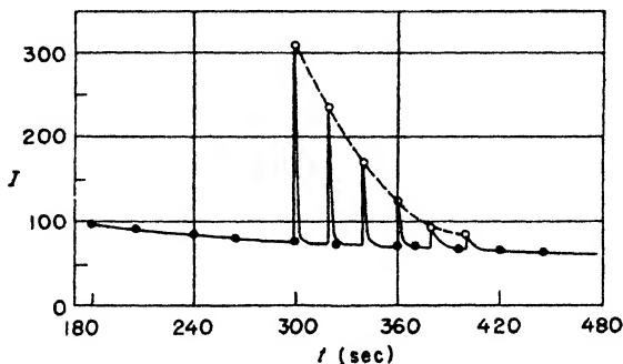
Fig. 178. Instantaneous enhancement of the phosphorescence of a ZnS(Mn)-phosphor by application of an electric field (Hinderer).
