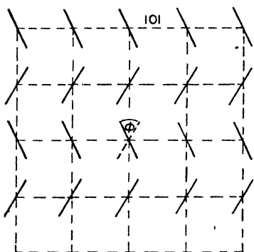
Fig. 132. Orientation of oscillators in anthracene crystals (Obreimow, Prikhotjko, and Shabalda).
