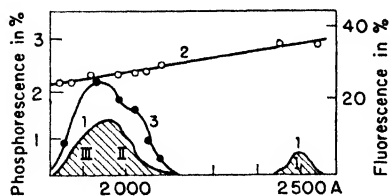
Fig. 191. Fluorescence and phosphorescence yield of a KCl(Tl)-phosphor (Buenger).
