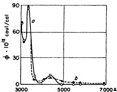
Fig. 177. Excitation spectrum of the photoelectric emission of a CaS(Bi)-phosphor (Goethel).
