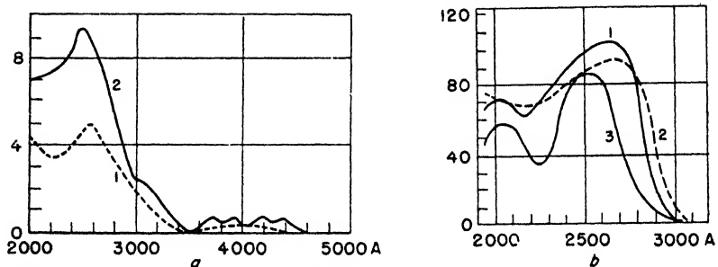
Fig. 200. Excitation and absorption spectra of zinc silicate phosphors.
