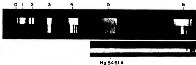
Fig. 148. Absorption and fluorescence spectrum of \text{Tb}_2(\text{SO}_4)_3 \cdot 8\text{H}_2\text{O} at -180^\circ \text{C} . (Gobrecht).
