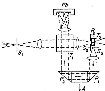
FIG. 5. Supersonic fluorimeter (Maercks).
