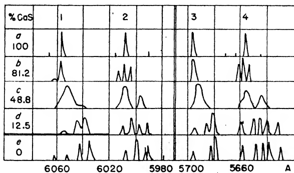
Fig. 155. Wavelength shift in two \text{Sm}^{+++} doublets in mixed crystals of CaS-SrS with increasing Sr-concentration (Tomaschek).
