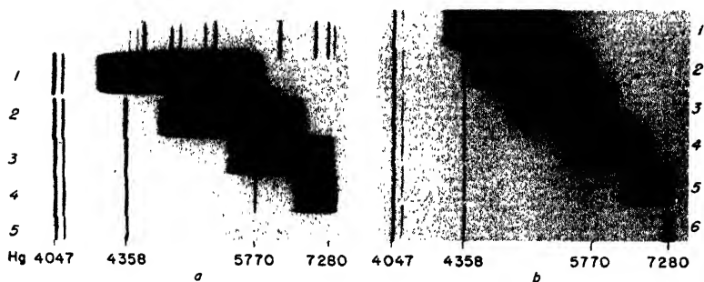
Fig. 198A. Phosphorescence spectra of mixed Zn,CdS-phosphors (Rothschild).
