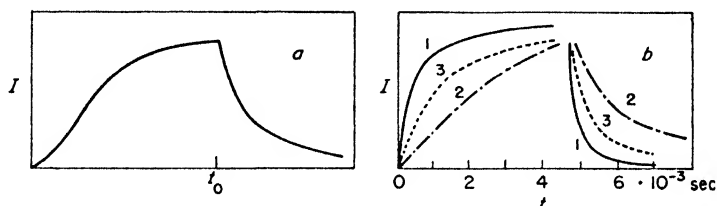
Fig. 186. Induction and decay curves for a second-order (recombination) luminescence, (a) theoretical curve, (b) experimental curves obtained with a ZnS(Cu)-phosphor.
