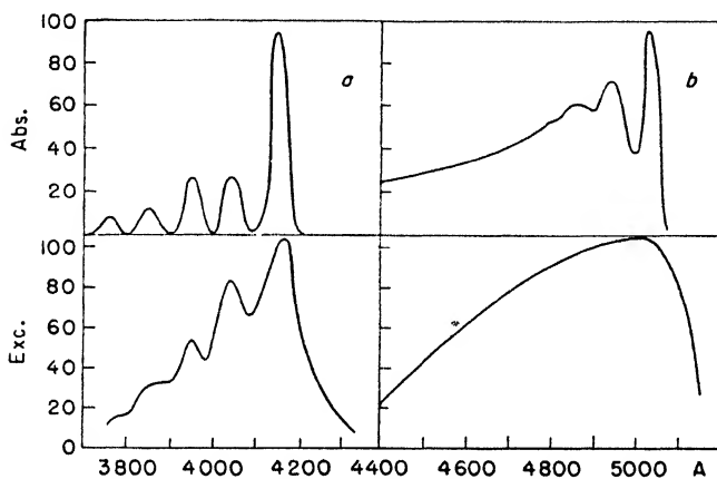
Fig. 216. Absorption and excitation spectra of diamonds (Mani).
