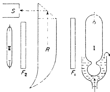
Fig. 16a. Wood's setup for the observation of stepwise excitation of mercury fluorescence.
