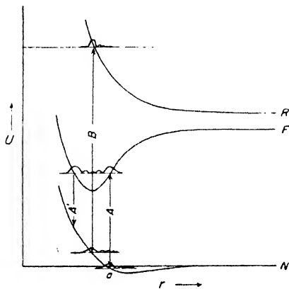
Fig. 83. Potential curves and eigenfunctions of molecules formed in a collision process [Finkelburg (393)].
