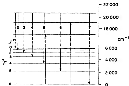
Fig. 150. Energy levels of Tb^{3+} (Gobrecht).
