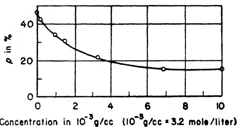
Fig. 128. Depolarization of fluorescence of fluorescein sodium in glycerol as a function of the dye concentration (Chauchois).
