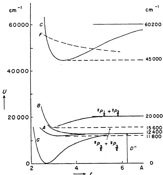
Fig. 64. Potential curves of the I_2 -molecule [after Curtis and Evans (254)].
