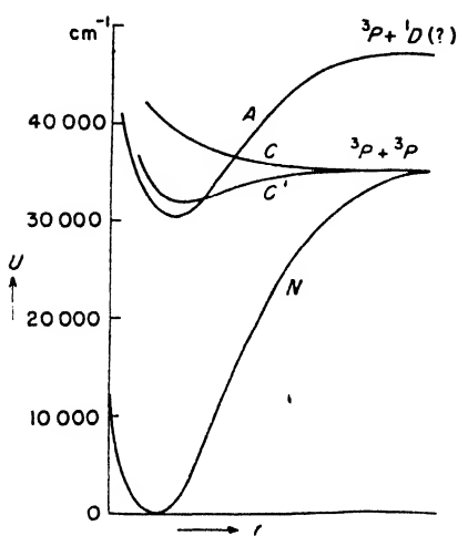
Fig. 75. Potential curves of S_2 (Rosen).
