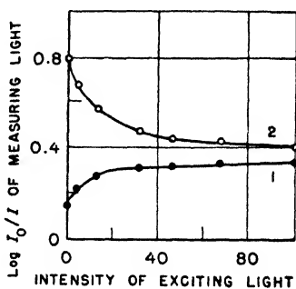
Fig. 107. Effect of intensity of exciting light on the absorption of fluorescein in boric acid [Lewis, Lipkin, and Magel (930)]. 1: 6500A. 2: 4360A.
