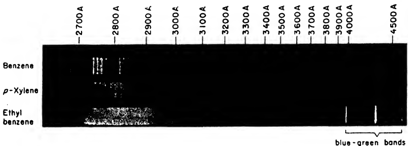
Fig. 92. Fluorescence spectra of benzene, p -xylene, and ethyl benzene (Marsh).
