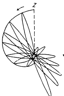
Fig. 30. Precession of a damped linear electric oscillator in a weak magnetic field perpendicular to E (Hanle).
