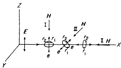
Fig. 22. Orientation of electric oscillators in a magnetic field H .
