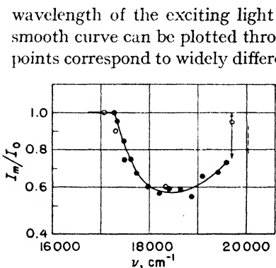
Fig. 73. Quenching of the \text{I}_2 -fluorescence by a magnetic field [Turner (1713)].
