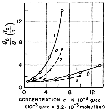
Fig. 117. Yield and lifetime of the fluorescence of fluorescein sodium in water (a) and in glycerol (b) as a function of the dye concentration (Szymanowski). 1: yield. 2: lifetime.
