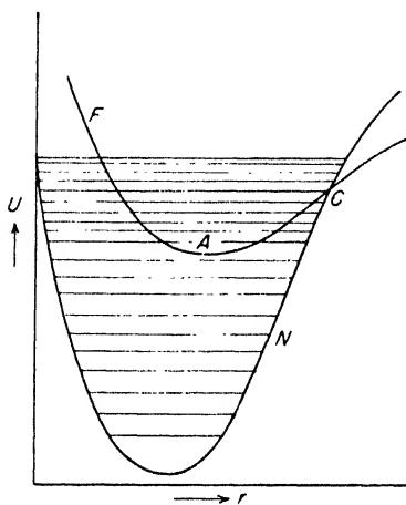
Fig. 84. Configuration potential curves for internal conversion.
