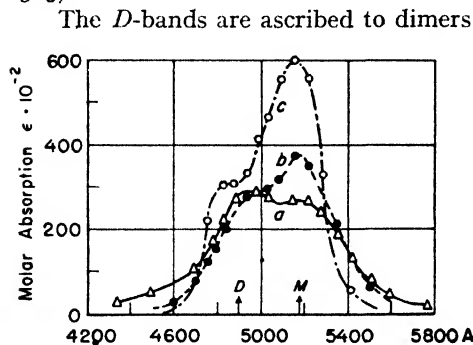
Fig. 119. Absorption bands of eosin in aqueous solutions at various dye concentrations (Soederberg).
