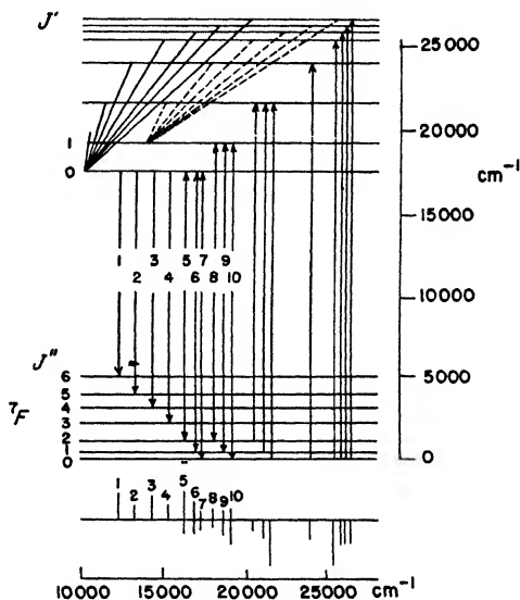
Fig. 149. Energy levels of \text{Eu}^{++} (Tomaschek and Gobrecht).
