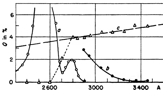
Fig. 105. Absorption and excitation spectra of magnesium platinocyanide in aqueous solution (Khvostikov).
