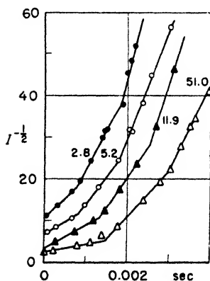
Fig. 95. Decay of fluorescence of uranyl salts at intensities varying from 2.8 to 51.0 (in arbitrary units) (Nichols and Merritt).
