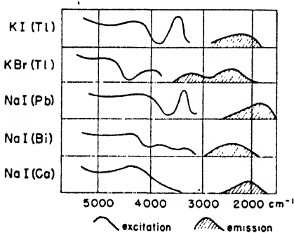
Fig. 206. Excitation and emission bands of surface-activated alkali halides (Terenin).
