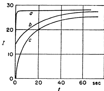
Fig. 185. Induction curves of a ZnS(Mn)-phosphor (Garlick and Wilkins).
