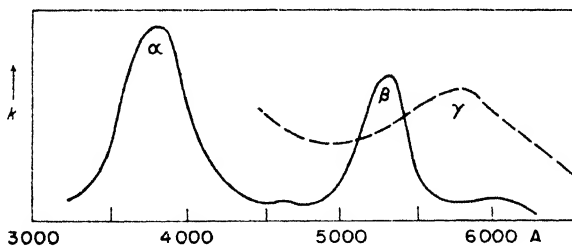
Fig. 217. Absorption bands of \text{CaF}_2 discolored by exposure to Ca-vapor (Mollwo).
