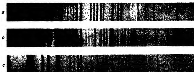
Fig. 170. X-ray diagrams of zinc silicate phosphors (Rooksby and McKeag).
