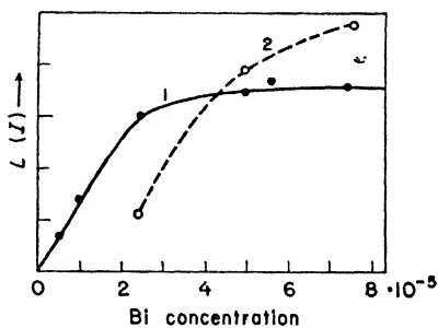
Fig. 193. Saturated light sum I and fluorescence intensity I of a CaS(Bi)-phosphor as a function of the Bi-concentration in g Bi per g phosphor (Lenard).
