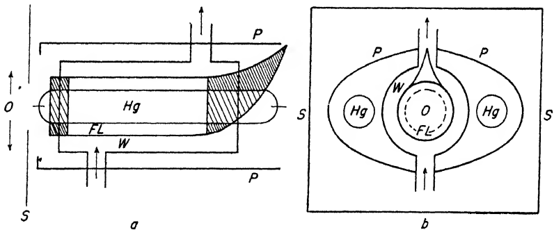
FIG. 8. Wood's device for high intensity excitation of fluorescence.
