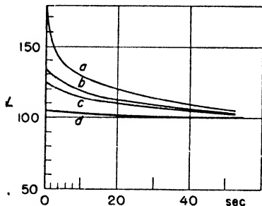
Fig. 194. Decay of the phosphorescence of a CaS(Bi)-phosphor of various Bi-concentrations during the first 60 sec (Kuppenheim).
