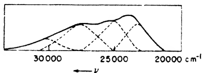
Fig. 171. Analysis of a complex emission band of a CaO(Ag)-phosphor (Schellenberg).
