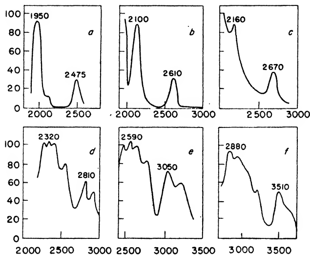
Fig. 202. Absorption bands of Tl- and Sn-activated alkali halide phosphors (Forró, Hueniger, and Rudolph).
