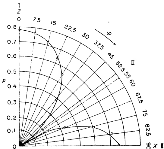
Fig. 23. Polarization of Hg-resonance radiation as a function of \varphi , the angle between H and E (Olsen).
