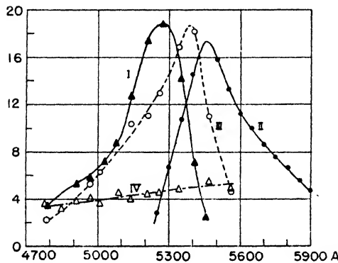
Fig. 103. Absorption, excitation, and emission spectra of eosin in aqueous solution (Nichols and Merritt).
