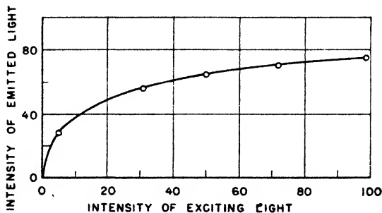
Fig. 98. Intensity of the phosphorescence of fluorescein in boric acid as a function of the exciting radiation at 18° C (Lewis, Lipkins, and Magel).
