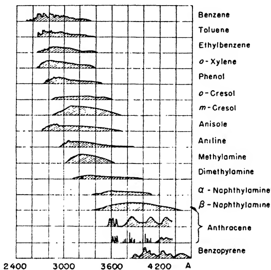
Fig. 94. Schematic drawing of the fluorescence spectra of various aromatic vapors.
