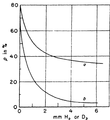
Fig. 40. Apparent ( a ) and real ( b ) depolarization of Hg-resonance radiation by hydrogen and deuterium (Suppe).
