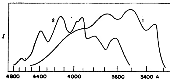
Fig. 134b. Fluorescence spectrum of trans -stilbene (Lewis, Magel, and Lipkin) in ether-alcohol mixture at -90^{\circ}\text{C} . (1) and crystalline at -190^{\circ}\text{C} . (2).
