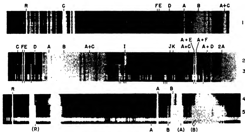
Fig. 161. Fluorescence spectra of uranyl salts.
