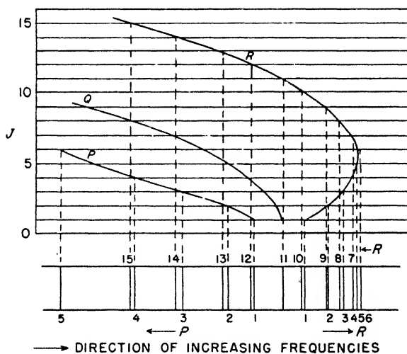
Fig. 55. Fortrat diagram for a band system with P -, Q -, and R -branches.
