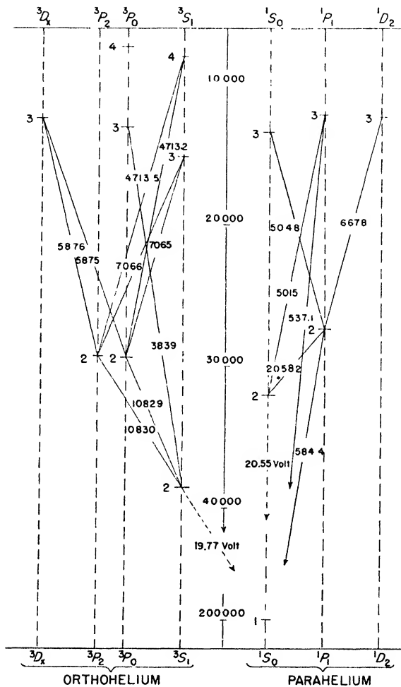
Fig. 17. Grotrian diagram for He.
