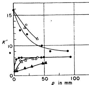
Fig. 76. Influence of foreign gases on the rotational structure of CN band at 3883A (Jakowlewa): A(●); N_2 (Δ); CO(○); H_2 (▲).
