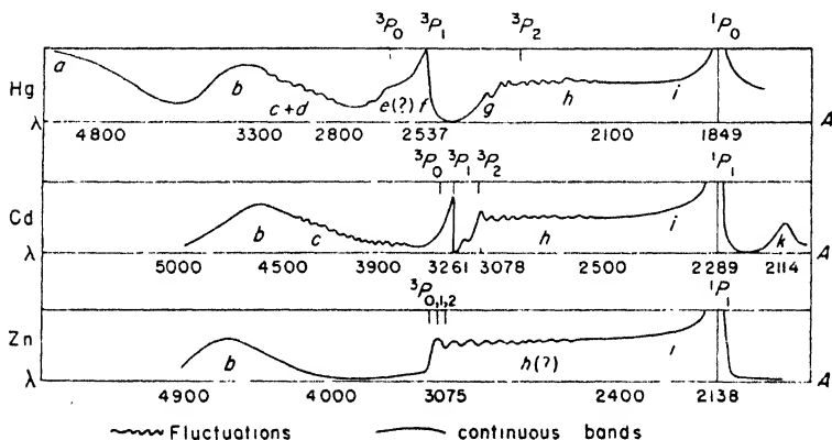
Fig. 82. The fluorescence bands of \text{Hg}_2 , \text{Cd}_2 , and \text{Zn}_2 (Mrozowski).
