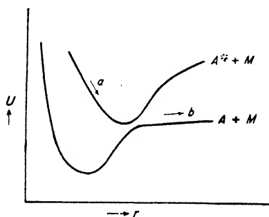
Fig. 49. Potential curves for quenching without transfer of excitation energy (Laidler).
