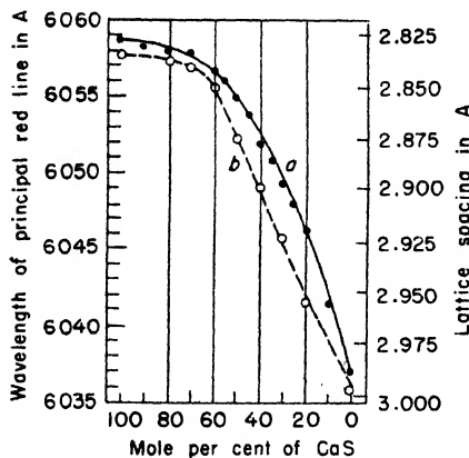
Fig. 154. Shift of the wavelength of a line in the fluorescence spectrum of \text{Sm}^{+++} imbedded in mixed crystals of \text{CaS} - \text{SrS} with increasing lattice spacing (Travnicek).
