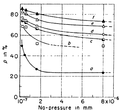
Fig. 43. Circular polarization of Na-resonance radiation as a function of Na-vapor pressure at various magnetic field strengths (Hanle).
