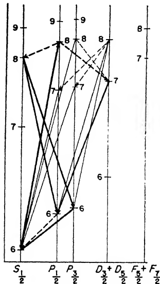
FIG. 13. Grotrian diagram for the fluorescence of Cs.
