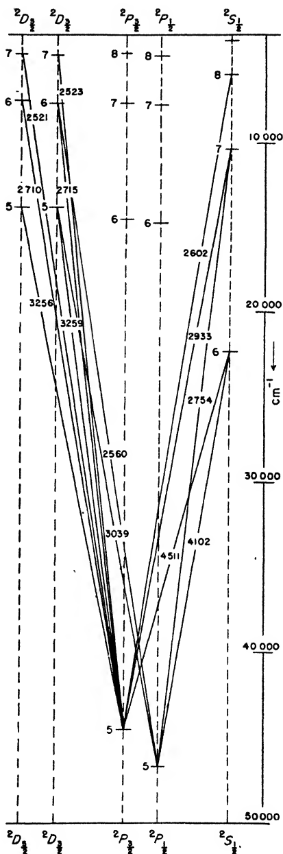
Fig. 53. Grotrian diagram of indium (Donat).
