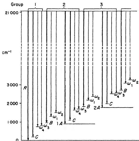
Fig. 162. Energy levels for the first three groups of the fluorescence spectrum of \text{CsUO}_2(\text{NO}_3)_3 . Heavy lines: \text{UO}_2 -vibrations; light lines: \text{NO}_3 -vibrations. The C and \omega levels are multiplets; concerning the interpretation of \omega_1 - \omega_3 , compare Table 103.
