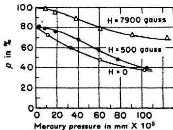
Fig. 42. Polarization of Hg-resonance radiation as a function of Hg-vapor pressure (Keussler).
