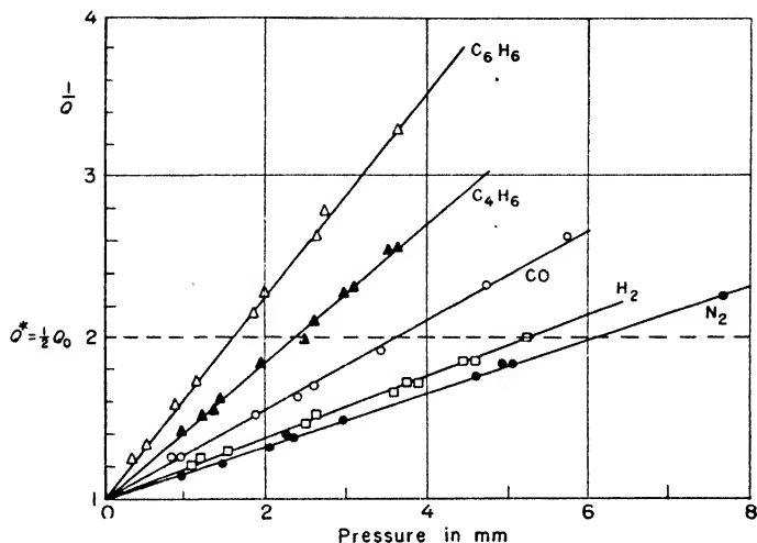
Fig. 46. Quenching of Na-resonance radiation by various gases (Norrish and Smith).
