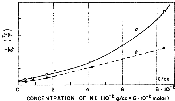
Fig. 109. Yield and lifetime of fluorescence of fluorescein sodium in water quenched by KI (Szymanowski).
