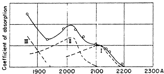
Fig. 78. Excitation spectra (broken line) of TII photodissociation (Frank). The continuous line in the absorption spectrum.
