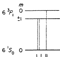
Fig. 33. Level diagram for Stark effect of Hg-line 2537A.
