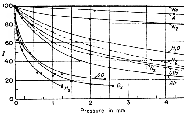
Fig. 45. Quenching of Hg- (continuous lines) and Na-resonance (broken lines) radiation by various gases (Mannkopf and Stuart).
