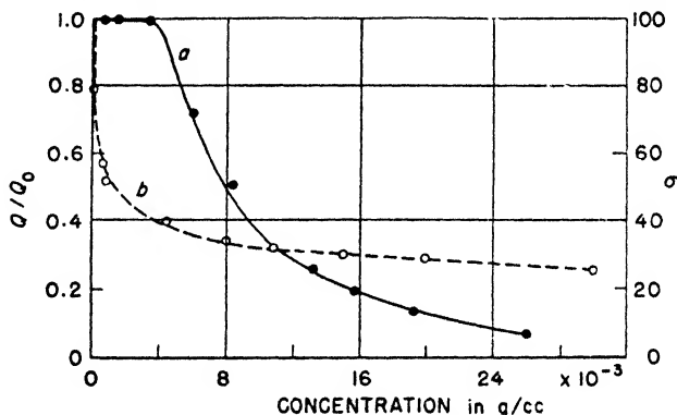
Fig. 125. Fluorescence yield and electric conductivity of an aqueous fluorescein solution as a function of the dye concentration (Vavilov).
