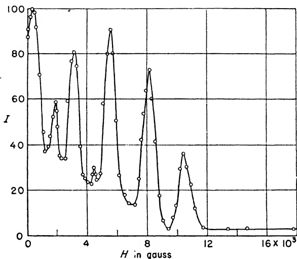
Fig. 18. Magnetic resolution of the hyperfine structure of the Hg-resonance line by the Schein method (Buhl). I = transmitted energy.
