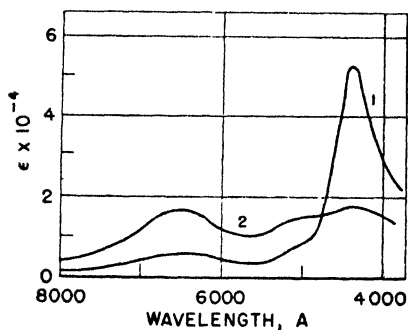
Fig. 106. Absorption spectrum of fluorescein in boric acid [Lewis, Lipkin, and Magel (930)]. 1: in ground state N . 2: partially excited quasi-stable state M .
