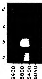
Fig. 144. Fluorescence and phosphorescence of erythrosin (Pringsheim and Vavilov).
