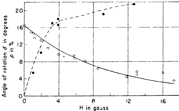
Fig. 32. Depolarization (continuous line) and rotation of plane of polarization (broken line) of sodium resonance radiation observed in the direction parallel to the magnetic field H .
