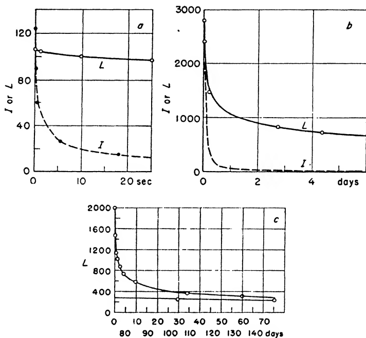
Fig. 187a-c. Decay curves of a CaS(Bi)-phosphor (Lenard). I : intensity. L : light sum.
