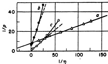
Fig. 127. Polarization of fluorescence as a function of the viscosity (Pringsheim and Vogels).
