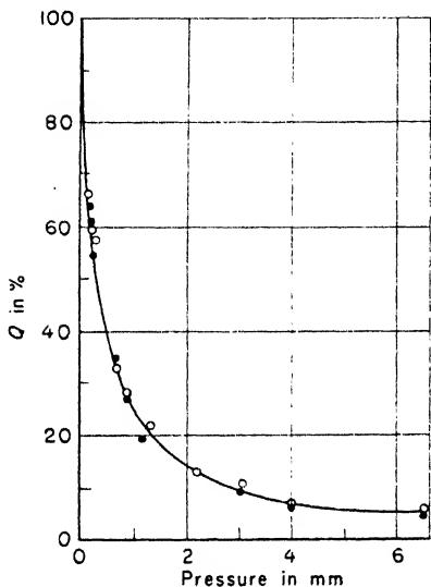
Fig. 48. Quenching of Hg-resonance radiation by H_2 (closed circle) and D_2 (open circle) (Suppe).
