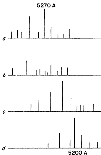
Fig. 166. Structure of the band at 5250 Å in the fluorescence spectra of various uranyl nitrates (Nichols and Merritt).
