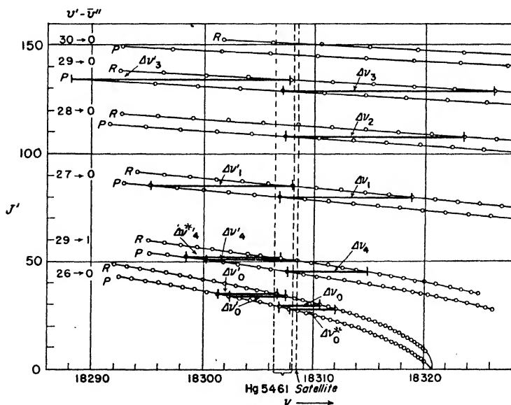
Fig. 62. Fortrat diagram for the doublets of zero order excited in I 2 -vapor by the green Hg-line.
