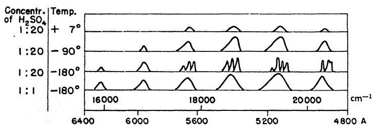
Fig. 167. Fluorescence spectra of solutions of uranyl potassium sulfate in water with addition of increasing quantities of sulfuric acid (Nichols and Merritt).
