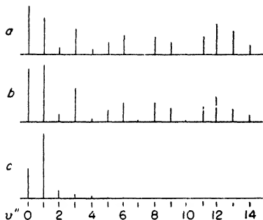
Fig. 69. Intensity distribution in the \text{Na}_2 resonance spectrum excited by Cd-line 4800A (Brown).
