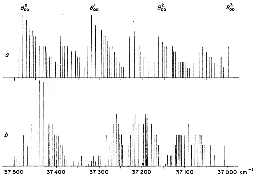
Fig. 91. Schematic representation of part of benzene fluorescence spectrum (Ingold and Wilson).
