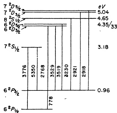
FIG. 9. Level diagram for the fluorescence of Tl [Mueller (1084)].
