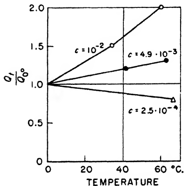
Fig. 122. Influence of temperature on the self-quenching of fluorescein in aqueous solutions (Levshin).
