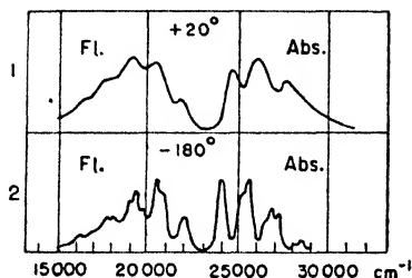
Fig. 141. Fluorescence and absorption bands of diphenyloctatetraene (Kuhn and Hausser).
