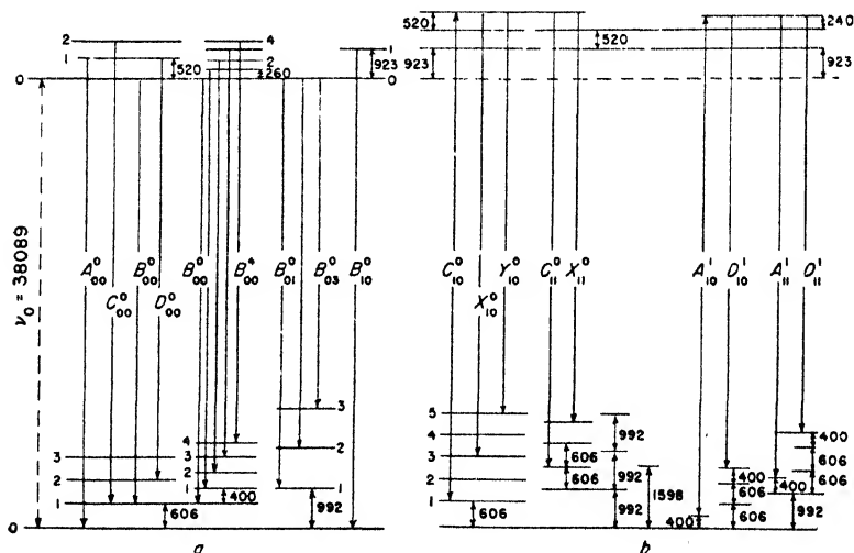
Fig. 90. Energy-level diagrams for fluorescence of benzene.
