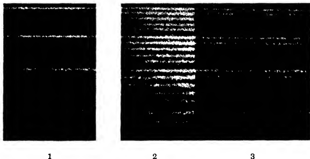
Fig. 37. Transfer of Hg-hyperfine-structure component - 25.4 by collisions of excited Hg-atoms with He-atoms (Mrozowski).
