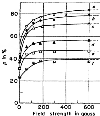
Fig. 41. Depolarization of circularly polarized Na-resonance radiation by He-Ne mixture at various magnetic field strengths (Hanle).
