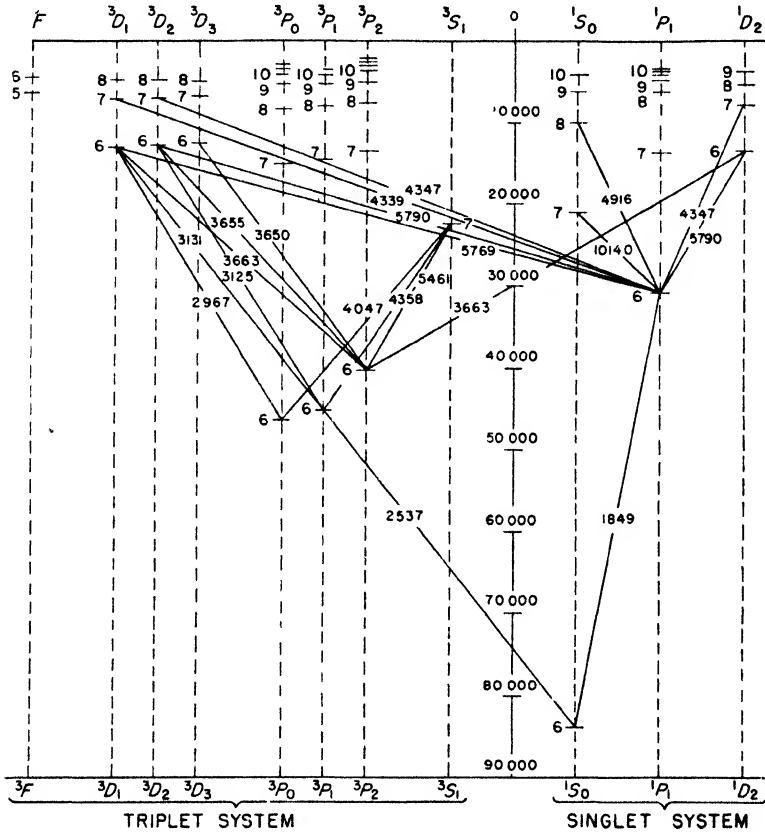
Fig. 15. Grotrian diagram for Hg.
