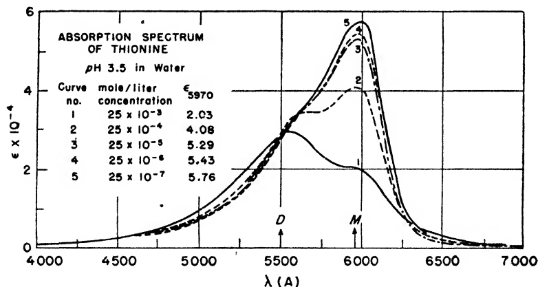
Fig. 120. Molar extinction coefficient of thionine in water [Rabinowitch and Epstein (1317 a )]
