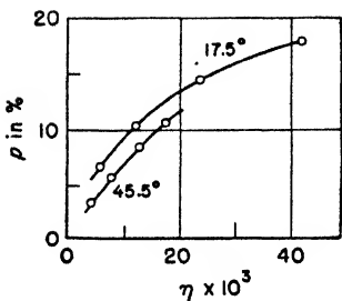
Fig. 126. Polarization of fluorescence of erythrosin in various alcohols as a function of the viscosity [Levshin (909)]
