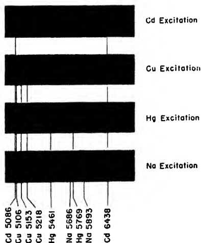
Fig. 63. Resonance spectra of I_2 excited by various lines.
