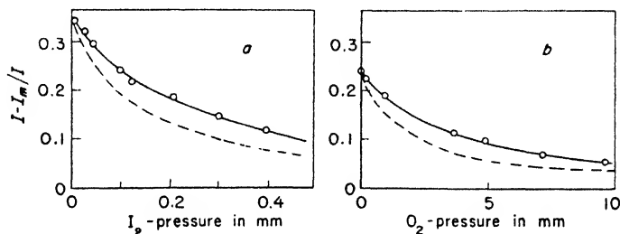
Fig. 74. Simultaneous action of collisions and a magnetic field on the I_2 -fluorescence (Berg).
