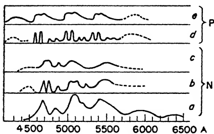
Fig. 146. Emission spectra of "boric acid phosphors" and "progressive phosphorescence" at liquid-air temperature. (a: after a photometer curve; b-e: from drawings after visual observation).
