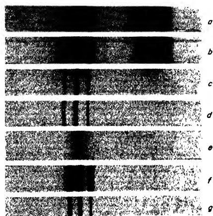
Fig. 182. Luminescence spectra of samarium-activated CaS-phosphors (Rothschild).
