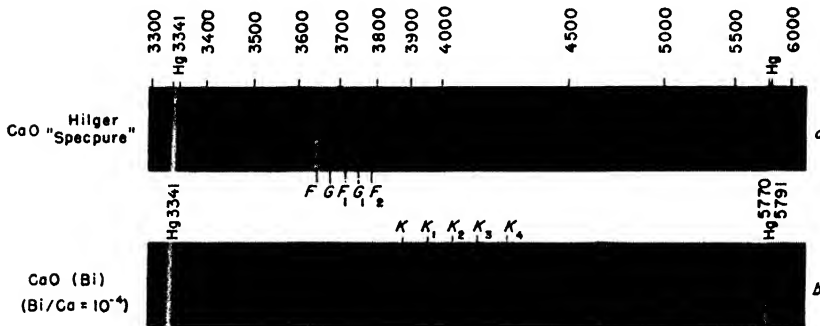
Fig. 199. Fluorescence spectra of CaO at -190^{\circ}\text{C} (Ewles). a : pure CaO. b : CaO with 10^{-2}\% Bi.
