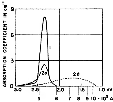
Fig. 173. Absorption bands of NaCl containing F -centers (Pick). 1: F -band of crystal in normal state. 2a: reduced F -band. 2b: F' -band of excited crystal.
