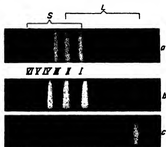
Fig. 208. Luminescence spectrum of a CO-activated KCl-phosphor (Roos). a : luminescence during the excitation. b : after-glow 0.25 sec after the end of the excitation. c : phosphorescence 1 sec after the end of the excitation.
