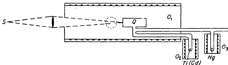
Fig. 51. Apparatus for production of sensitized fluorescence (Cario). S: light source. Q: resonance lamp. O_1 , O_2 , and O_3 : electric ovens.
