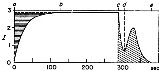
Fig. 189. Induction deficiency and stored light sum of a ZnS(Cu)-phosphor: a-b : induction period; a-c : period of constant excitation; c-d : spontaneous decay; d-e : I driven out by heating (Randall).
