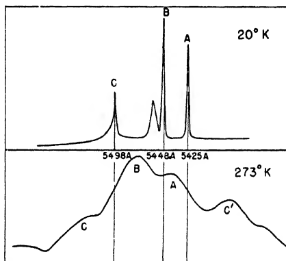
Fig. 164. Photometer curves of the third group in the fluorescence spectrum of \text{Cs}_2\text{UO}_2\text{Cl}_4 at 20^\circ and 273^\circ \text{K} .
