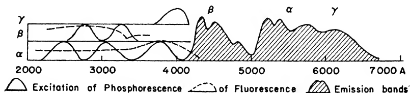
Fig. 210b. Excitation and emission bands of carbon-activated boron nitride phosphors (Tiede).
