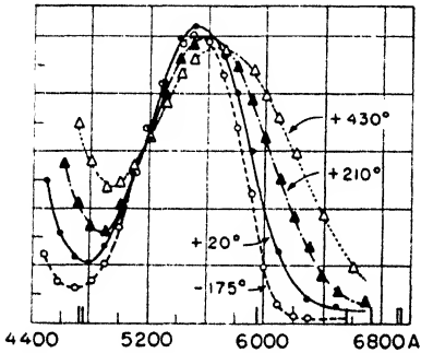
Fig. 215. Absorption band of ruby at various temperatures.
