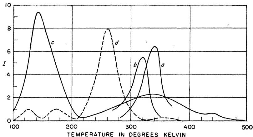
Fig. 181. Glow curves for various phosphors (Randall).
