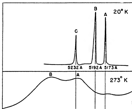
Fig. 165. Photometer curves of the third group in the fluorescence spectrum of \text{Cs}_2\text{UO}_2(\text{NO}_3)_3 at 20^\circ and 273^\circ K.
