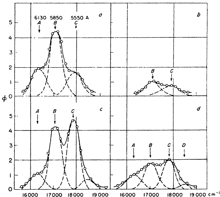
Fig. 195. Phosphorescence spectrum of a ZnS(Mn)-phosphor (Nitka). Wavelength of exciting light: (a) 4358Å; (b) 4047Å; (c) 3655Å; (d) 3132Å.
