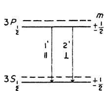
Fig. 34. Level diagram for Stark effect of Na-line D_1 .
