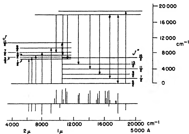
Fig. 151. Energy levels of Sm^{3+} (Gobrecht).
