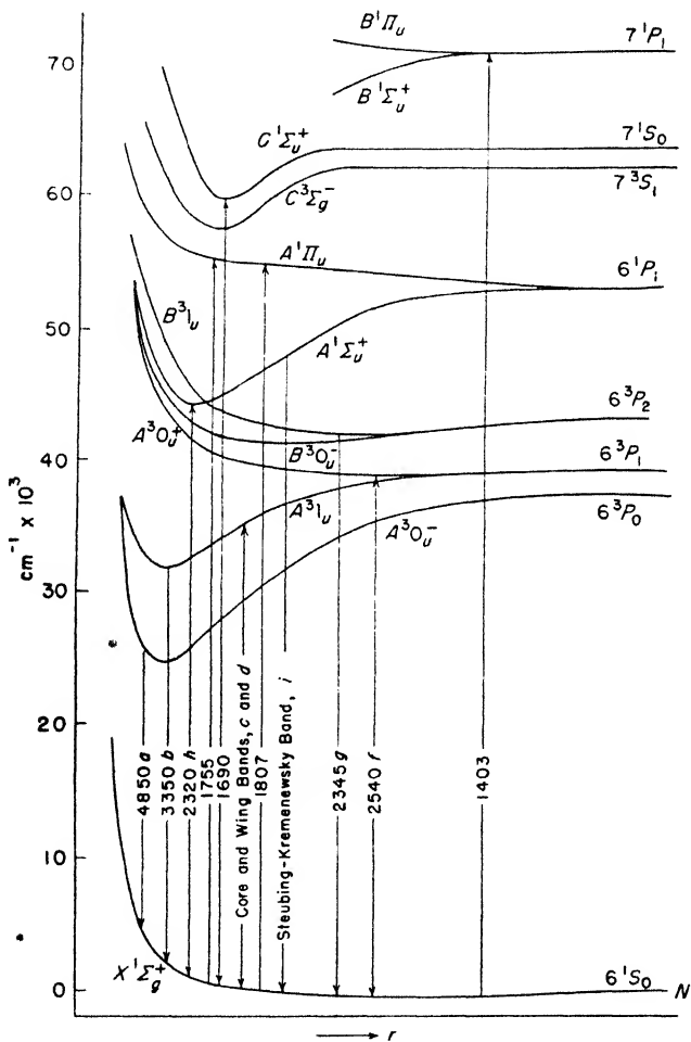
Fig. 81. Potential curves of Hg 2 (Mrozowski).
