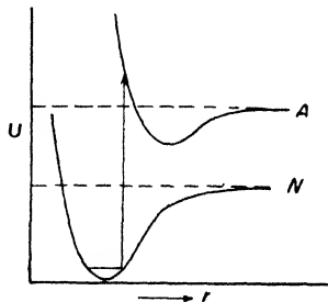
Fig. 59. Potential curves of a molecule with a continuous band prevailing in the absorption spectrum.
