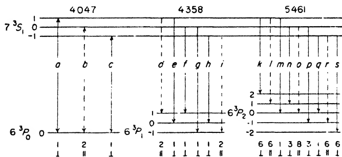
Fig. 28. Magnetic sublevels for stepwise-excited Hg-fluorescence [Richter (1357)]. The numbers below the diagram indicate the relative intensities of the components.
