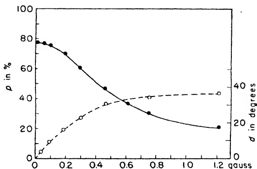
Fig. 31. Depolarization (continuous line) and rotation of plane of polarization (broken line) of Hg-resonance radiation observed in the direction parallel to the magnetic field H (Keussler).
