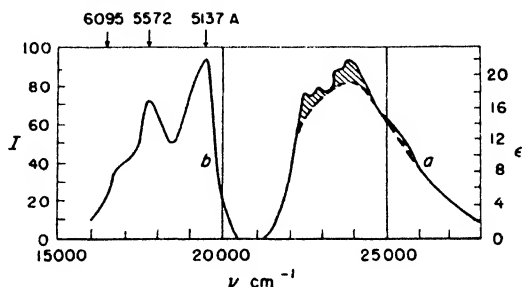
Fig. 88. Absorption and fluorescence spectrum of biacetyl vapor at room temperature (Lewis and Kasha).
