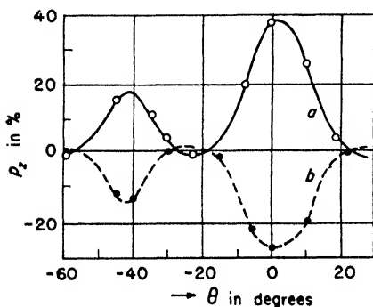
Fig. 130. Polarization of the fluorescence of euchrysrine adsorbed on cellophane as a function of the angle \theta between Z and \zeta (Jablonski).
