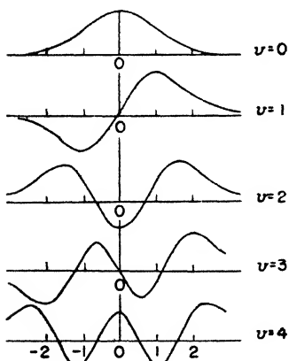
Fig. 58. Eigenfunctions of the five lowest vibrational states of a harmonic oscillator.
