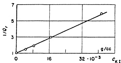
Fig. 108. Quenching of the fluorescence of fluorescein sodium in aqueous solution by KI of various concentrations (Vavilov).
