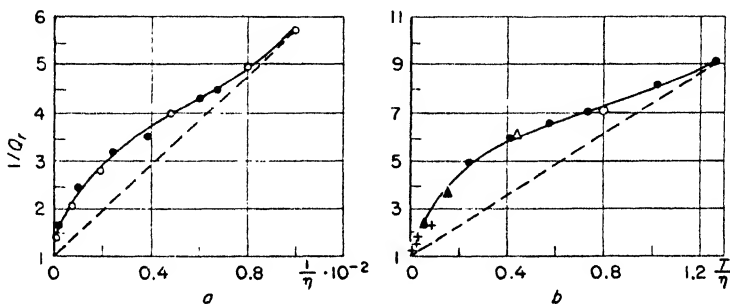
Fig. 110. Quenching of the fluorescence of fluorescein (a) by potassium iodide and (b) by aniline as a function of viscosity [Sveshnikov (1600)]
