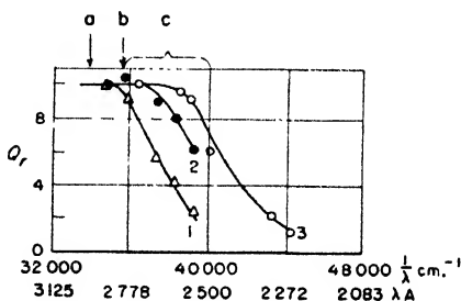
Fig. 93. Spectral distribution of relative quantum yield of aniline fluorescence [Terenin, Vartanian, and Neporent (1648)].
