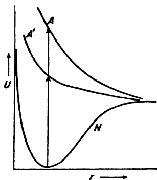
Fig. 112. Potential curves for the photosensitized decomposition of ethyl iodide.
