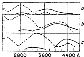
Fig. 142. Absorption and fluorescence spectra of aliphatic compounds dissolved in ethanol (Gelbke). Broken lines: absorption; continuous lines: emission.
