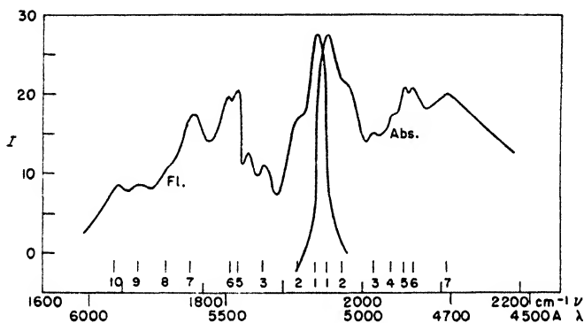
Fig. 100 b . Mirror symmetry of absorption and fluorescence bands.
