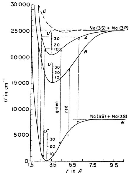
Fig. 68. Potential curves of Na 2 (Loomis and Nile).
