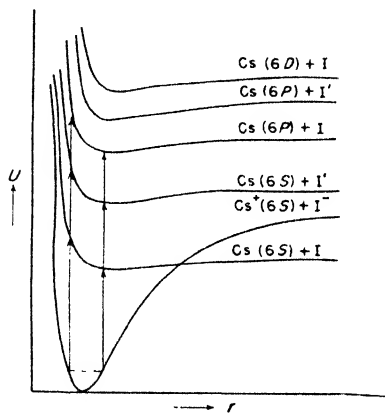
Fig. 77. Potential curves of CsI (Mulliken).
