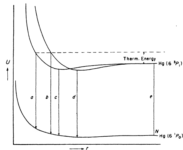
Fig. 80. Potential curves for the system rare gas-mercury (Oldenberg).
