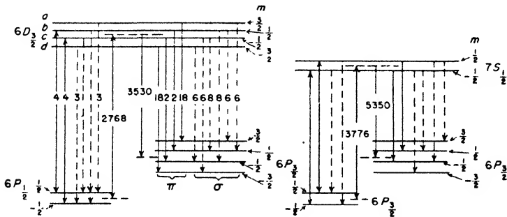
Fig. 27. Magnetic sublevels for the Tl-line 5350A [Guelke (547)]. The numbers indicate the relative intensities of the components.
