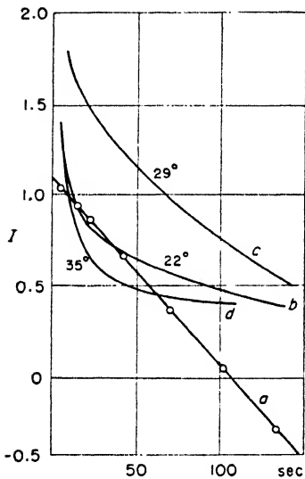
Fig. 190. Decay curves of KCl(Tl)-phosphors (Buenger and Flechsig, Randall).
