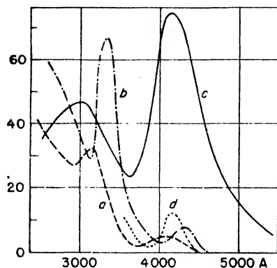
Fig. 176. Excitation spectra of a CaS(Bi)-phosphor.
